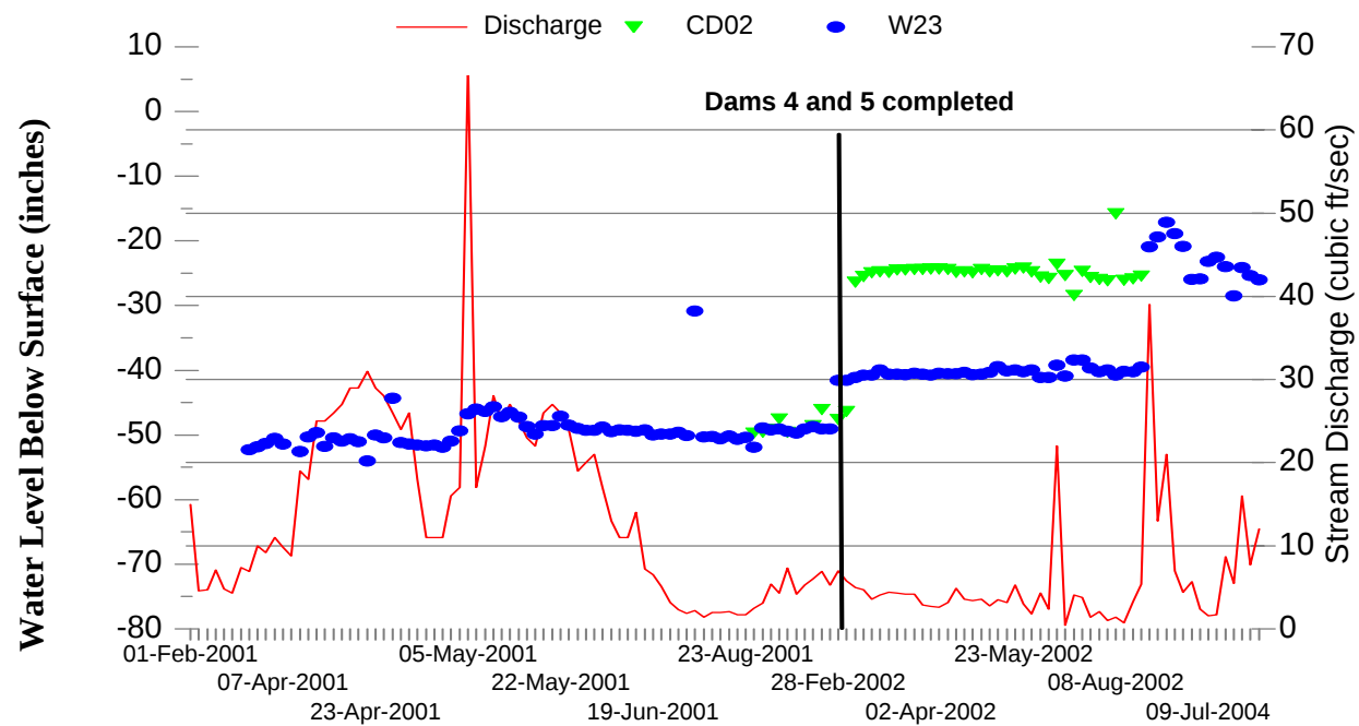
Figure 9. Groundwater Elevations in Two Monitoring Wells Between Check Dams 3 and 6 with Stream Discharge, 2001-2004, East Plum Creek, Douglas County, CO
