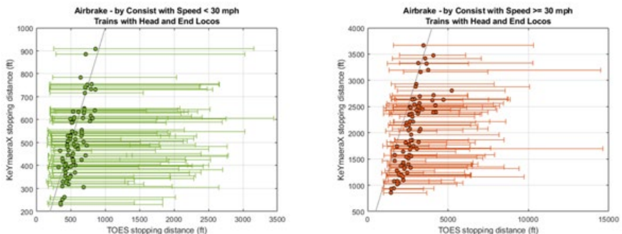
Figure 16. Airbrake model head-end locomotives – stopping distances by consist.
