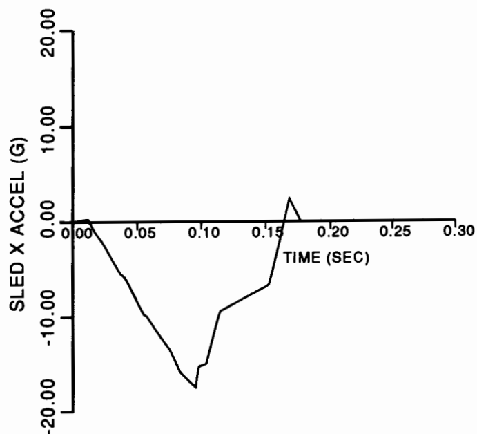
Figure 26. Test sled acceleration, test A87040.
