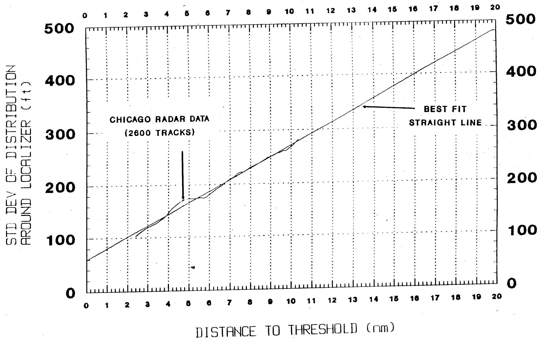
FIGURE 6. STANDARD DEVIATION OF AIRCRAFT FROM LOCALIZER (FT) AS A FUNCTION OF DISTANCE TO THRESHOLD (NMI)
