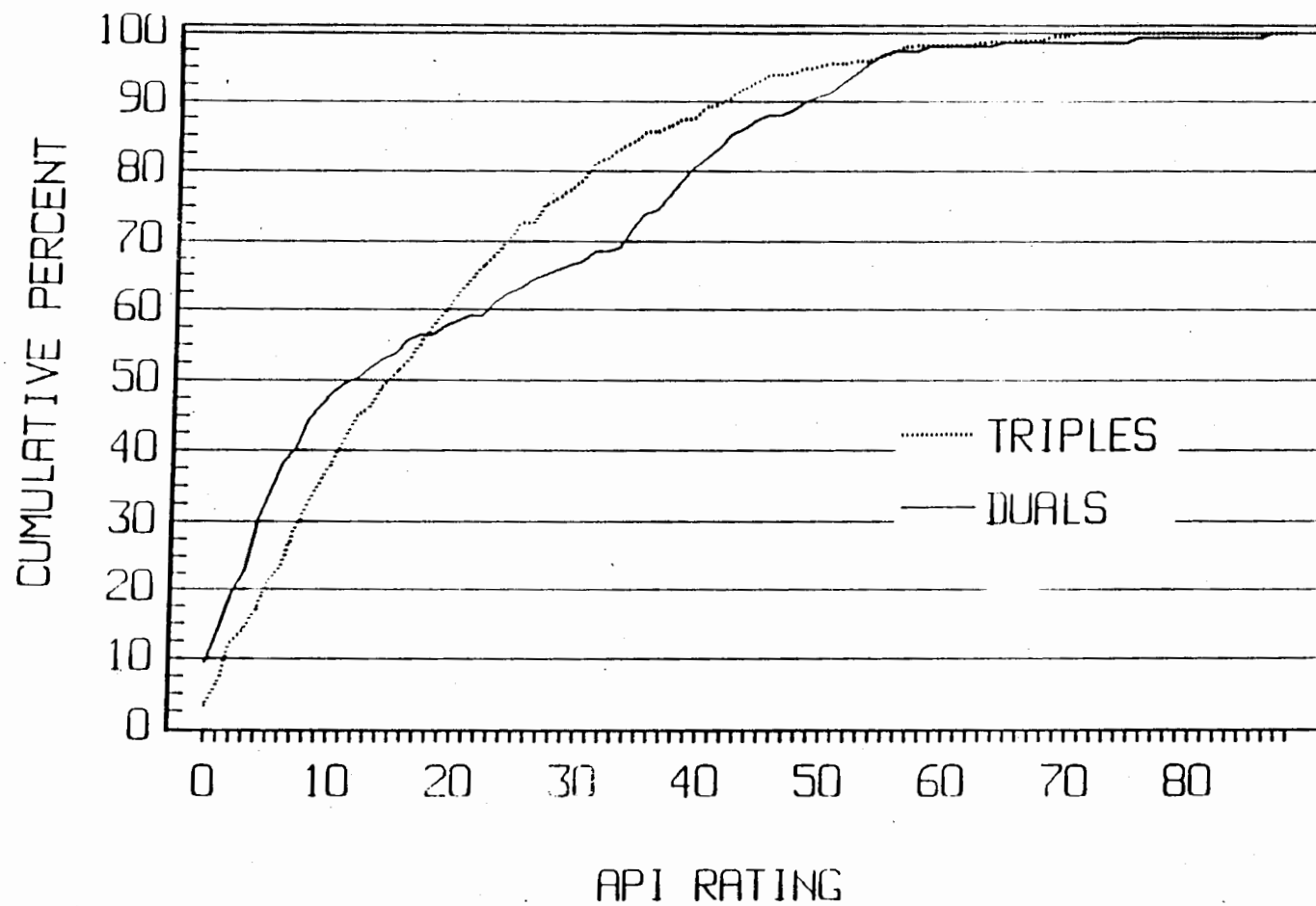
FIGURE 7. CUMULATIVE DISTRIBUTIONS OF API VALUES FOR DUAL AND TRIPLE APPROACH CONDITIONS
