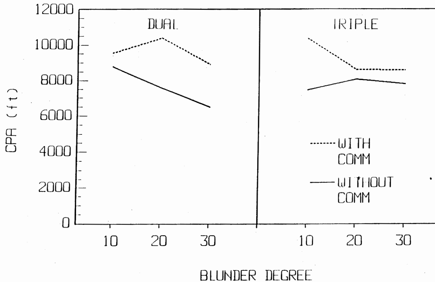
FIGURE 8. AVERAGE OF CPA VALUES AS A FUNCTION OF APPROACH CONDITION, DEGREE FO BLUNDER, AND COMMUNICATION CONDITION
