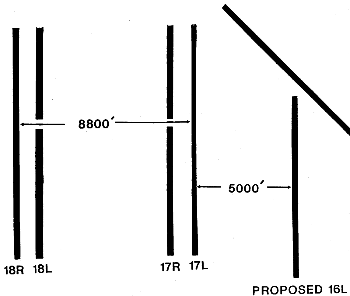
FIGURE 1. D/FW AIRPORT CONFIGURATION
