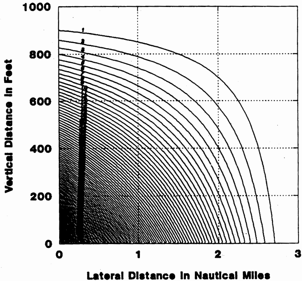
Figure 1. CONTOUR PLOT
