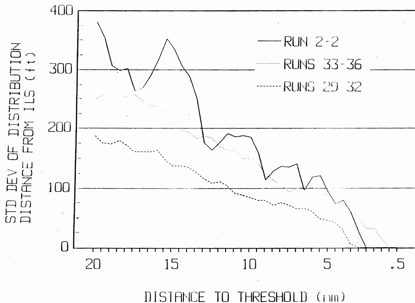
FIGURE 15. FLIGHT TECHNICAL ERROR FOR THE THREE NAVIGATIONAL MODELS USED IN D/FW PHASE II
