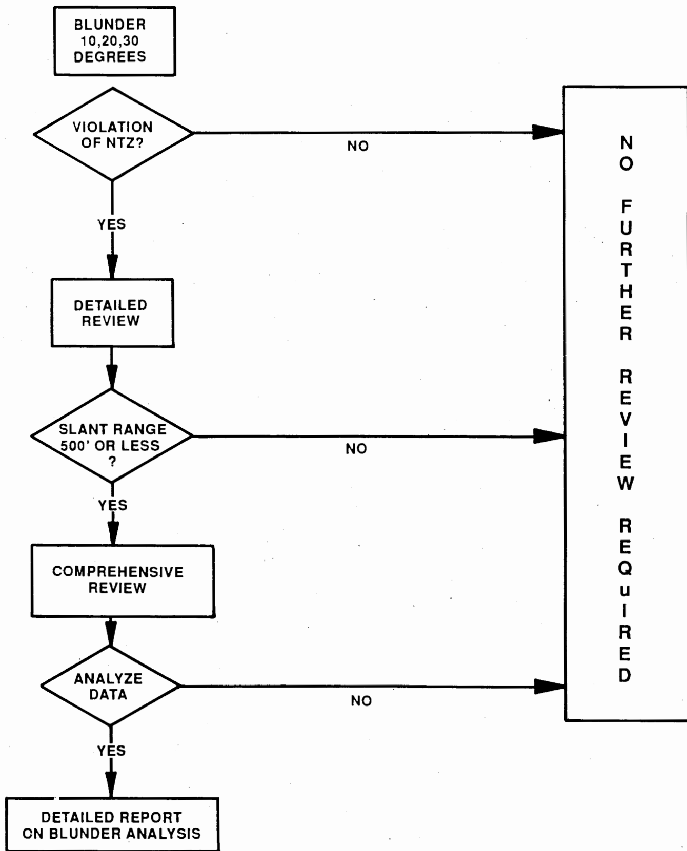
FIGURE 2. OPERATIONAL ASSESSMENT DECISION TREE
