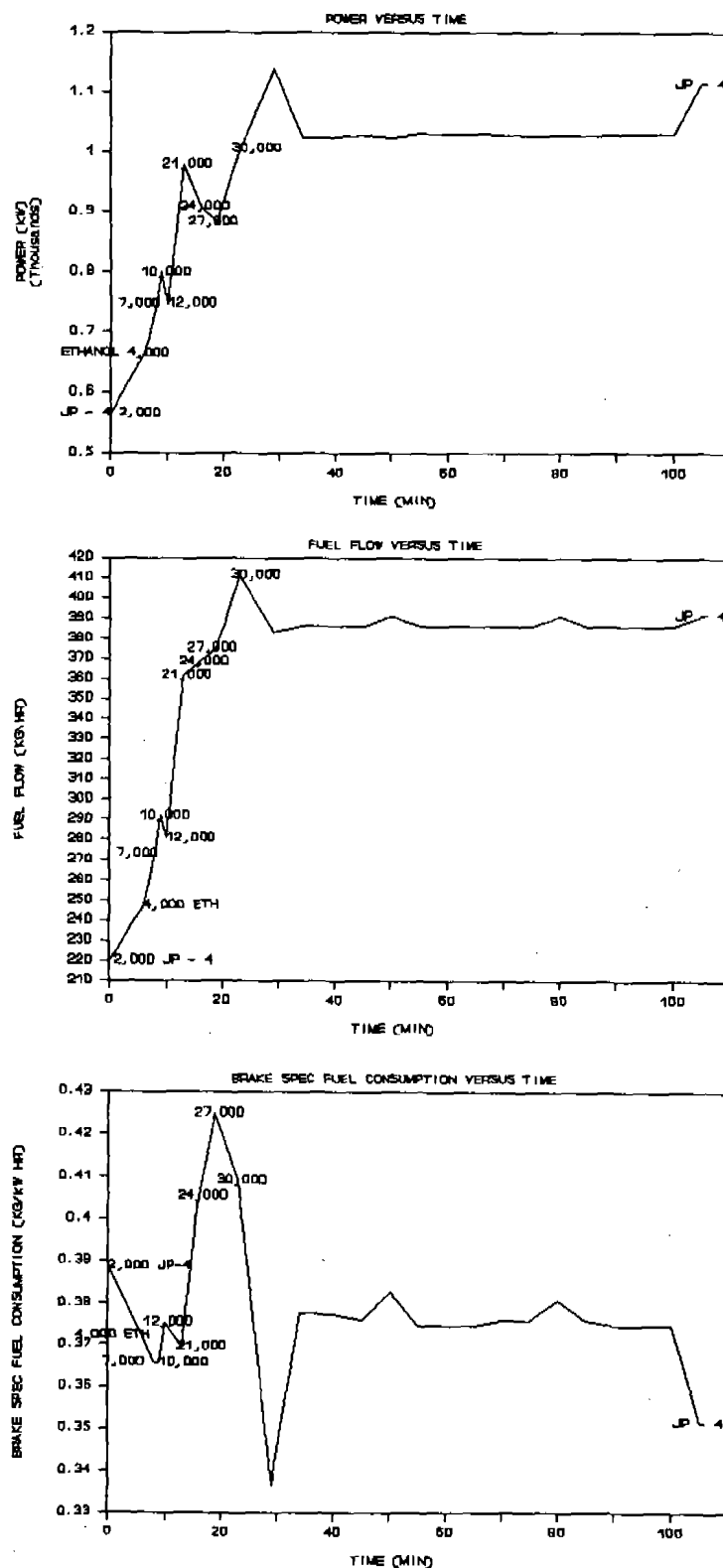
FIGURE A-9. EFFECTS OF 10 PERCENT ETHANOL DURING A 30,000-FOOT ALTITUDE ENDURANCE RUN AT MAXIMUM RANGE POWER
