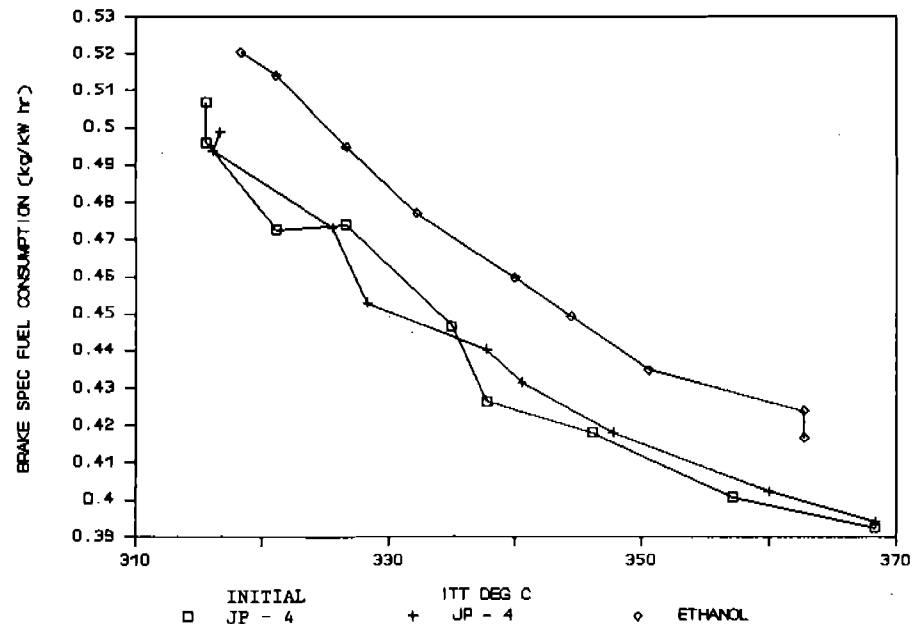
FIGURE 6. BRAKE SPECIFIC FUEL CONSUMPTION VERSUS ITT FOR THE GROUND RUNS
