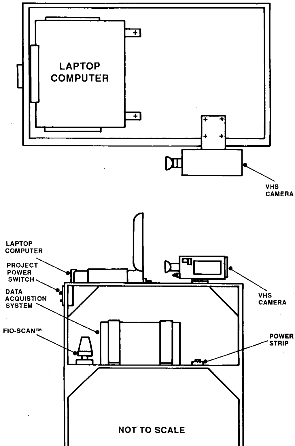
FIGURE 2. INSTRUMENTATION RACK - TOP AND SIDE VIEW
