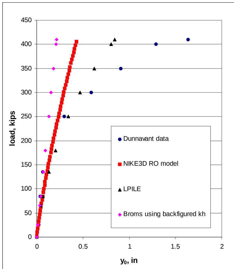
Figure B-21 Comparisons between Broms, LPILE, and NIKE3D for Dunnivant Case
