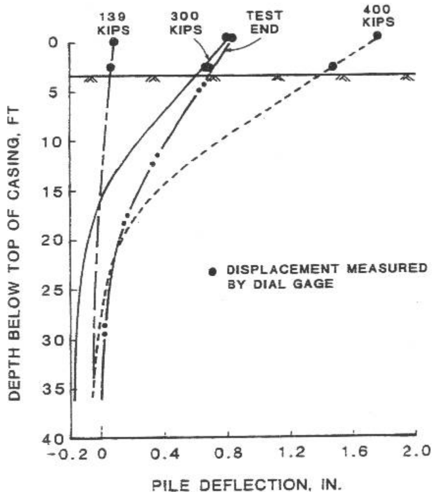
Figure B-7 Deformed Shapes of Dunnivant's Pier at Different Loads (Dunnivant's 1986)
