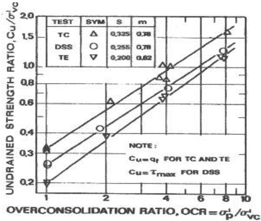
Figure 7-10 Unddrained Shear Strength Ratio vs. OCR for Marine Clay (Jamiolkowski et al. 1985).
