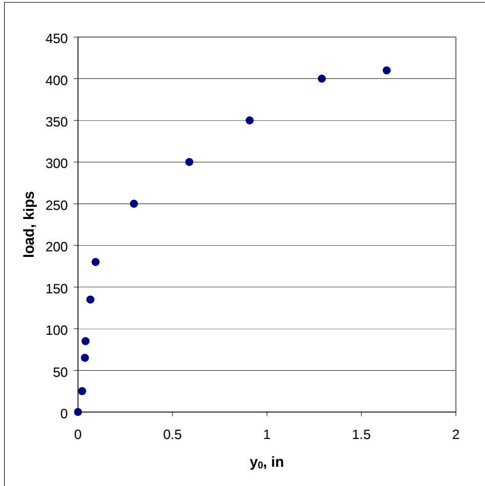
Figure B-6 Ground-line Deflections from Dunnavant Test
