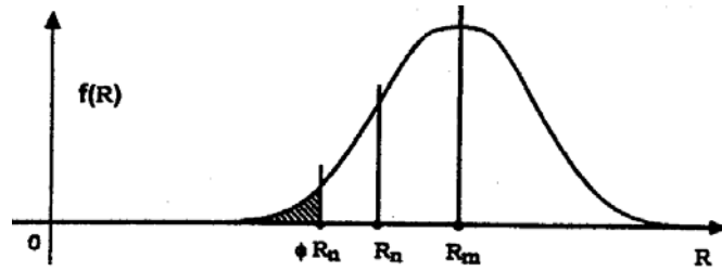
Figure 2.2 Probability Density Function for Resistance
