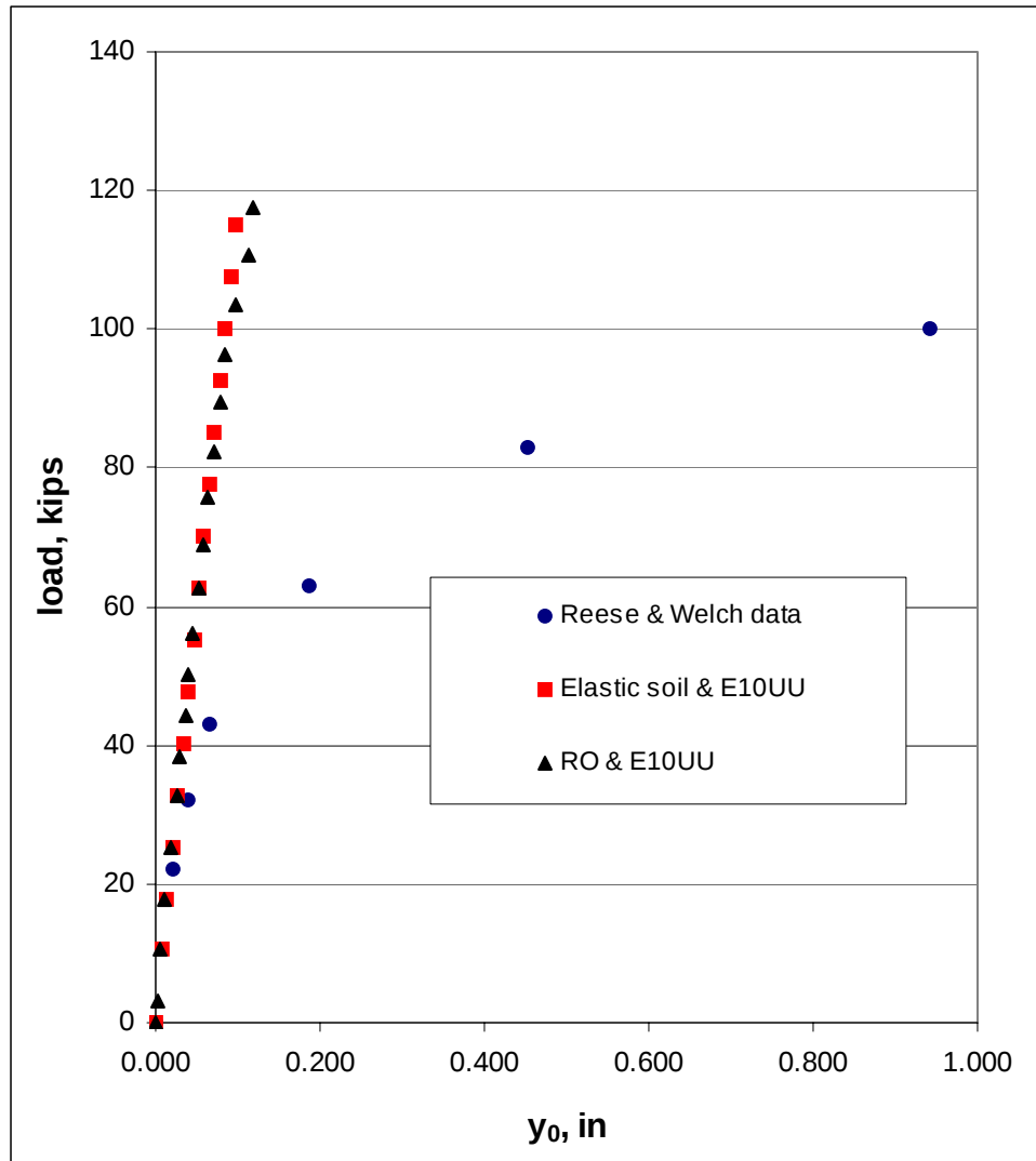
Figure B-16 NIK3D Elastic and RO Models of Ground-line Deflections with 3-layered Soil (5-ft, 15-ft, and 22-ft layers) using 10 times Elasticity from UU Tests
