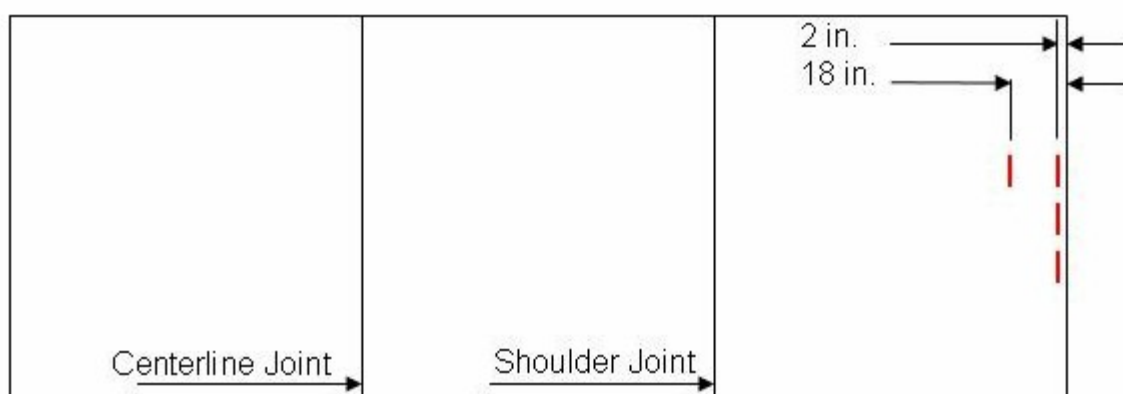
Instrumentation layout for the free edge.
