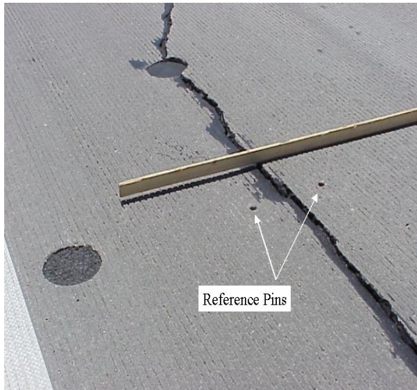
Figure 26: Differential Settlement
