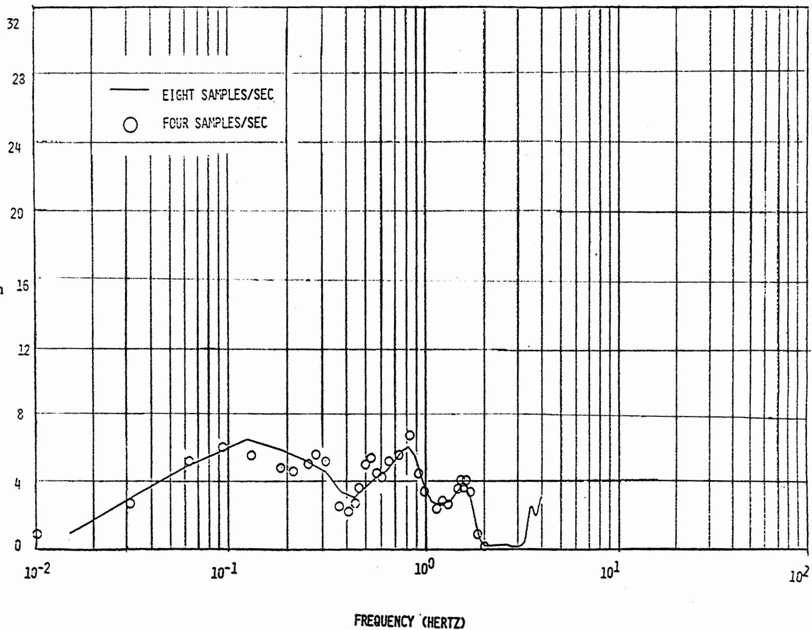
FIGURE A-3.- Effect of sample rate on definition of power spectra: L 1011.
