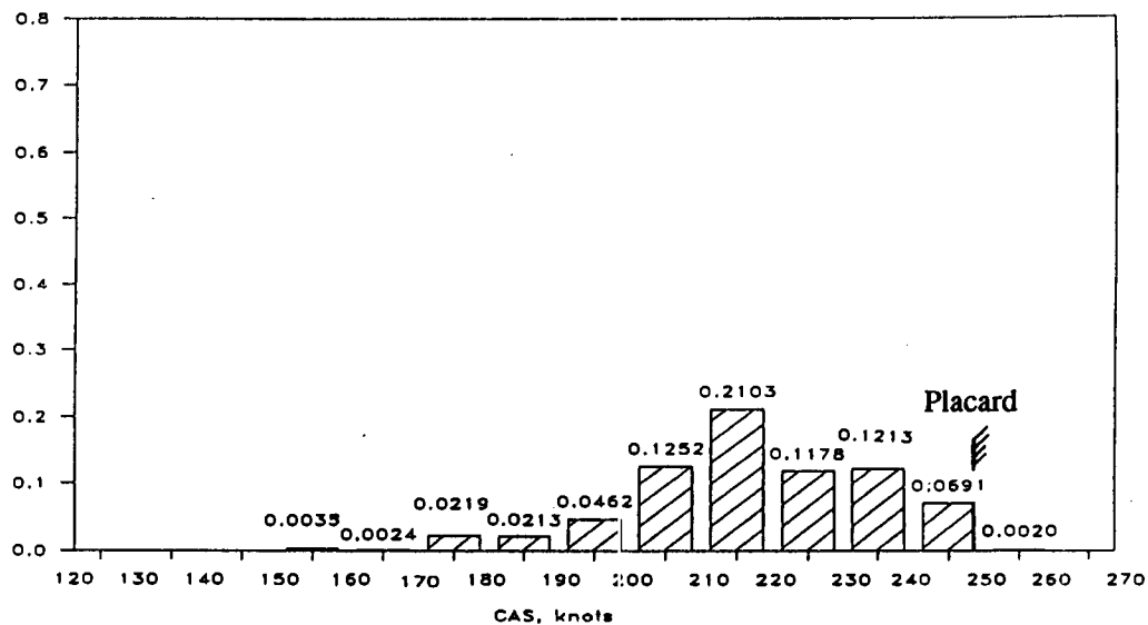
(c) Landing with flaps = 4 deg. (1.4914 hours)
