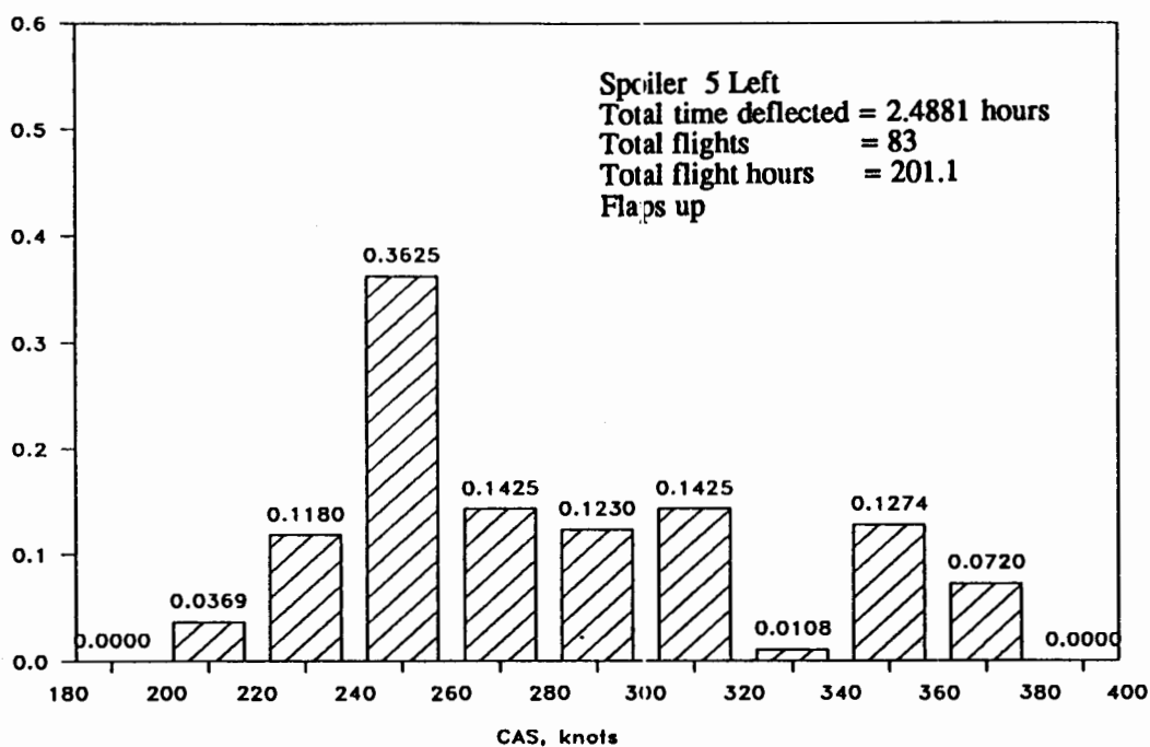
(c) Spoiler use vs. airspeed, histograms
