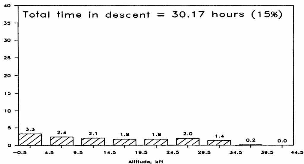
(c) Percent time vs. altitude for climb, level, and descent
