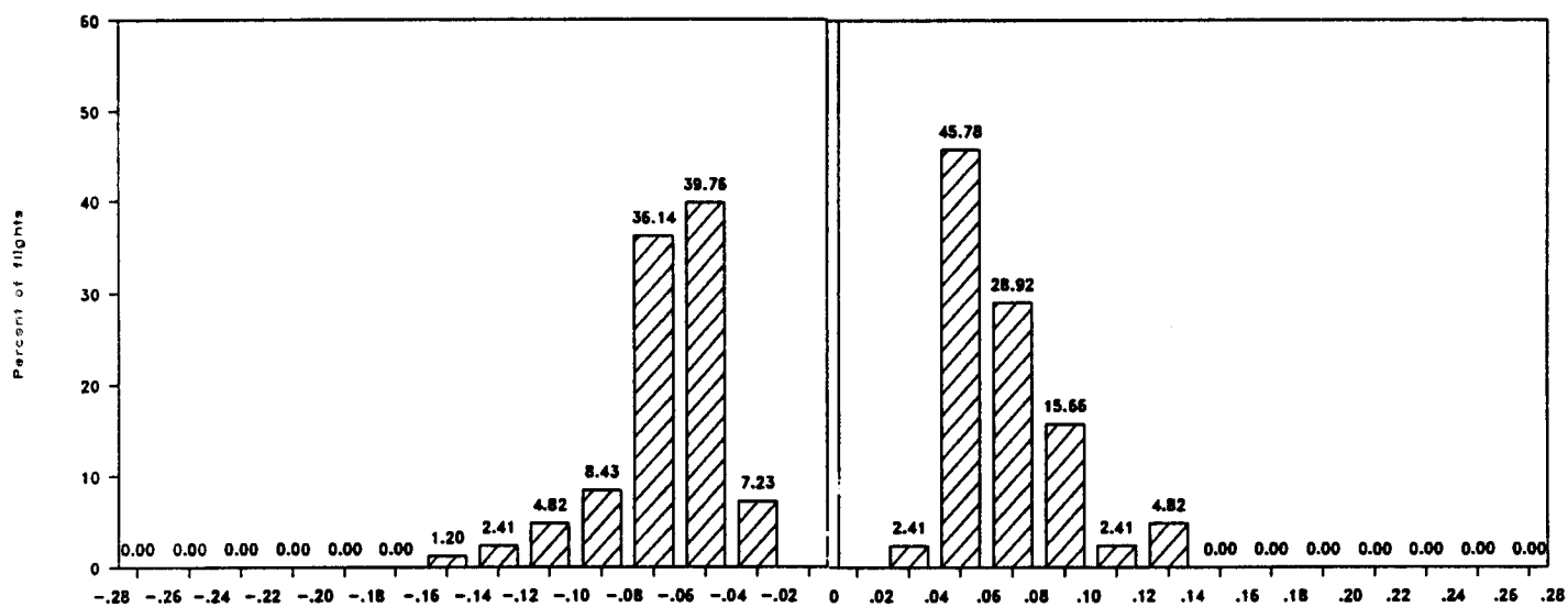
(c) a_y
