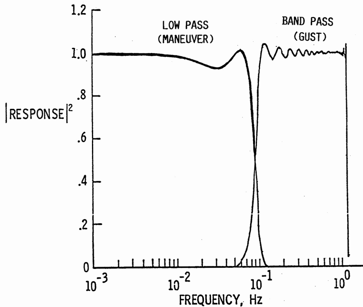
Figure 9.- Frequency response of numerical filters used to separate gust and maneuver accelerations, and to eliminate elastic responses above 1.2 Hz.
