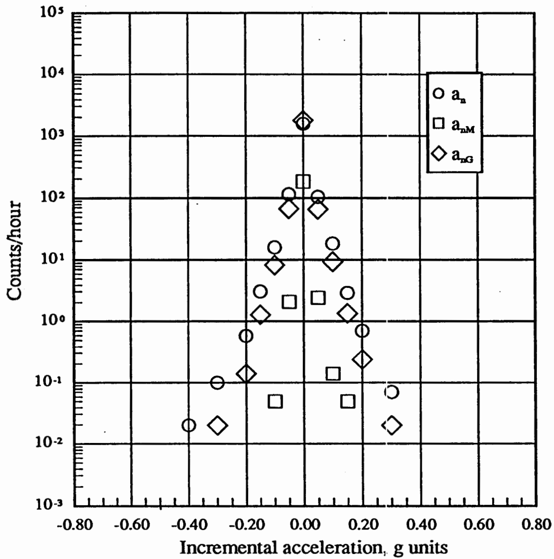
(k) a_n , a_{nM} , a_{nG} , 34500 to 39500 ft
