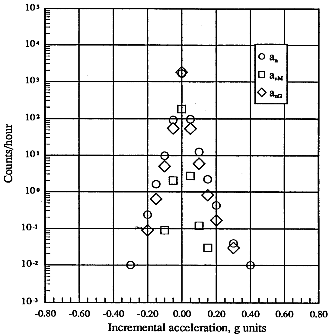
(j) a_n , a_{nM} , a_{nG} , 29500 to 34500 ft
