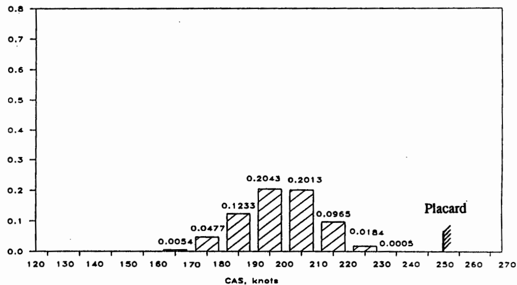
(b) Take-off with flaps = 4 deg. (1.4050 hours)
