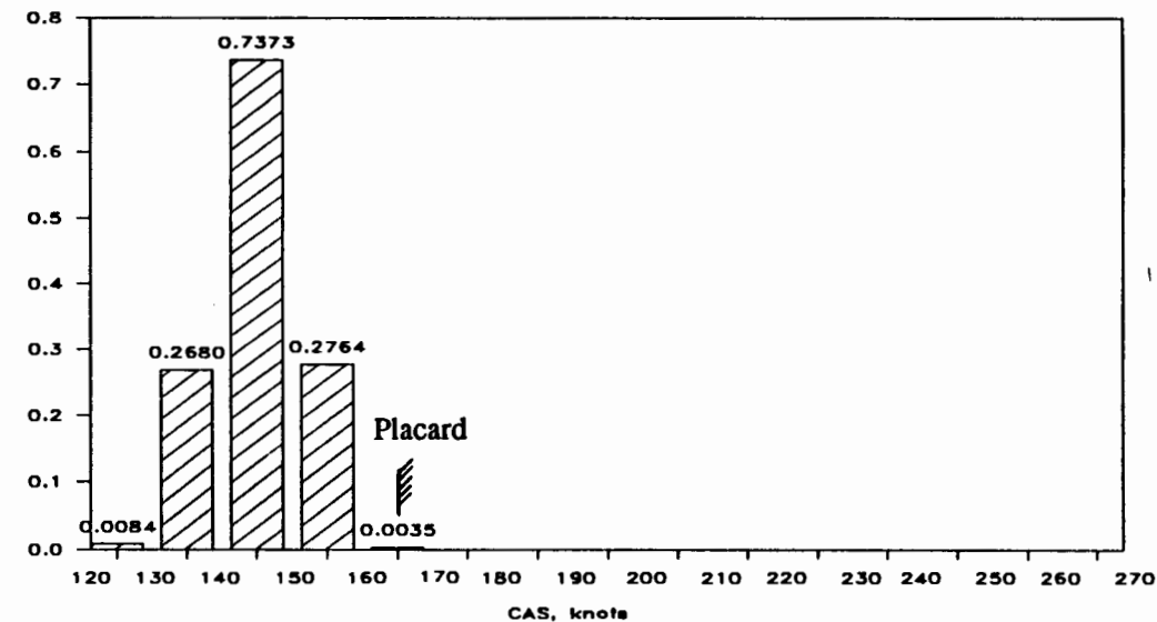
(f) Landing with flaps = 42 deg. (2.6018 hours)
