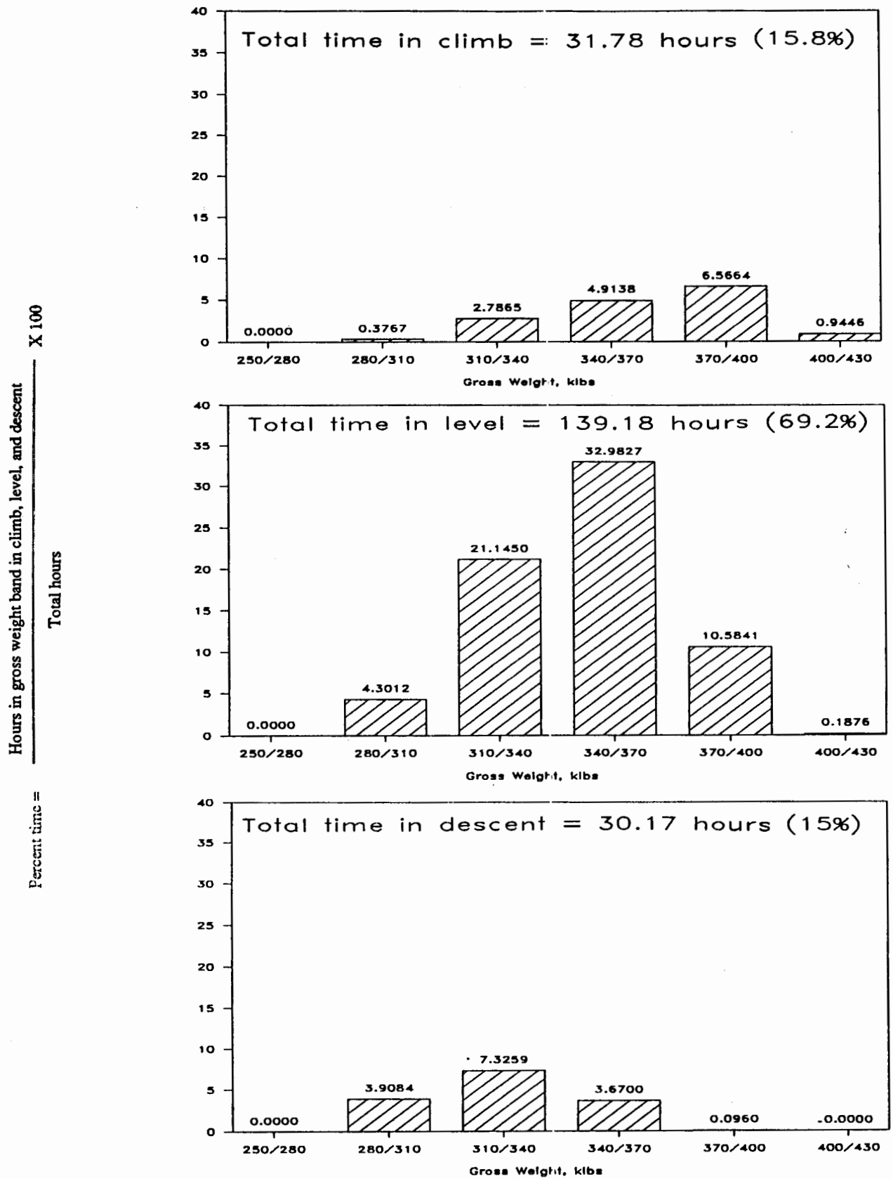
(b) Percent time vs. gross weight for climb, level, and descent
