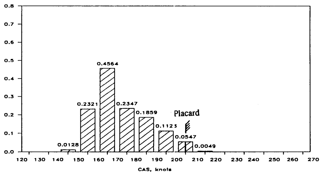
(e) Landing with flaps = 22 deg. (2.6022 hours)
