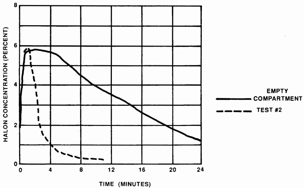
FIGURE 7. HALON CONCENTRATION
