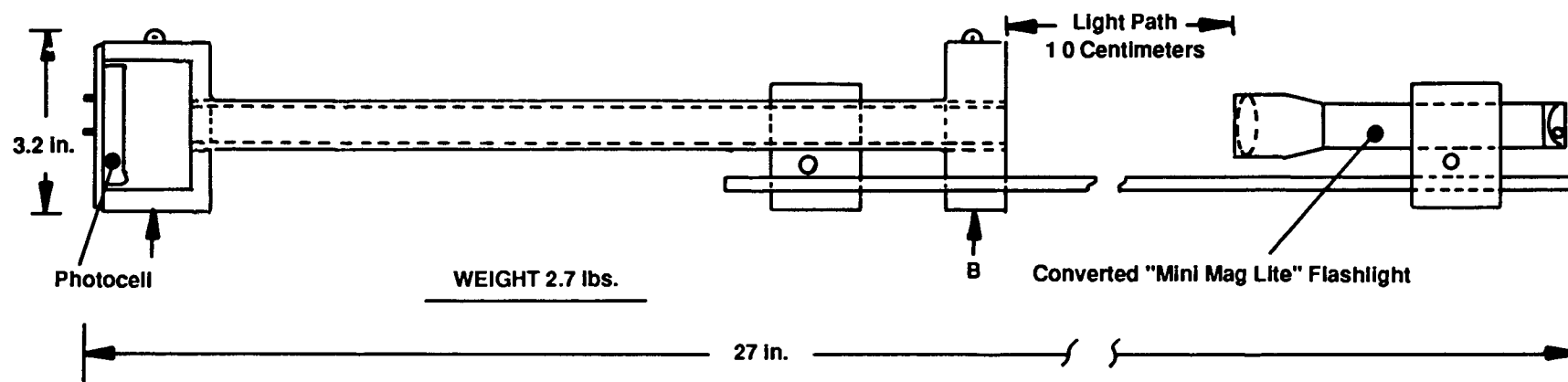
Federal Aviation Administration Aerosol Meter (FAAAM)
