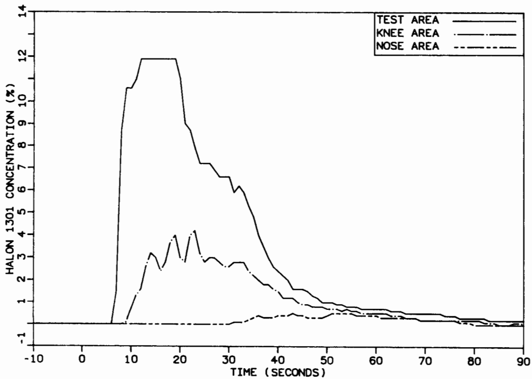
FIGURE 14. HALON 1301 CONCENTRATIONS CIRCUIT BREAKER PANEL PILOT'S SIDE
