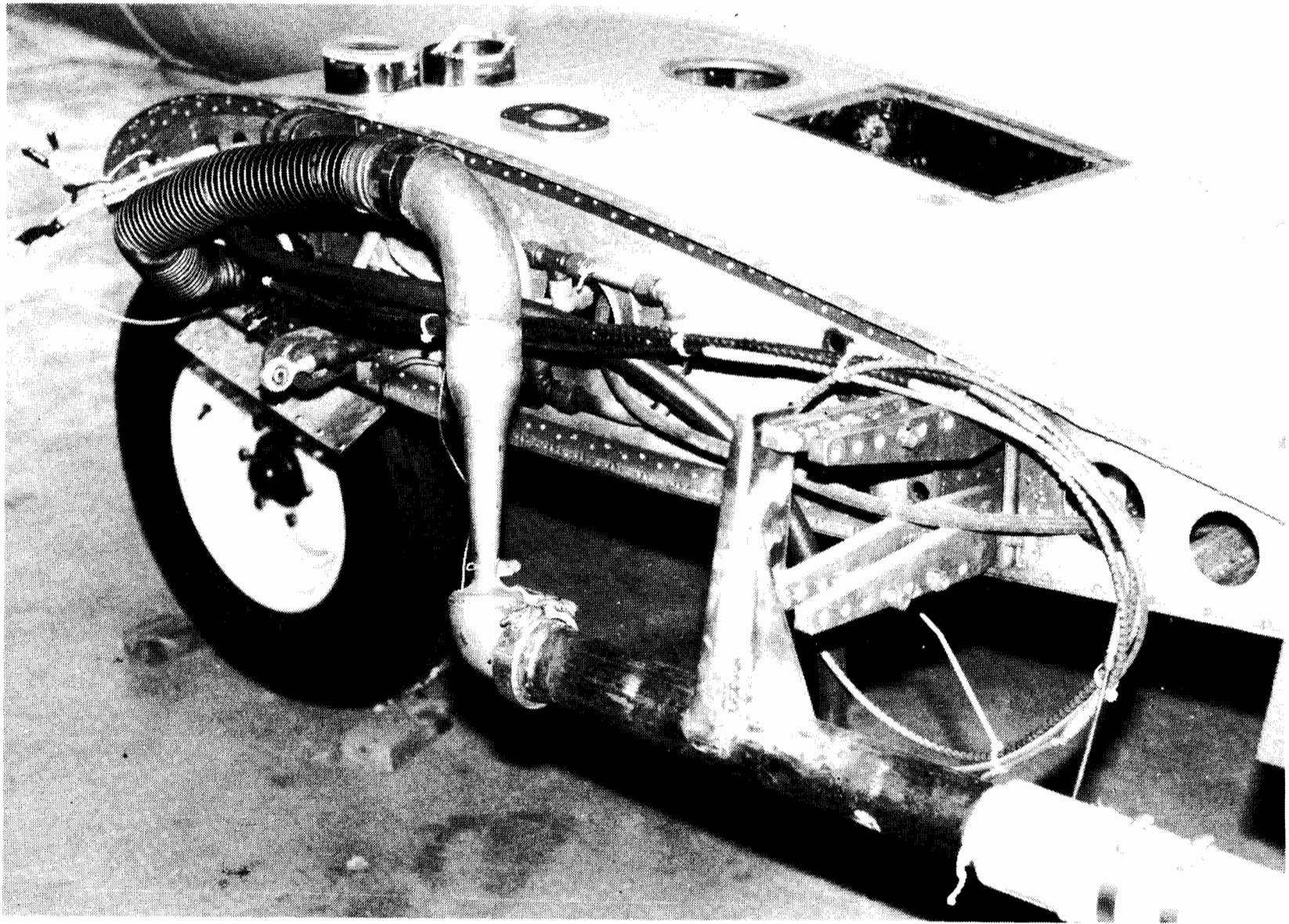
FIGURE 3. SONIC VENTURI
