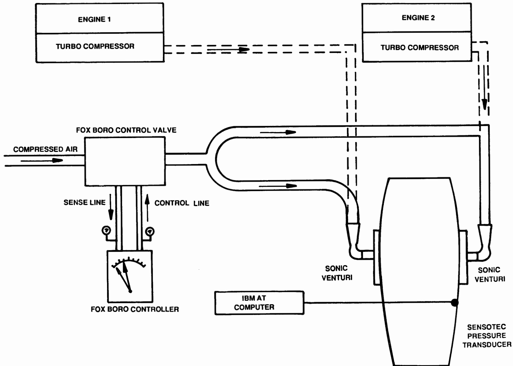
FIGURE 1. AIR PRESSURIZATION SYSTEM
