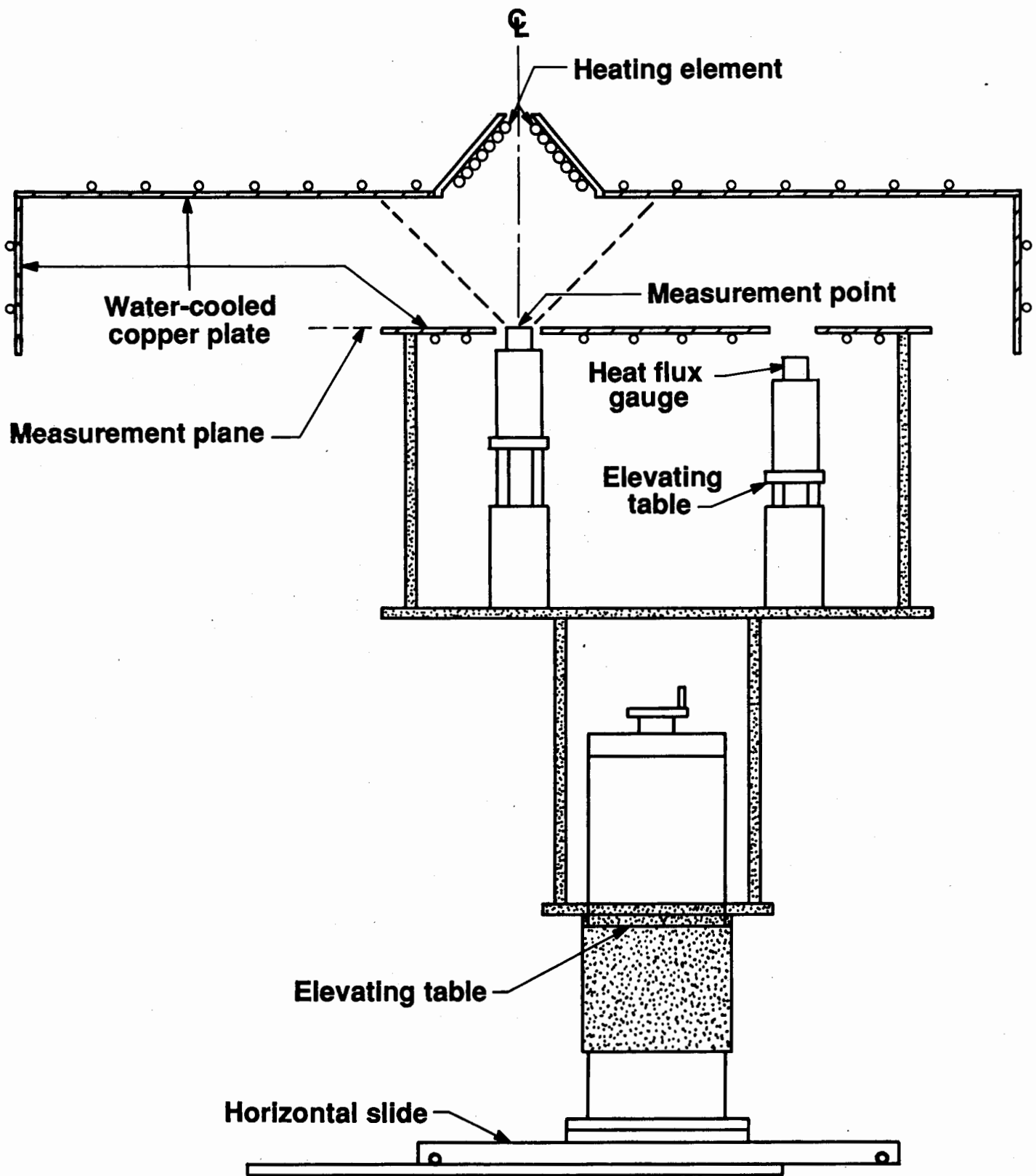
FIGURE 6. CFR CALIBRATION APPARATUS FOR HEAT FLUX SENSORS
