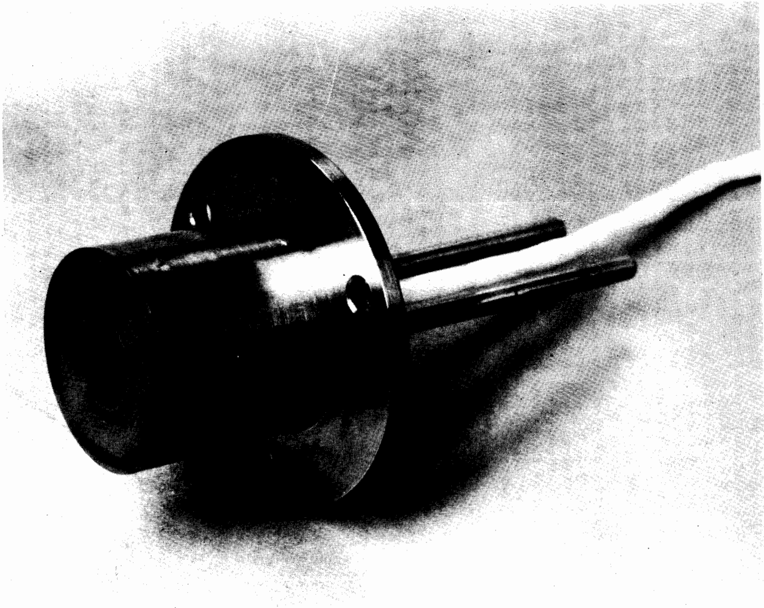
FIGURE 1. GARDON HEAT FLUX GAUGE
