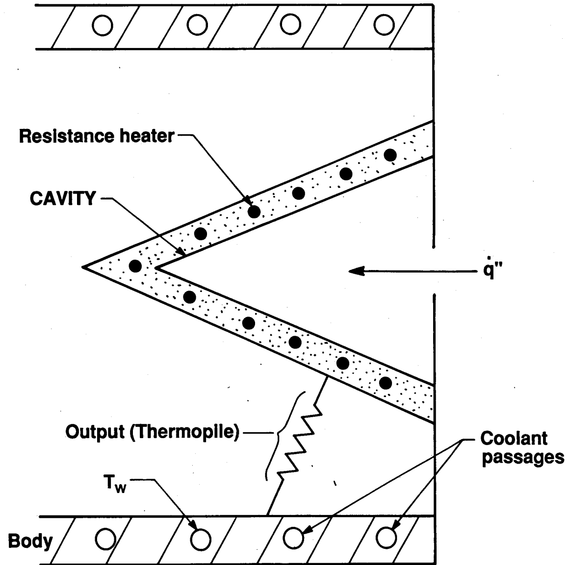
FIGURE 4. OPERATING PRINCIPLE OF ECR
