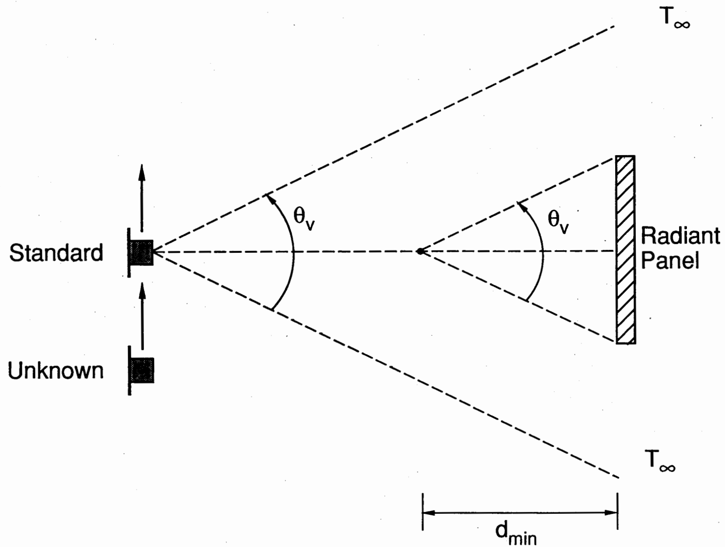
FIGURE 2. SUBSTITUTION TECHNIQUE
