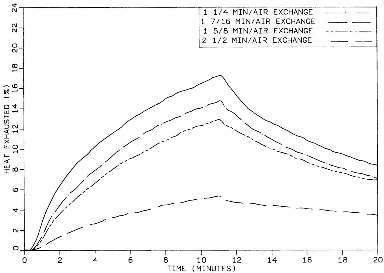
FIGURE 10. PERCENT HEAT EXHAUSTED AT 1 1/4, 1 7/16, 1 5/8, 2 1/2 MIN/AIR EXCHANGE
