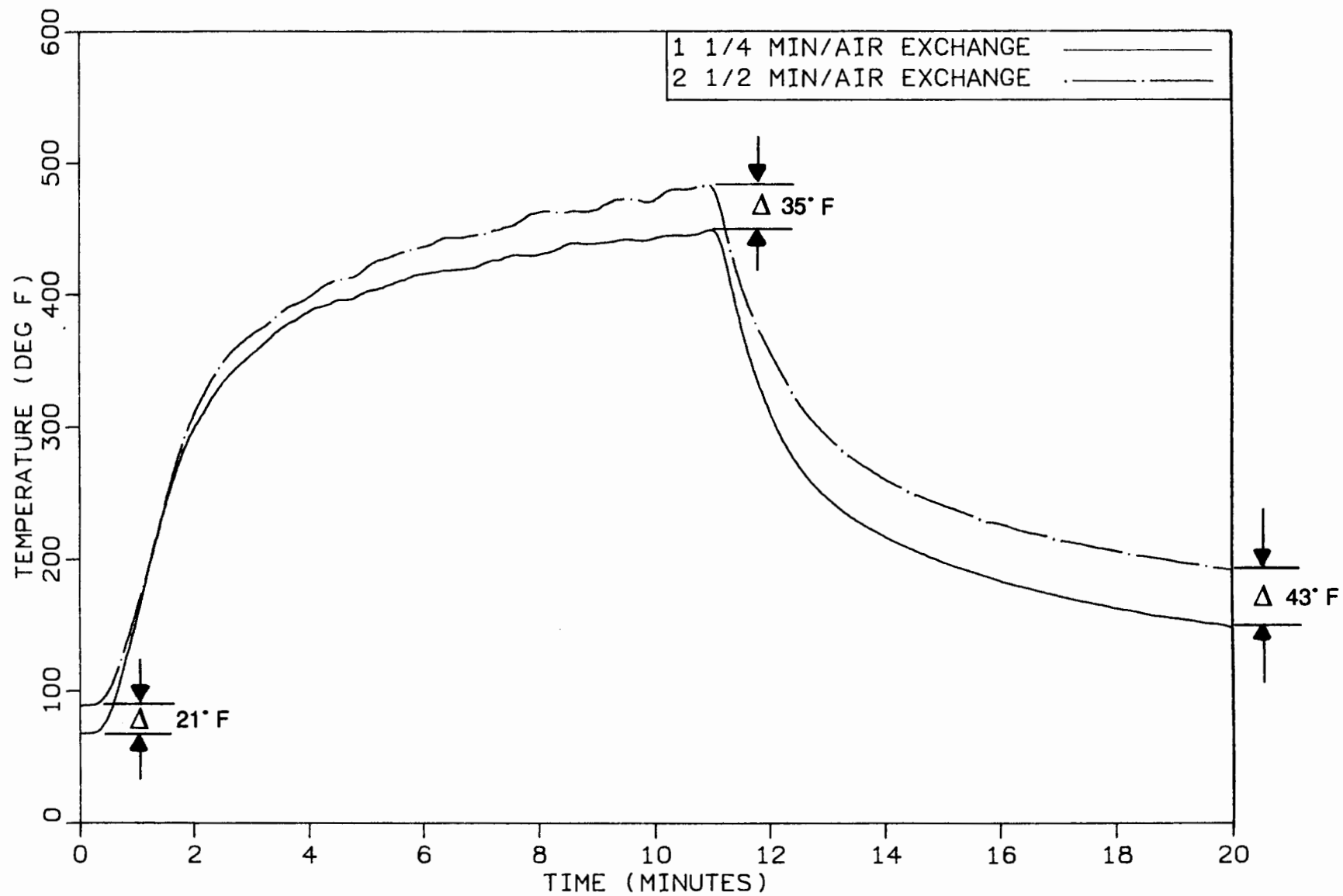
FIGURE 13. TEMPERATURE PROFILES AT 1 1/4 & 2 1/2 MIN/AIR EXCHANGE (DIFFERENT AMBIENT TEMPERATURES)
