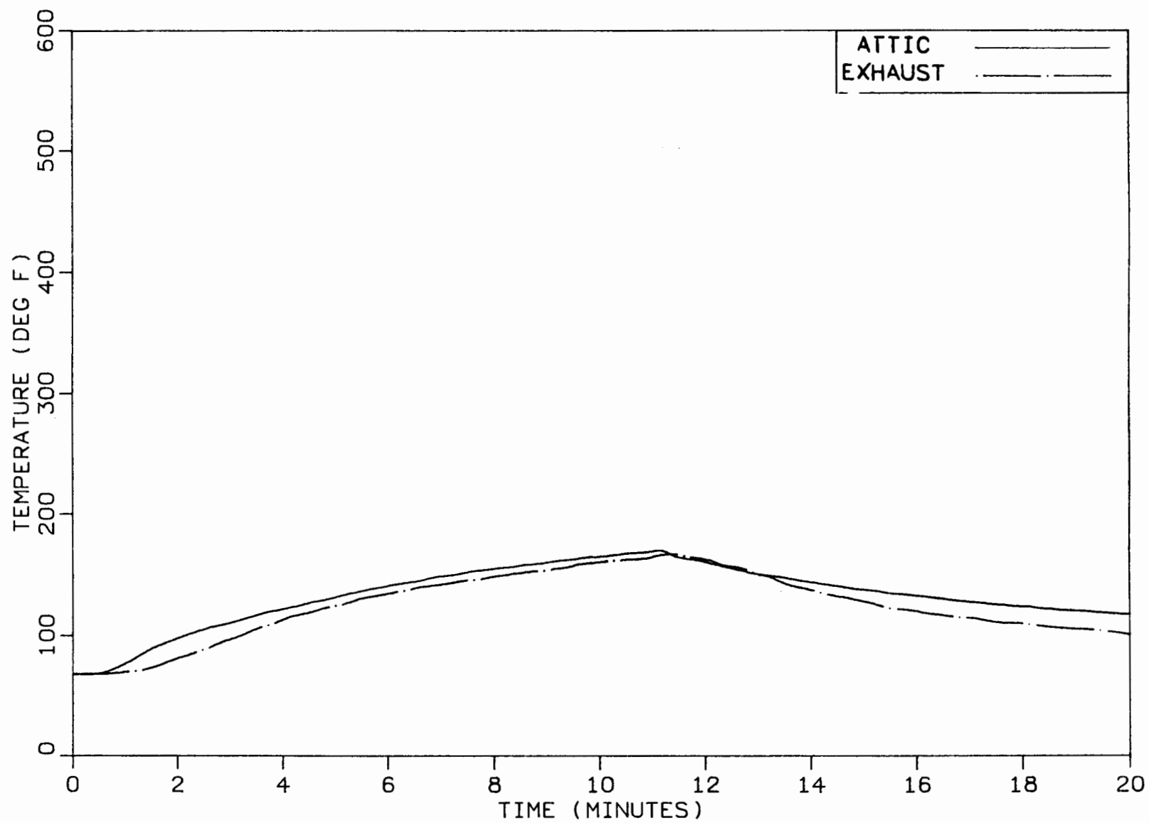
FIGURE 7. TYPICAL ATTIC/EXHAUST TEMPERATURE PROFILES
