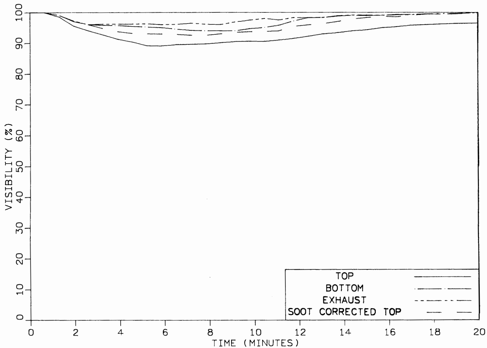
FIGURE 19. TYPICAL SMOKE PROFILE FOR 2 1/2 MIN/AIR EXCHANGE INCLUDING SOOT CORRECTRION
