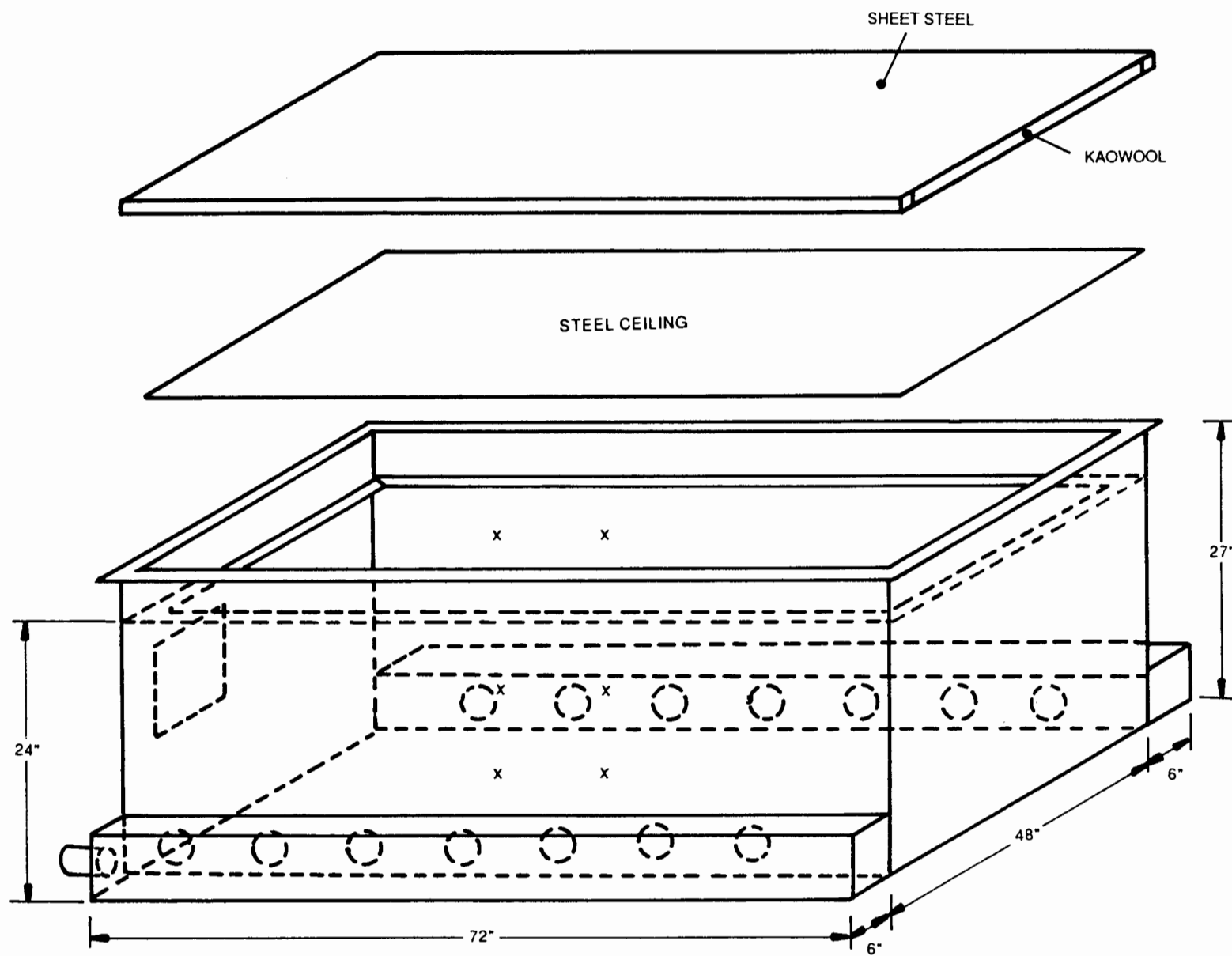
FIGURE 2. 3-DIMENSIONAL MODEL VIEW
