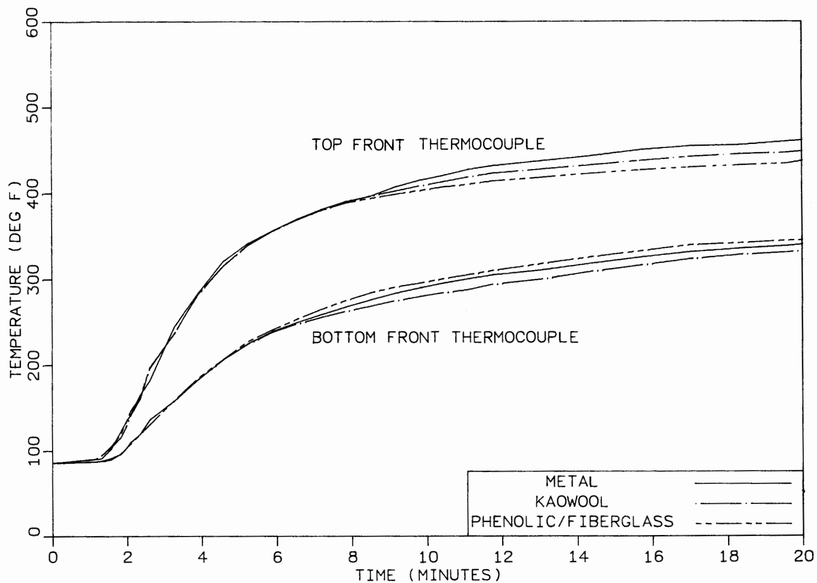
FIGURE 5. MIXED CEILINGS - TOP FRONT TEMPERATURE PROFILES AT 2 1/2 MIN/AIR EXCHANGE
