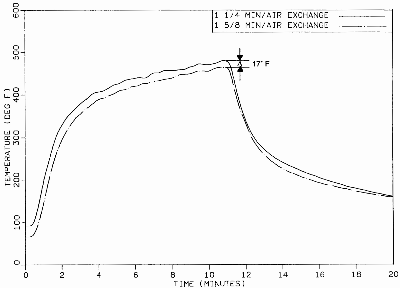
FIGURE 12. TEMPERATURE PROFILES AT 1 1/4 & 1 5/8 MIN/AIR EXCHANGE (DIFFERENT AMBIENT TEMPERATURES)
