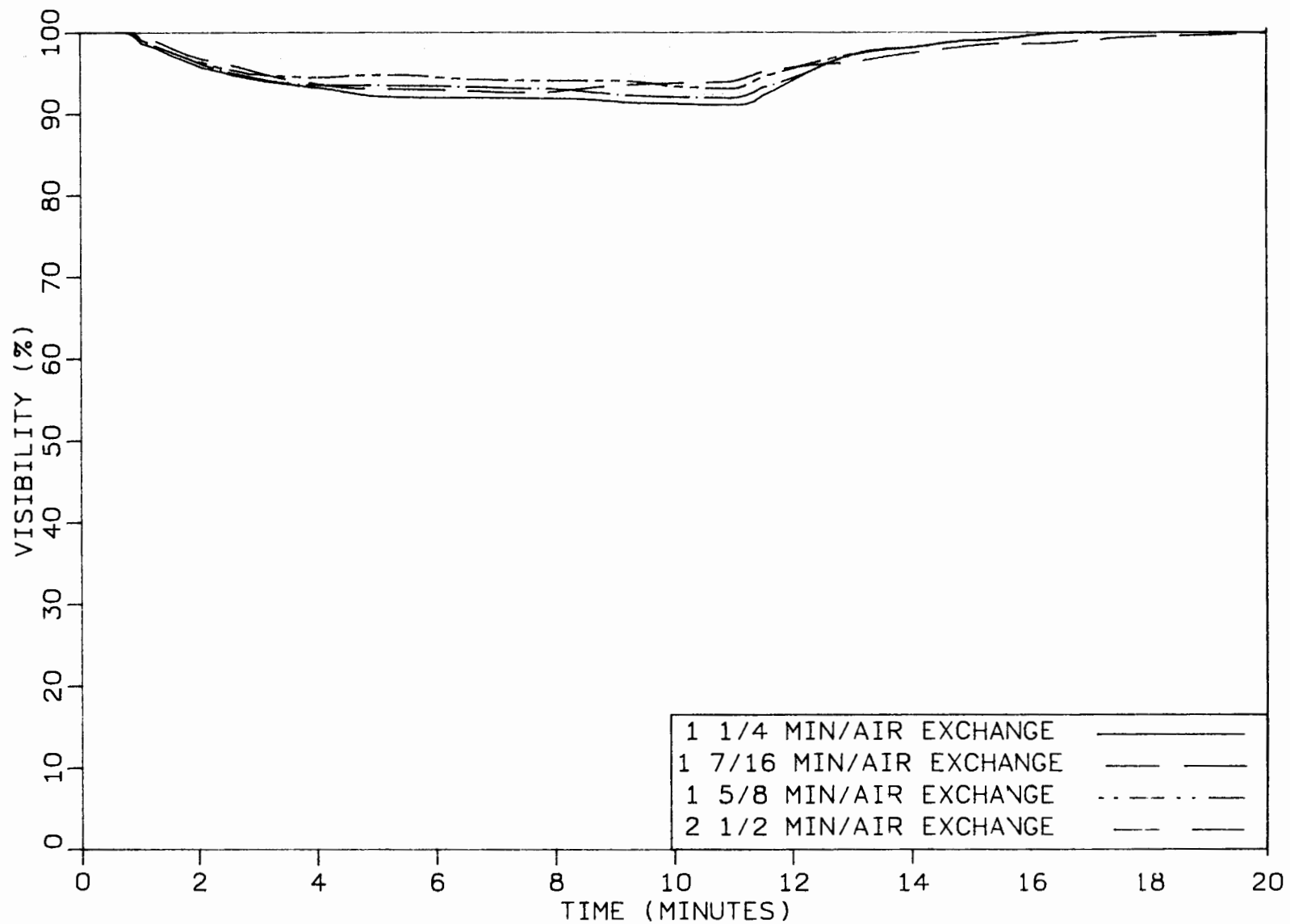
FIGURE 20. TYPICAL SMOKE PROFILES FOR TOP SMOKE METER FOR 1 1/4, 1 7/16, 1 5/8, 2 1/2 MIN/AIR EXCHANGE
