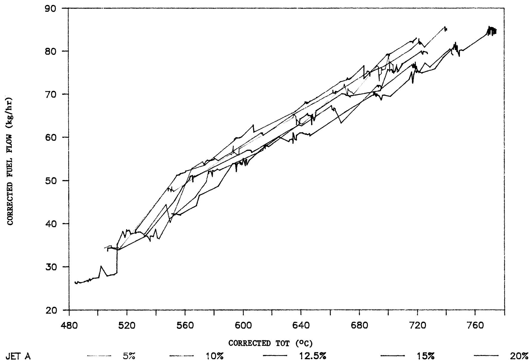
FIGURE 5. CORRECTED FUEL FLOW VERSUS CORRECTED TURBINE OUTLET TEMPERATURE FOR JET-A/ETHANOL BLENDS
