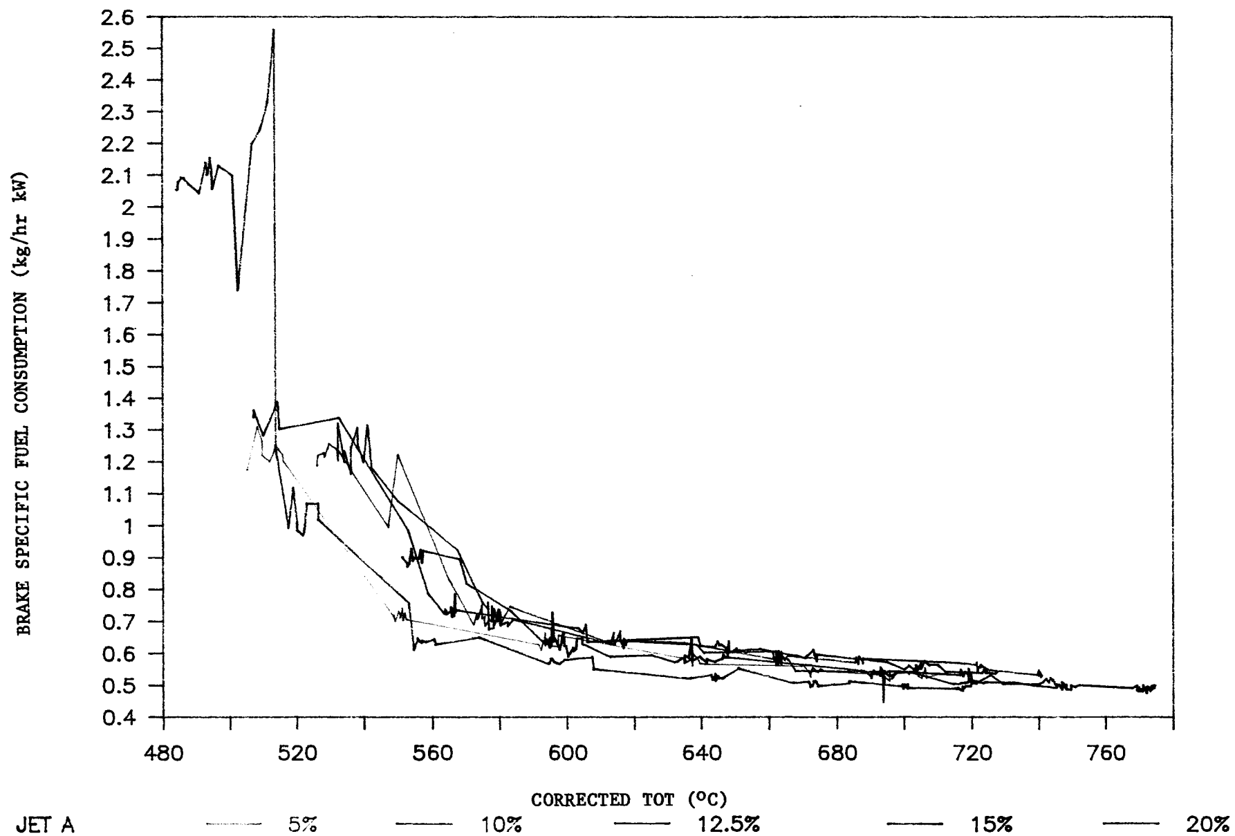
FIGURE 7. BRAKE SPECIFIC FUEL CONSUMPTION VERSUS CORRECTED TURBINE OUTLET TEMPERATURE
