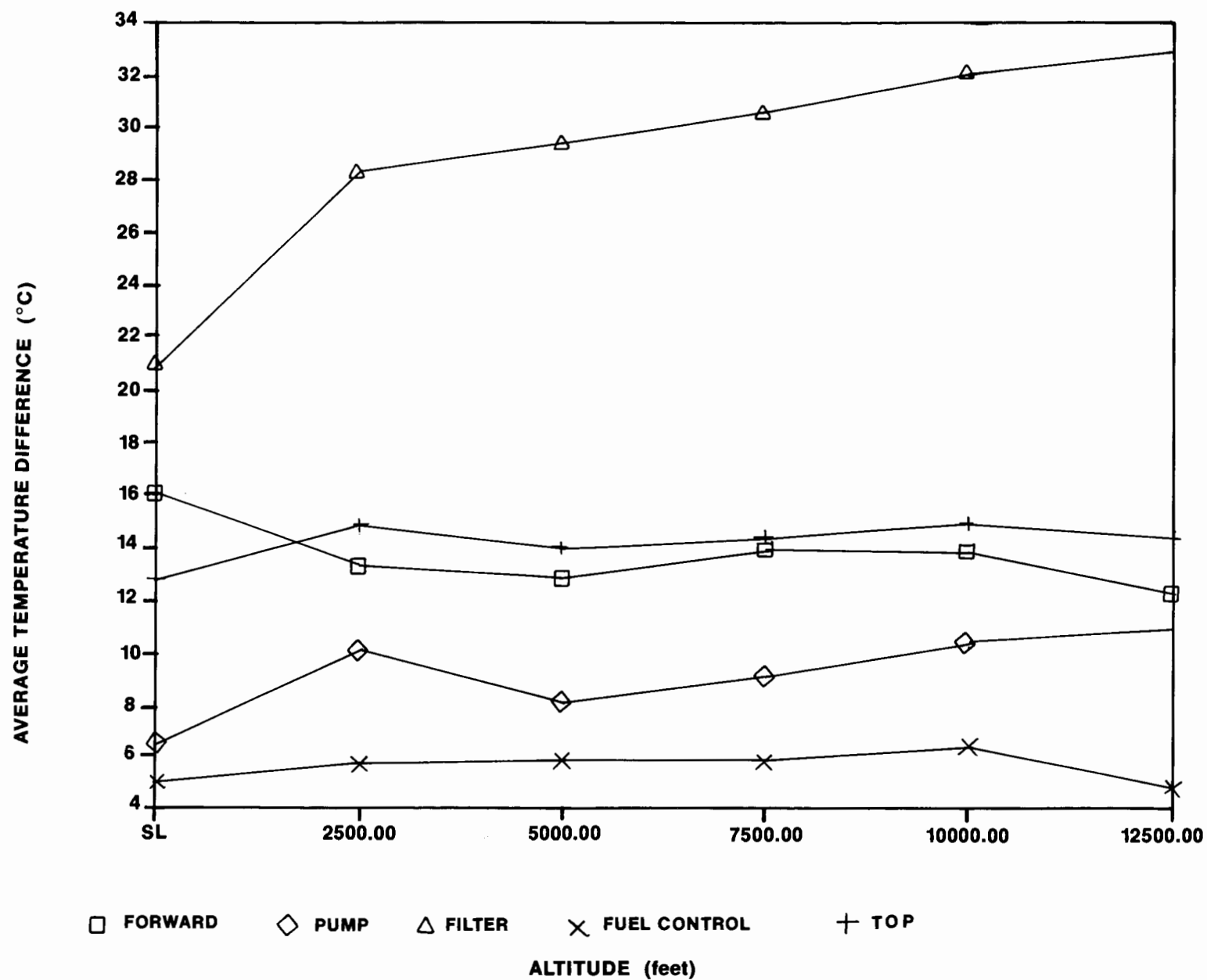
FIGURE 13. TEMPERATURE DIFFERENCE AS A FUNCTION OF ALTITUDE
