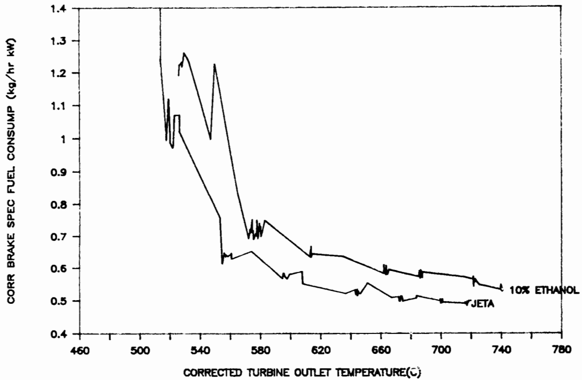
FIGURE A-7. CORRECTED BRAKE SPECIFIC FUEL CONSUMPTION VERSUS CORRECTED TURBINE OUTLET TEMPERATURE
