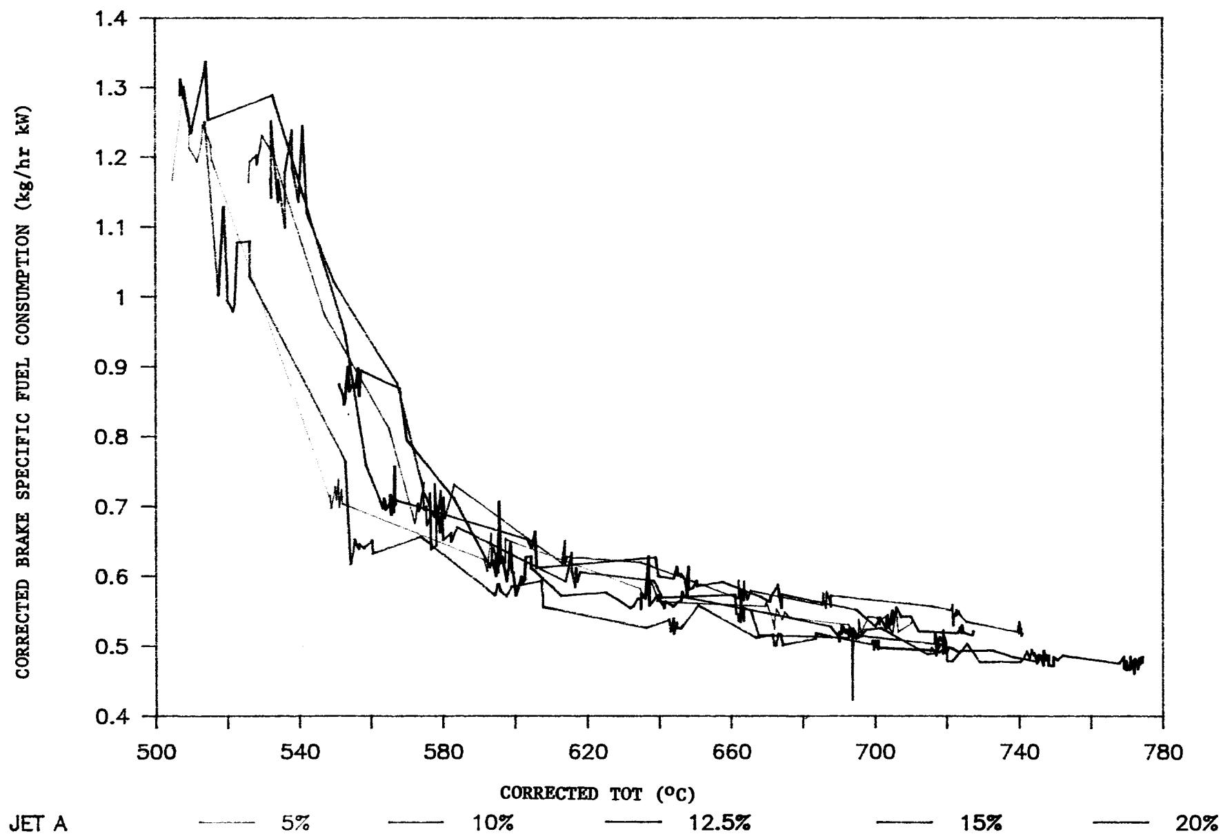
FIGURE 6. CORRECTED BRAKE SPECIFIC FUEL CONSUMPTION VERSUS CORRECTED TURBINE OUTLET TEMPERATURE
