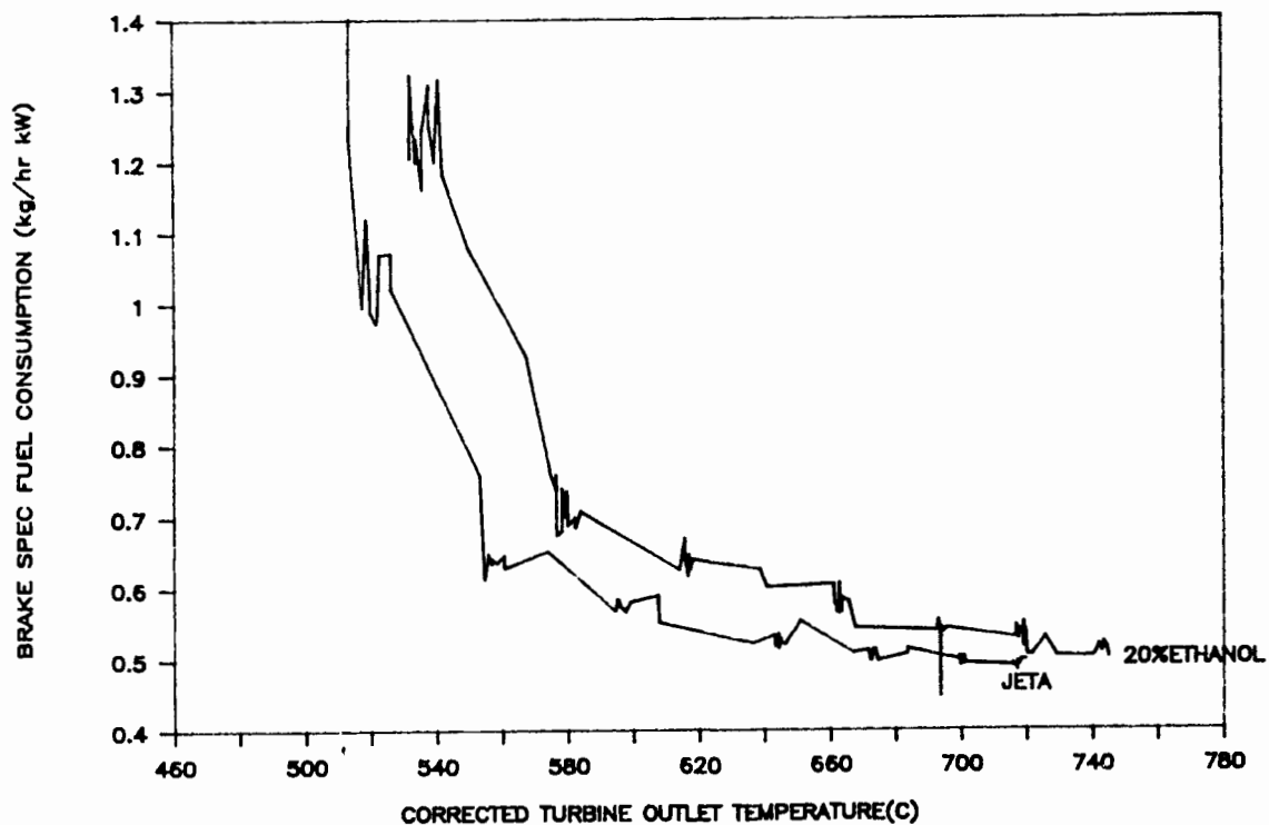
FIGURE A-20. BRAKE SPECIFIC FUEL CONSUMPTION VERSUS CORRECTED TURBINE OUTLET TEMPERATURE
