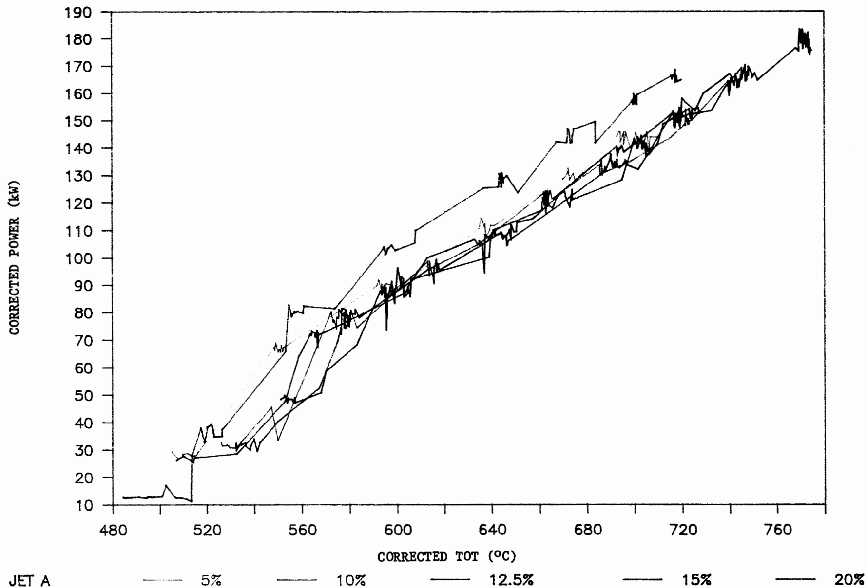
FIGURE 4. CORRECTED POWER DEVELOPED VERSUS CORRECTED TURBINE OUTLET TEMPERATURE FOR JET-A/ETHANOL BLENDS
