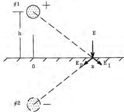
Fig. 9.25 Conductor over a ground plane.
