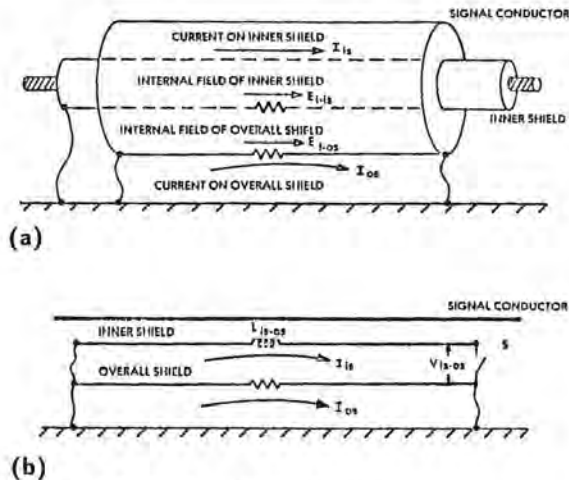
Fig. 15.9 Double shielded cable.
