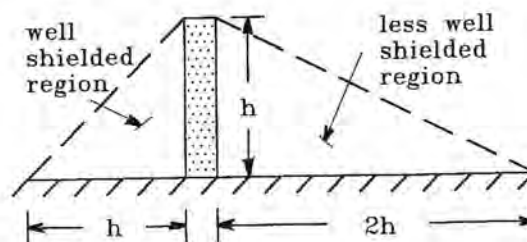
Fig. 2.43 Shielded areas.
