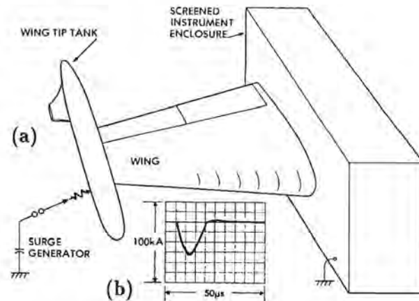
Fig. 8.11 High current injection tests on a wing from a fighter aircraft. (a) Test arrangement (b) Waveshape of injected current
