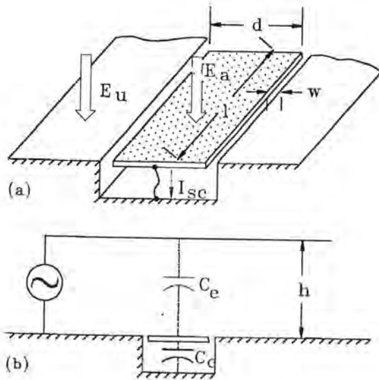
Fig. 14.10 Displacement currents. (a) Geometry (b) Equivalent circuit
