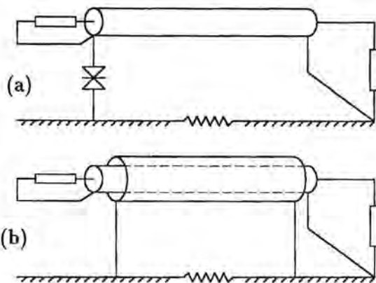
Fig. 17.3 Elimination of common mode voltage.
