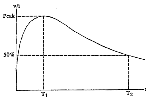
Current Waveform 1 T_1 = 6.4 \text{ us} \pm 20\% T_2 = 70 \text{ us} \pm 20\%
