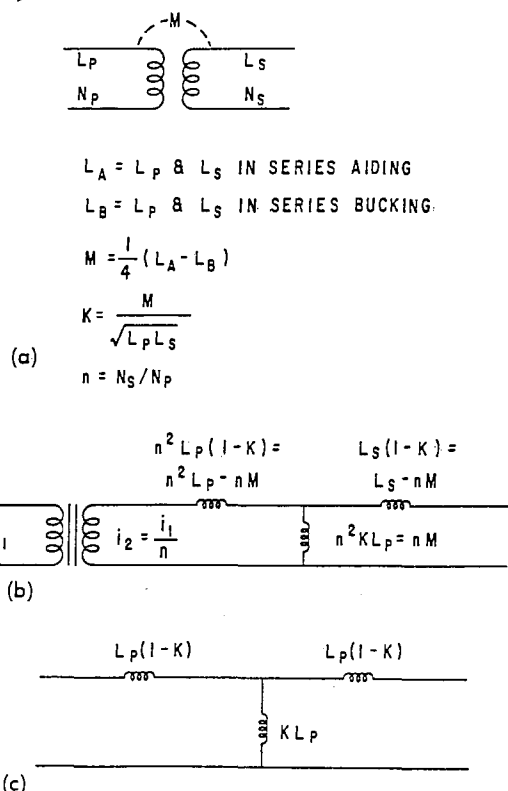
Fig. 18.25 Development of equivalent circuits.
