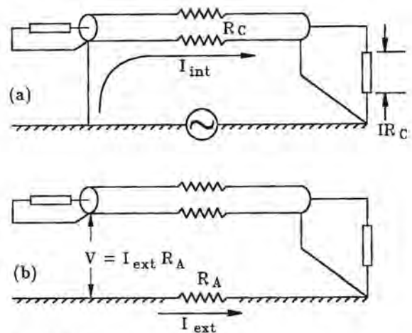
Fig. 17.2 Single ended transmission.
