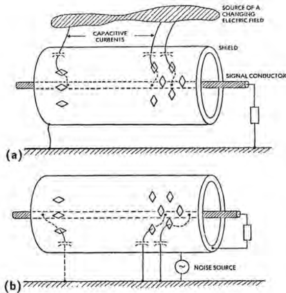
Fig. 15.20 Coupling via capacitive leakage through holes.
