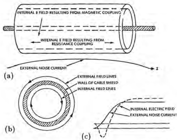
Fig. 15.19 Magnetic coupling giving effect of a negative coupling inductance.
