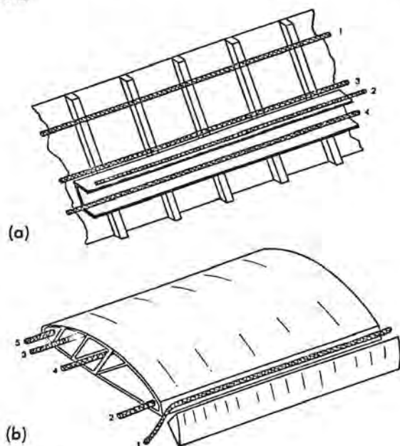
Fig. 16.2 Conductor routing.
