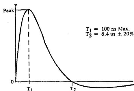
Voltage Waveform 2
