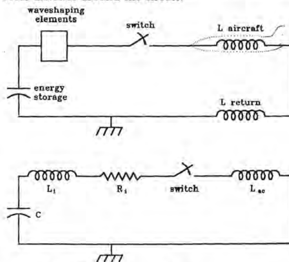
Fig. 13.1 Basic test circuit.
