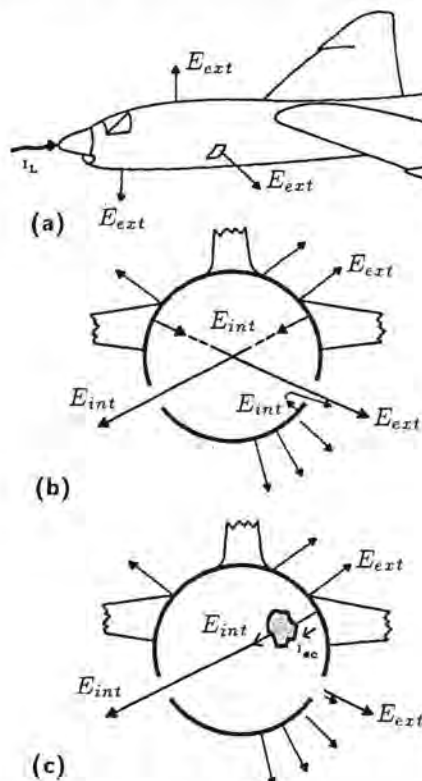
Fig. 8.10 Aperture-type electric field coupling. (a) External field patterns (b) Internal field patterns (c) Induced current
