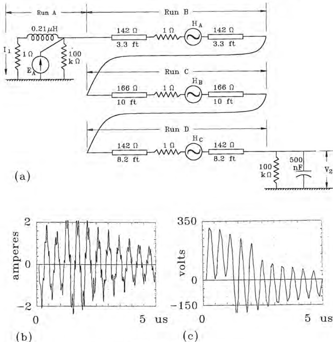
Fig. 14.32 Circuit modeled as transmission lines.
