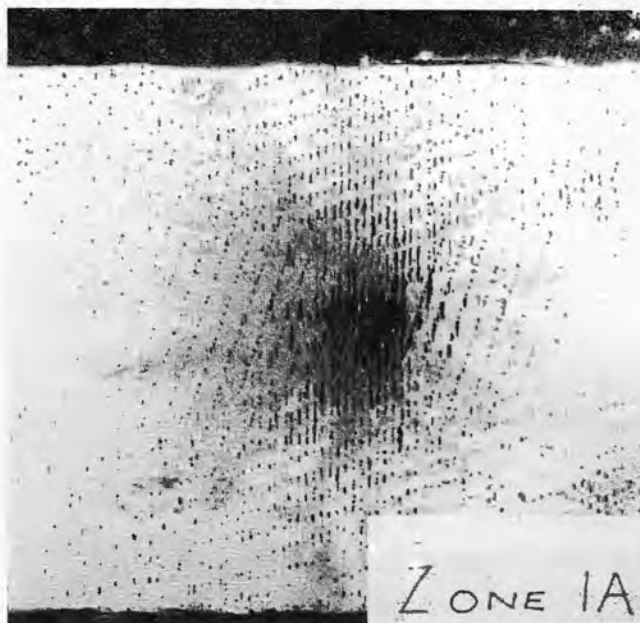
Fig. 6.47 Damage to protected graphite composite panel 1mm (0.040 in) thick. Zone 1A flash, 190 kA, 1.24 \times 10^6 \text{ A}^2\text{-s} .
