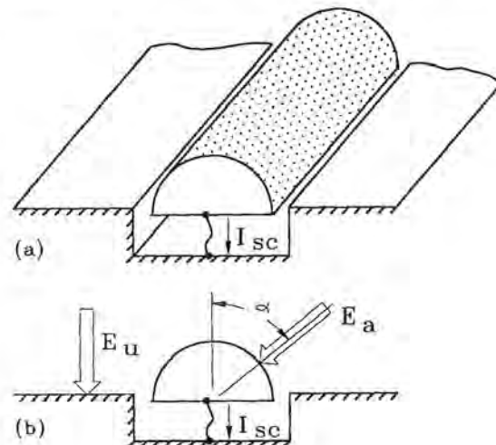
Fig. 14.12 Hemicylinder. (a) Geometry (b) End view
