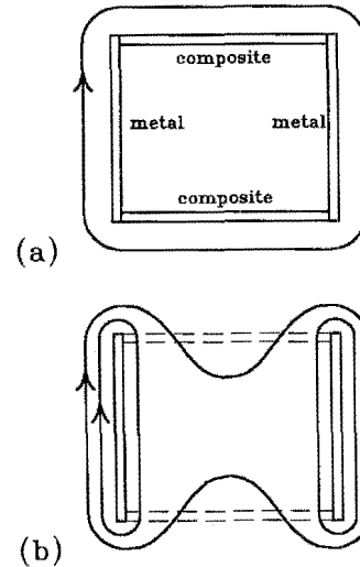
Fig. 11.33 Magnetic field patterns.
