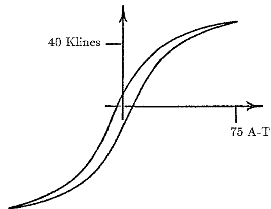
Fig. 18.22 B-H loop of a gapped ferrite core.
