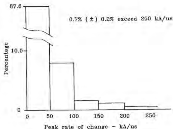
Fig. 3.29 I -dot measurements on the F-106B.
