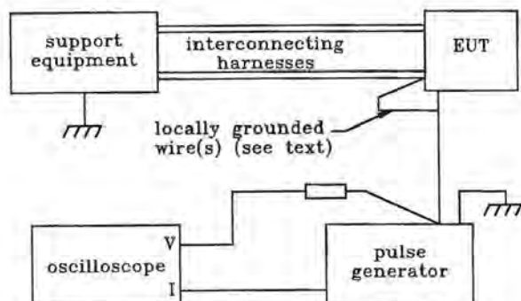
Fig. 18.41 Test setup for ground injection.
