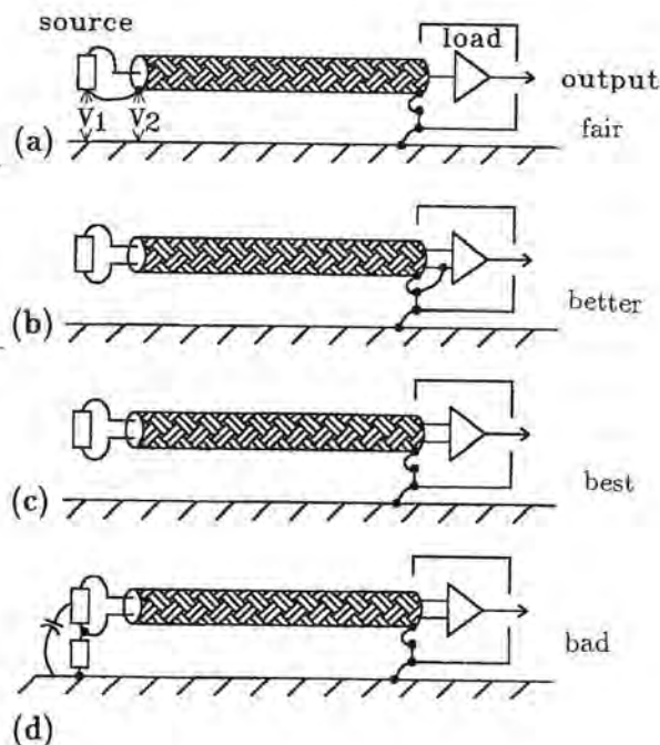
Fig. 15.1 Single point ground on shield.
