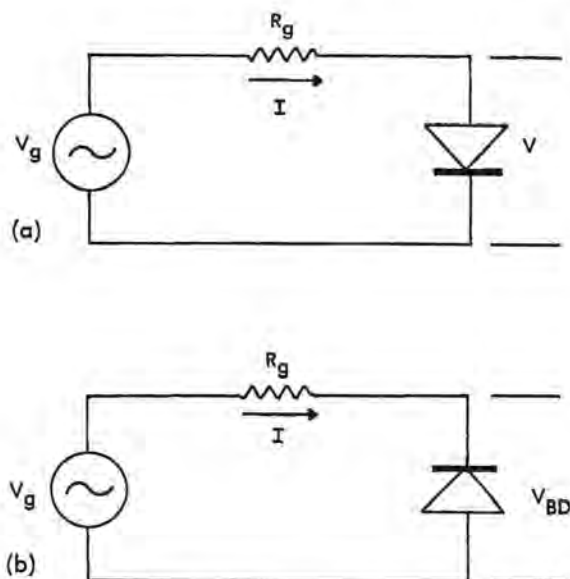
Fig. 17.25 Voltage and current through a diode junction [17.9].
