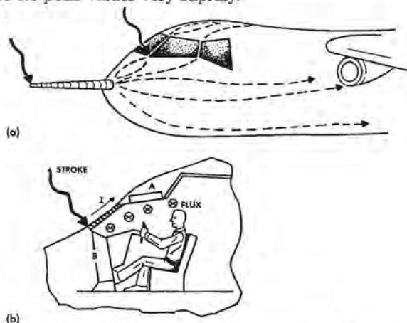
Fig. 16.3 Current flow along windshield posts.
