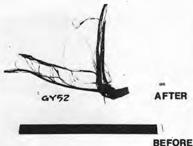
Fig. 4.12 Typical lightning stroke current damage to CFC skin material.
