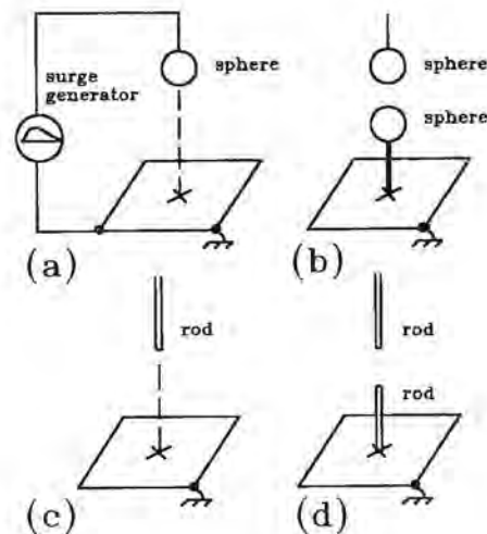
Fig. 1.14 Electrode configurations.
