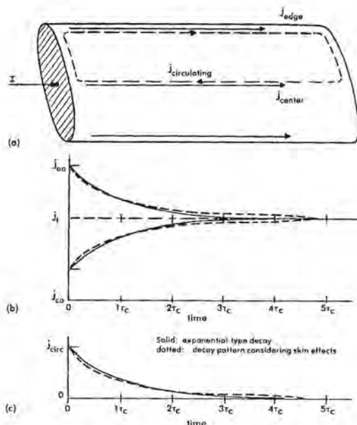
Fig. 11.18 Variation of current density with time. (a) Current components defined (b) Edge and center currents (c) Circulating currents
