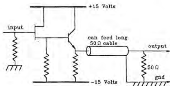
Fig. 13.17 Active probe.
