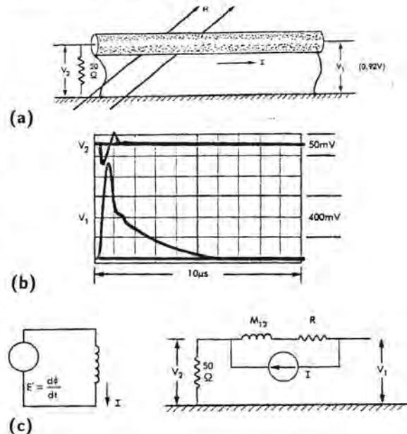
Fig. 15.8 Shield grounded at both ends
