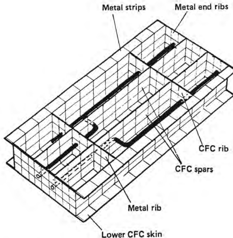
Fig. 11.35 Wing box analyzed with 3DFD technique.
