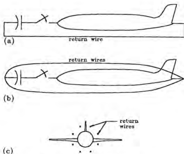
Fig. 13.2 Return circuits.
