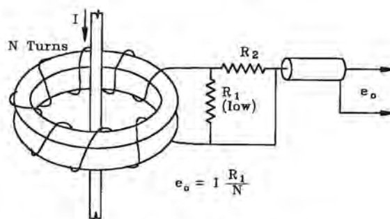
Fig. 18.31 Current transformer.
