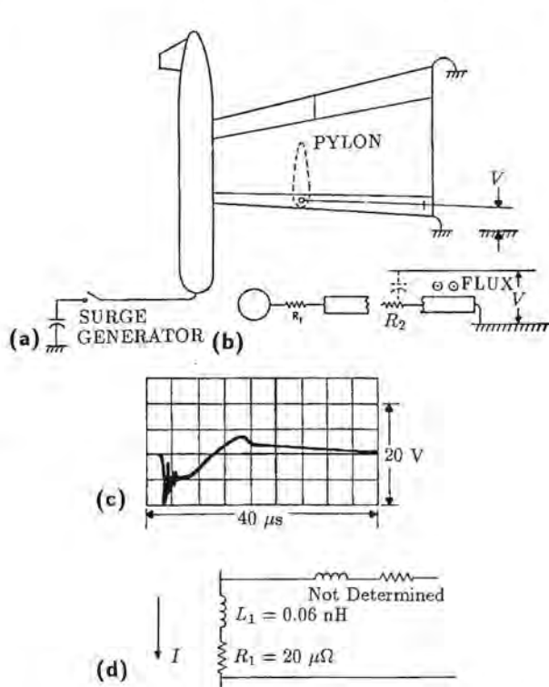
Fig. 8.13 A pylon circuit - open at pylon.
