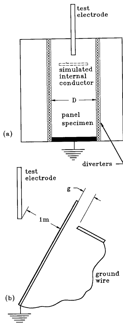
Fig. 6.33 Test of flat panel to determine diverter spacing.
