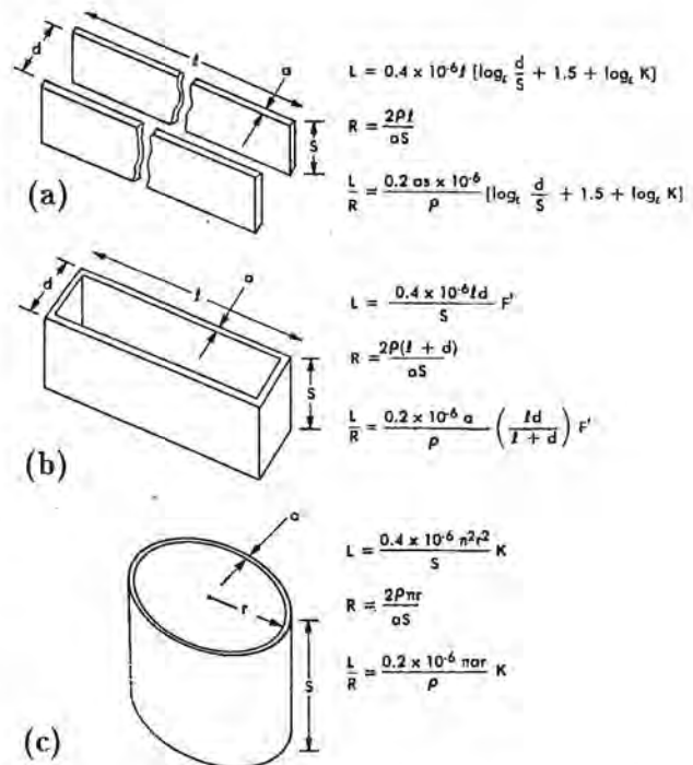
Fig. 11.41 Typical current paths and characteristic impedances.
