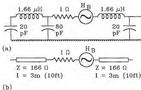
Fig. 14.30 Equivalent impedance for run C in zone B.
