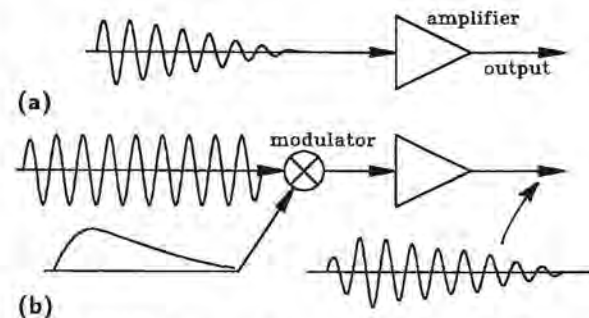
Fig. 18.13 Transient generation with amplifiers.
