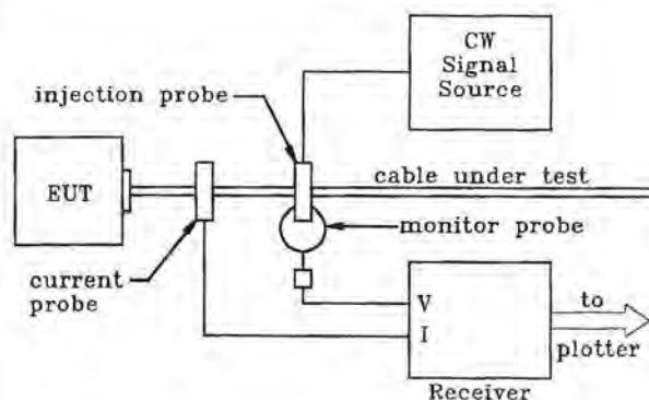
Fig. 18.39 Measurement of cable impedance.
