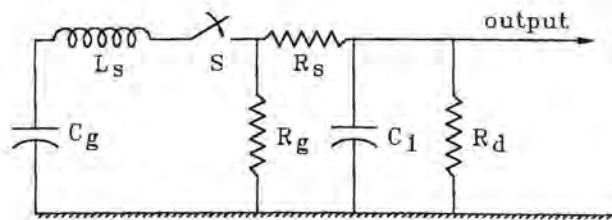
Fig. 6.57 Generator circuit including waveshaping elements.
