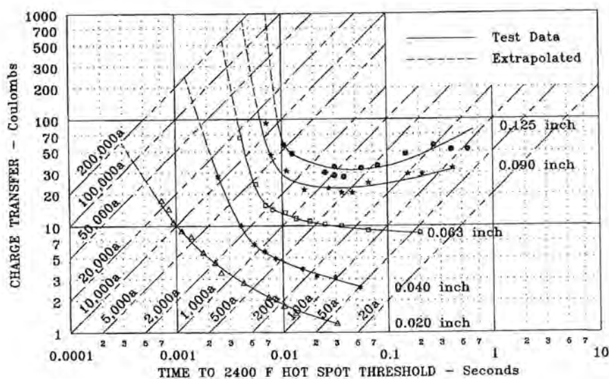
Fig. 6.3 Melt-through thresholds of metal skins.
