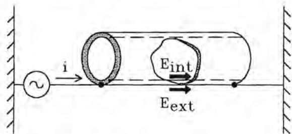
Fig. 9.8 Transfer impedance.
