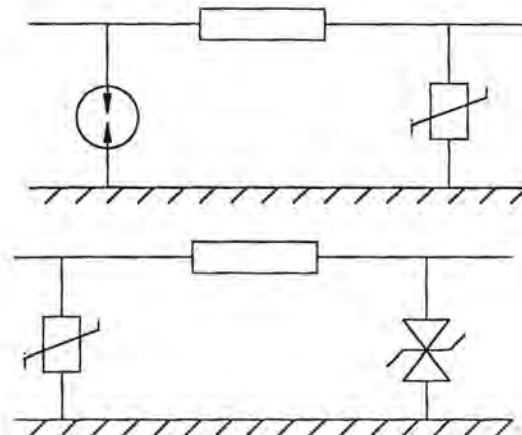
Fig. 17.24 Hybrid protectors. (a) Sparkgap and MOV (b) MOV and diode
