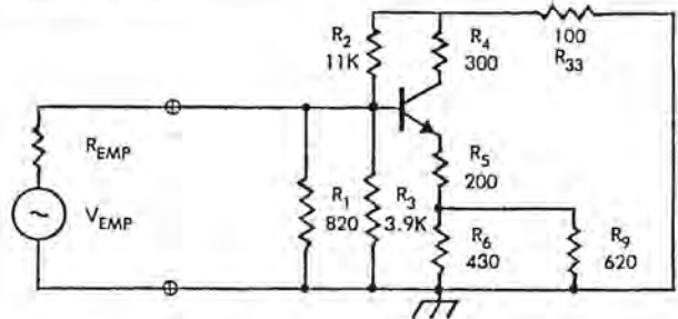
Fig. 17.40 Simplified phase-splitter circuit [17.29].
