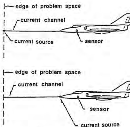
Fig. 10.26 Locations of current source used in computer code. (a) Natural lightning (b) Triggered lightning
