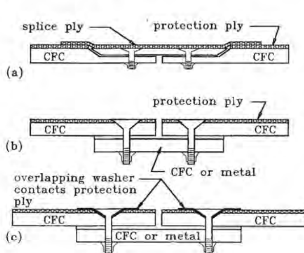
Fig. 6.50 Splices across manufacturing joint.
