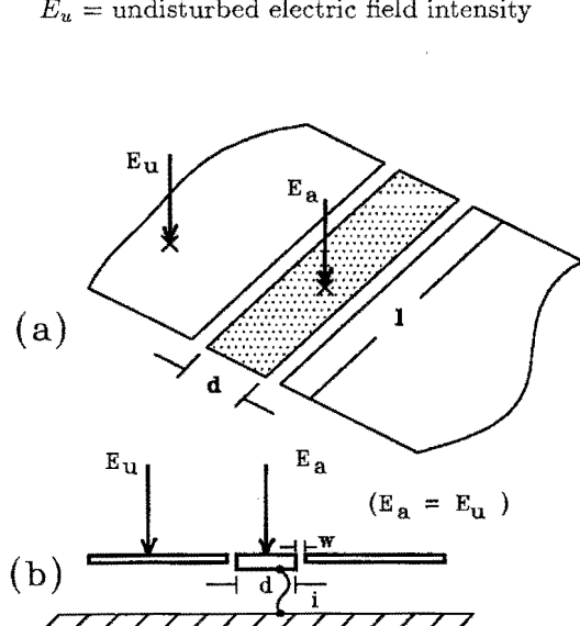
Fig. 9.26 A surface exposed to an electric field.
