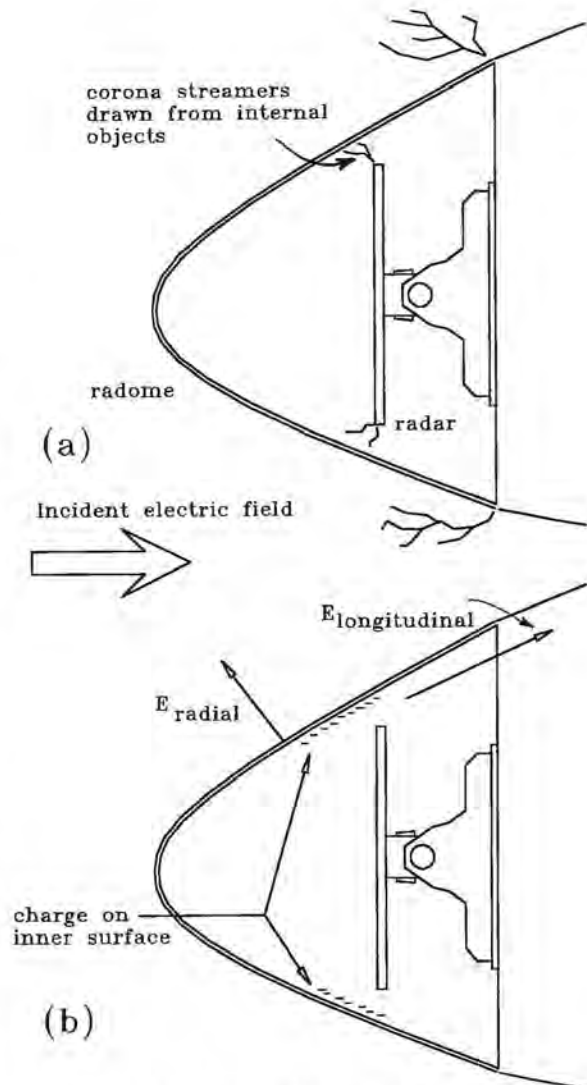
Fig. 6.24 Streamers and charges induced by an incident electric field.
