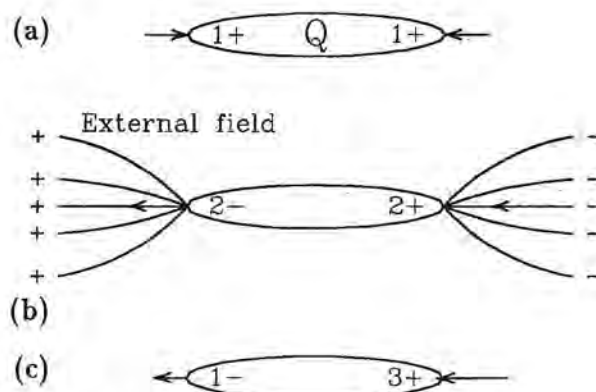
Fig. 10.7 Charge distribution. (a) Due to a net charge (b) Due to an external field (c) Due to both factors
