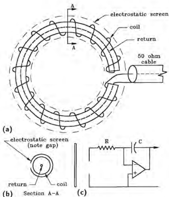
Fig. 18.33 Rogowski coil.
