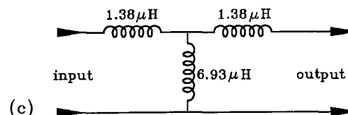
Fig. 18.27 Equivalent circuit of a typical transformer.
