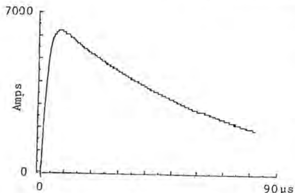
Fig. 13.14 Current waveform.
