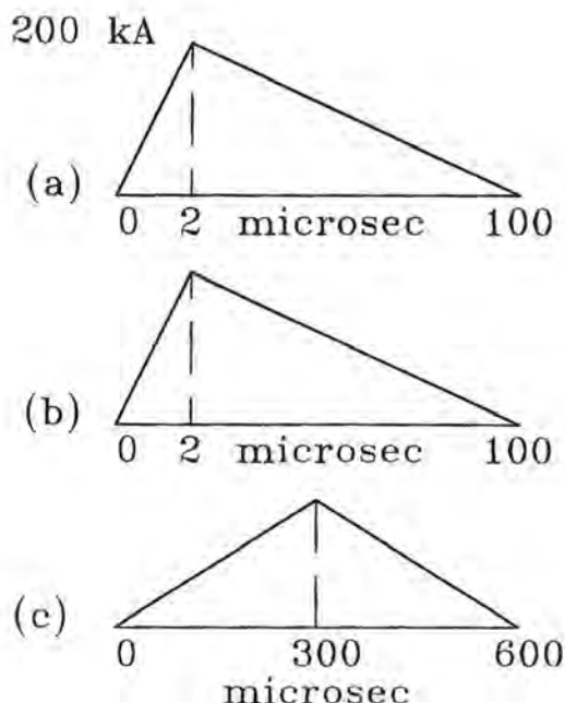
Fig. 14.18 Waveforms used for Orbiter analysis.
