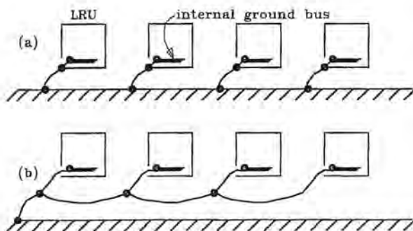
Fig. 16.5 Multiple point grounding.
