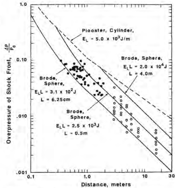
Fig. 6.15 Shock wave overpressure as a function of distance from a 4-m laboratory spark.
