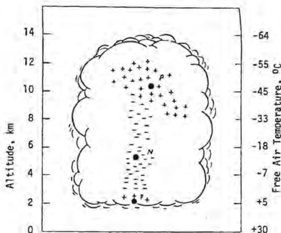
Fig. 3.19 Thunderstorm charge separation model.
