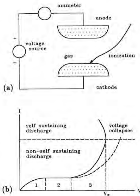
Fig. 1.1 Current-voltage relations in pre-spark regions.
