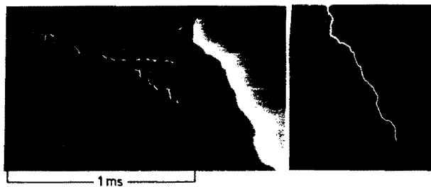
Fig. 2.8 Boys camera photograph of a lightning leader [2.15]
