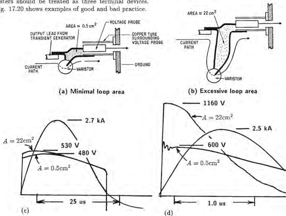
Fig. 17.19 Lead effects [17.1].
