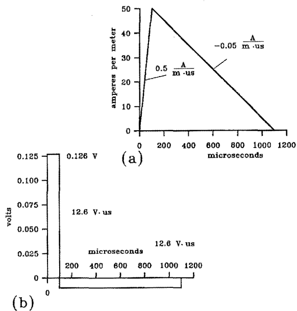
Fig. 14.27 Magnetic field effects in zone C.
