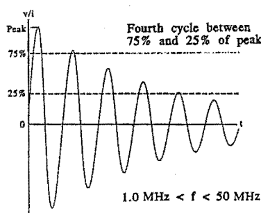
Voltage Waveform 3
