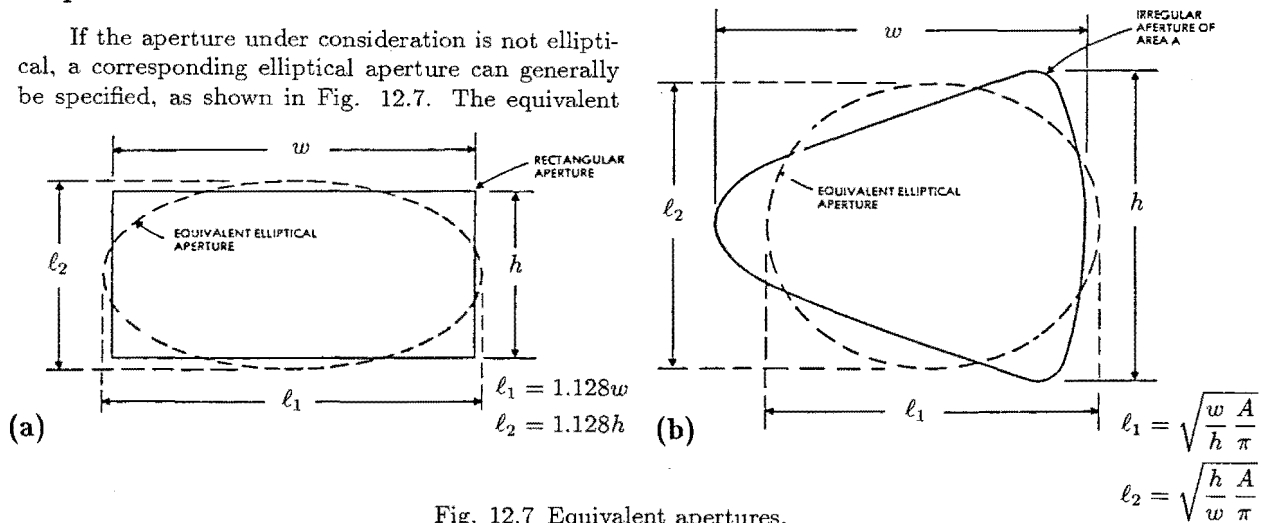
Fig. 12.7 Equivalent apertures.
