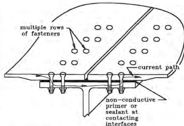
Fig. 7.24 Bonding through mechanical fasteners. Mating surfaces coated with non-conductive finishes and sealers.
