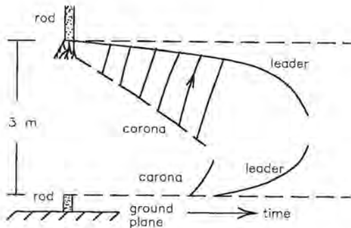
Fig. 1.21 Negative polarity sparkover of 3 meter gap rod to rod on plane gap. 1.5/1000 microsecond wave. Adapted from [1.1] and [1.10].
