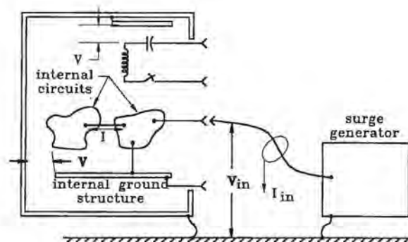
Fig. 18.34 Pin injection on an ungrounded system.
