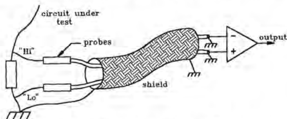
Fig. 13.21 Differential amplifiers.
