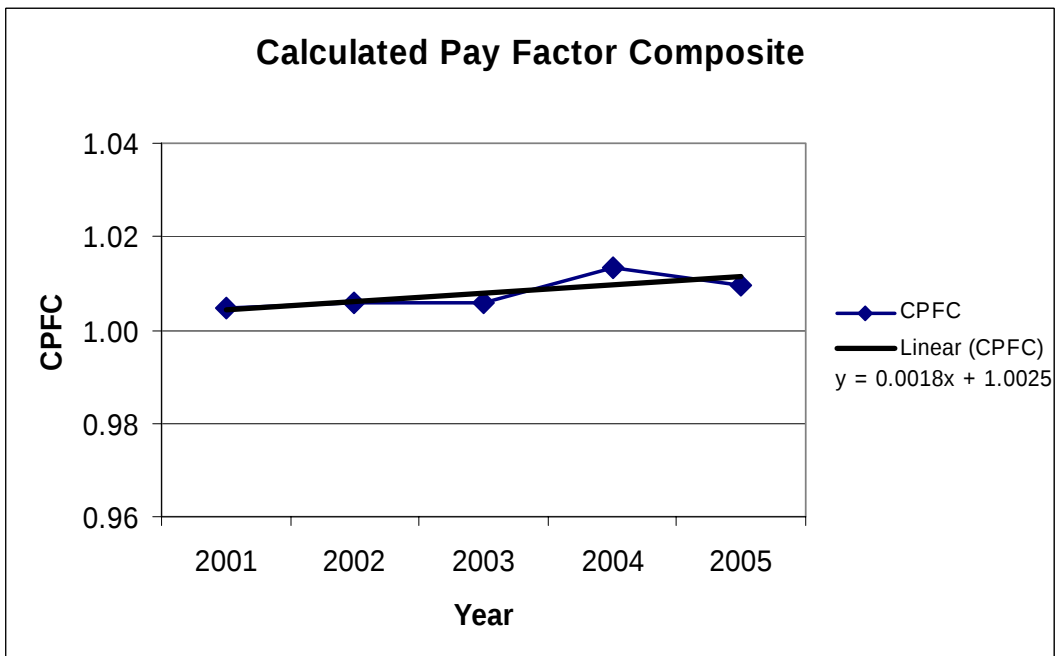
Figure 3. Calculated Pay Factor Composite by Year with Trendline
