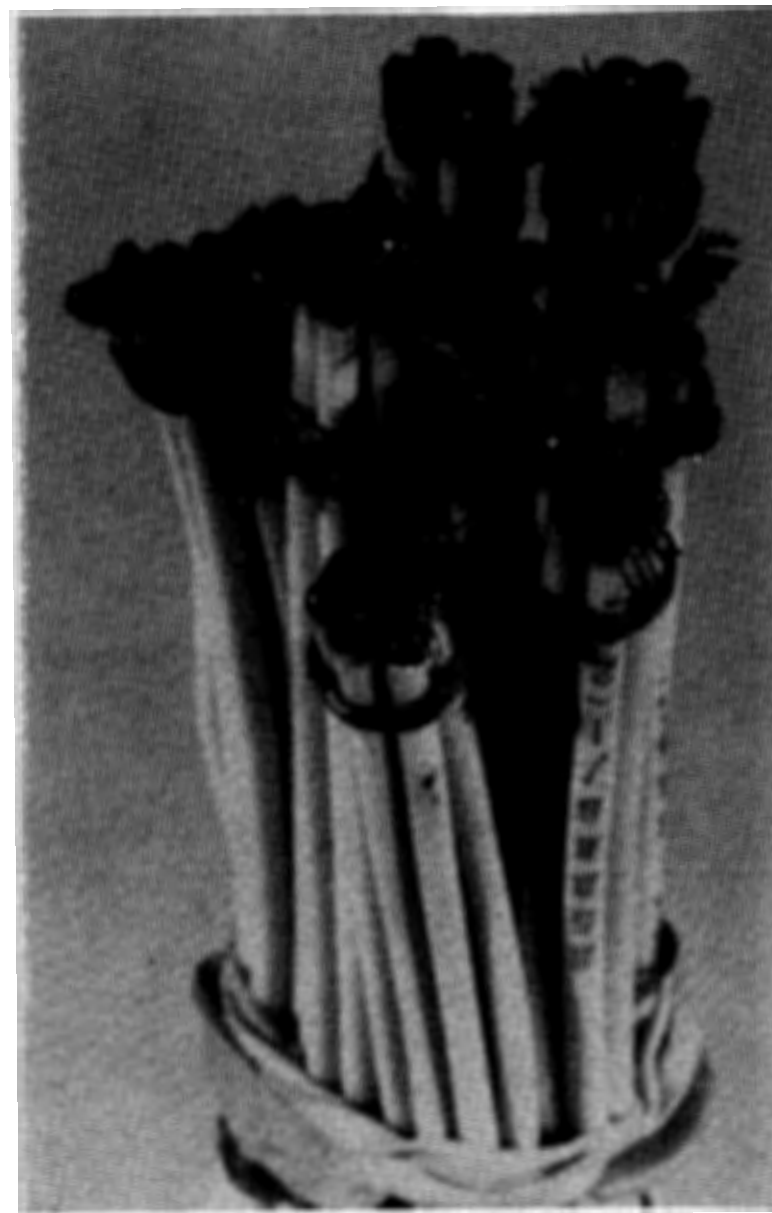
FIGURE 5. MIL-W-5086/1 PHOTOGRAPH
