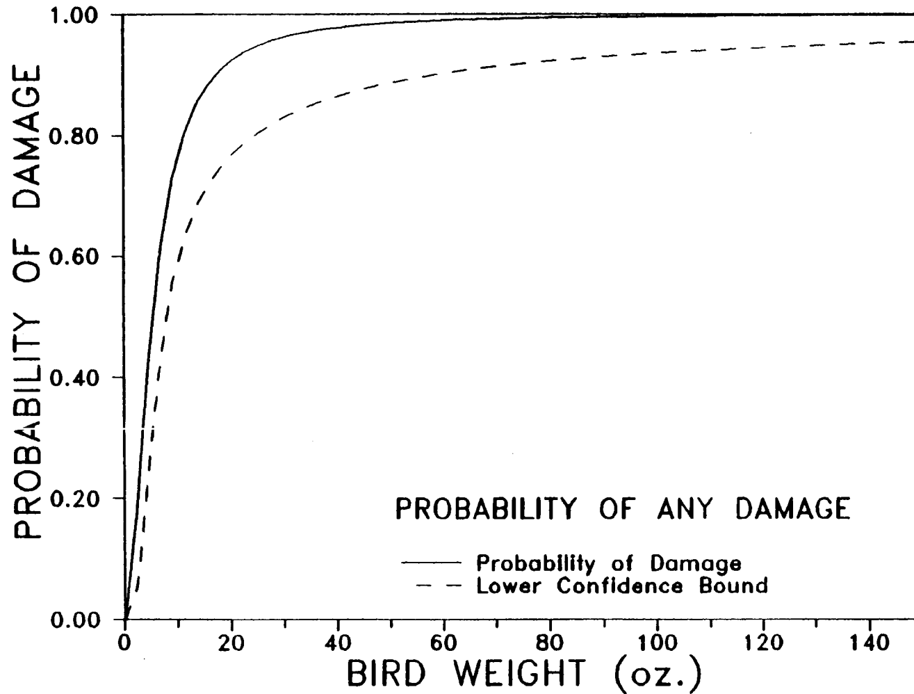
Figure 6.1 Estimated POD Function for Any Damage with the 95 Percent Confidence Bound.
