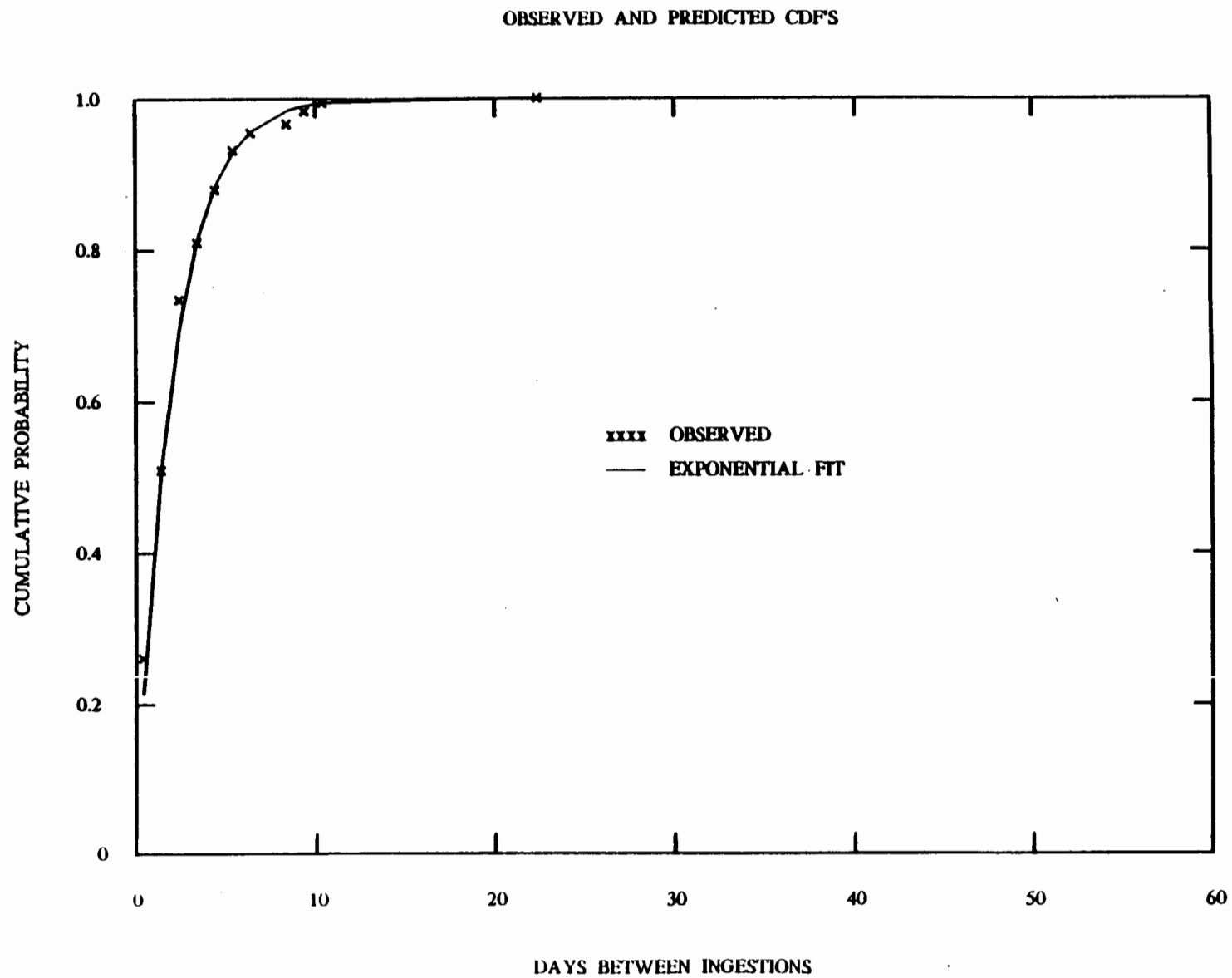
Figure 4.3 Comparison of Observed and Predicted CDFs for Foreign JT8D Aircraft Ingestion Events
