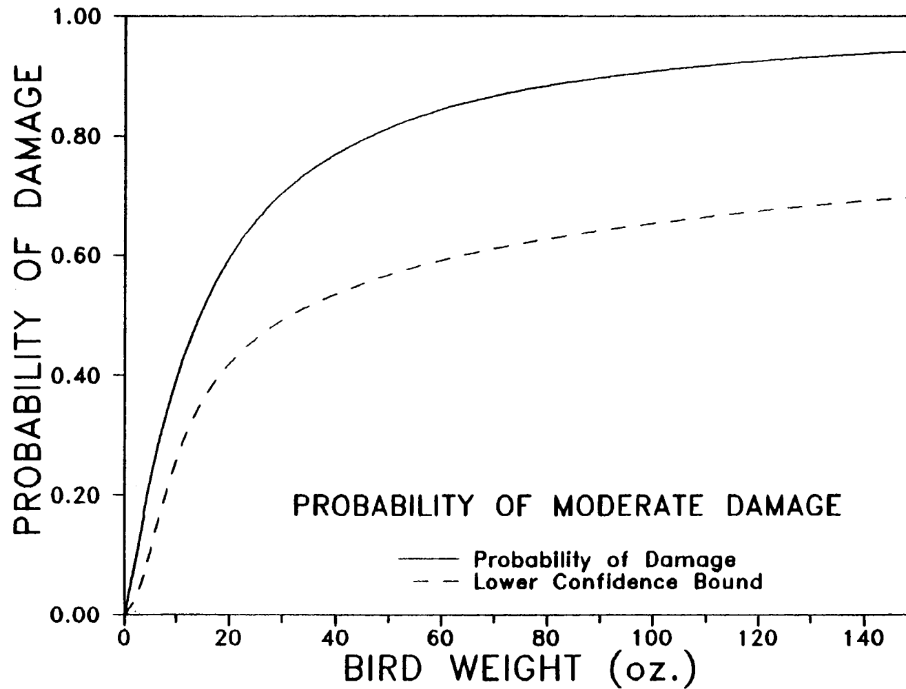
Figure 6.2 Estimated POD Function for Moderate or Worse Damage with the 95 Percent Confidence Bound.
