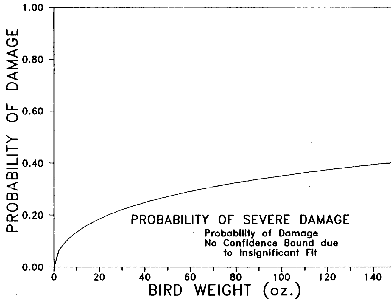
Figure 6.3 Estimated POD Function for Severe Damage.
