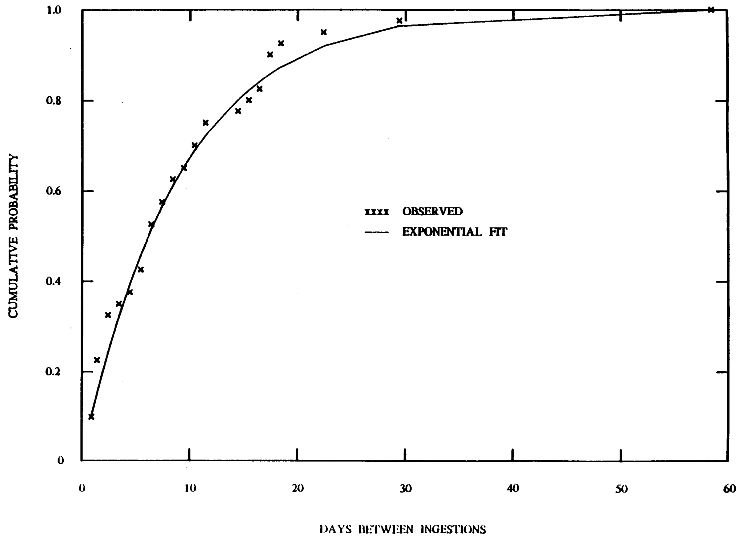
Figure 4.4 Comparison of Observed and Predicted CDFs for Domestic CFM56 Aircraft Ingestion Events
