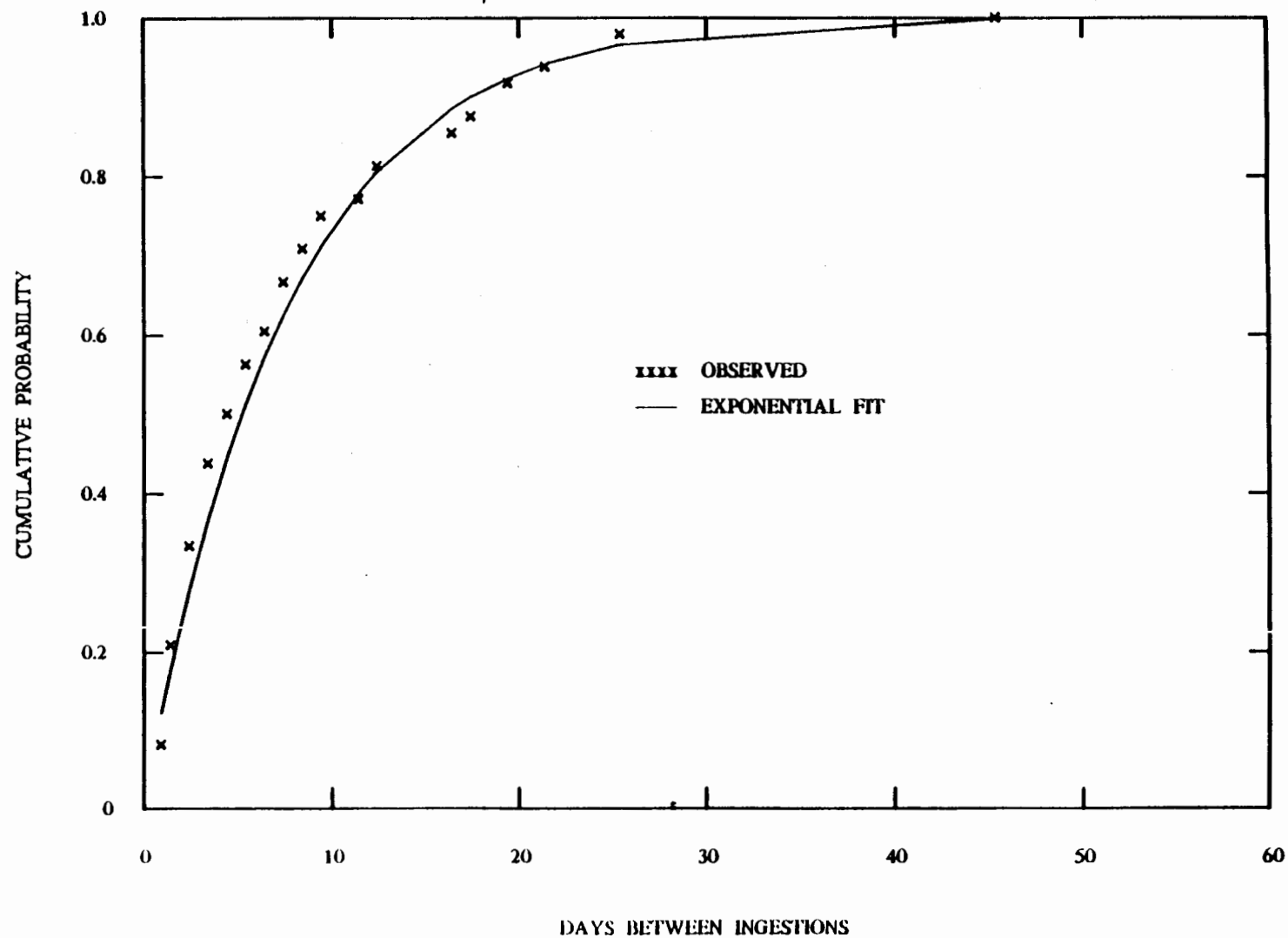
Figure 4.5 Comparison of Observed and Predicted CDFs for Foreign CFM56 Aircraft Ingestion Events
