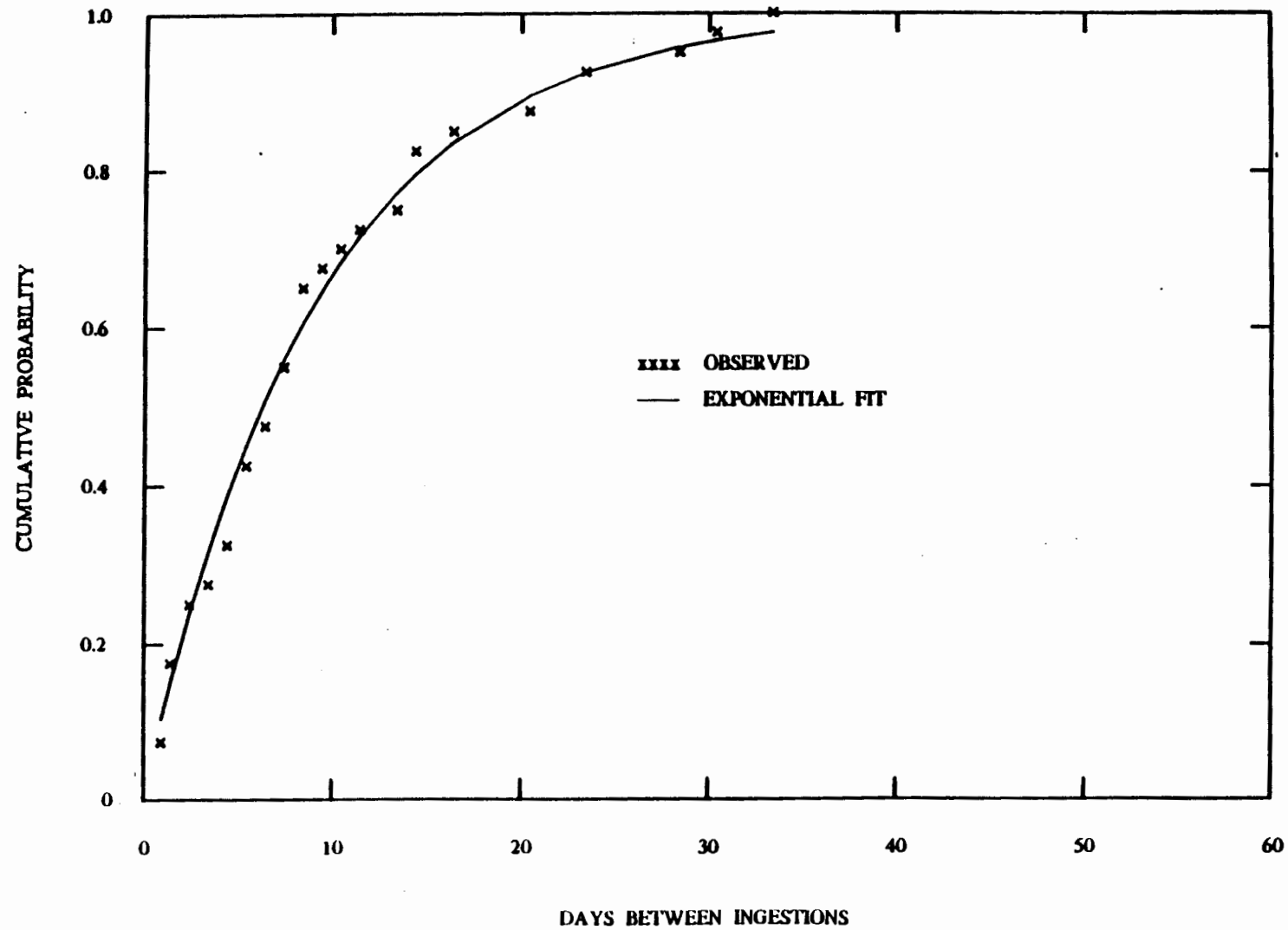
Figure 4.2 Comparison of Observed and Predicted CDFs for Domestic JT8D Aircraft Ingestion Events
