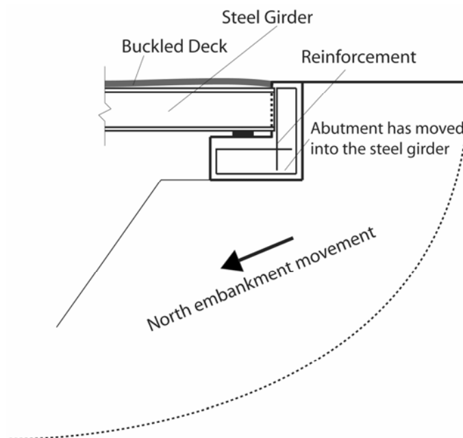
Figure 1: Mead Bridge abutment
