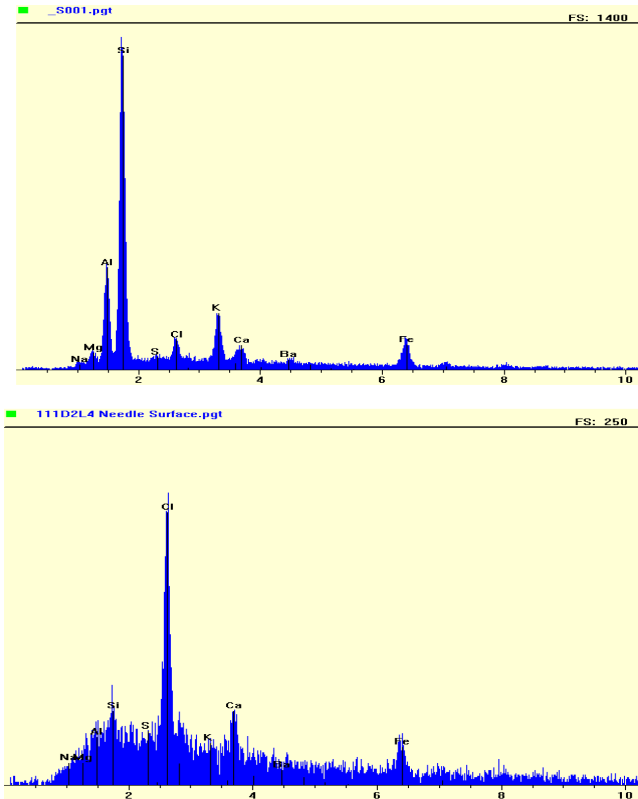
Figure 8. Two elemental analyses of surface deposits on P.contorta needles, site 111D (I-70), documenting the presence of Na, Mg, and Cl, as well as minerals associated with quartz and feldspars (see also Figure 7. f).
