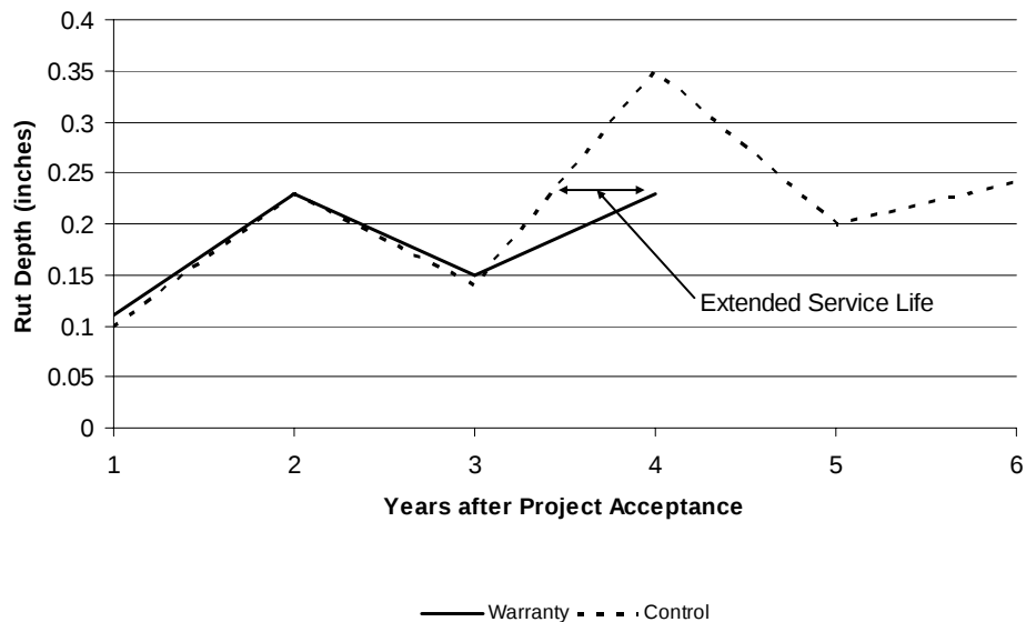
Figure 20 Comparison of the US 50 Kannah Creek / US 50 Whitewater rut depth performance
