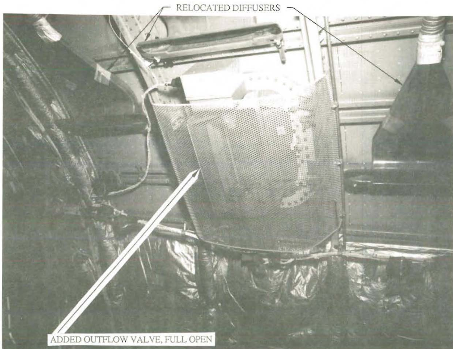
FIGURE 2.1.1-1 FORWARD CABIN MODIFICATIONS
