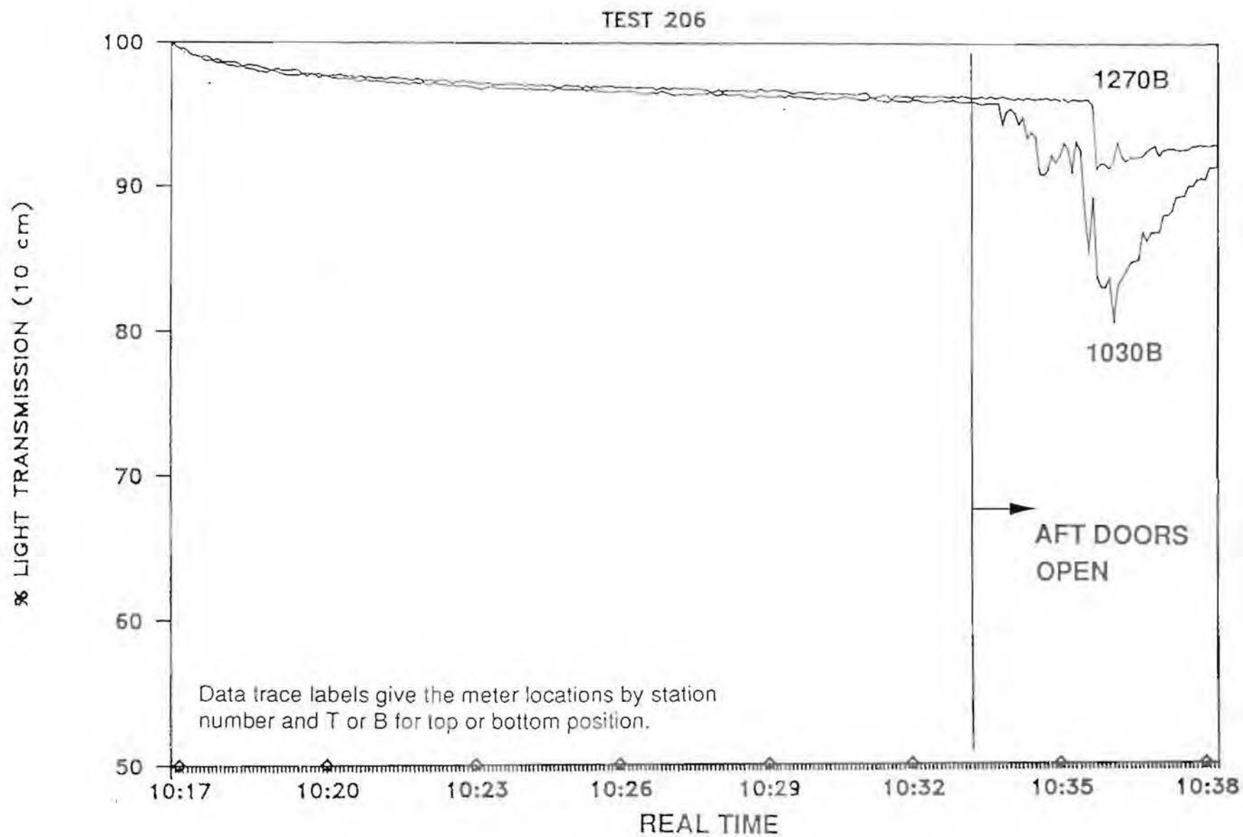
FIGURE 4.2.1-6 SMOKE METER DATA, TEST .206
