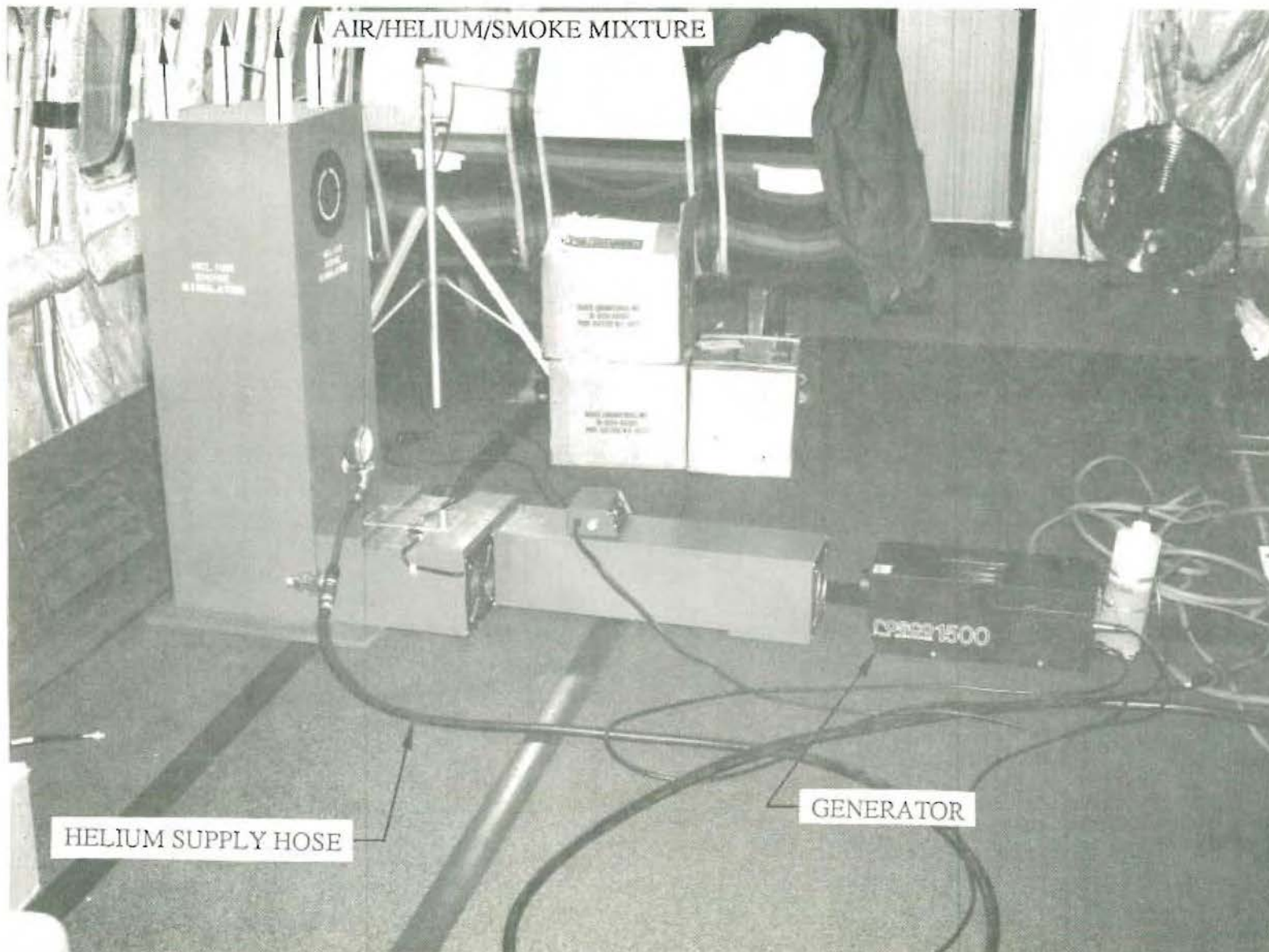
FIGURE 2.2.1-1 HELIUM/SMOKE MIXING CHAMBER
