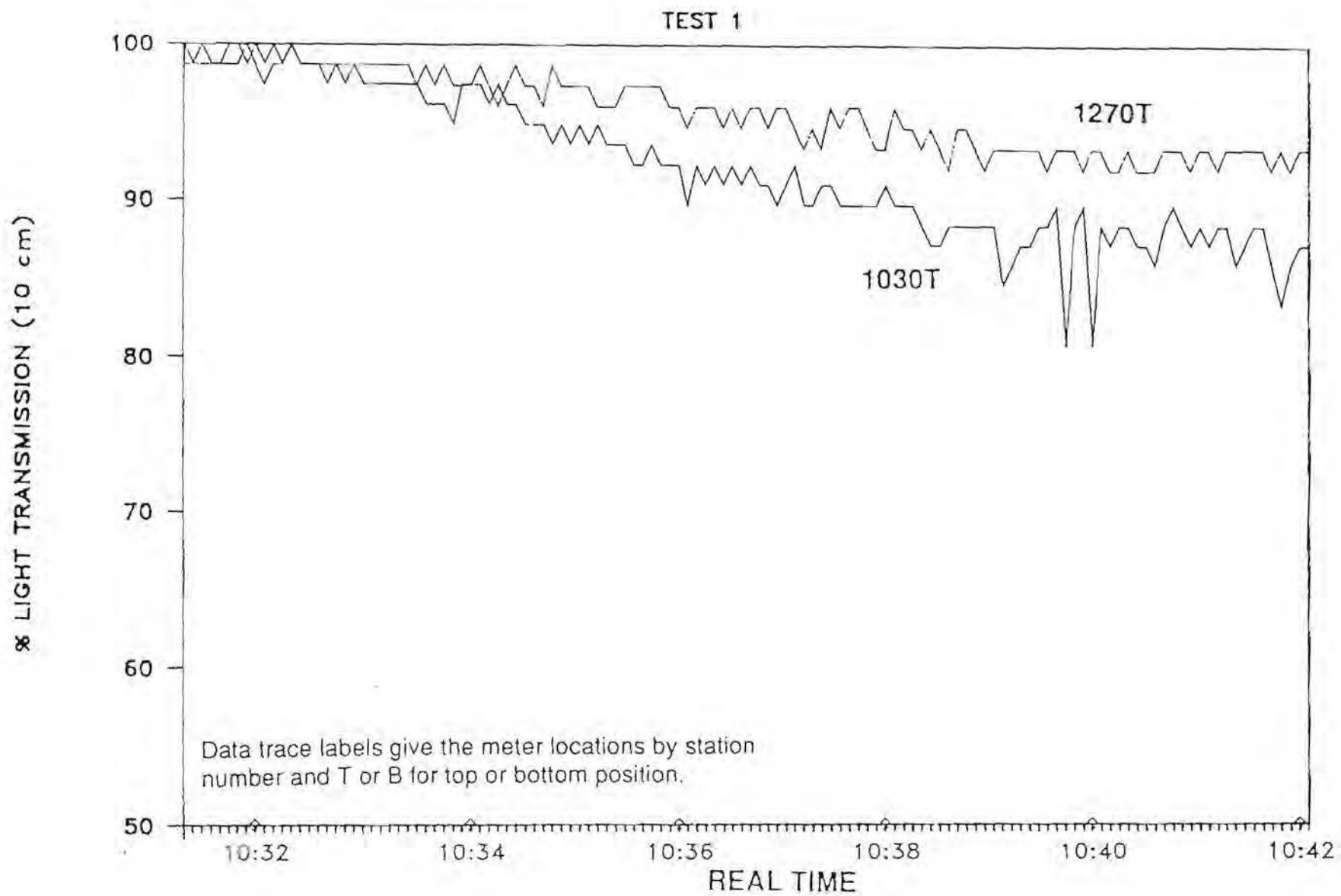
FIGURE 4.2.1-1 SMOKE METER DATA, TEST .001
