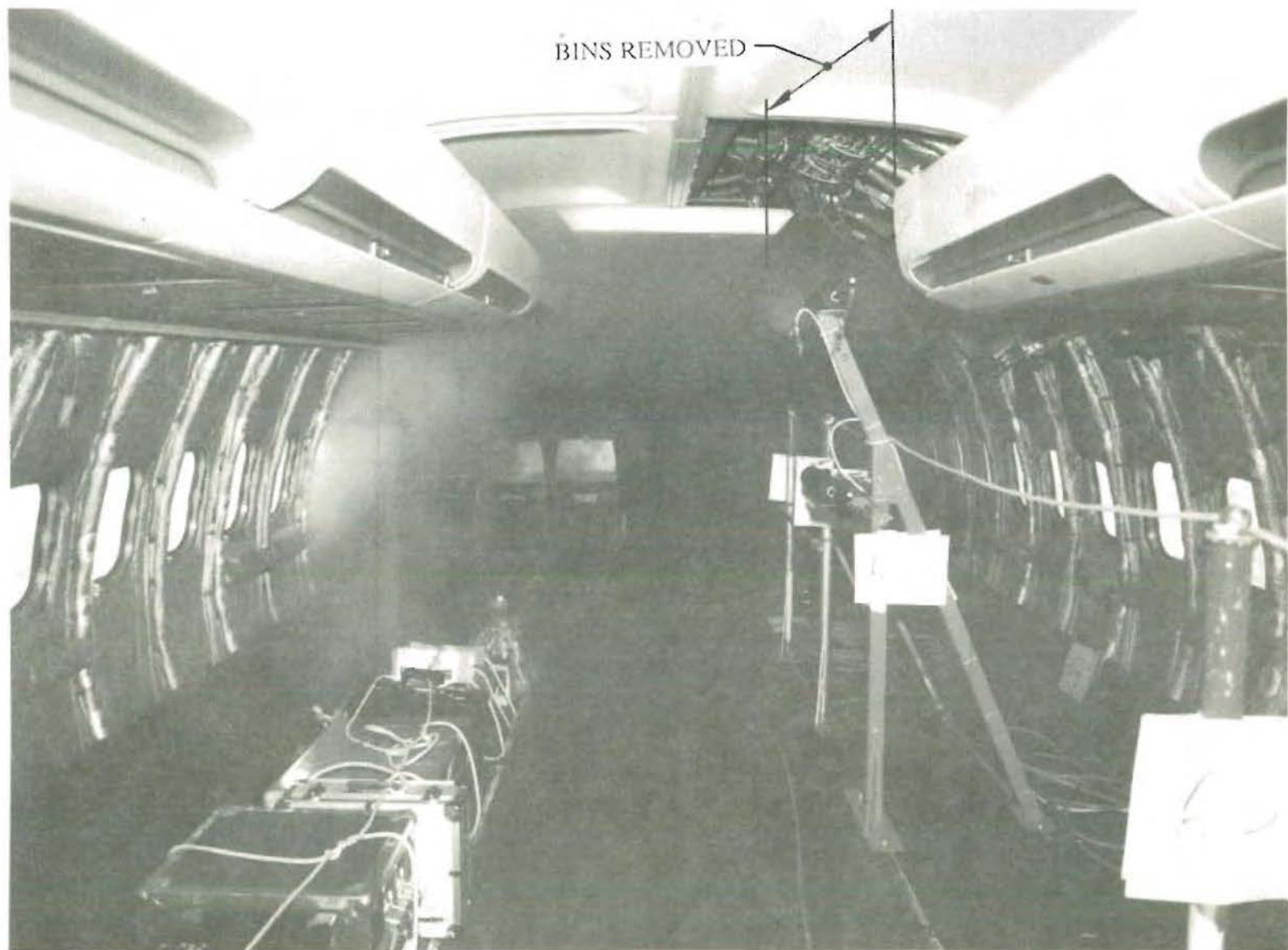
FIGURE 2.1.1-11 FORWARD BINS REMOVED
