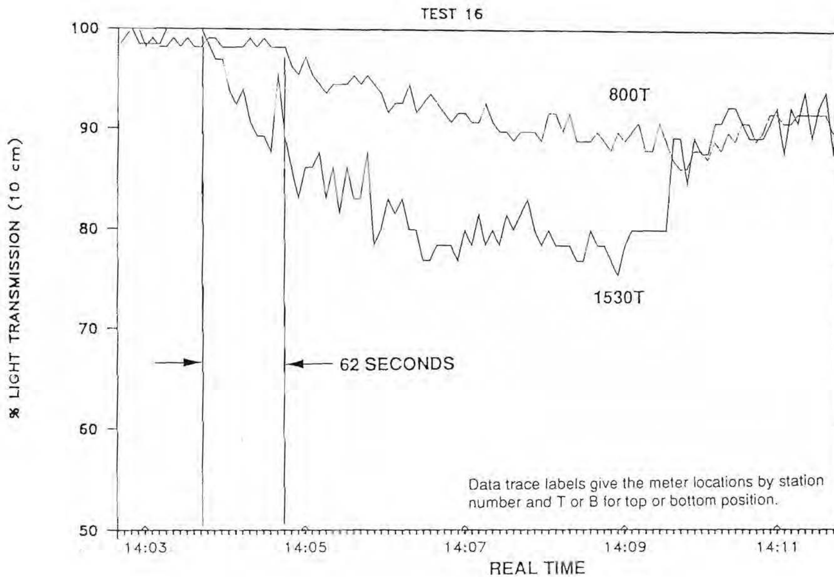
FIGURE 4.2.1-3 SMOKE METER DATA, TEST .016
