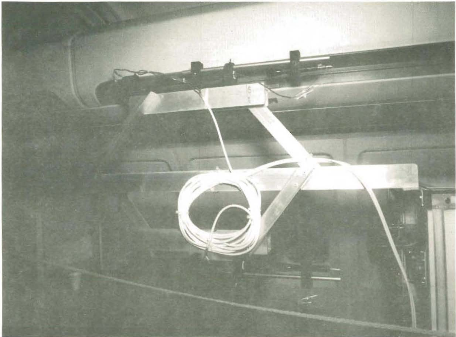
FIGURE 2.3.2-2 SMOKE METERS, STATION 1530
