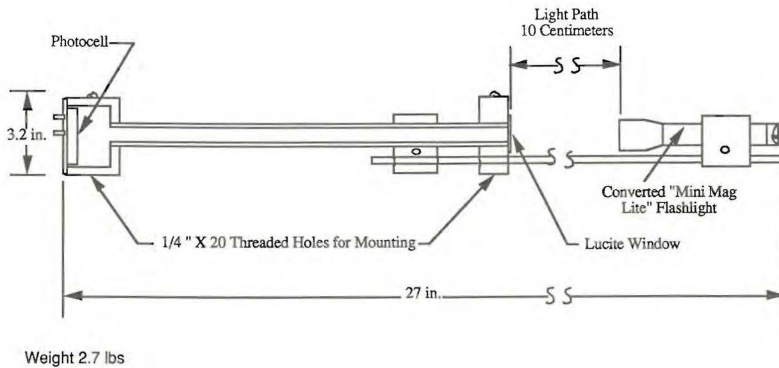
FIGURE 2.3.2-3 SMOKE METER DETAILS
