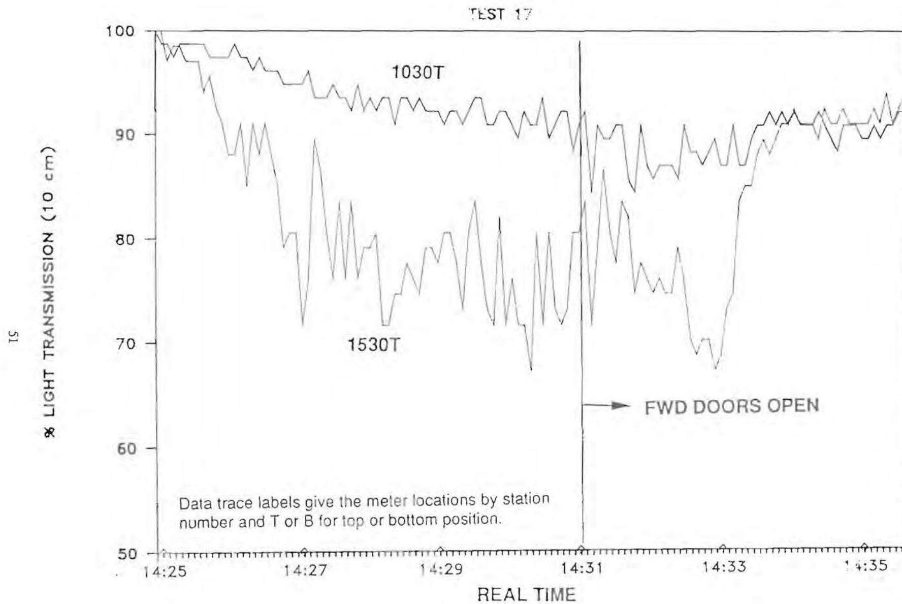
FIGURE 4.2.1-5 SMOKE METER DATA, TEST .017
