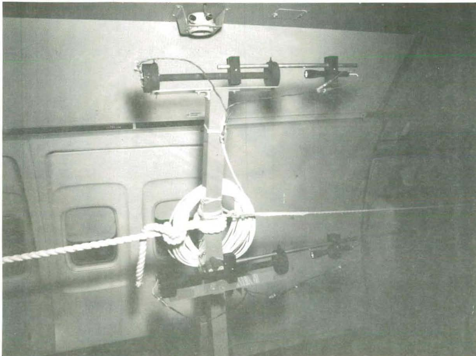
FIGURE 2.3.2-1. SMOKE METERS, TYPICAL FOR STATIONS 560, 800, 1030 AND 1270
