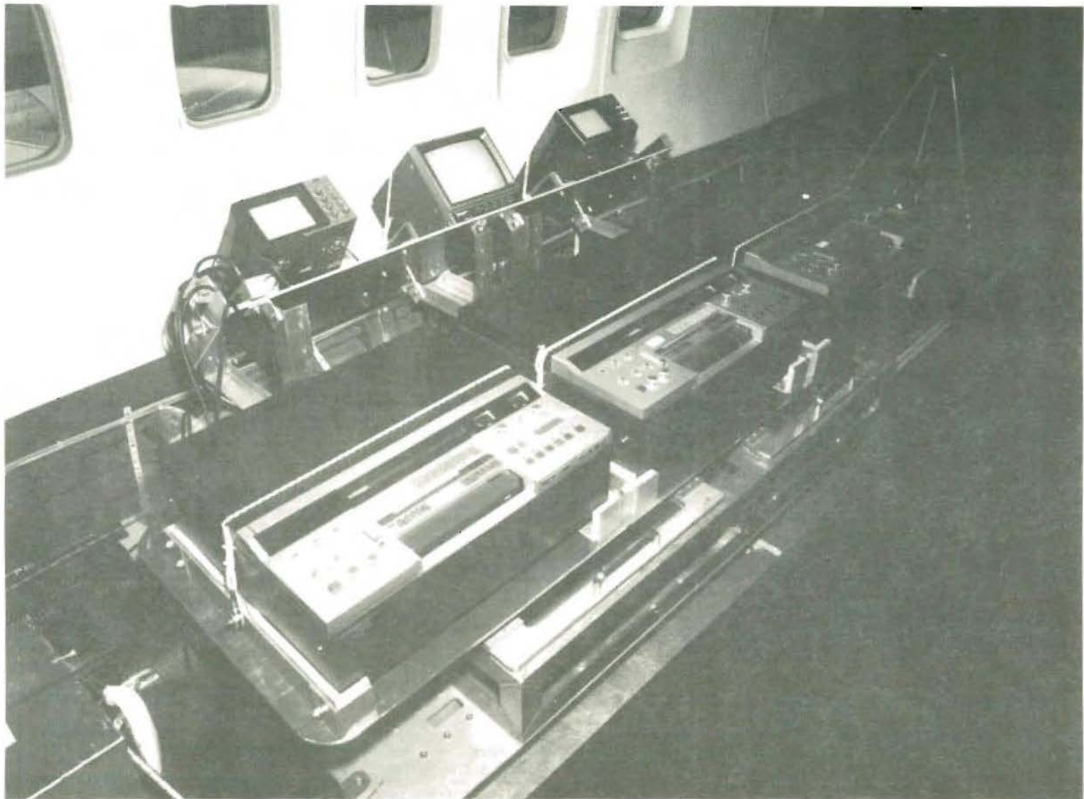
FIGURE 2.3.1-4 VIDEO RECORDERS AND MONITORS
