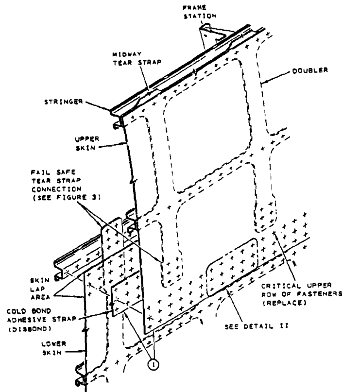
Figure 7. Lap joint inspection specification.
