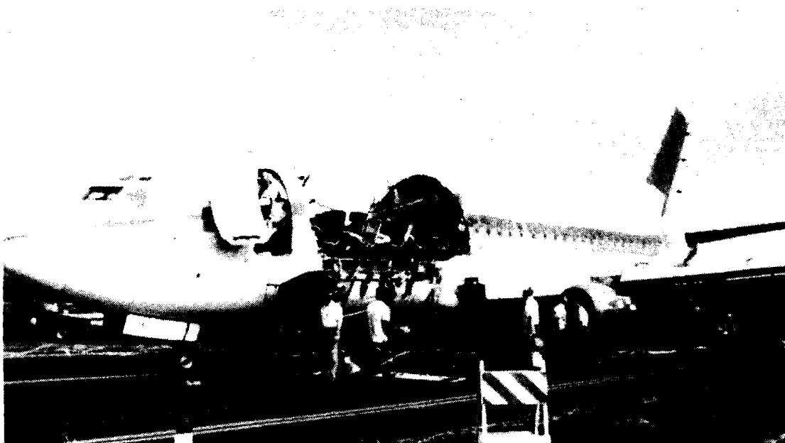
Figure 1. An extreme example of aging effect. This aircraft suffered an in-flight structural failure.
