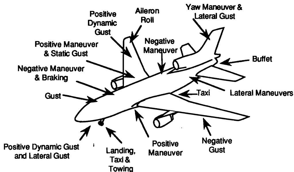
Figure 6. Critical loads on aircraft structure.
