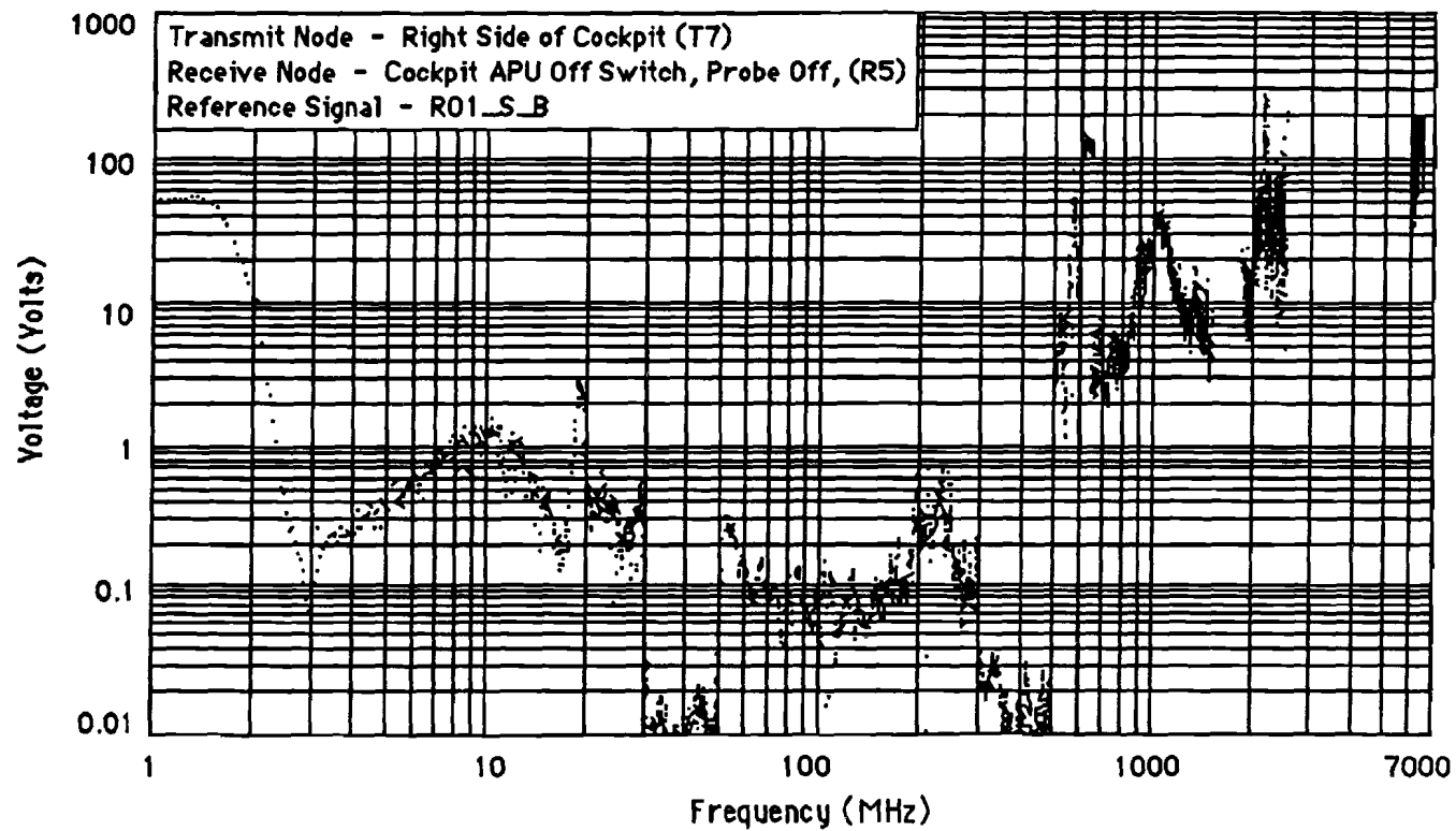
Figure F-17 Maximum Induced Voltage (138B)
