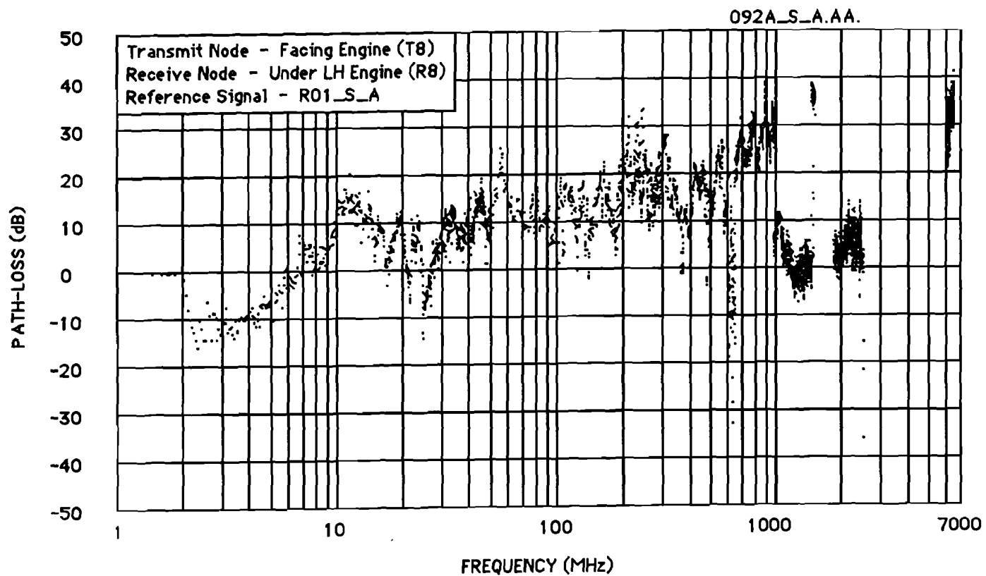
Figure E-25 Antenn Path-Loss Function (Test 092A)
