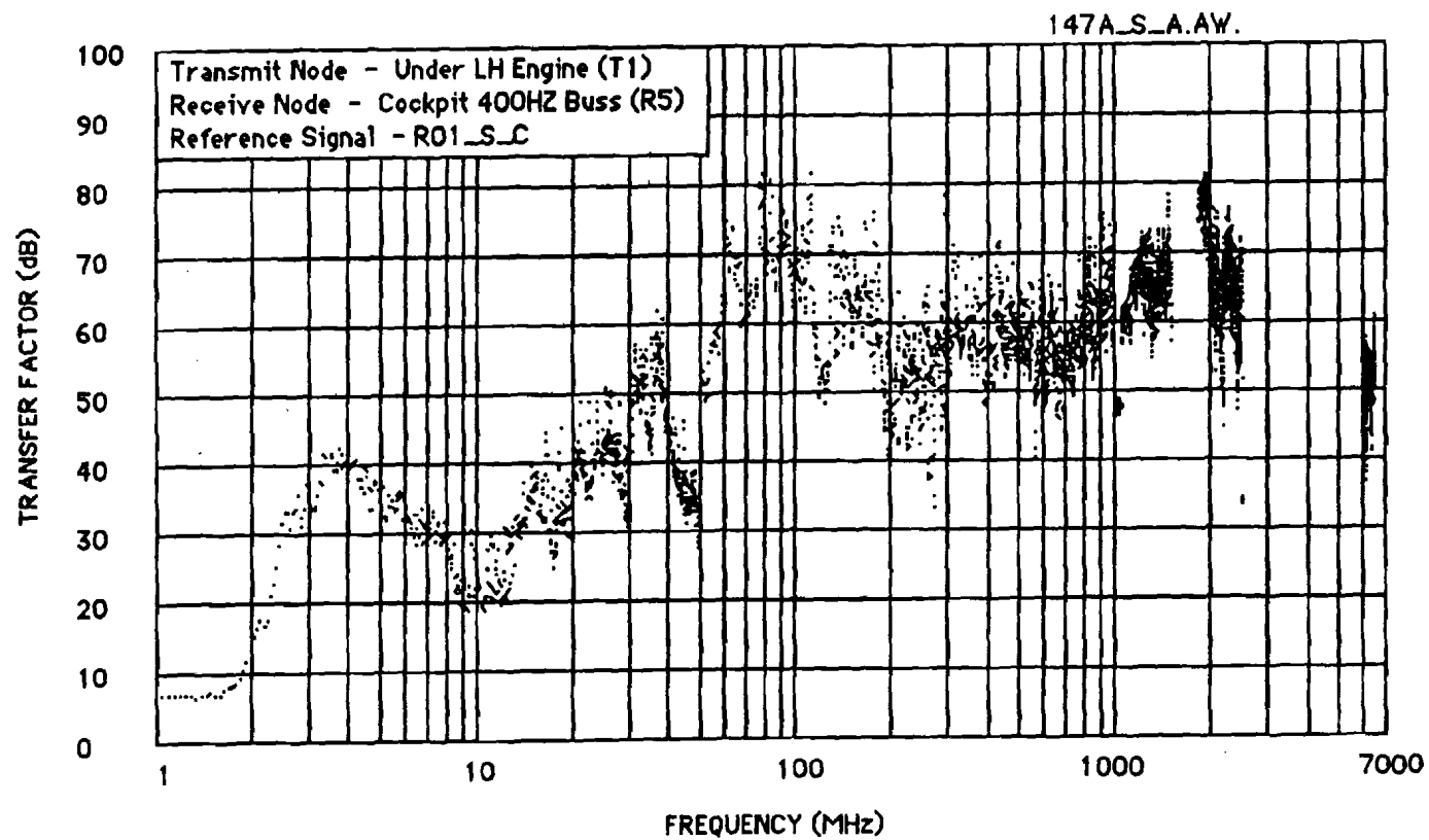
Figure E-23 Probe Transfer Factor (Test 147A)
