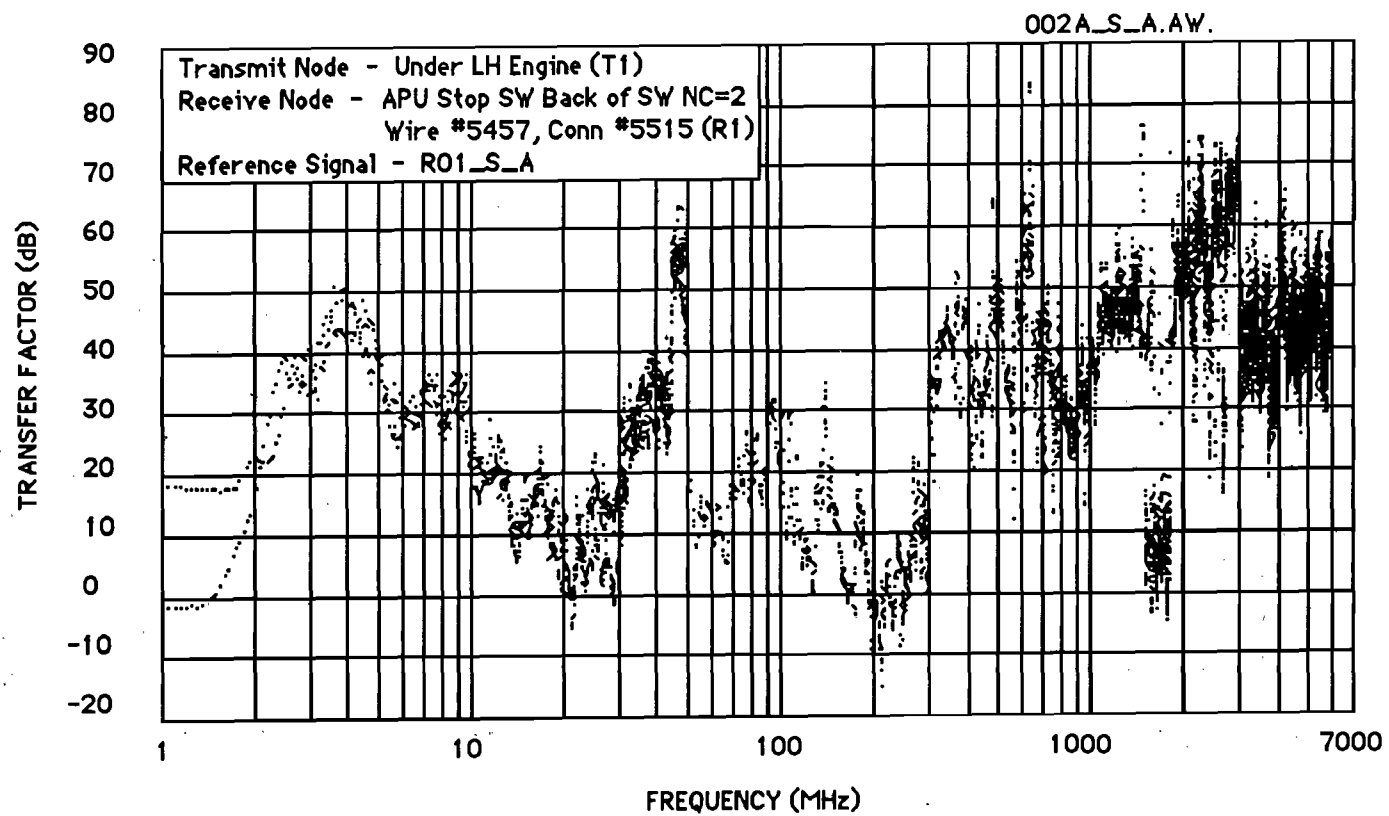
Figure E-4 Probe Transfer Factor (Test 002A)
