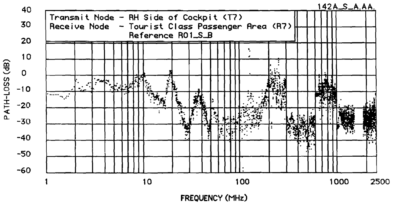
Figure 7.3.7 Antenna Path-Loss Function (Test 142A)
