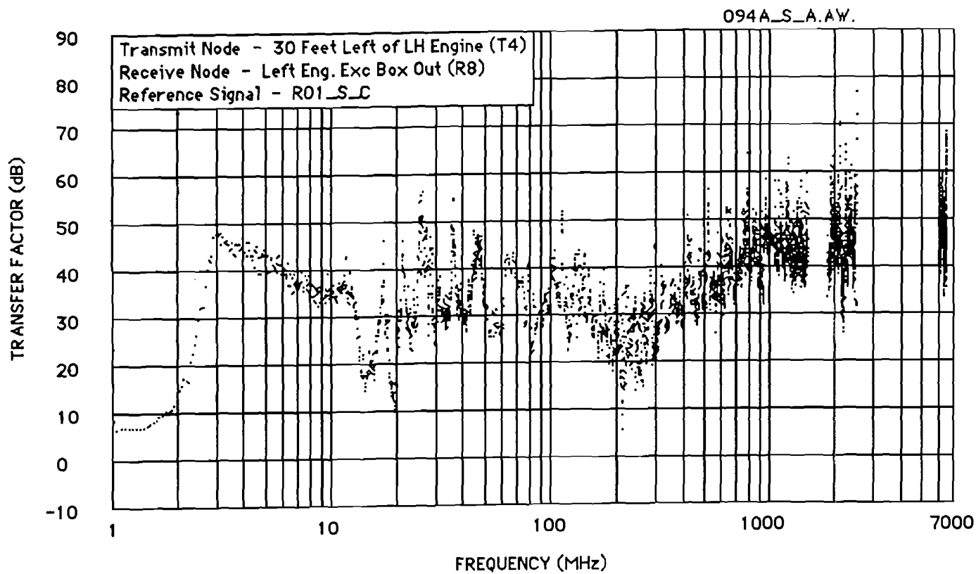
Figure E-12 Probe Transfer Factor (Test 094A)
