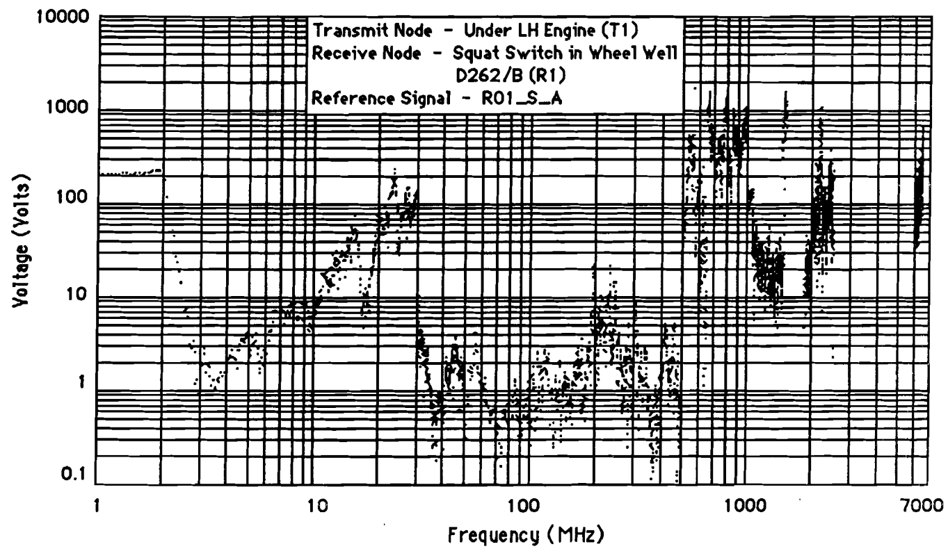
Figure F-3 Maximum Induced Voltage (013A)
