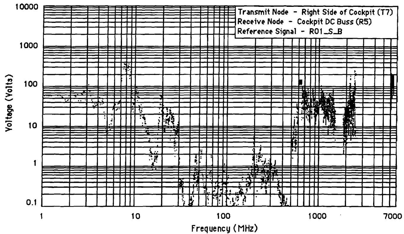
Figure F-15 Maximum Induced Voltage (133A)
