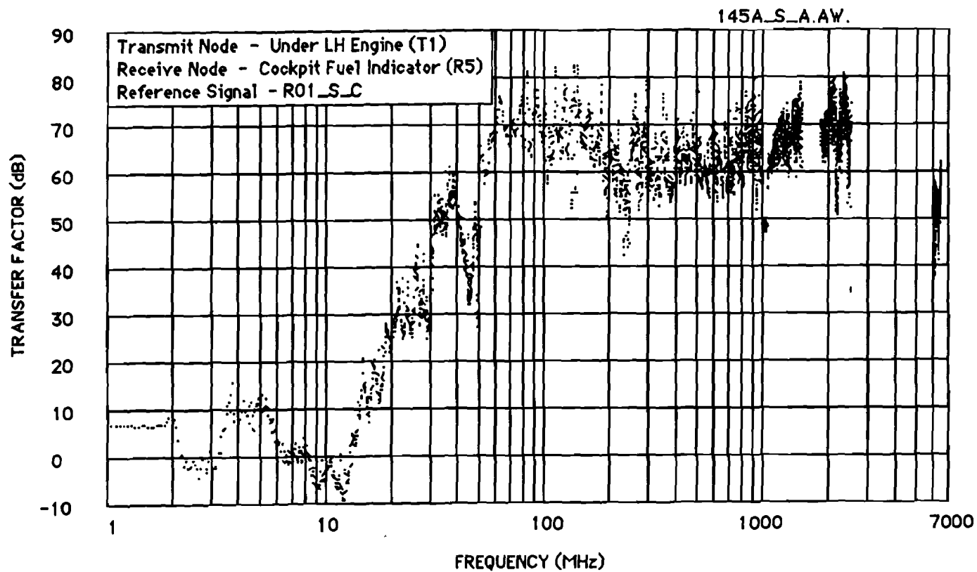
Figure E-22 Probe Transfer Factor (Test 145A)
