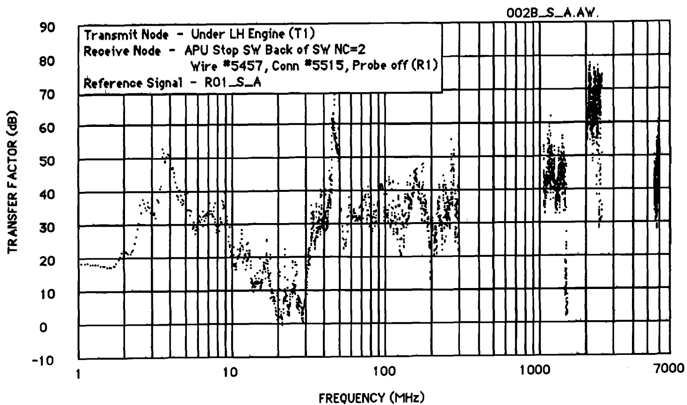
Figure E-5 Probe Transfer Factor (Test 002B)
