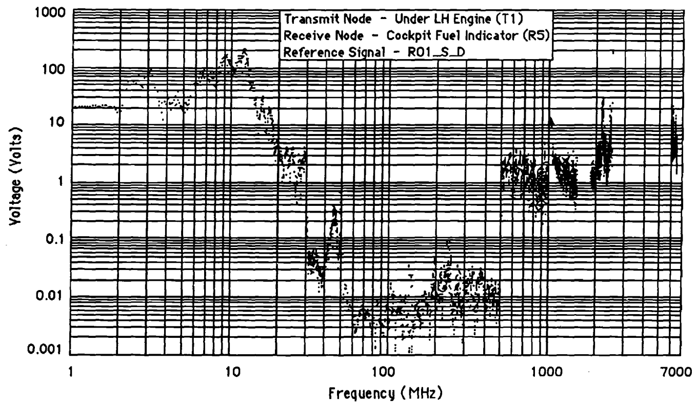
Figure F-19 Maximum Induced Voltage (145A)
