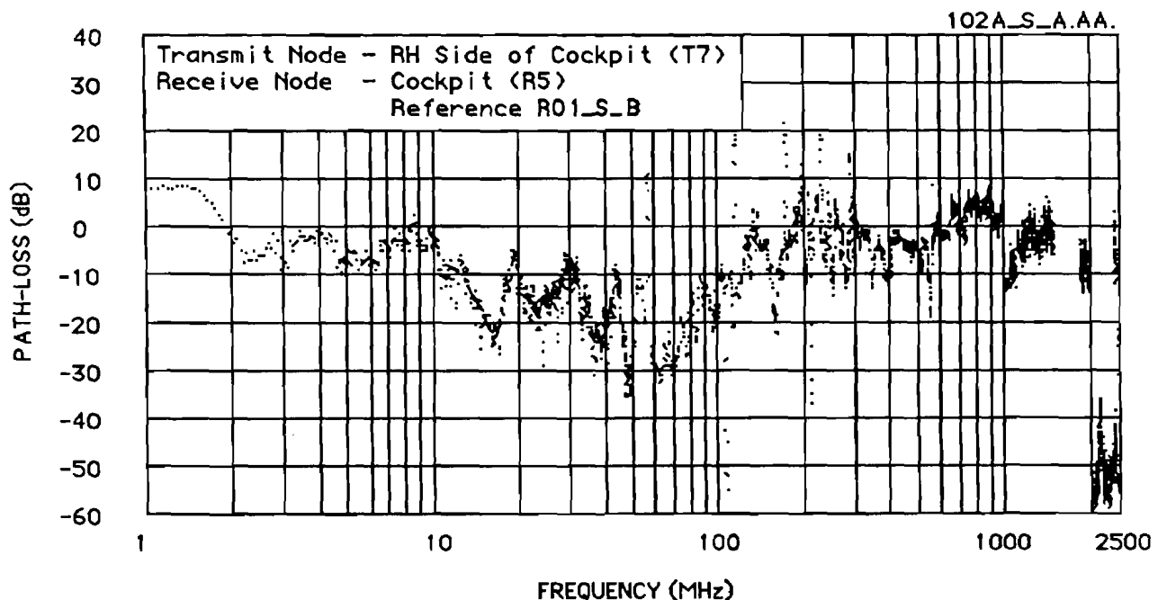
Figure 7.3.3 Antenna Path-Loss Function (Test 102A)
