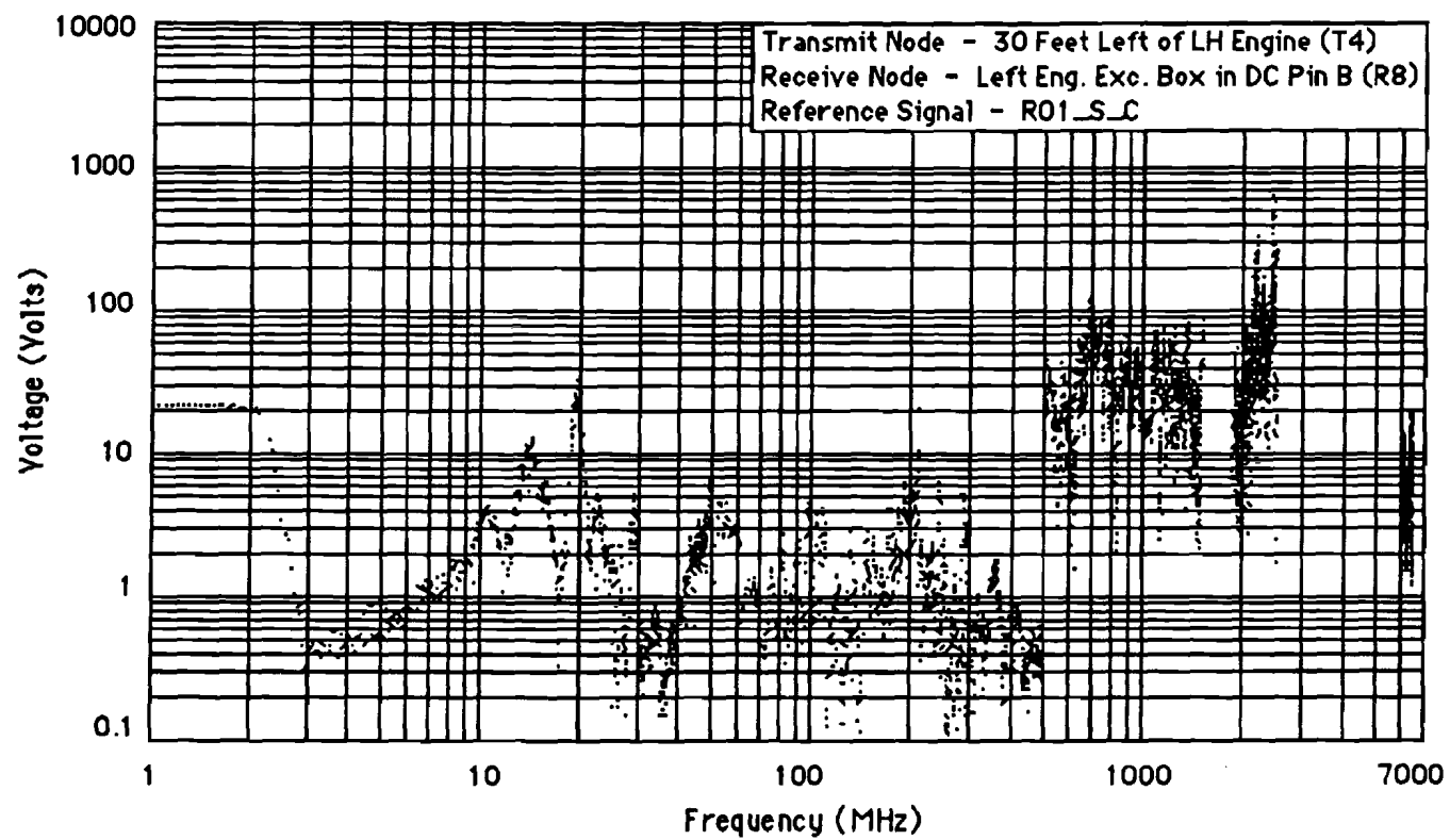
Figure F-7 Maximum Induced Voltage (093A)
