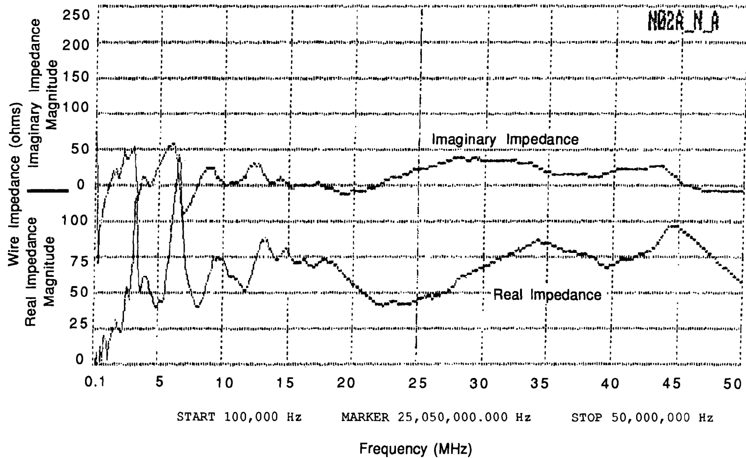
Figure 7.3.2 Typical Network Analyzer Data
