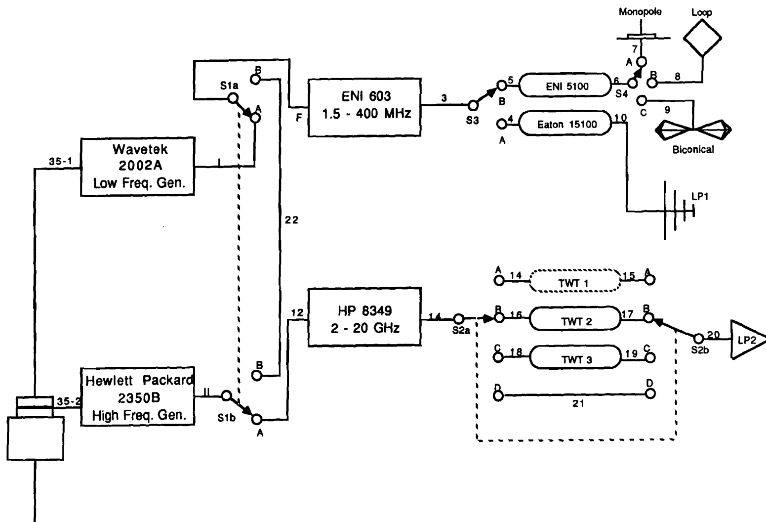
Figure 6.2.2 Field Test Transmit Node.
