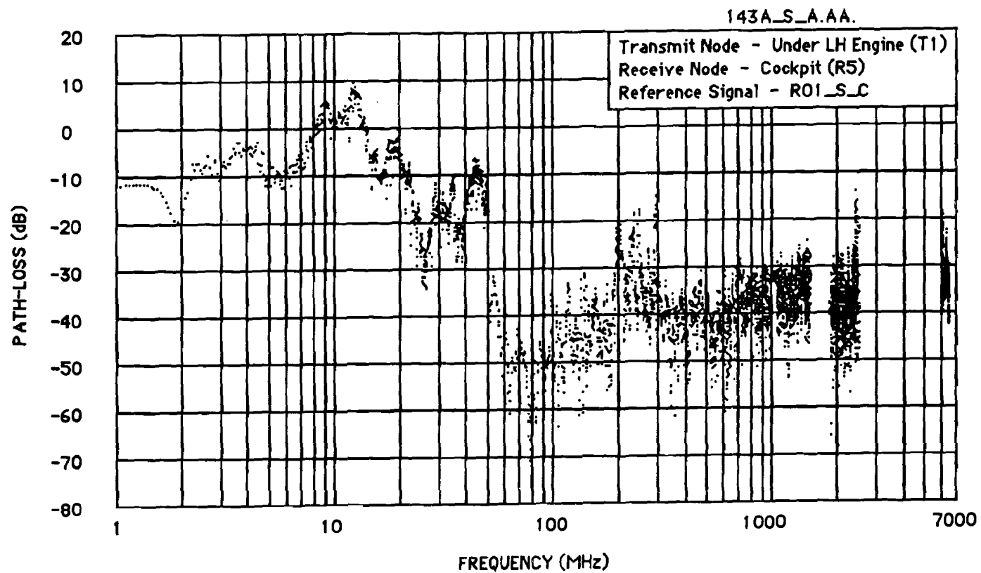
Figure E-28 Antenn Path-Loss Function (Test 143A)
