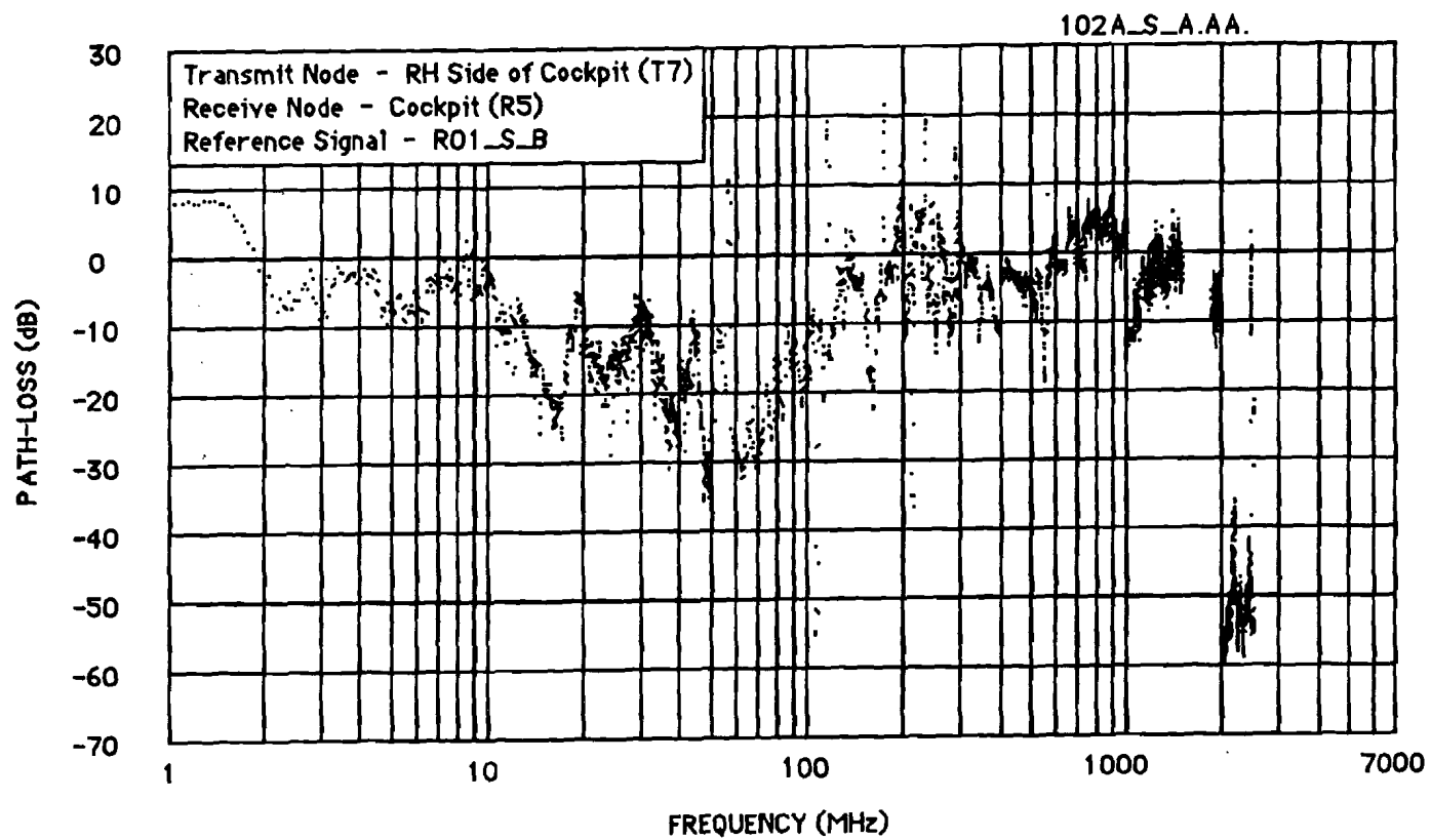
Figure E-26 Antenn Path-Loss Function (Test 102A)
