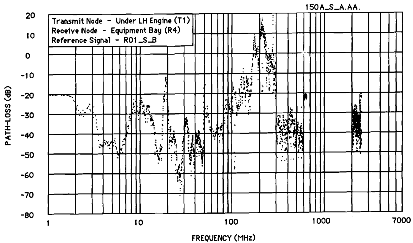
Figure E-30 Antenn Path-Loss Function (Test 150A)
