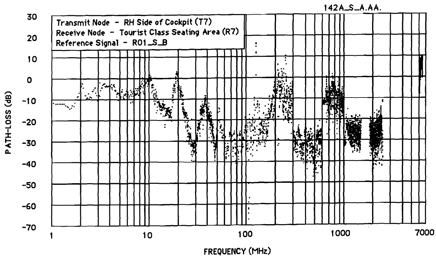
Figure E-27 Antenn Path-Loss Function (Test 142A)
