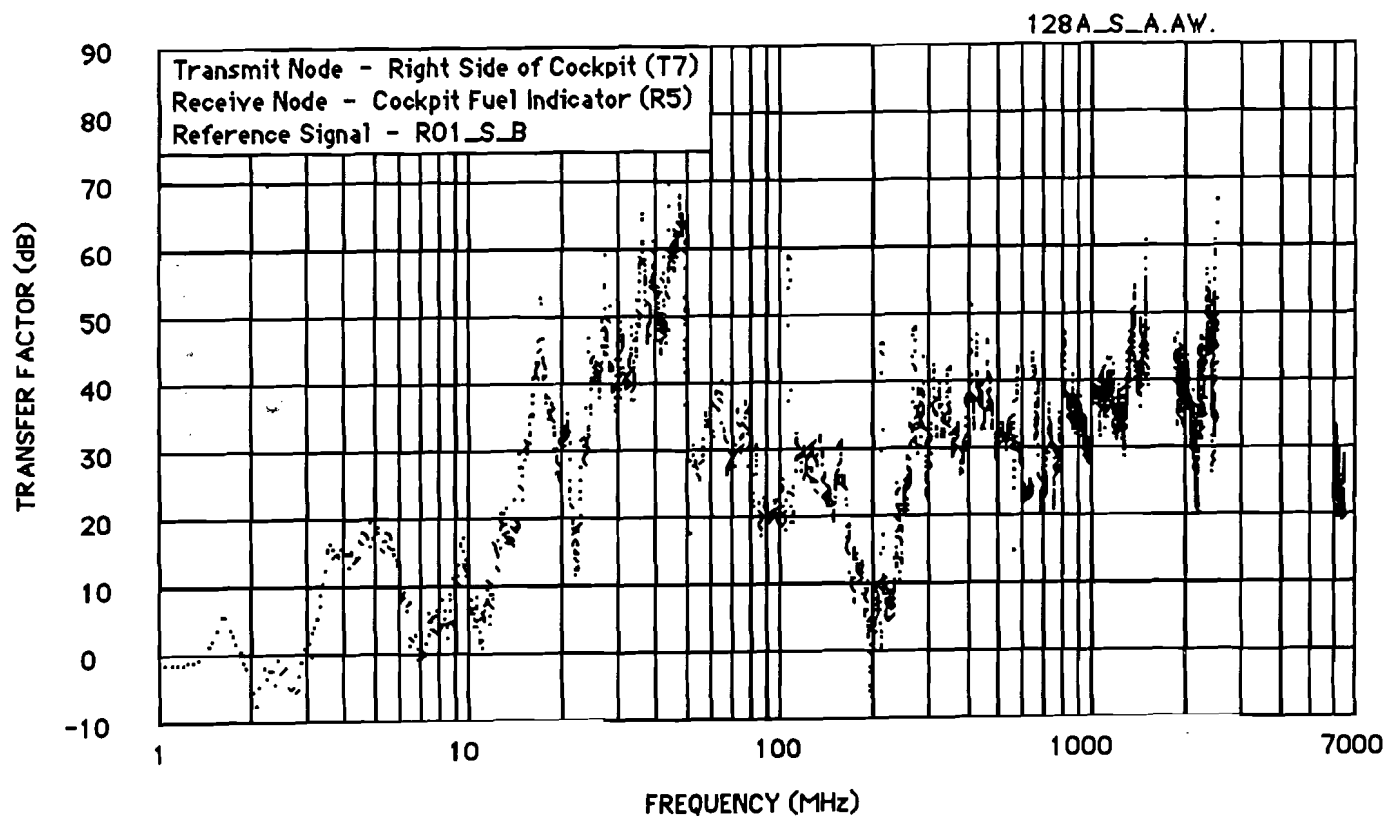
Figure E-16 Probe Transfer Factor (Test 128A)
