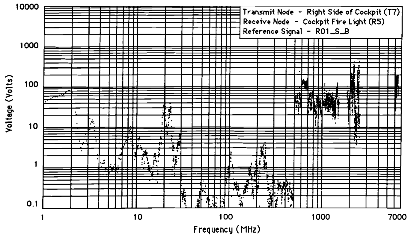
Figure F-12 Maximum Induced Voltage (126A)
