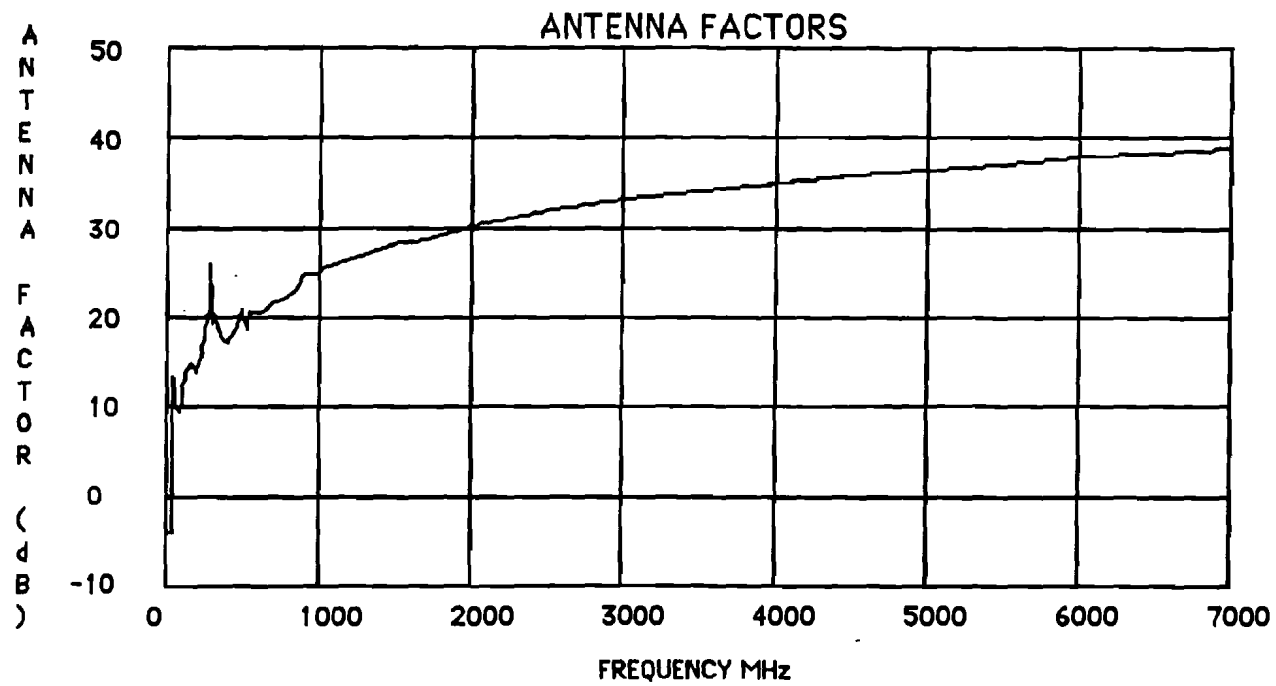
Figure E-2 Antenna Factors vs. Frequency
