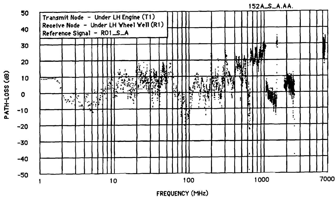
Figure E-32 Antenn Path-Loss Function (Test 152A)
