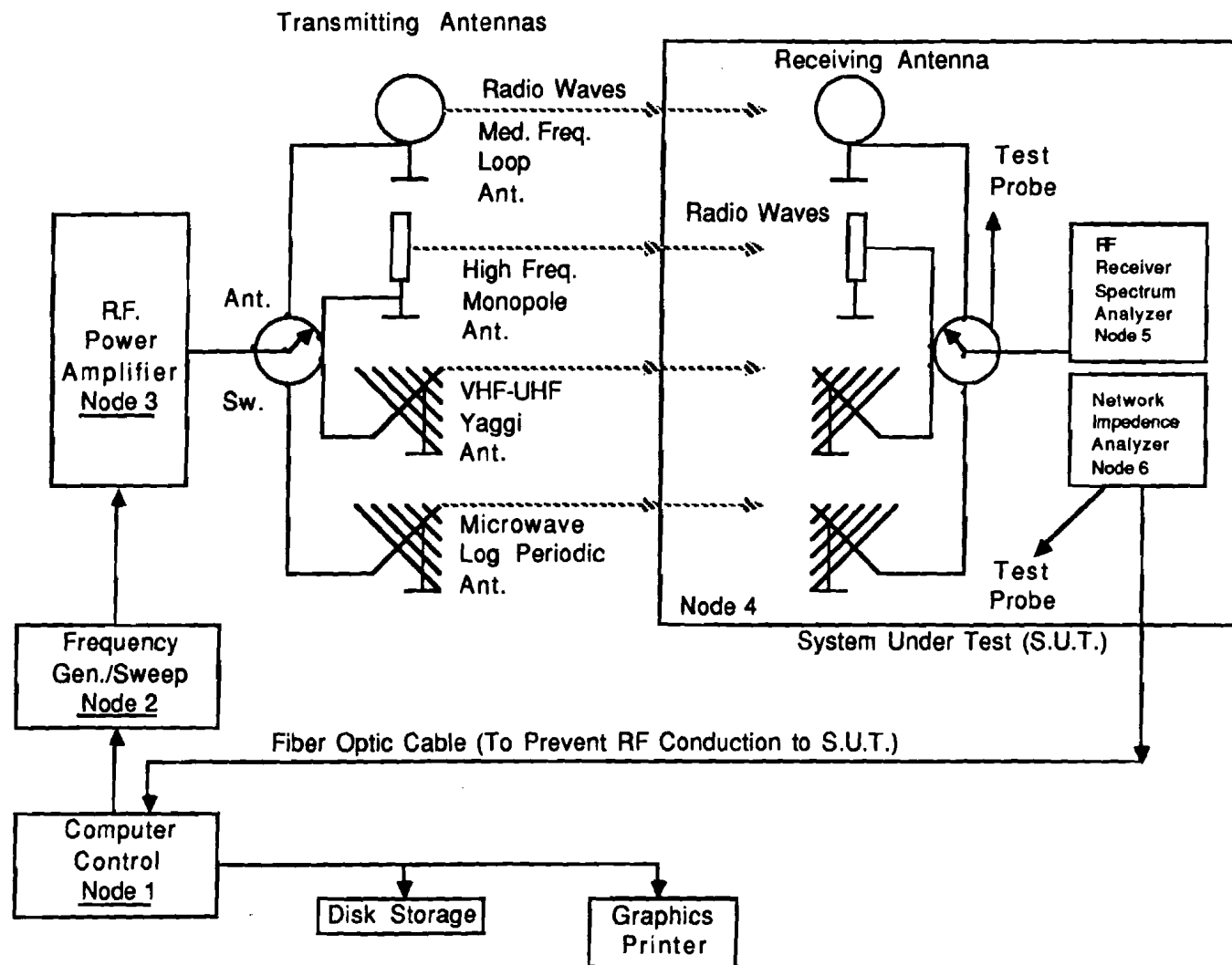
Figure 6.2.1 Field Test Data Acquisition System (DAS).
