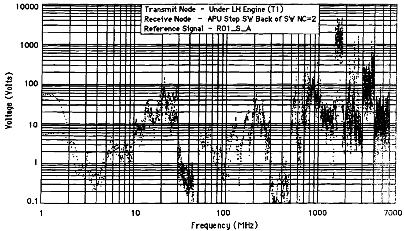
Figure F-1 Maximum Induced Voltage (002A)
