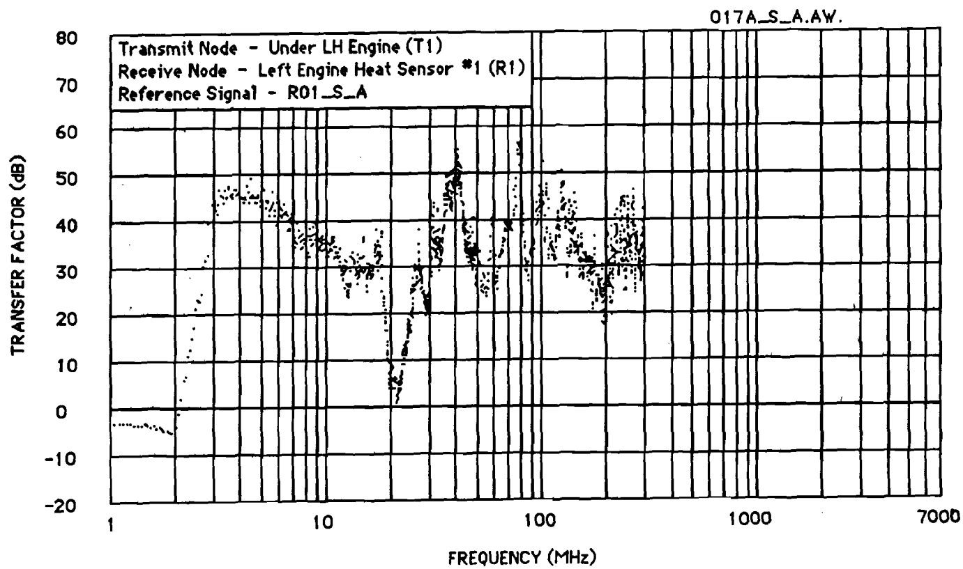
Figure E-7 Probe Transfer Factor (Test 017A)
