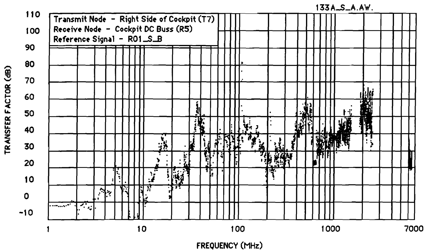
Figure E-18 Probe Transfer Factor (Test 133A)
