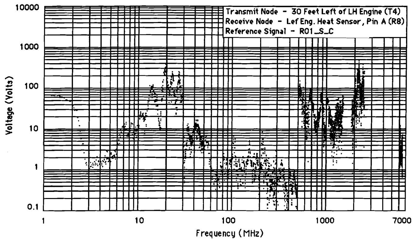
Figure F-10 Maximum Induced Voltage (095A)
