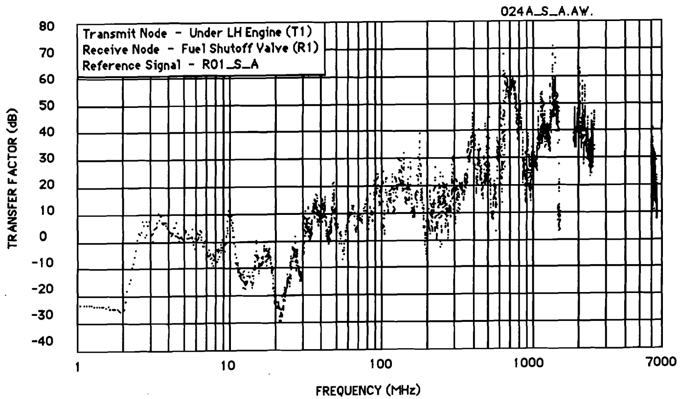
Figure E-9 Probe Transfer Factor (Test 024A)
