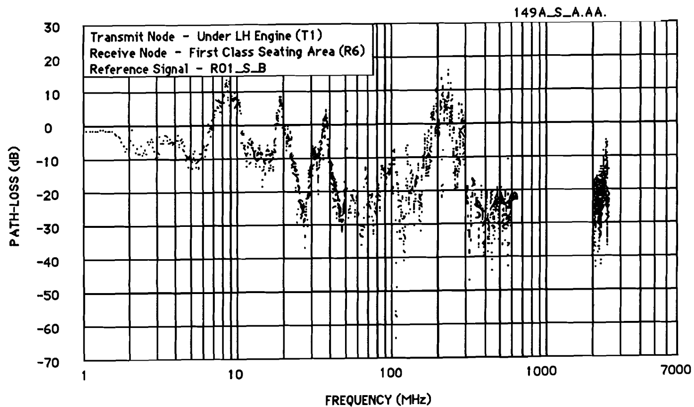
Figure E-29 Antenn Path-Loss Function (Test 149A)
