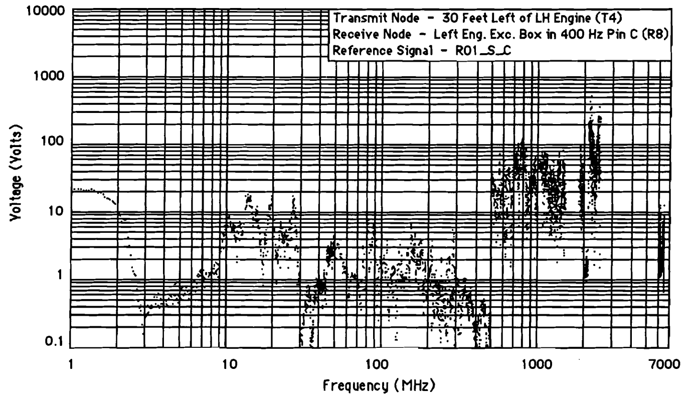
Figure F-8 Maximum Induced Voltage (093AA)
