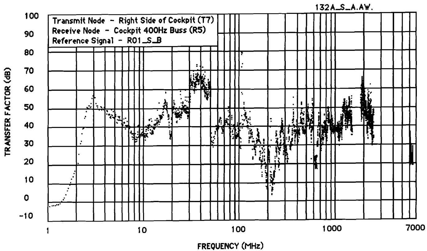
Figure E-17 Probe Transfer Factor (Test 132A)
