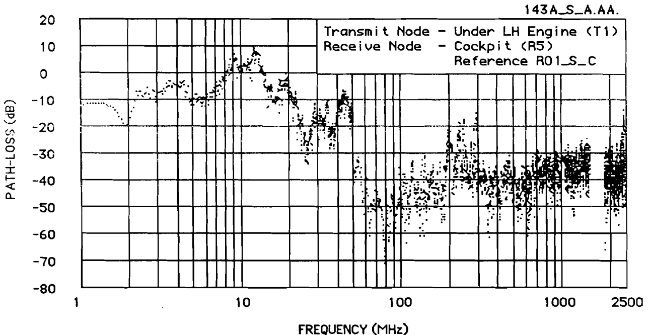
Figure 7.3.4 Antenna Path-Loss Function (Test 143A)
