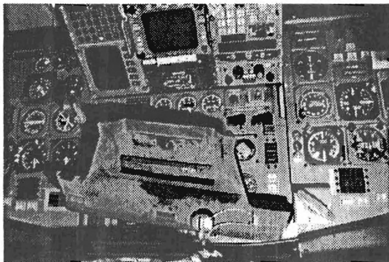
25. View showing panel to engine fire switches removed for access to wiring.
