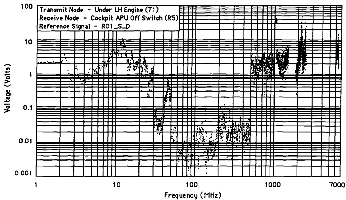
Figure F-18 Maximum Induced Voltage (144A)
