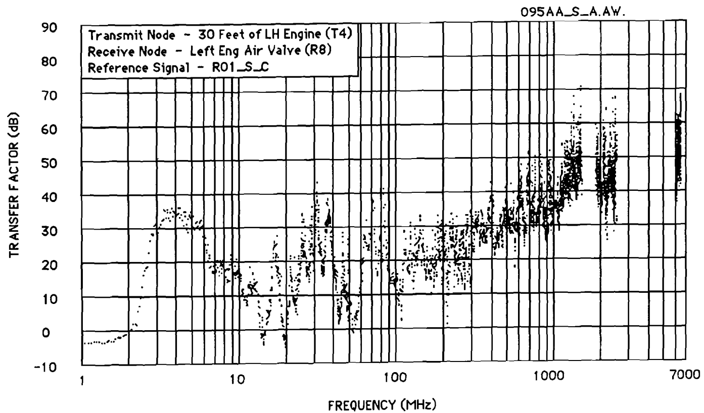
Figure E-14 Probe Transfer Factor (Test 095AA)
