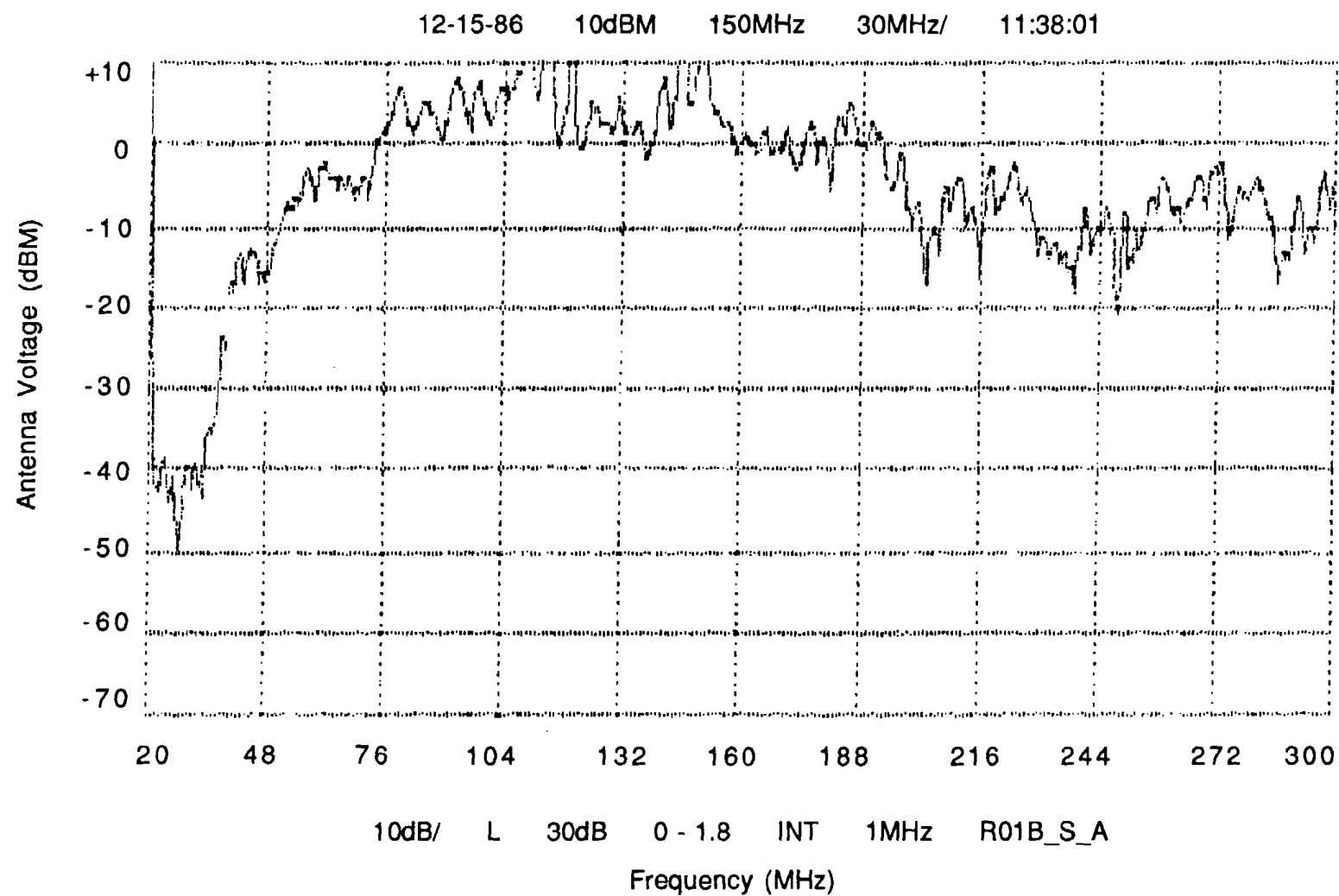
Figure 7.3.1 Typical Spectrum Analyzer Data (Test Sequence No.)
