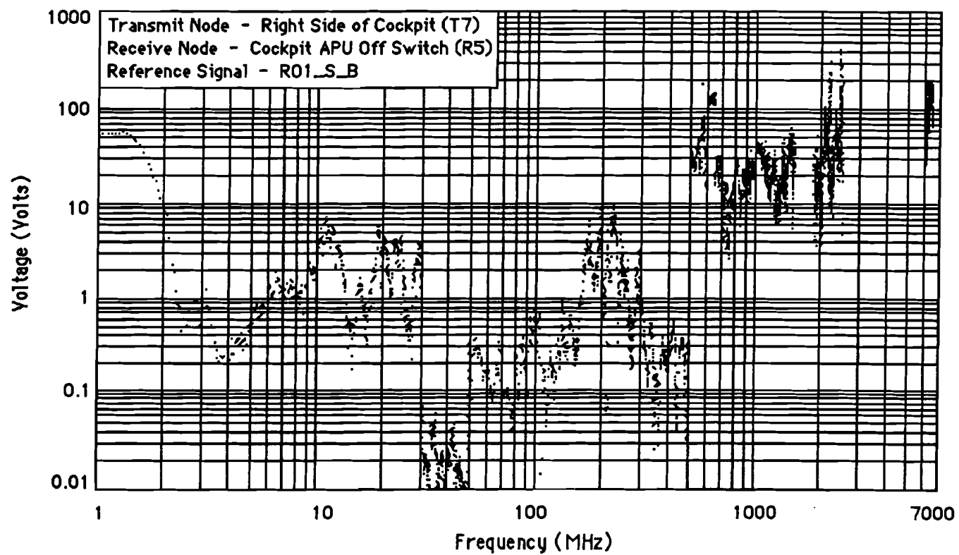
Figure F-16 Maximum Induced Voltage (138A)
