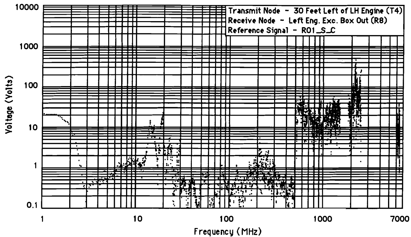
Figure F-9 Maximum Induced Voltage (094A)
