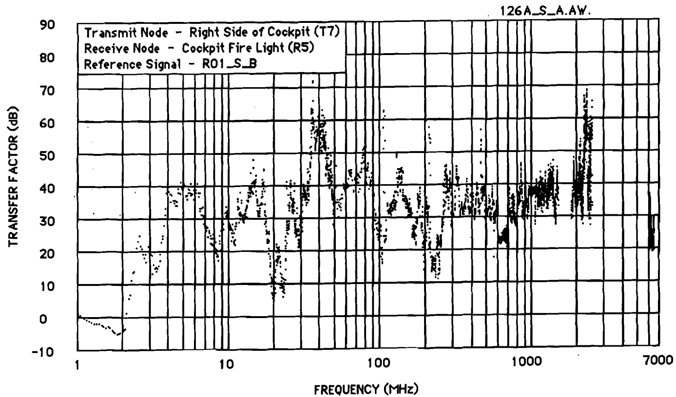
Figure E-15 Probe Transfer Factor (Test 126A)
