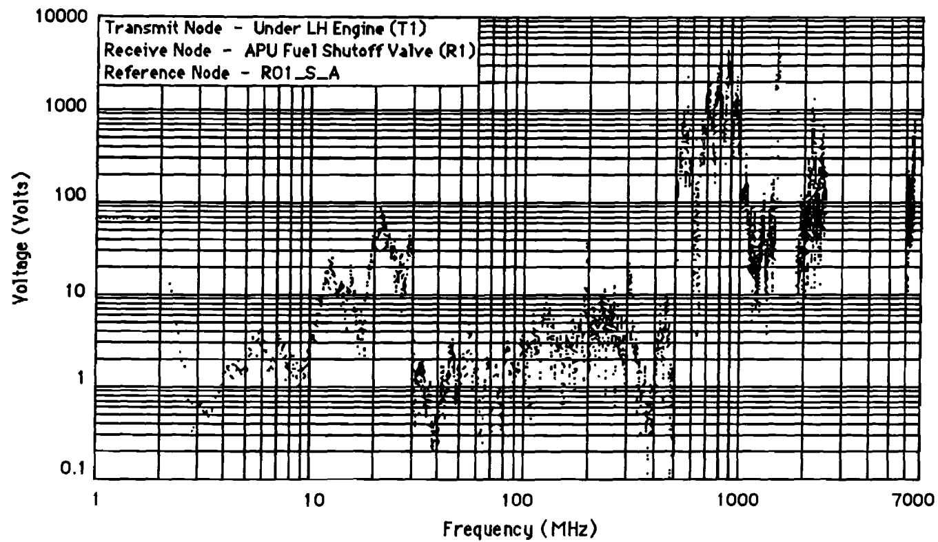
Figure F-5 Maximum Induced Voltage (022A)
