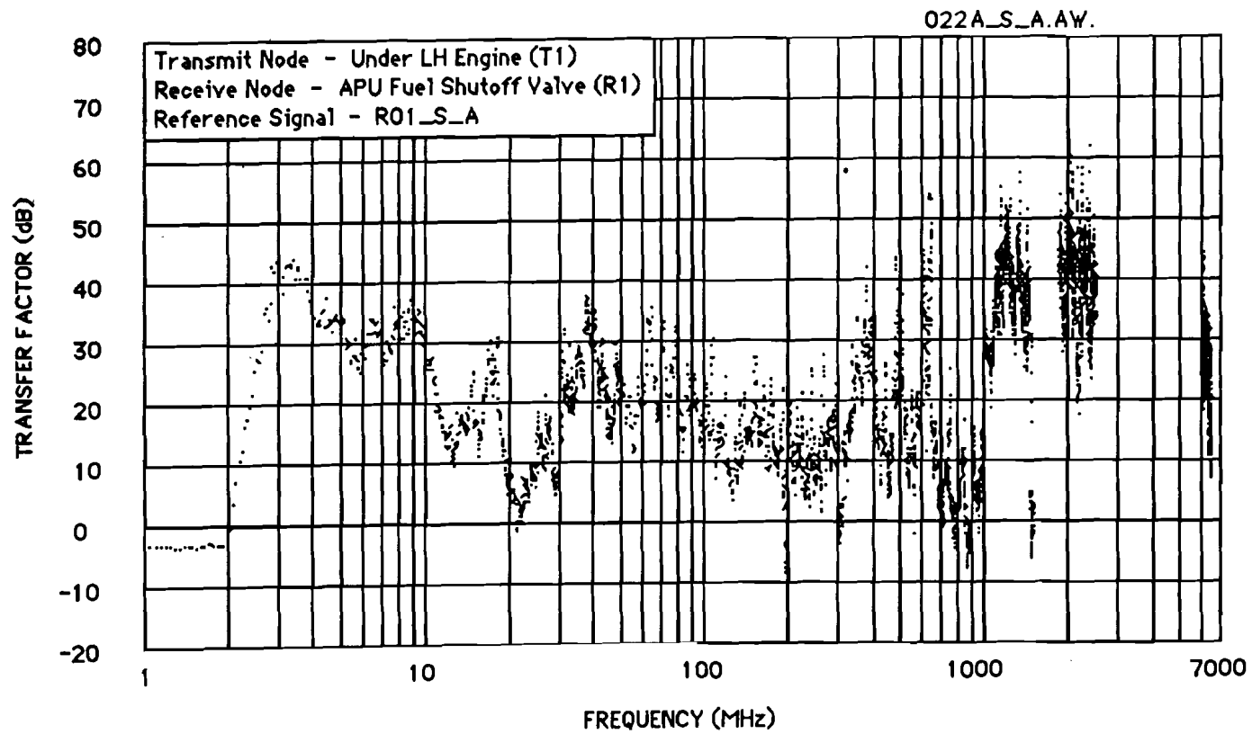
Figure E-8 Probe Transfer Factor (Test 022A)
