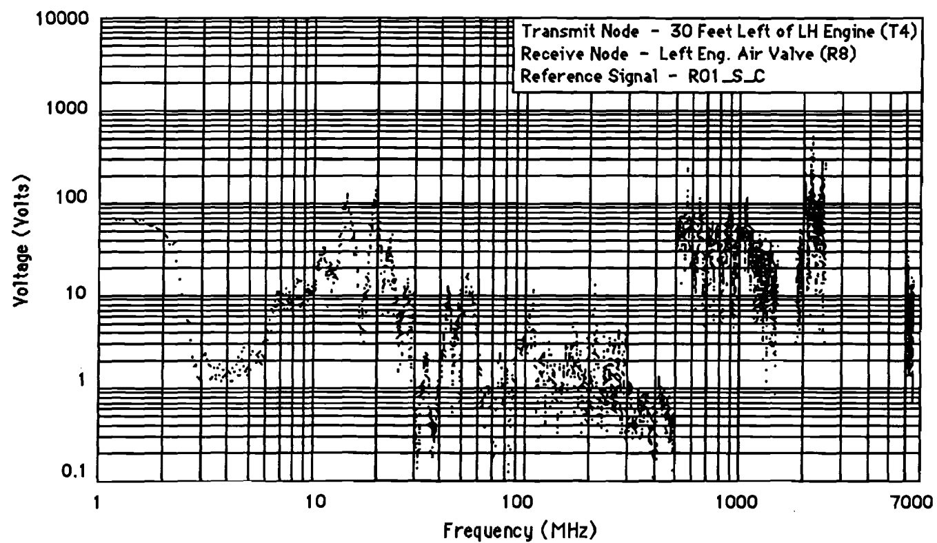
Figure F-11 Maximum Induced Voltage (095AA)
