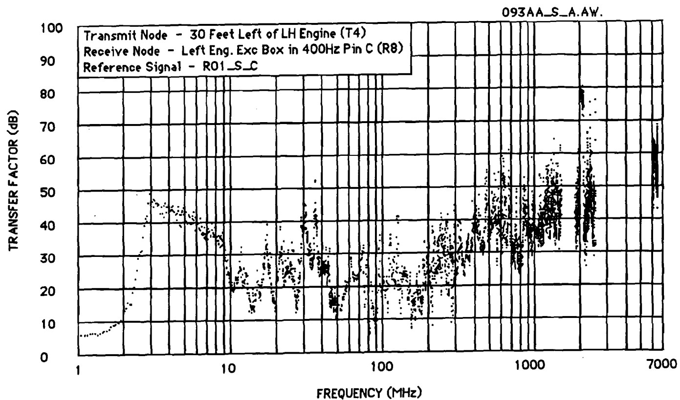
Figure E-11 Probe Transfer Factor (Test 093AA)
