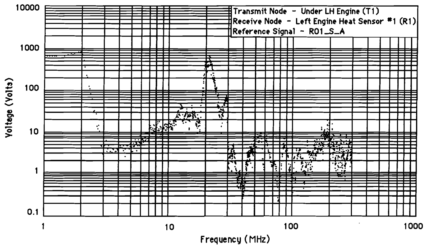
Figure F-4 Maximum Induced Voltage (017A)
