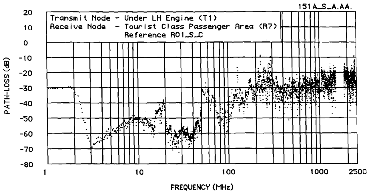
Figure 7.3.8 Antenna Path-Loss Function (Test 151A)
