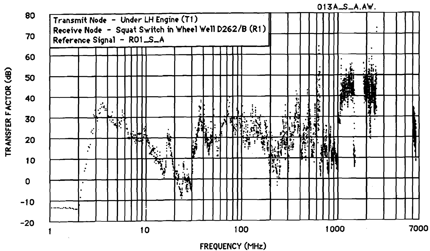
Figure E-6 Probe Transfer Factor (Test 013A)
