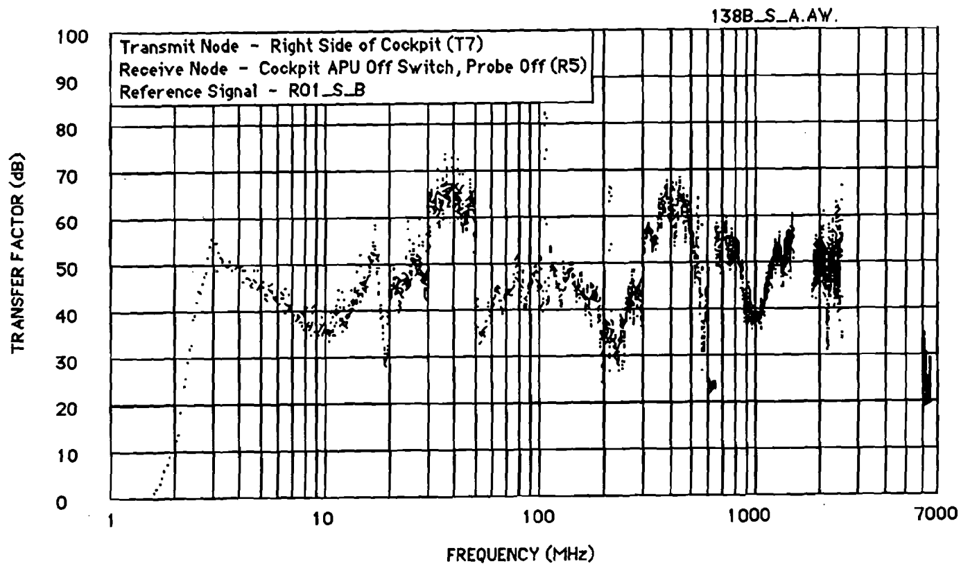
Figure E-20 Probe Transfer Factor (Test 138B)
