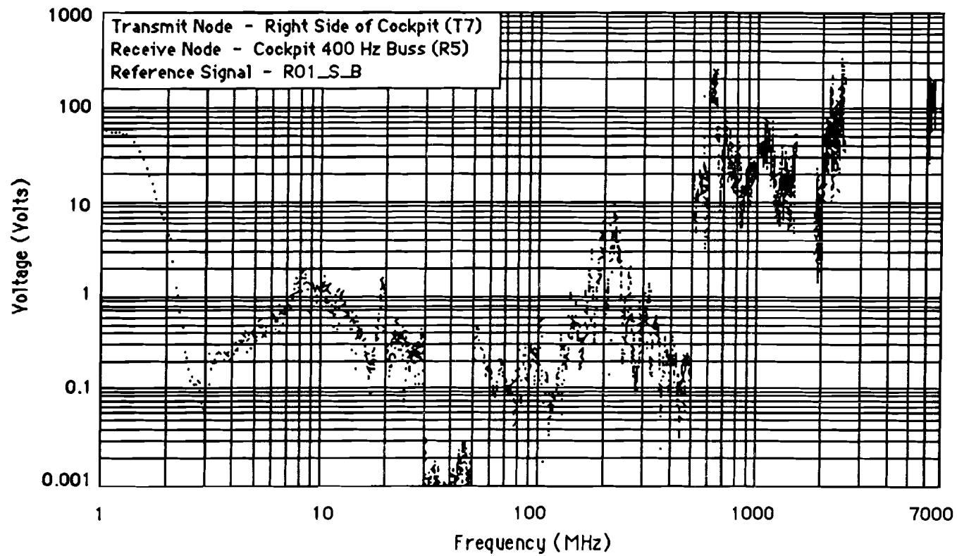
Figure F-14 Maximum Induced Voltage (132A)
