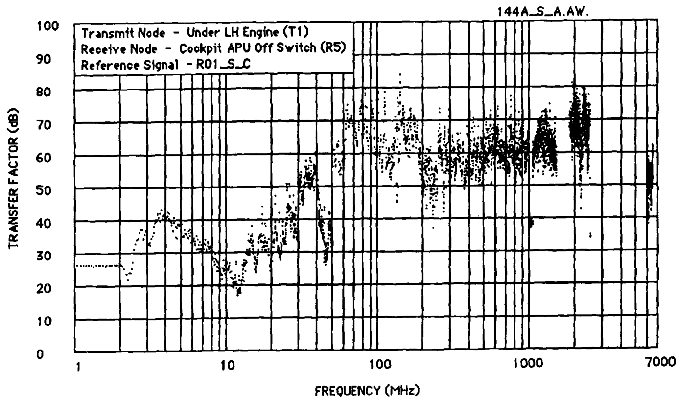
Figure E-21 Probe Transfer Factor (Test 144A)
