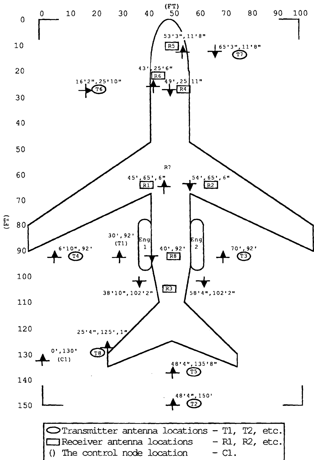
Figure 6.1.1. Measurement Locations in Graphical Form.
