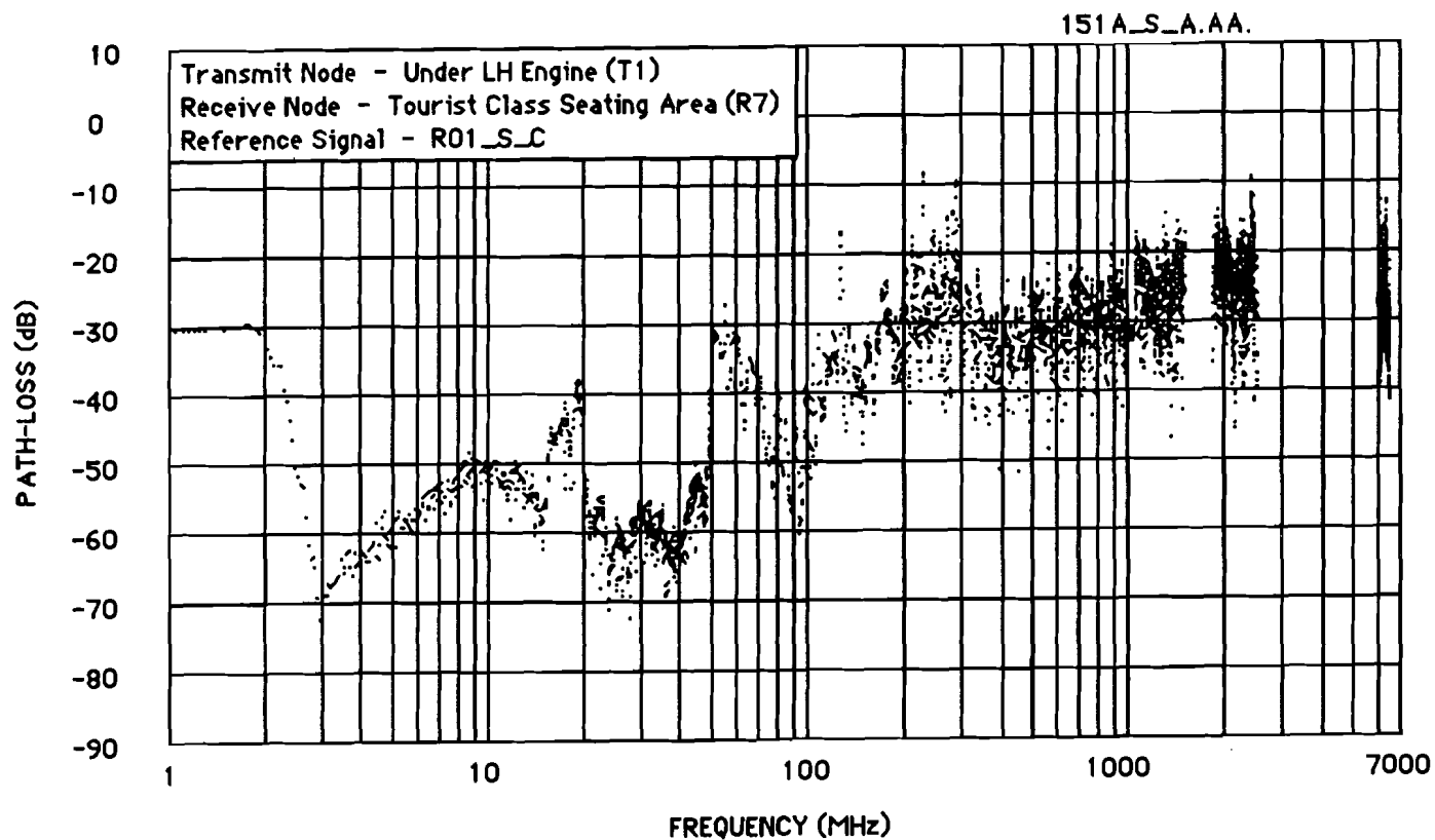
Figure E-31 Antenn Path-Loss Function (Test 151A)
