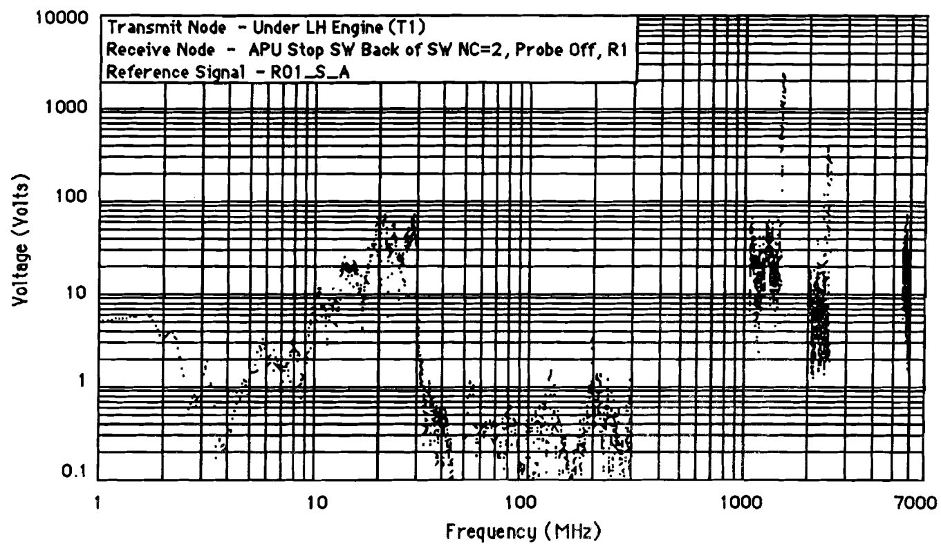
Figure F-2 Maximum Induced Voltage (002B)
