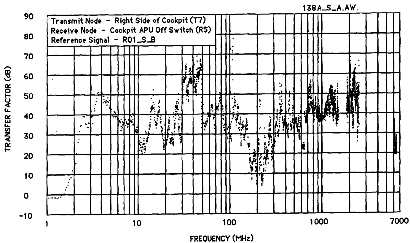
Figure E-19 Probe Transfer Factor (Test 138A)
