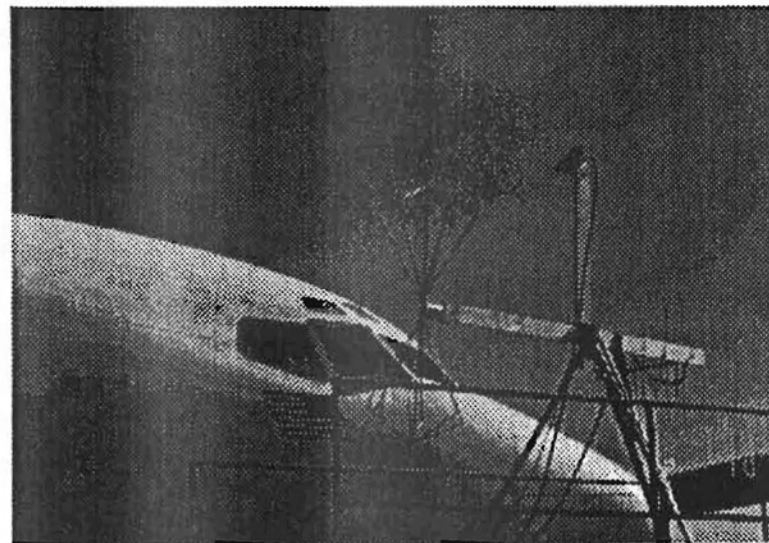
12. Transmit antennas at right side of cockpit (location T7).
