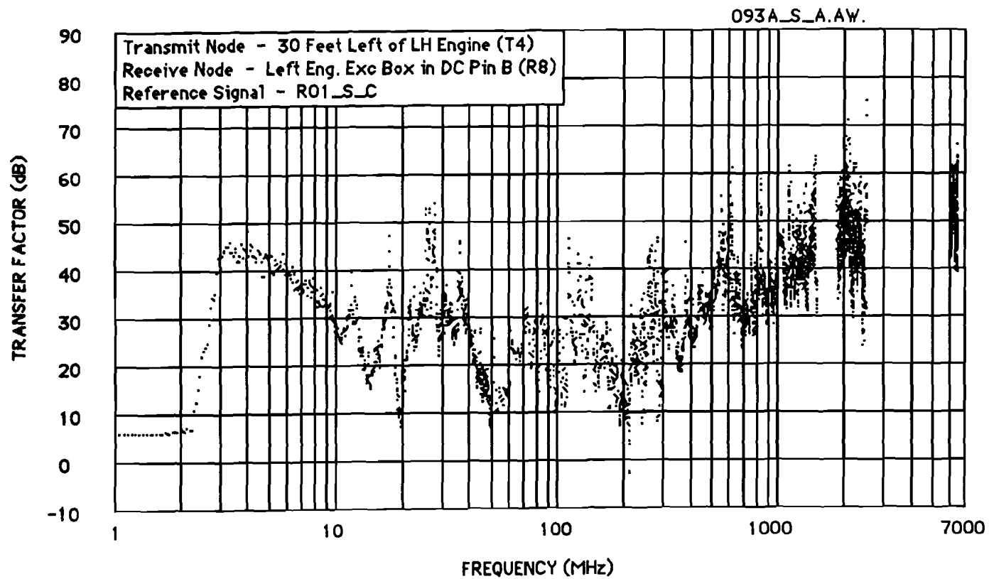
Figure E-10 Probe Transfer Factor (Test 093A)
