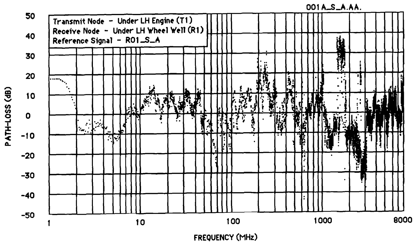
Figure E-24 Antenn Path-Loss Function (Test 001A)
