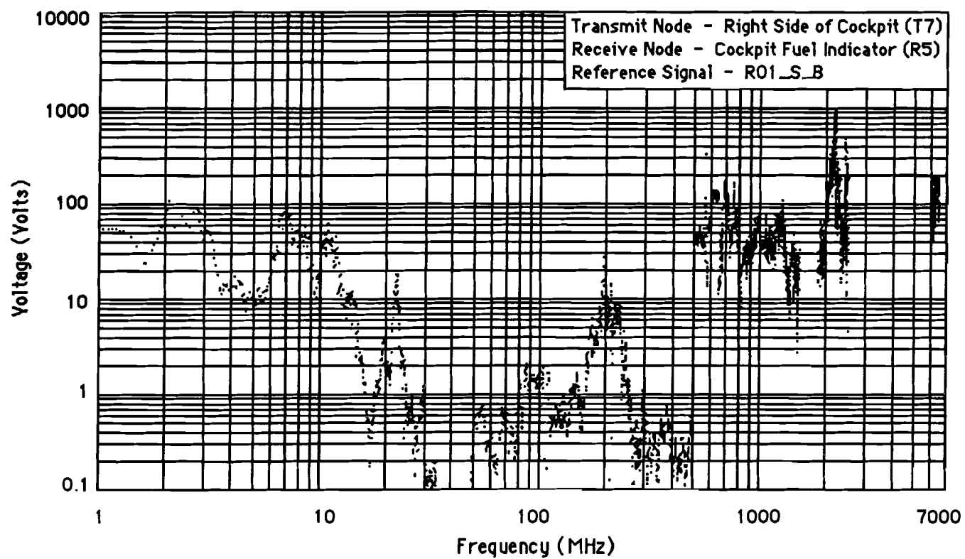
Figure F-13 Maximum Induced Voltage (128A)
