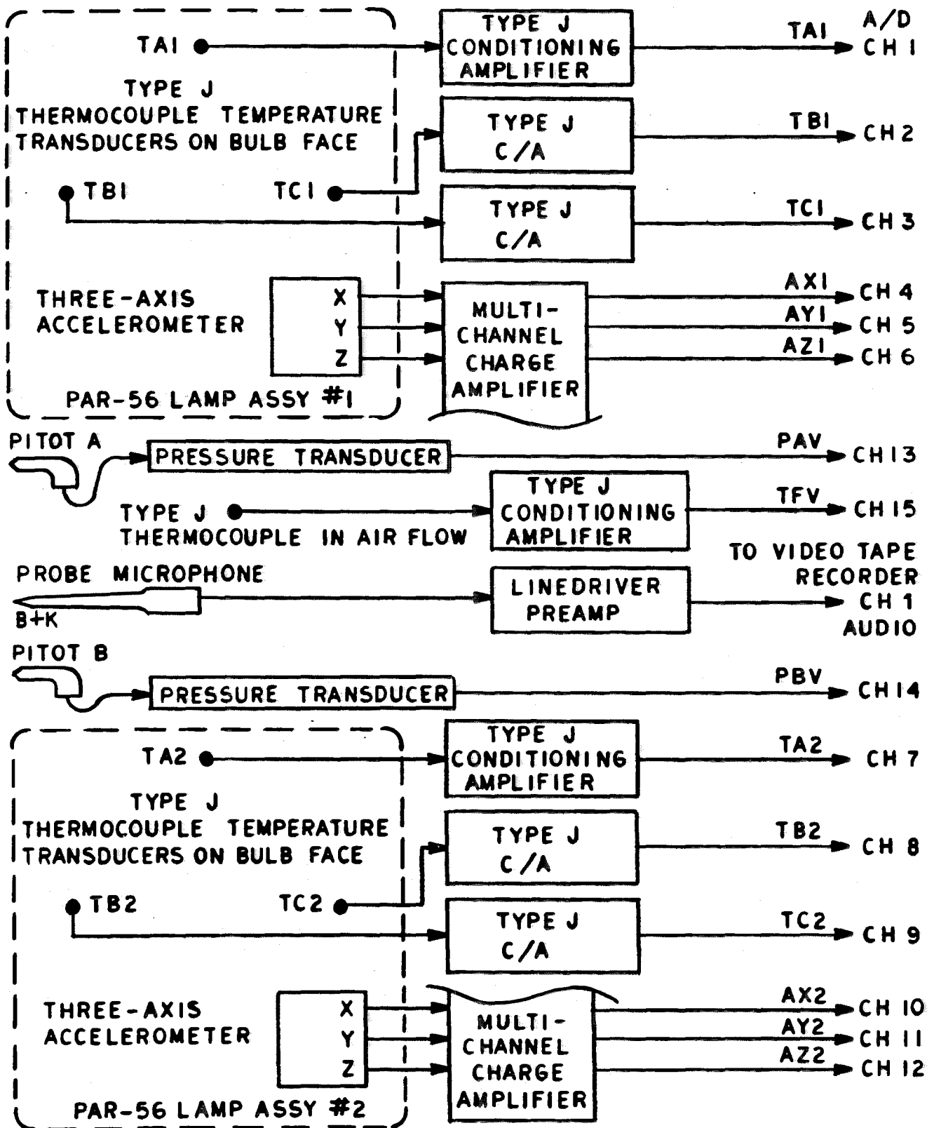
FIGURE 3. SENSOR ARRAY
