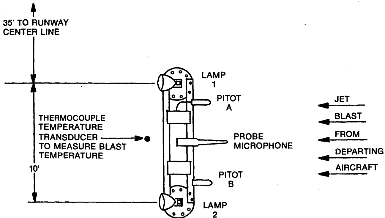
TOP VIEW OF SENSOR ARRAY
