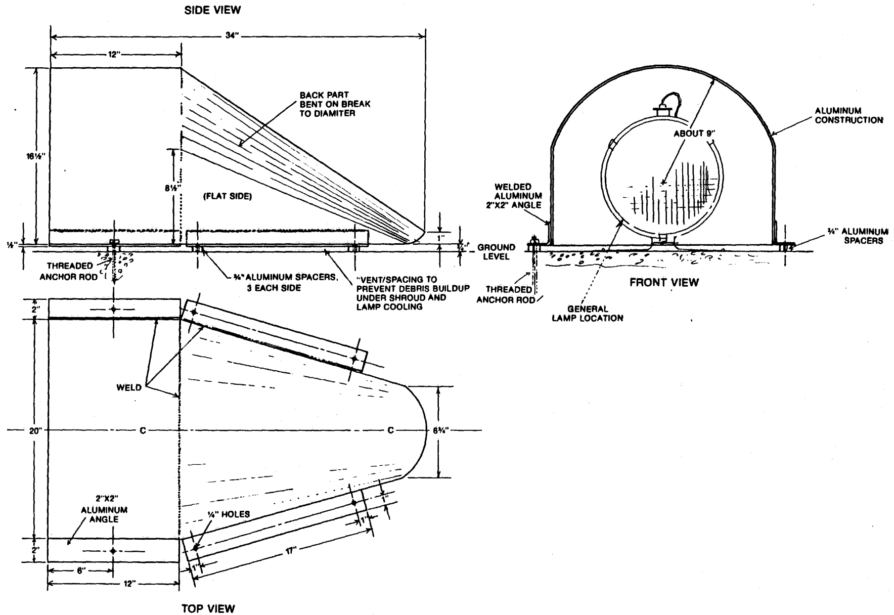
FIGURE 12. EXPERIMENTAL SHROUD ASSEMBLY
