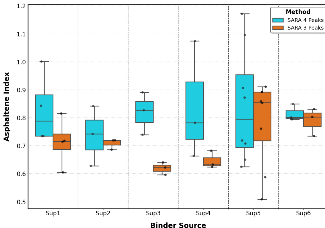
Figure 14. AI plots for PG 67-22 asphalt binders
