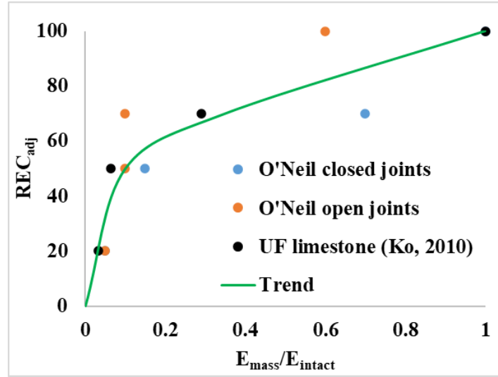
Figure 3-5 Adjusted REC versus E_{mass}/E_{intact} .
