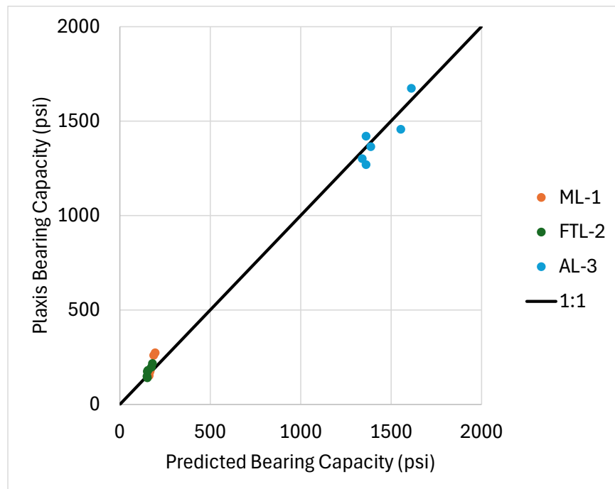
Figure 5-24 PLAXIS versus predicted bearing capacity for eccentric cases in Table 28.
