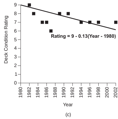
Figure 1 - Example of Trend Line for Deck Condition Ratings
