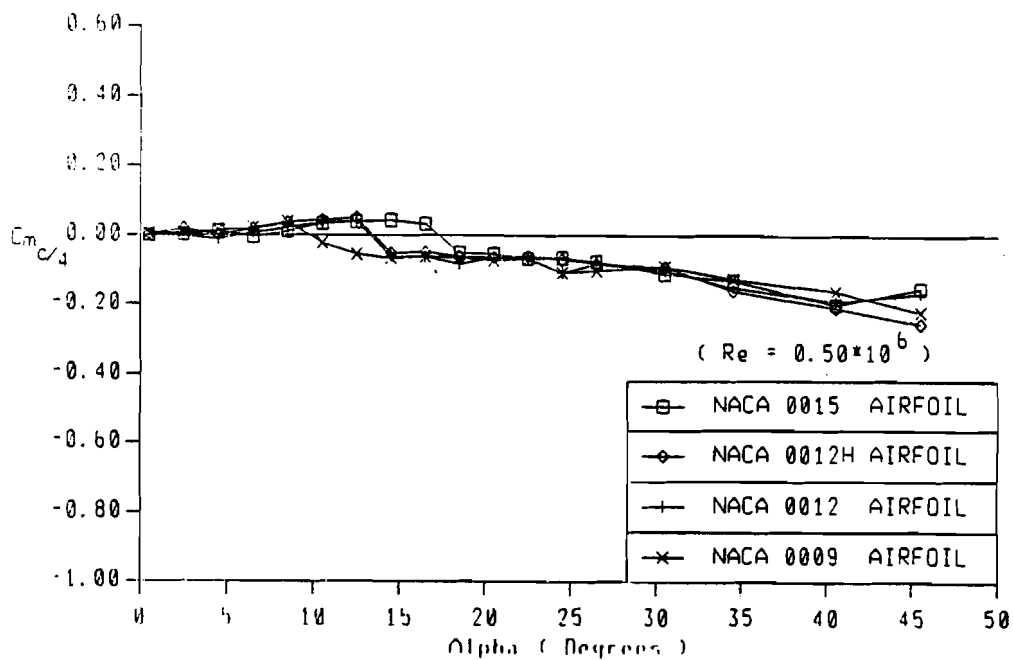
Figure 10. (c) Moment coefficients of NACA 00-series airfoils
