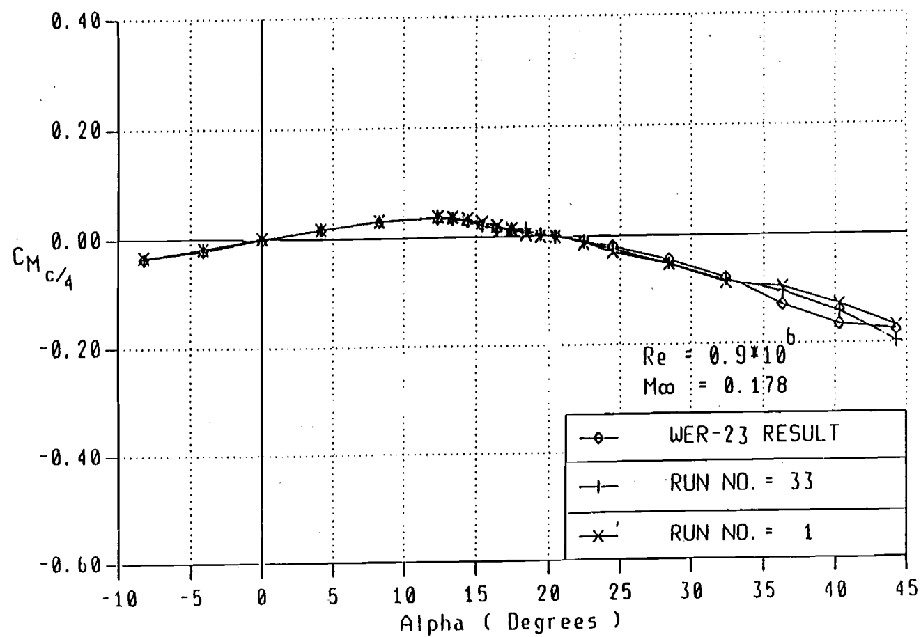
Figure 5. Wing Moment Coefficient for Three Tests
