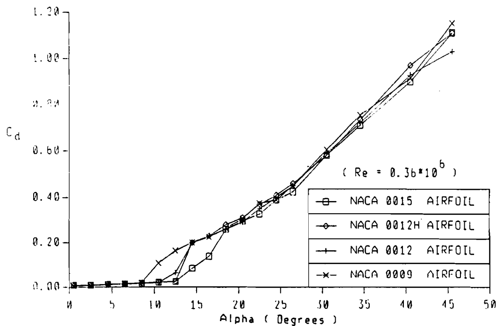
Figure 9. (b) Drag coefficients of NACA 00-series airfoils
