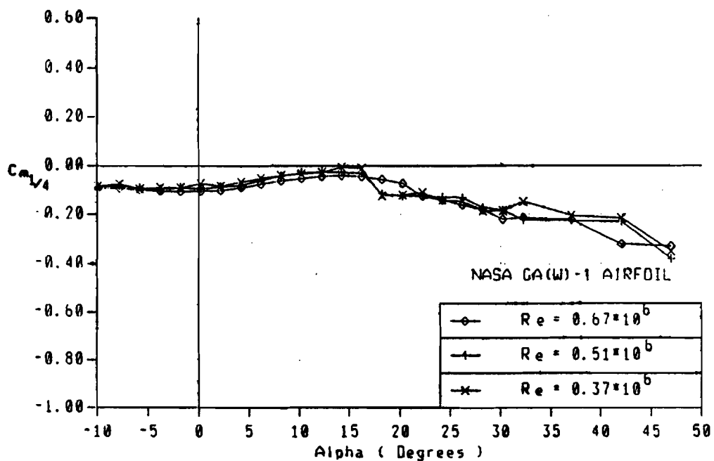
Figure 19. (c) Moment coefficients of NASA GA(W)-1 airfoil
