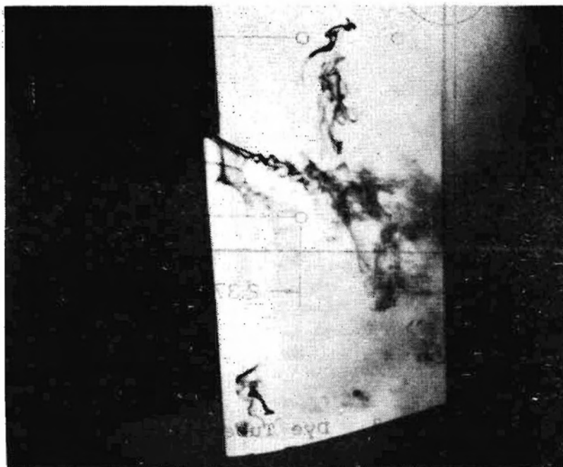
FIGURE 5. DLEE from 70 TO 100 Percent of Semi-Span. \alpha = 20^\circ
