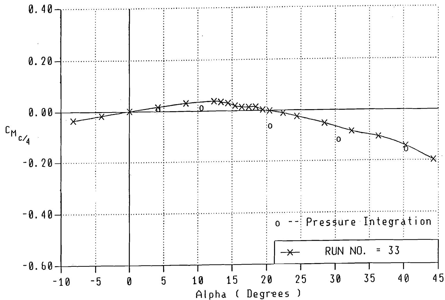
Figure 8. Wing Moment Coefficient By Balance and Integration of Surface Pressure
