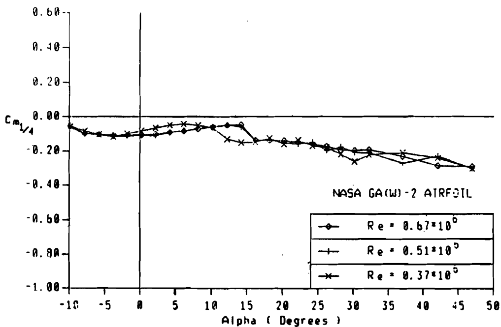
Figure 20. (c) Moment coefficients of NASA GA(W)-2 airfoil
