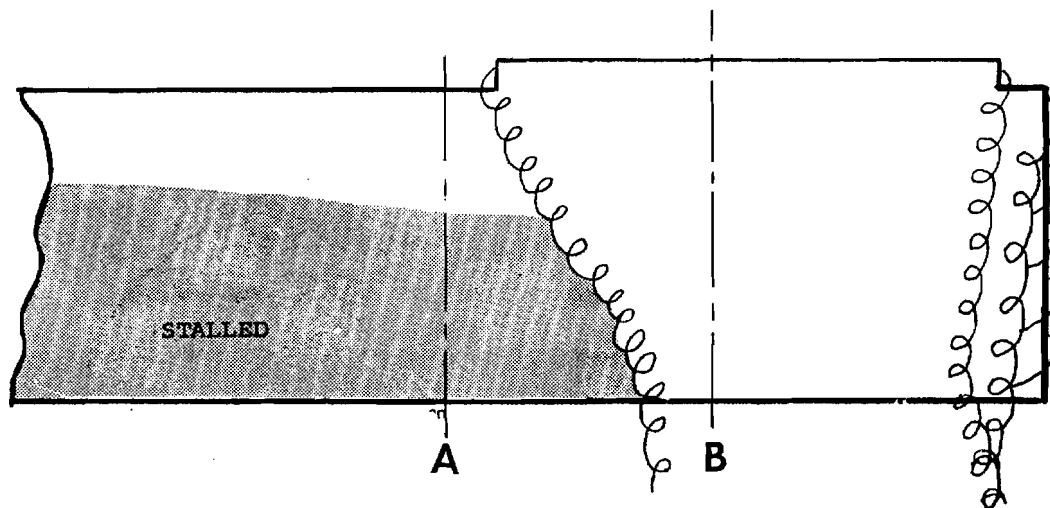
a. Wing with DLEE at Angle of Attack Producing Stalled Inboard Sections.
