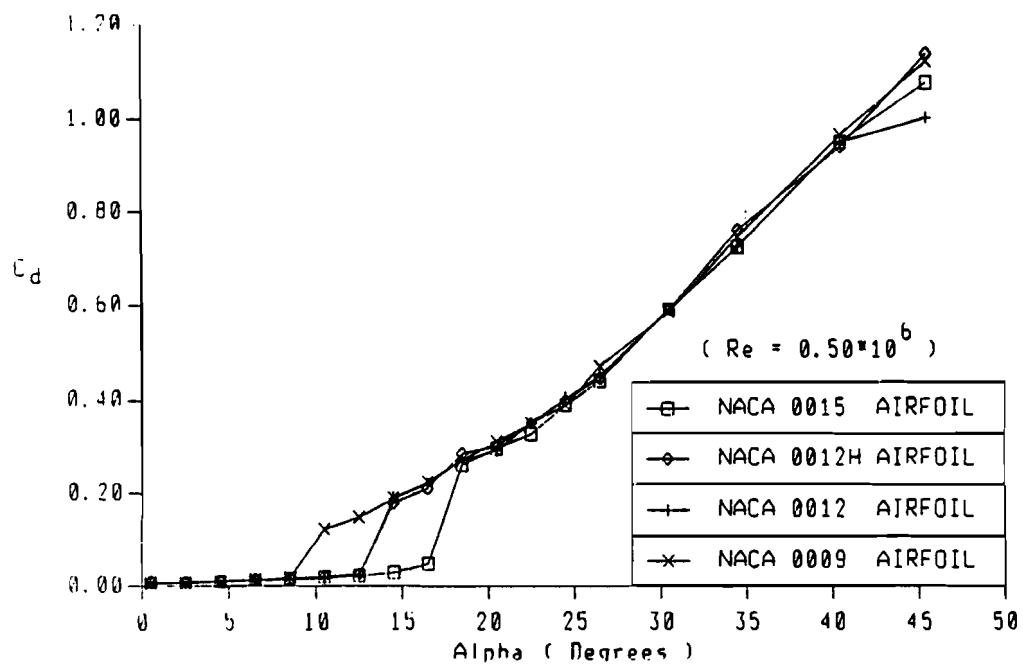
Figure 10. (b) Drag coefficients of NACA 00-series airfoils
