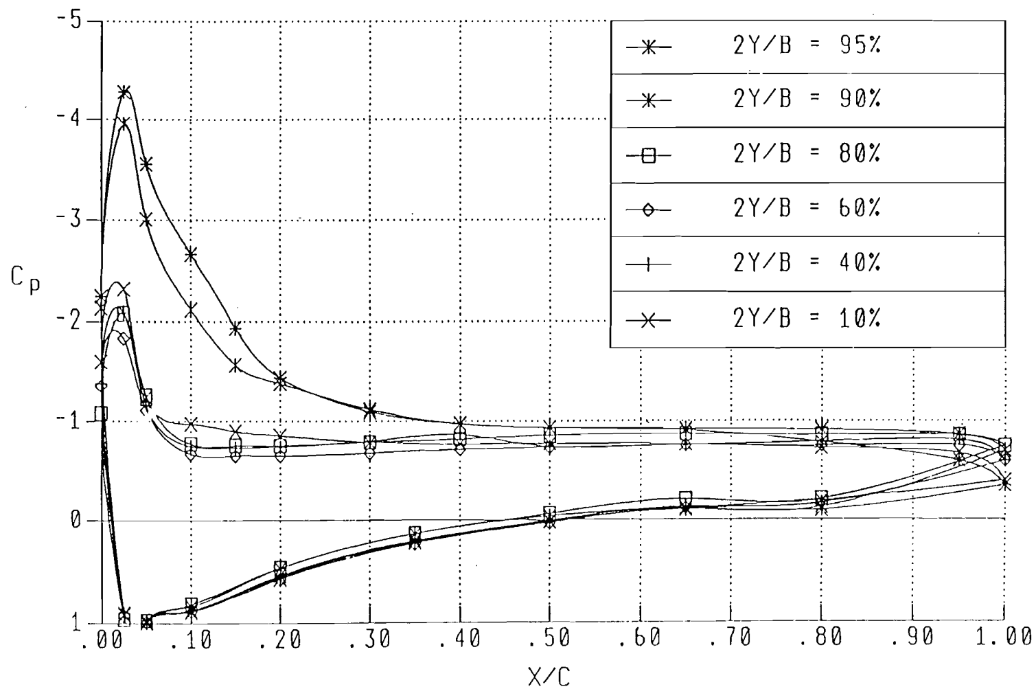
Figure 7. Wing Sections Pressure Distribution \alpha = 30^\circ
