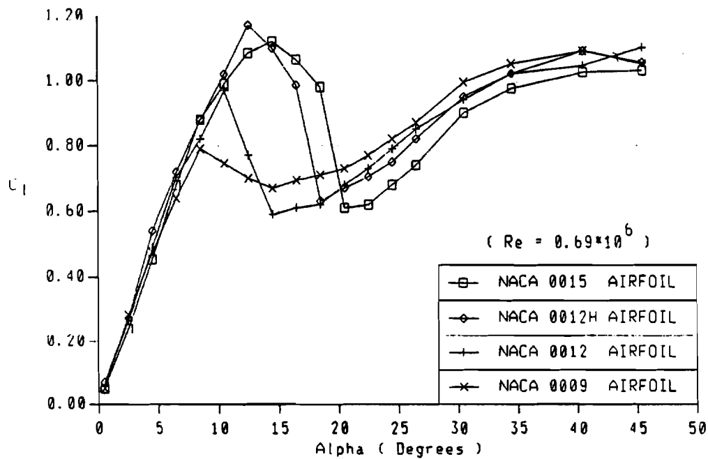
Figure 11. (a) Lift coefficients of NACA 00-series airfoils
