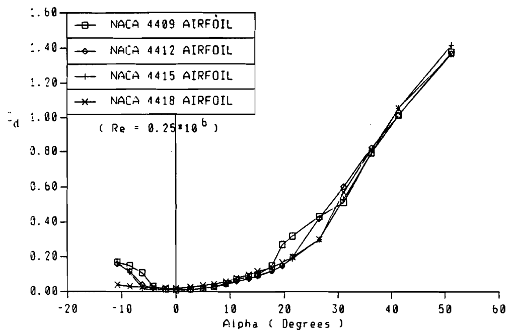
Figure 16. (b) Drag coefficients of NACA 44-series airfoils
