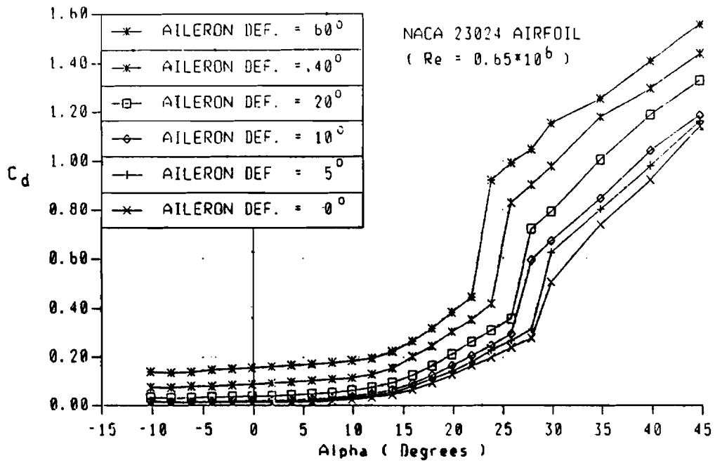
Figure 21. (b) Drag coefficients of NACA 23024 airfoil
