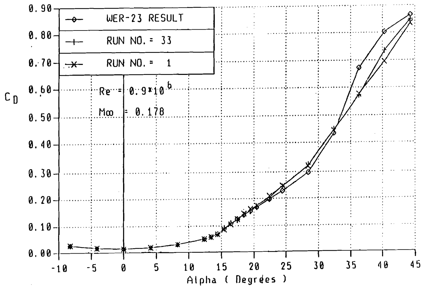
Figure 4. Wing Drag Coefficient for Three Tests
