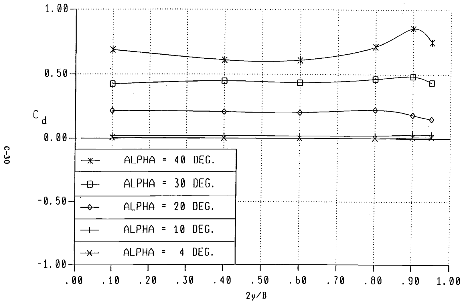
Figure 15. Drag Distribution in Spanwise Direction
