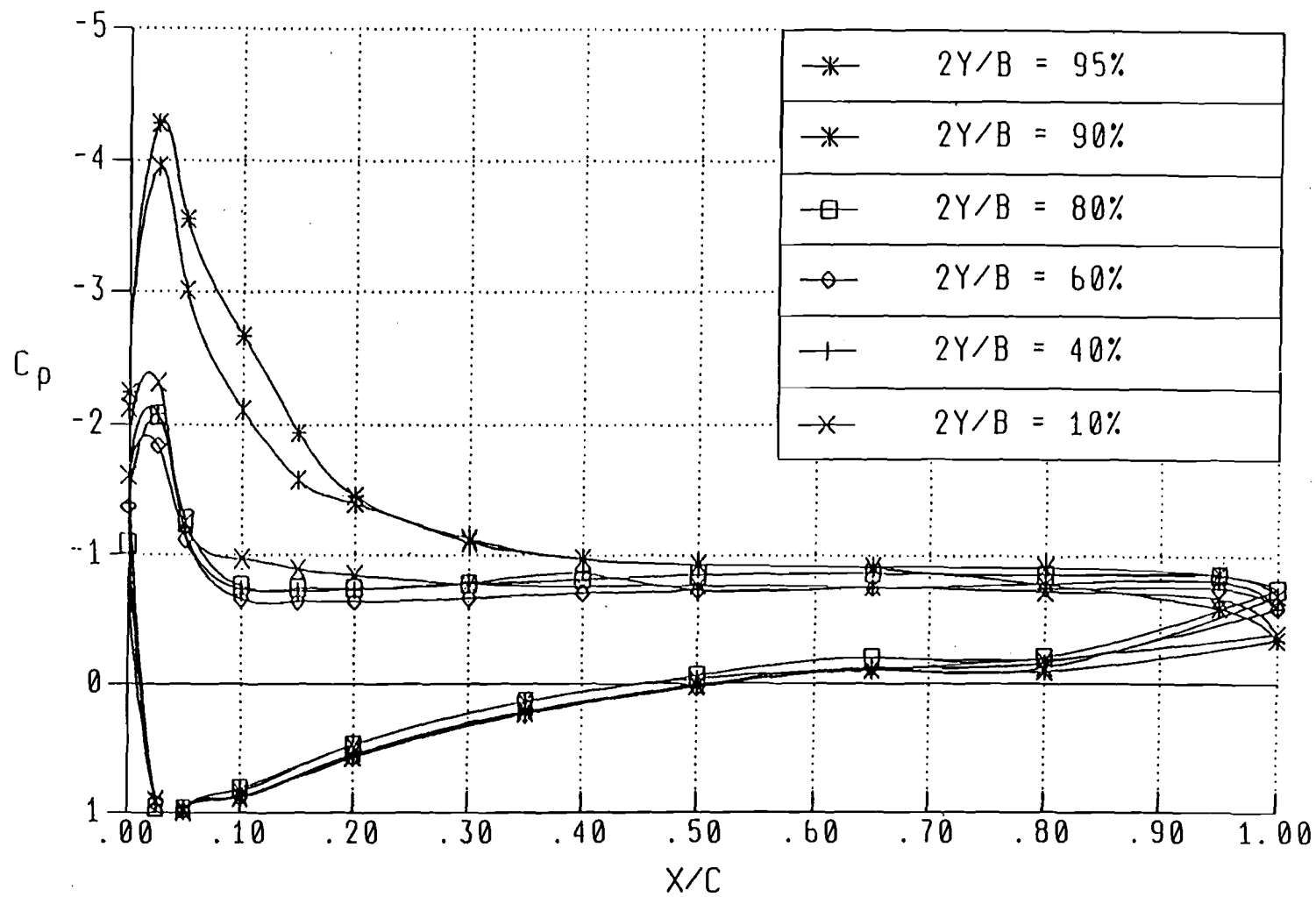
Figure 12. Wing Sections Pressure Distribution \alpha = 30^\circ
