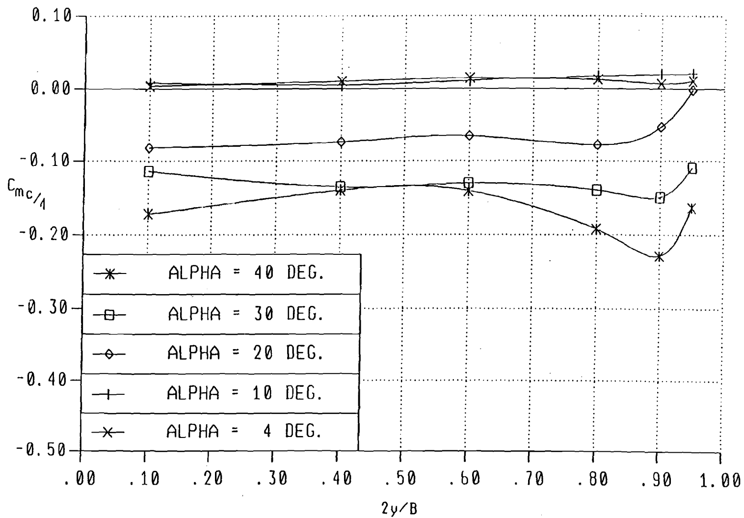
Figure 16. Moment Distribution in Spanwise Direction
