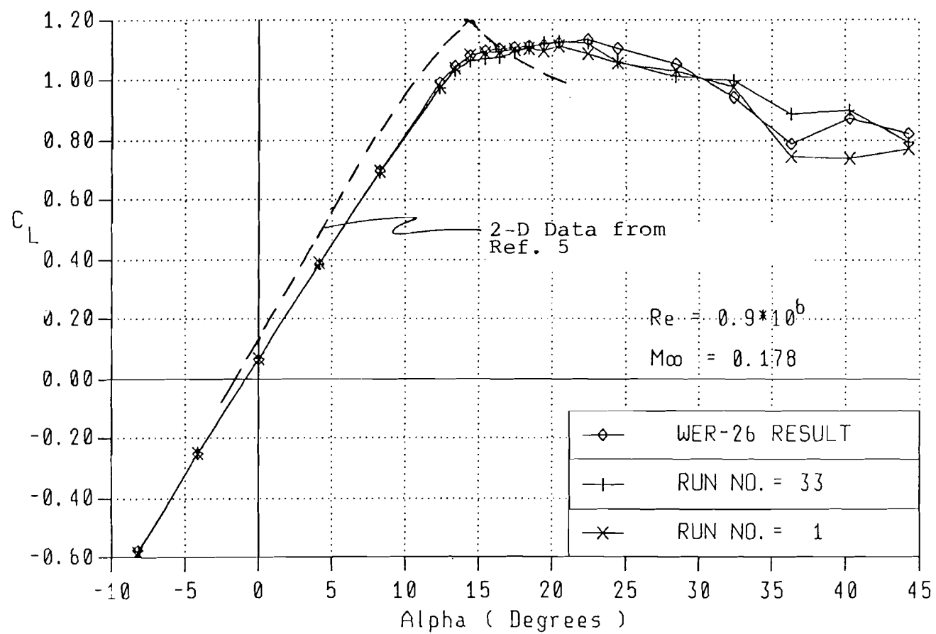
Figure 3. Lift Coefficient, 2-D Compared to 3-D (A.R.=13.3)
