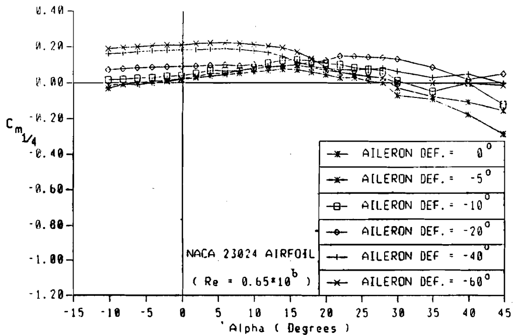
Figure 22. (c) Moment coefficients of NACA 23024 airfoil
