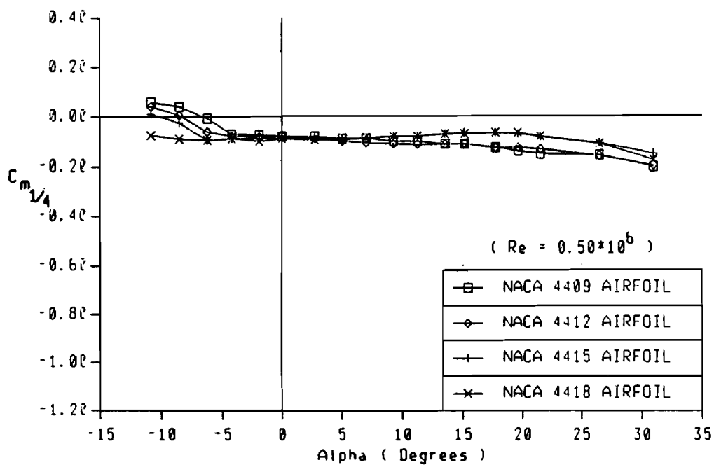
Figure 17. (c) Moment coefficients of NACA 44-series airfoils
