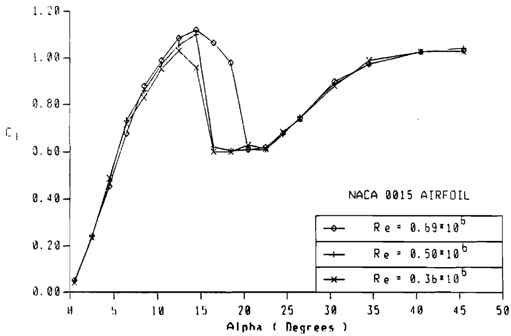
Figure 8. (a) Lift coefficients of NACA 0015 airfoil
