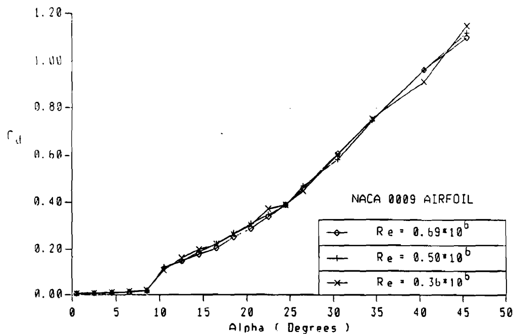
Figure 5. (b) Drag coefficients of NACA 0009 airfoil
