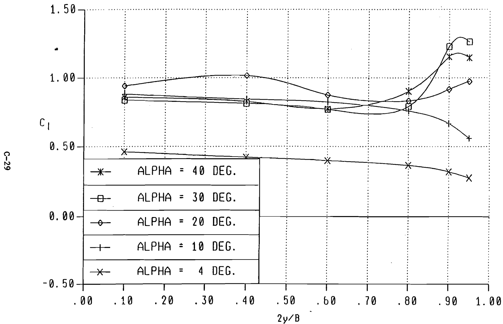
Figure 14. Lift Distribution in Spanwise Direction
