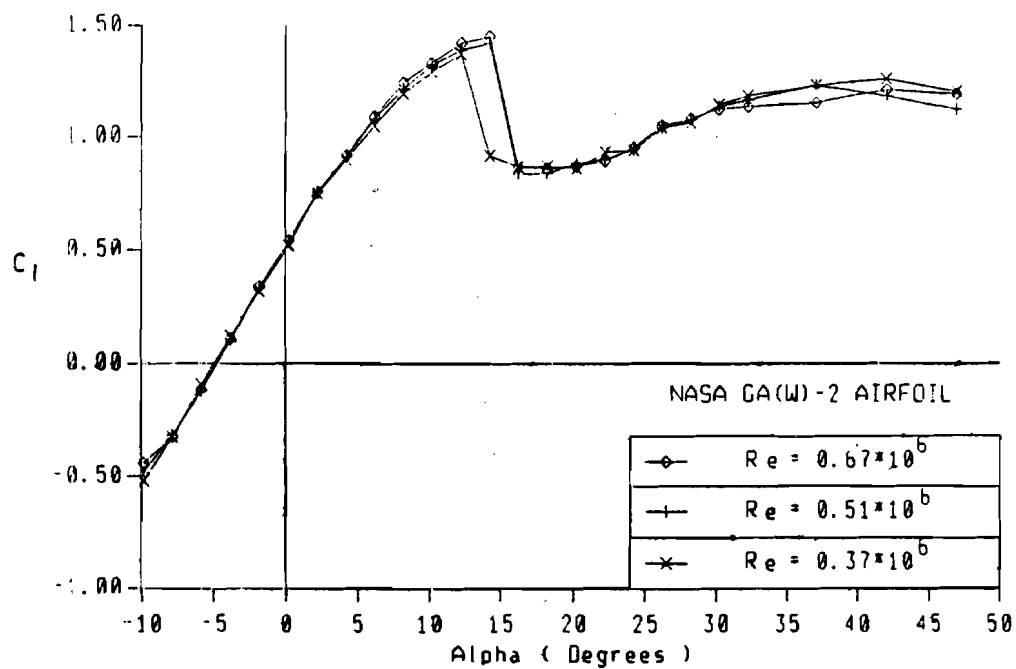
Figure 20. (a) Lift coefficients of NASA GA(W)-2 airfoil
