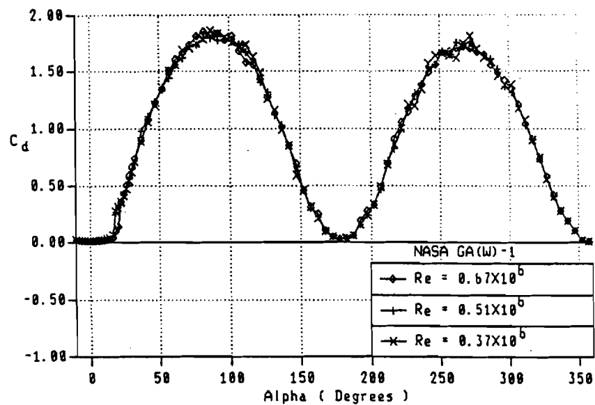
Figure 2. (b) Drag coefficients of NASA GA(W)-1 airfoil
