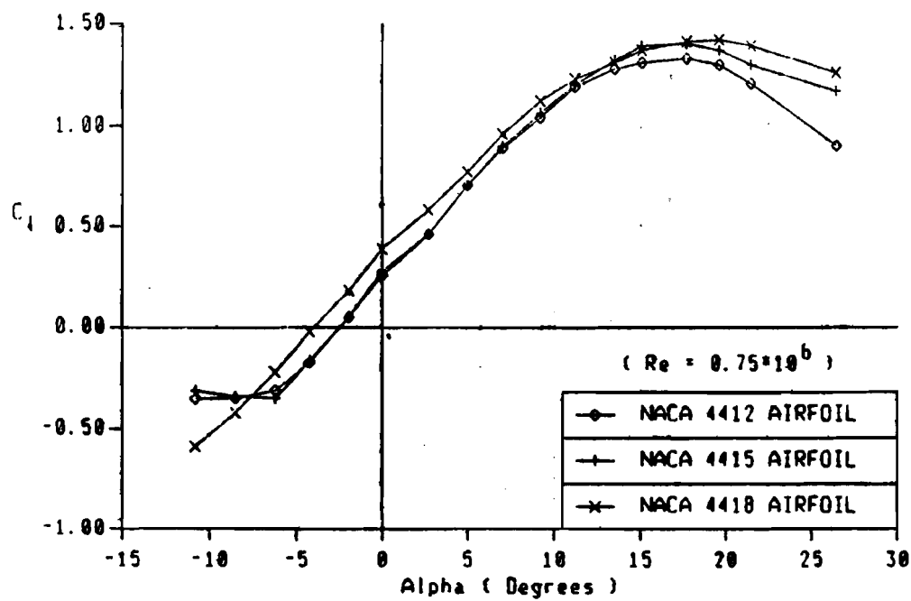
Figure 19. (a) Lift coefficients of NACA 44-series airfoils
