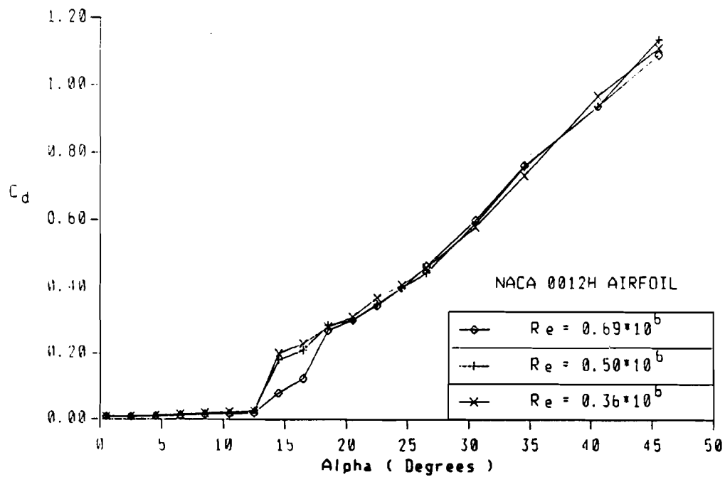
Figure 7. (b) Drag coefficients of NACA 0012H airfoil
