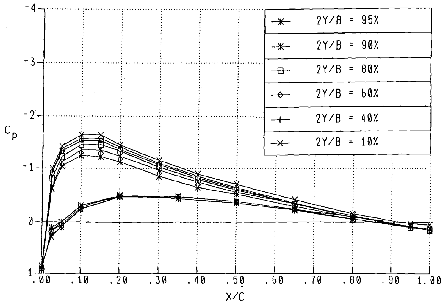
Figure 9. Wing Sections Pressure Distribution \alpha = 4^\circ
