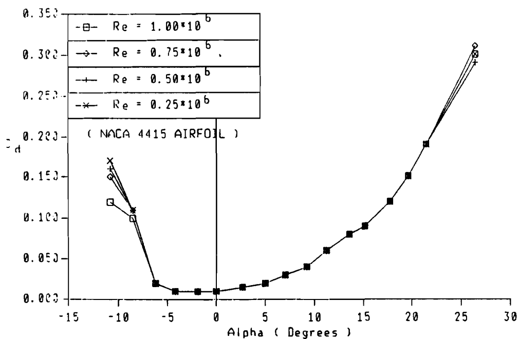
Figure 14. (b) Drag coefficients of NACA 4415 airfoil
