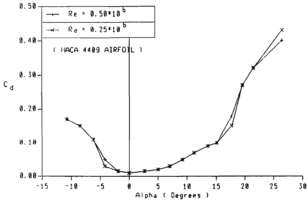
Figure 12. (b) Drag coefficients of NACA 4409 airfoil
