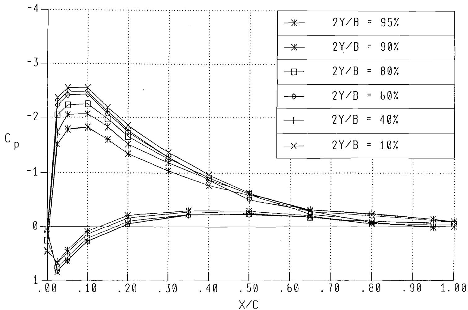
Figure 5. Wing Sections Pressure Distribution \alpha = 10^\circ
