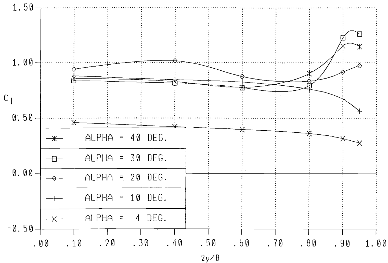
Figure 4. Lift Distribution in Spanwise Direction
