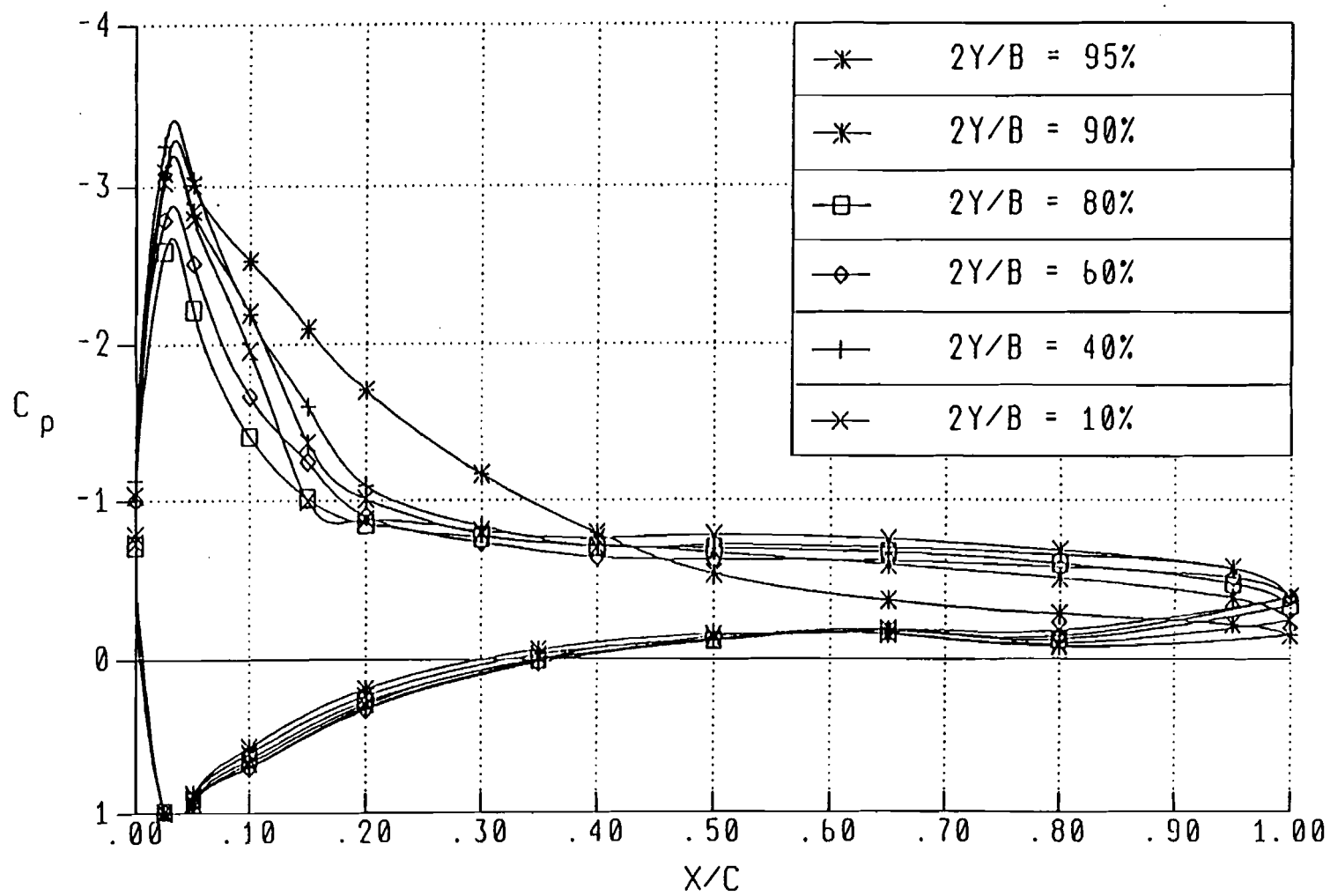
Figure 11. Wing Sections Pressure Distribution \alpha=20^\circ
