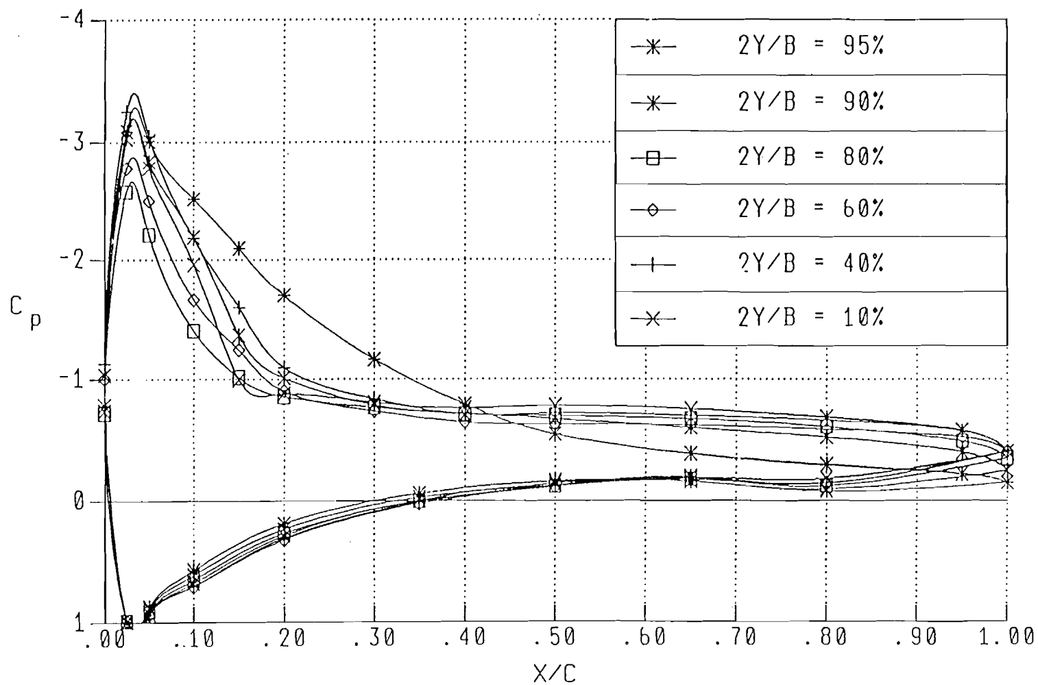
Figure 6. Wing Sections Pressure Distribution \alpha = 20^\circ
