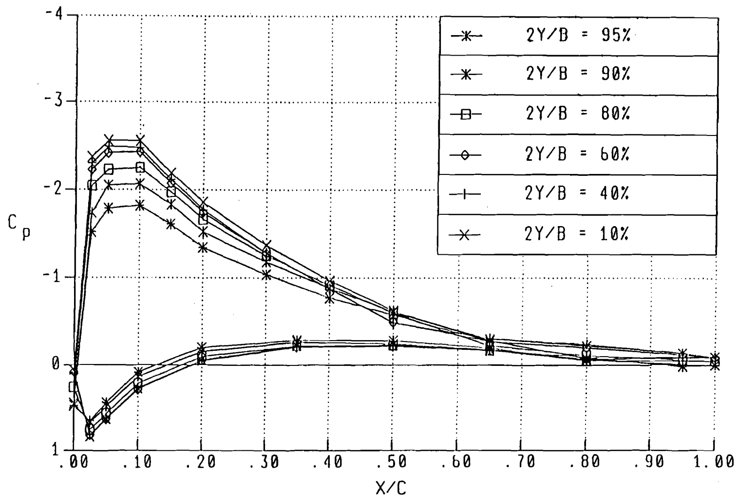
Figure 10. Wing Sections Pressure Distribution \alpha = 10^\circ
