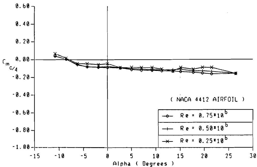
Figure 13. (c) Moment coefficients of NACA 4412 airfoil
