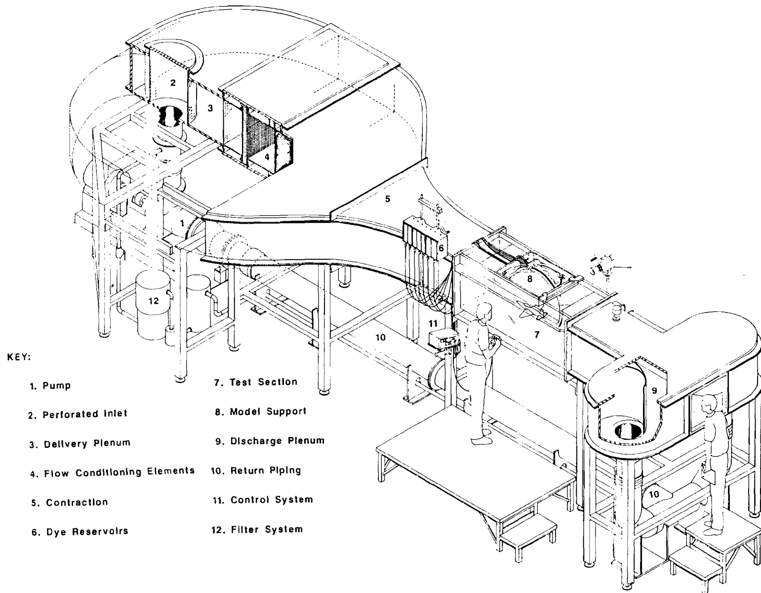
Figure 1a. FluidDyne Water Tunnel.
