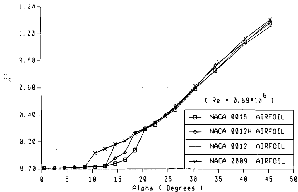
Figure 11. (b) Drag coefficients of NACA 00-series airfoils
