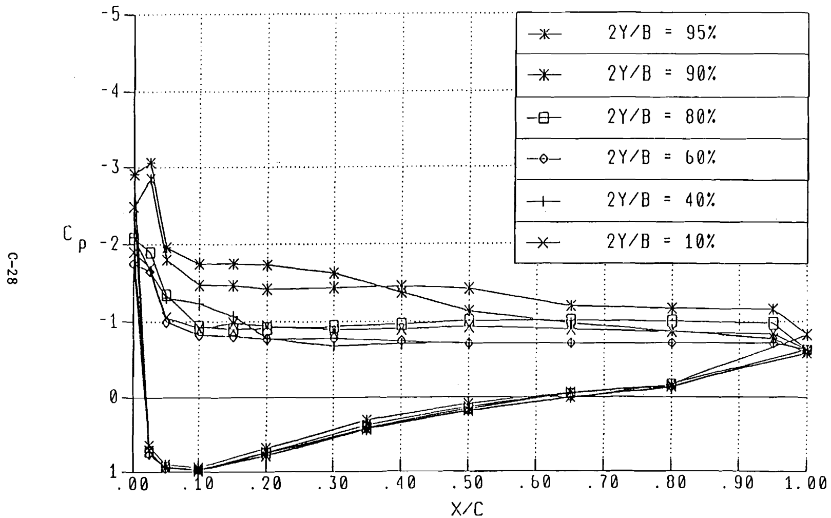
Figure 13. Wing Sections Pressure Distribution \alpha = 40^\circ
