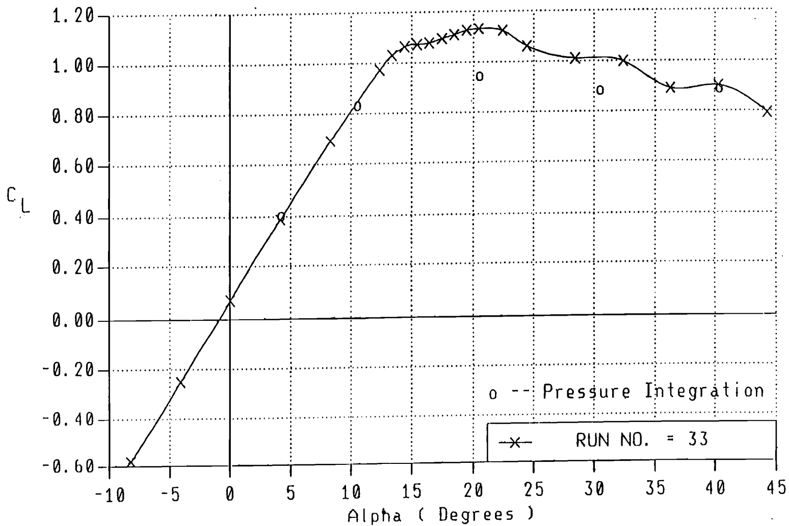
Figure 6. Wing Lift Coefficient By Balance and Integrattion of Surface Pressure
