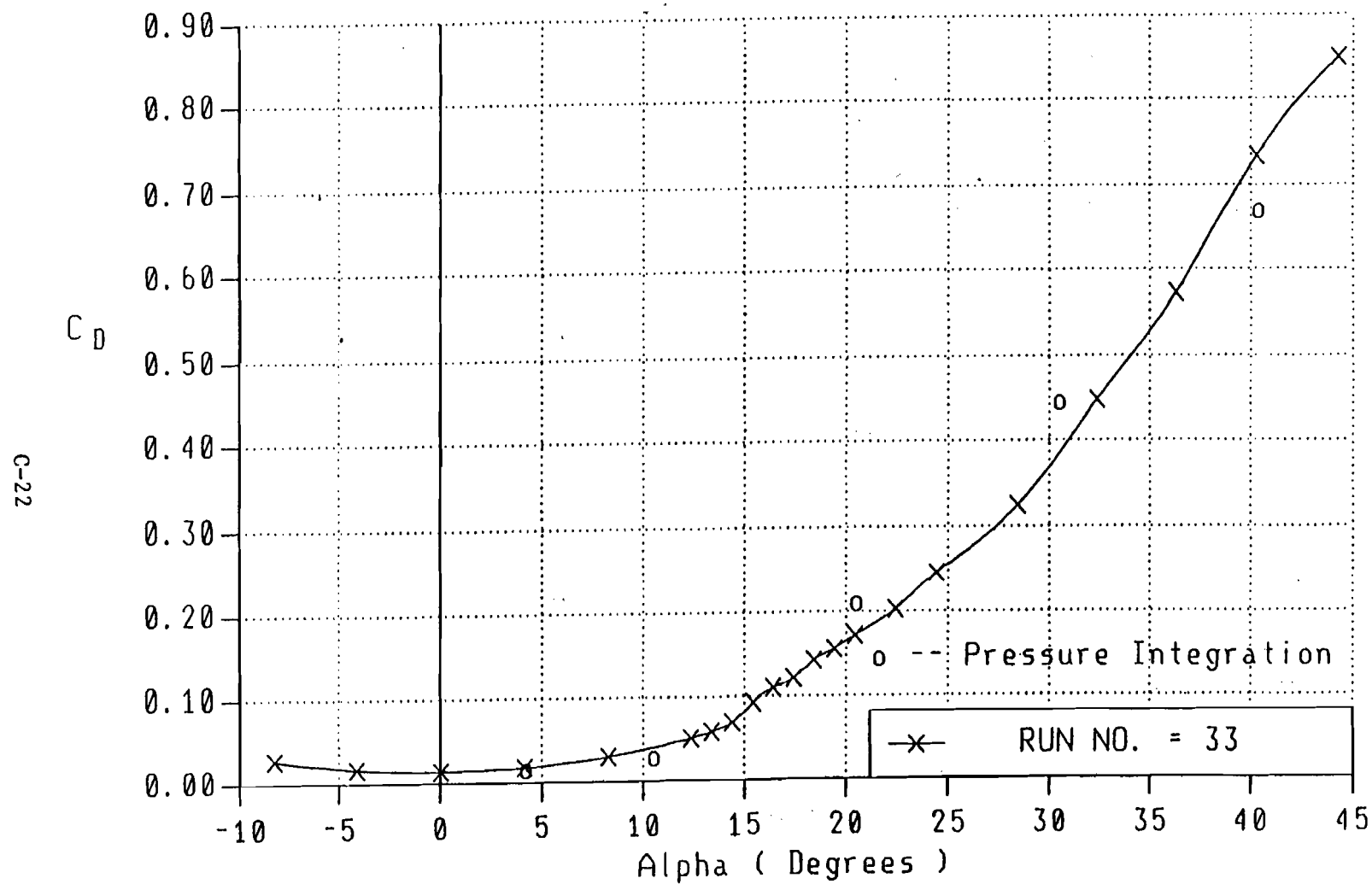
Figure 7. Wing Drag Coefficient By Balance and Integration of Surface Pressure
