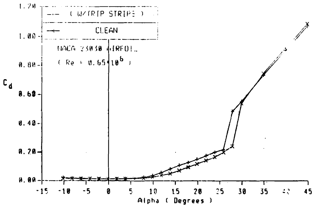
Figure 23. (b) Drag coefficients of NACA 23024 airfoil
