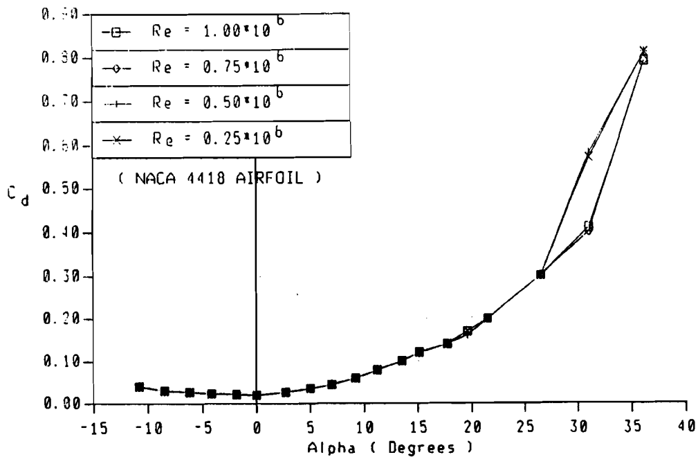
Figure 15. (b) Drag coefficients of NACA 4418 airfoil
