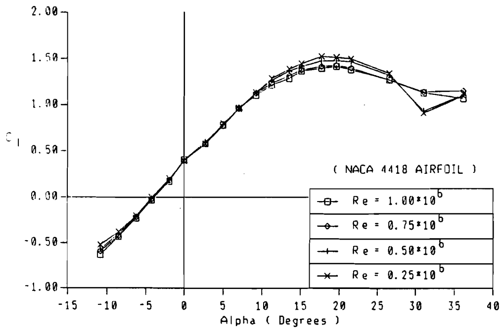
Figure 15. (a) Lift coefficients of NACA 4418 airfoil
