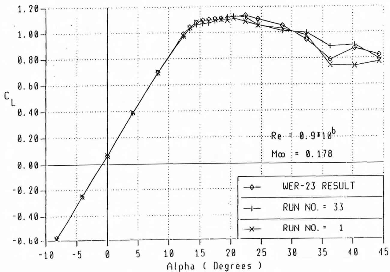
Figure 3. Wing Lift Coefficient for Three Tests
