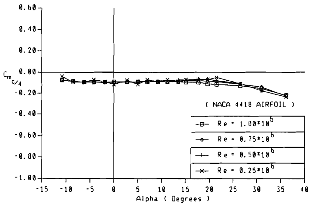
Figure 15. (c) Moment coefficients of NACA 4418 airfoil
