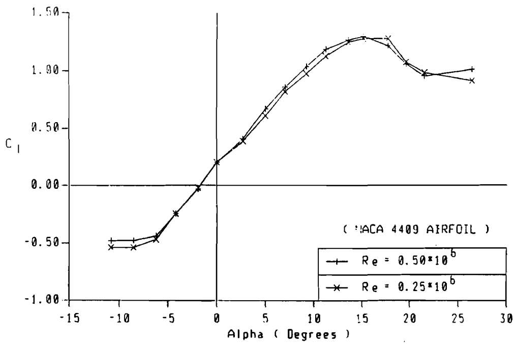
Figure 12. (a) Lift coefficients of NACA 4409 airfoil
