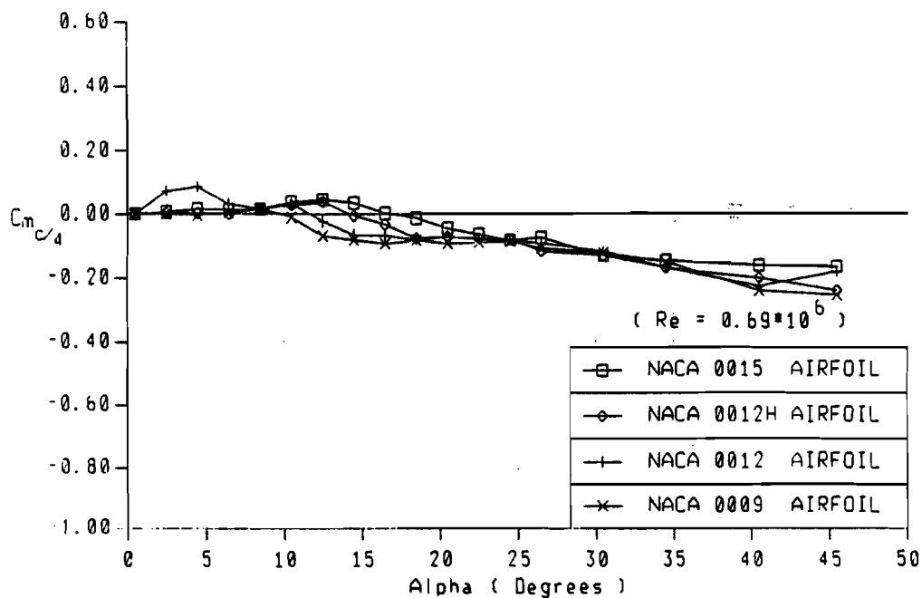
Figure 11. (c) Moment coefficients of NACA 00-series airfoils
