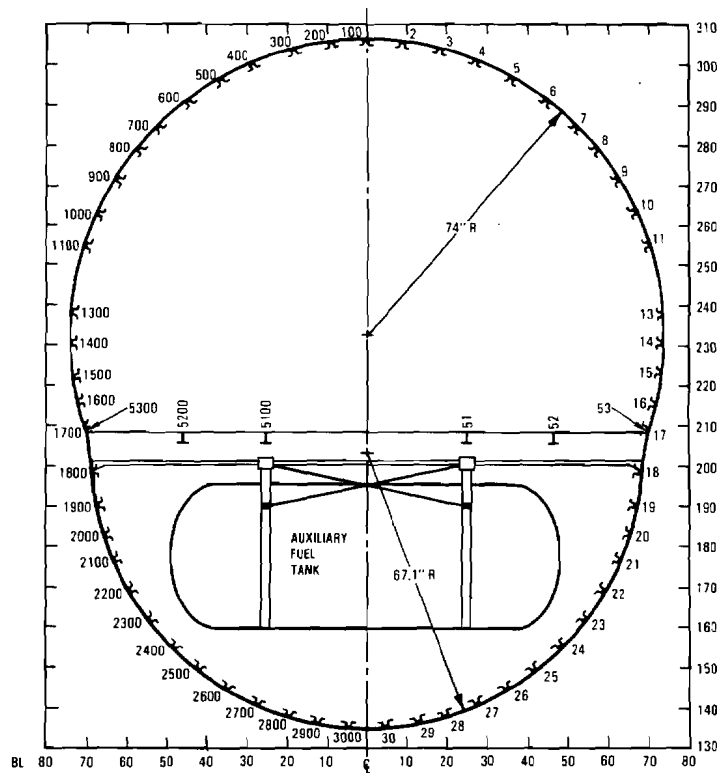
Figure 3-8. Installation Layout
