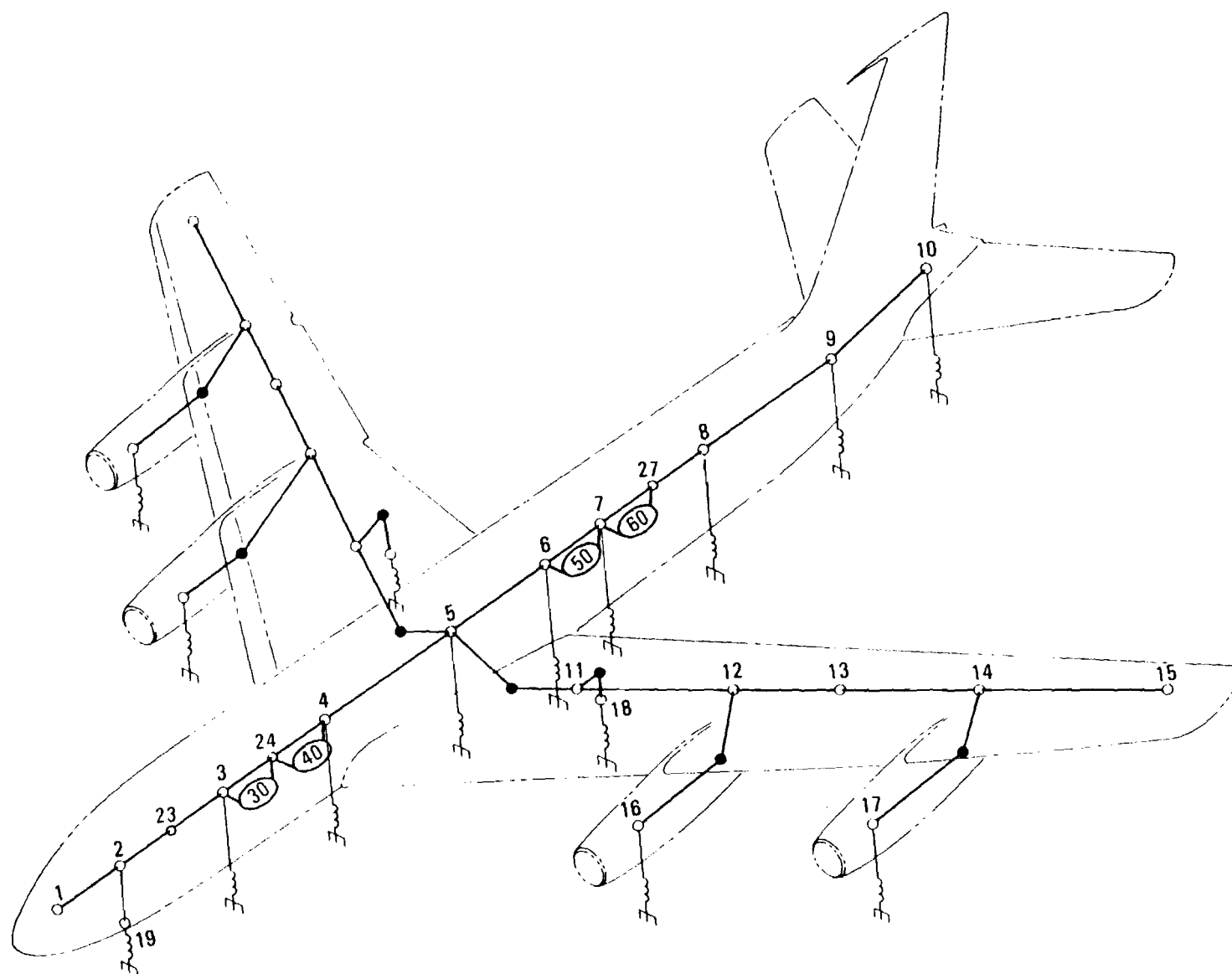
Figure 3-5. Symmetrical Airplane Stick Model
