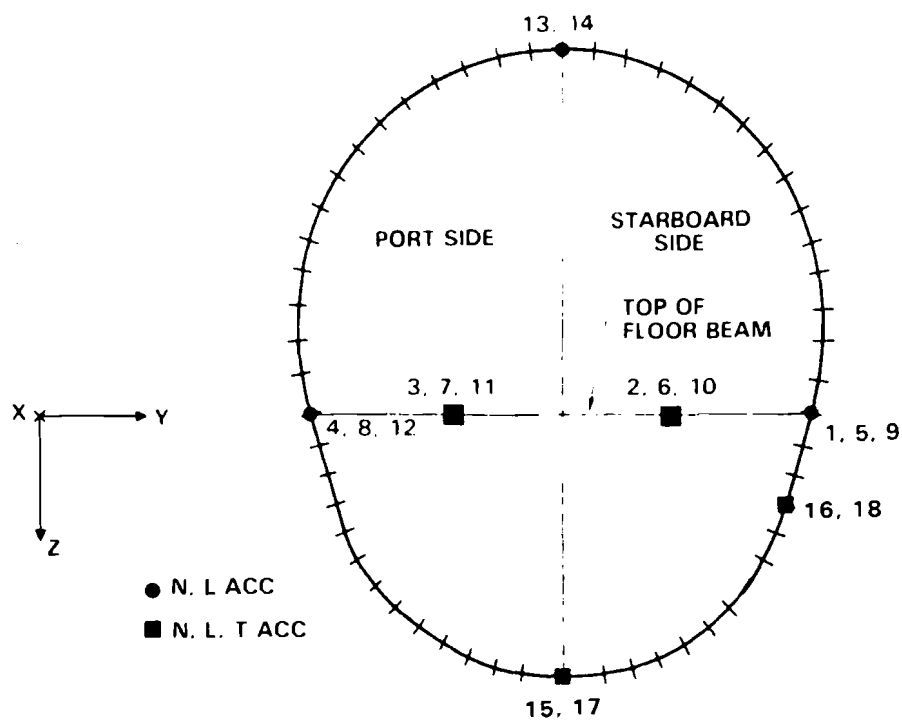
Figure A-11. End View of Floor and Airframe Instrumentation - Vertical Impact
