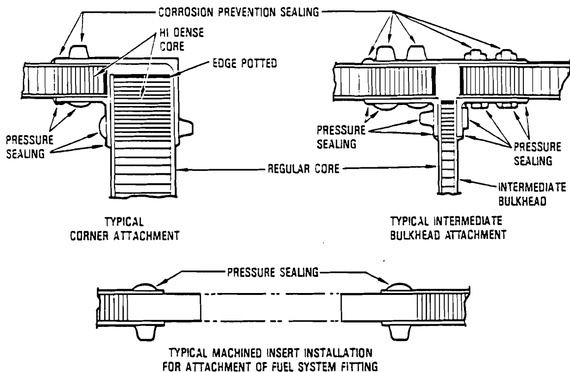
Figure 3-13. Fuel Tank Shell Construction
