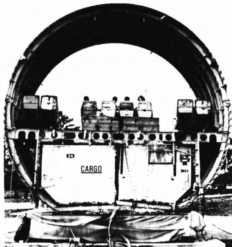
(b) HEAVILY LOADED SECTION: 25 FT/SEC IMPACT VELOCITY
