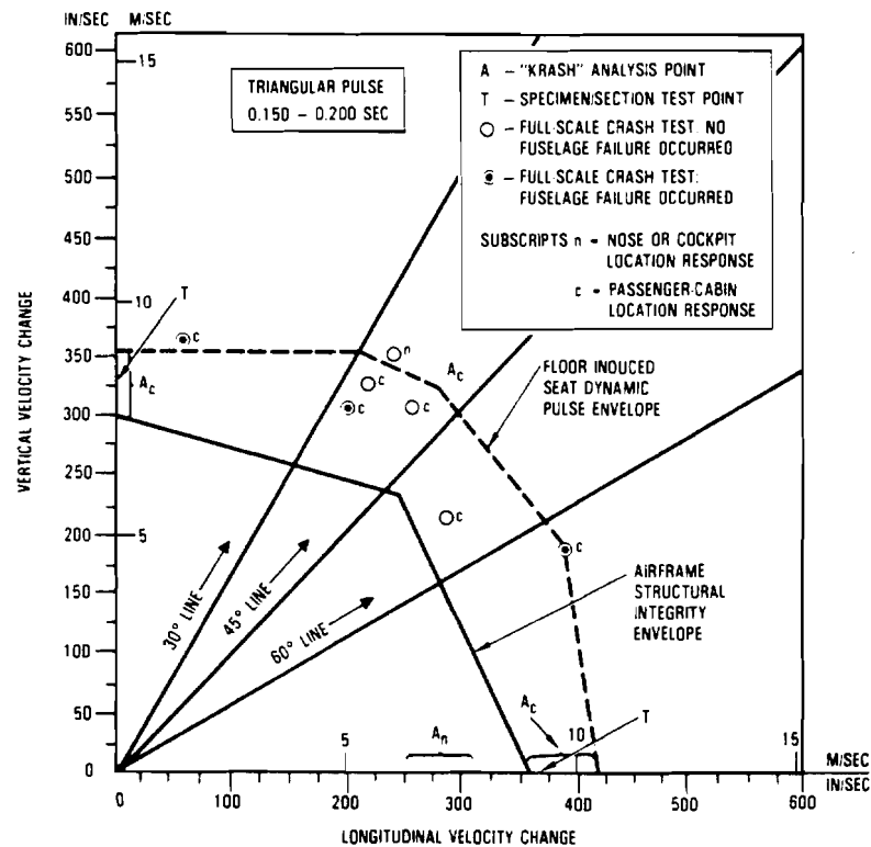
Figure 2-1. Structural Integrity Velocity Envelopes for Transport Category Airplanes
