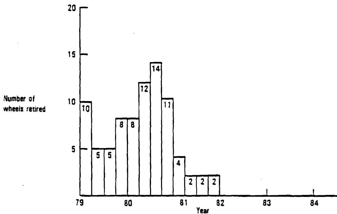
Figure 2-29. Number of Broken Flange Retirements, 10-1213 Outboard Half
