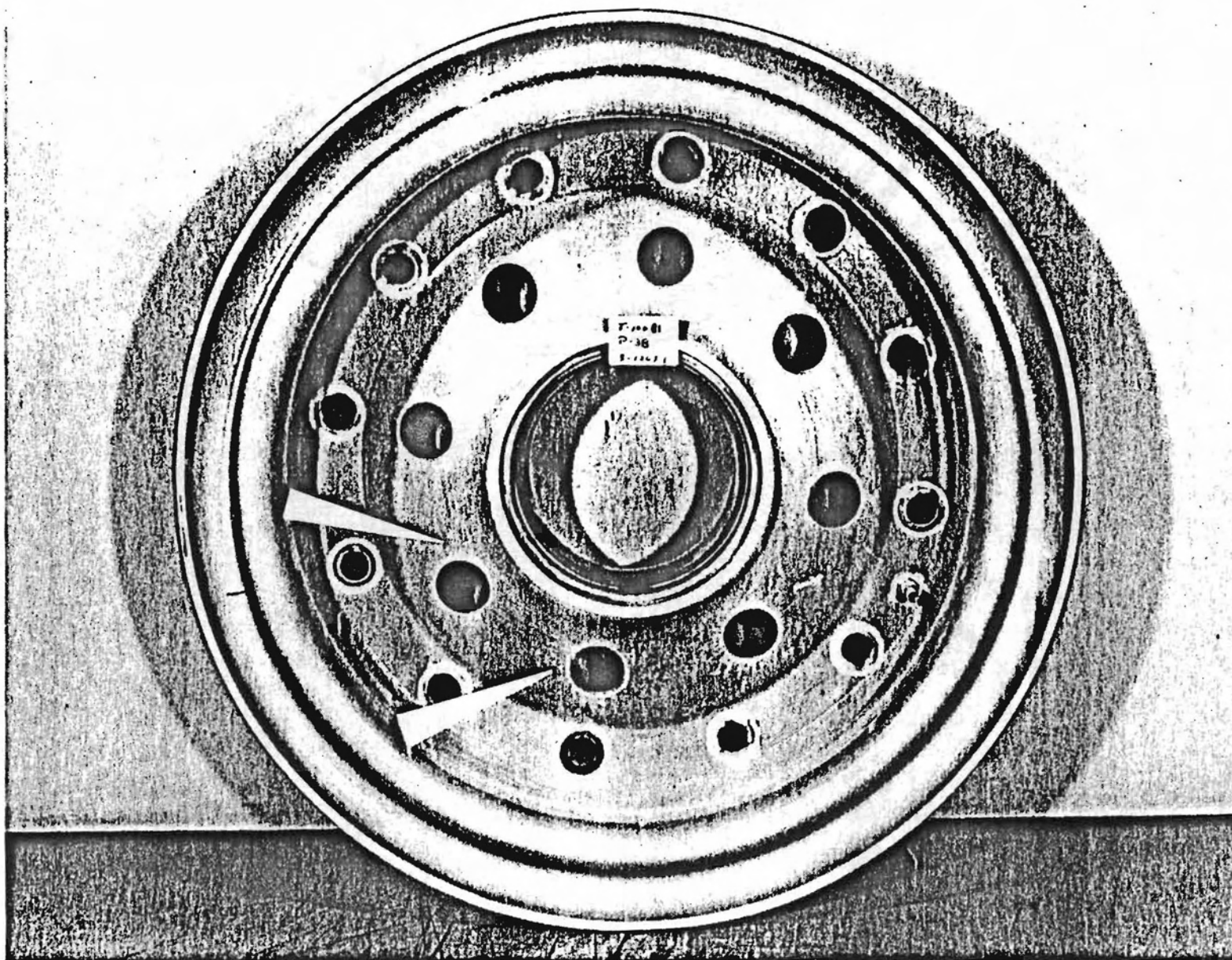
Figure 2-10. Stress Coat Test Results, Outboard Wheel Half
