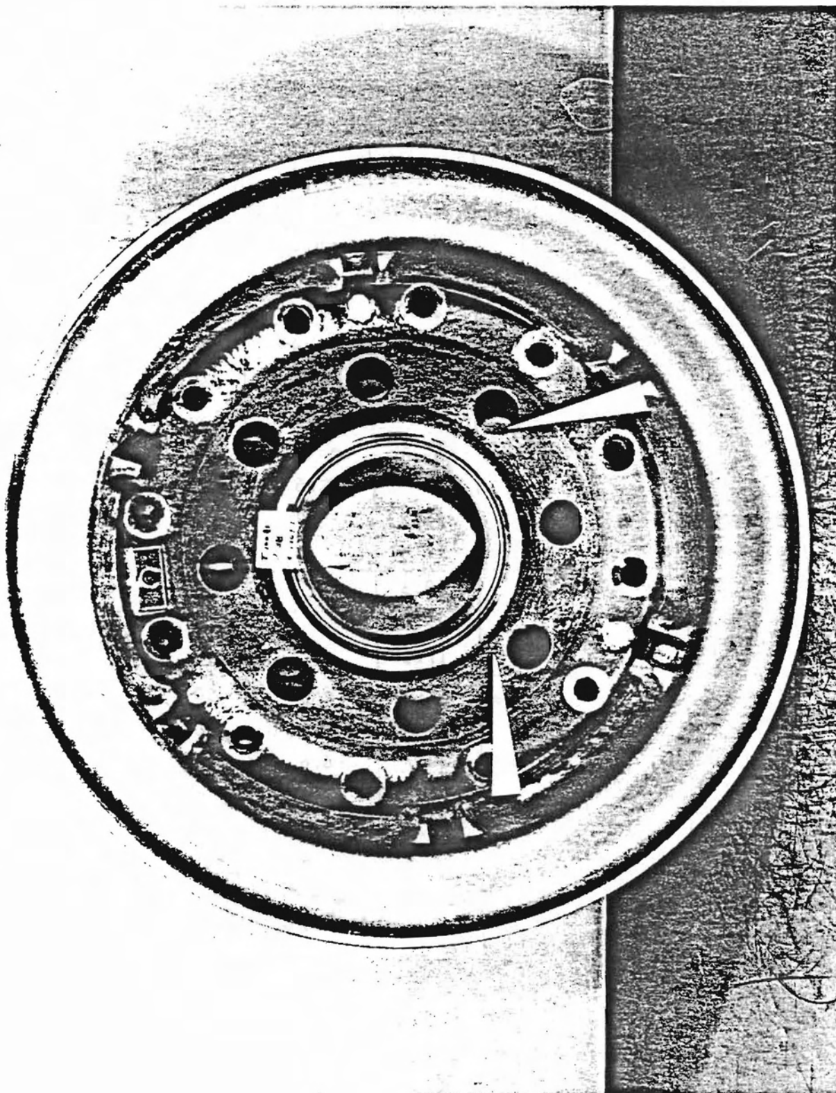
Figure 2-8. Stress Coat, Results, Inboard Wheel Half
