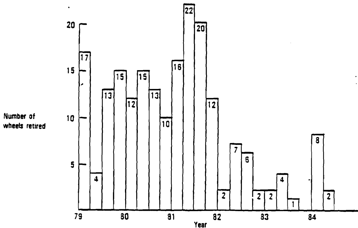
Figure 2-30. Number of Cracked Flange Retirements, 10-1213 Outboard Half
