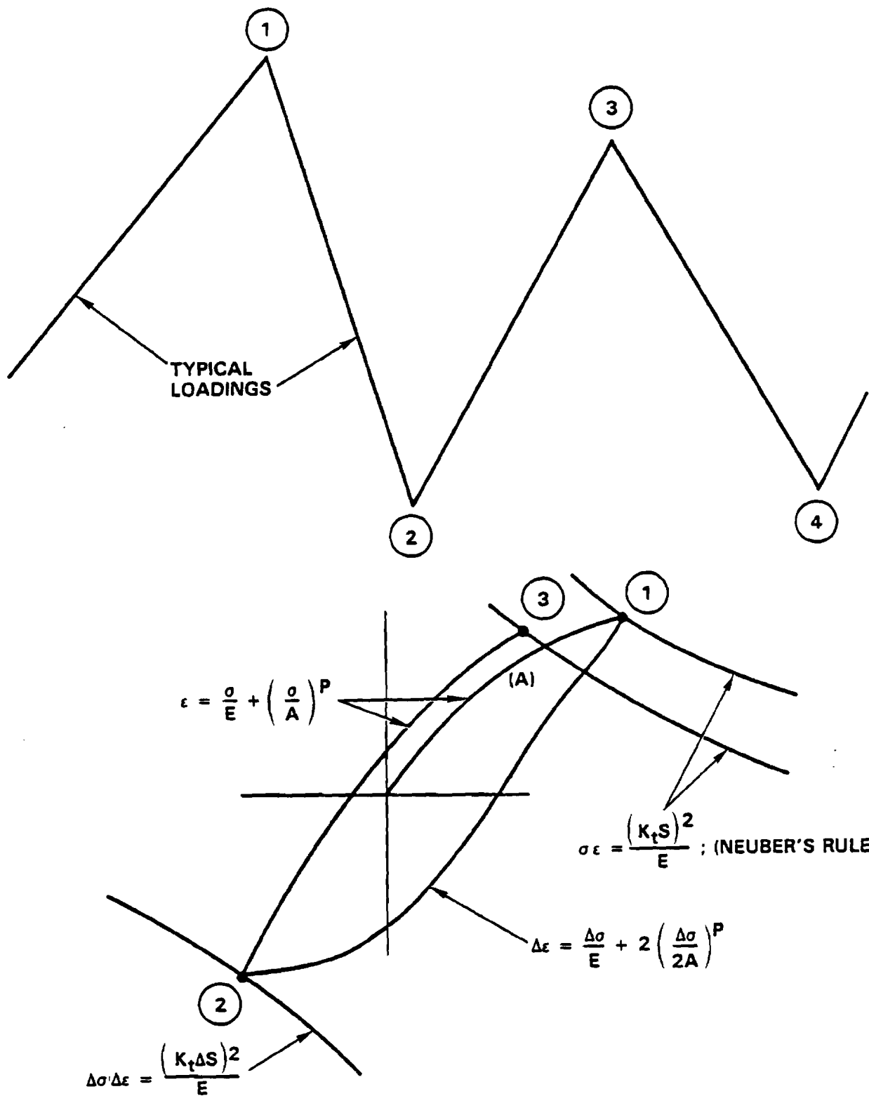
Figure 2-16. Local Stress-Strain for Typical Loadings
