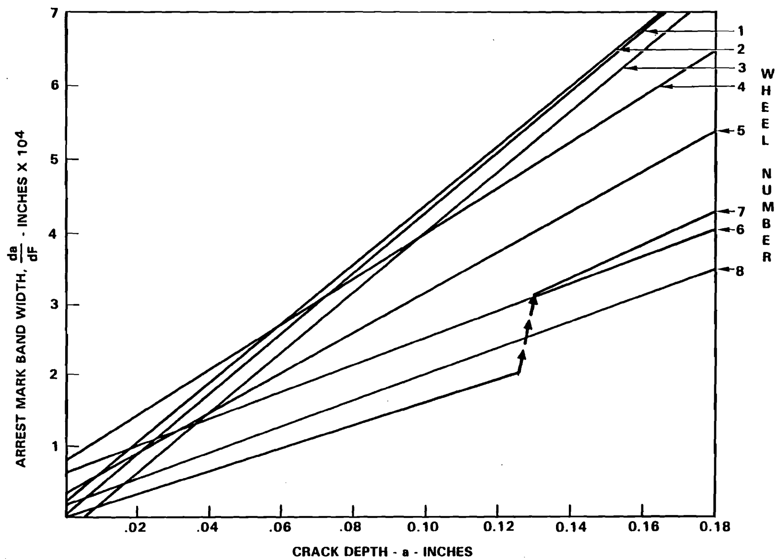
Figure 2-21. Linear Regression Plots of Arrest Mark Spacing Versus Crack Depth
