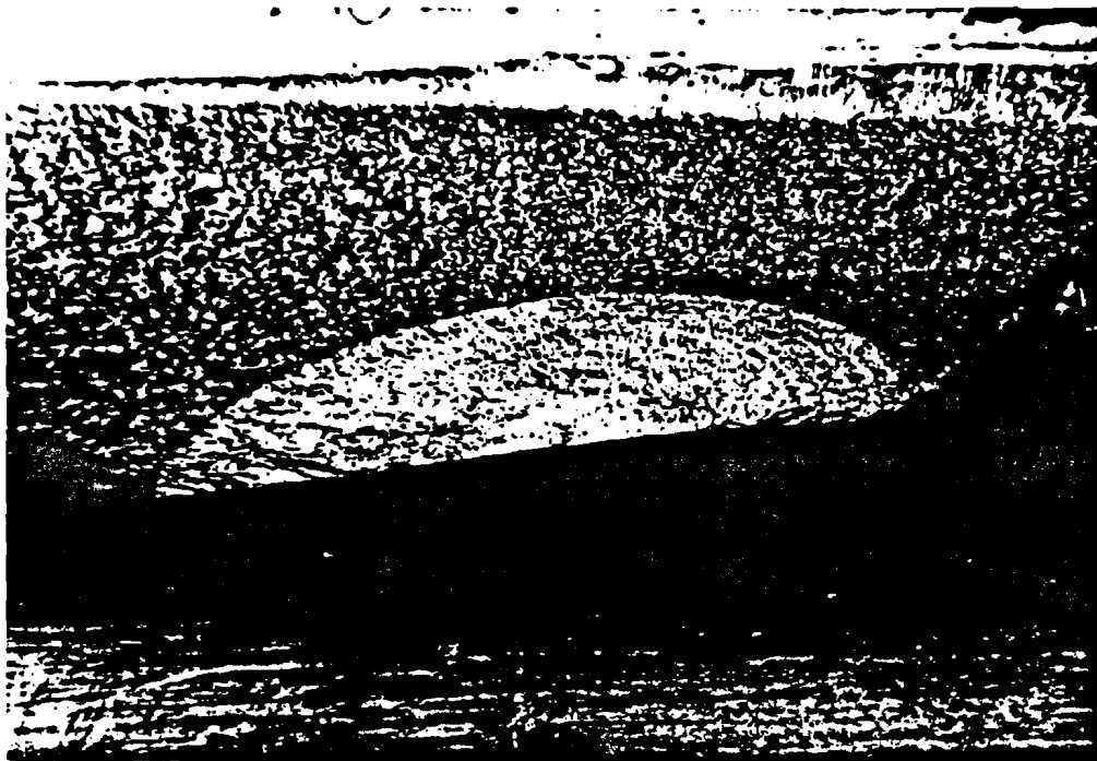
Figure 2-18. Fracture Surface of a Wheel Flange Showing Typical Semi-Elliptical Surface Crack Where Cracking Originated.
