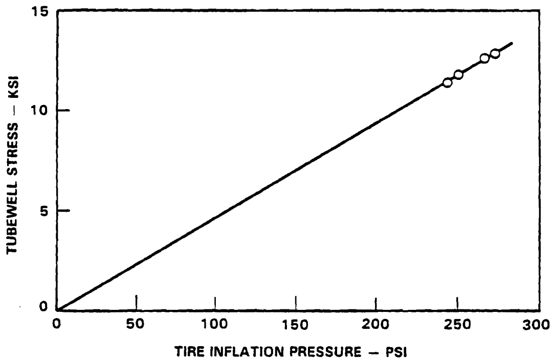
Figure 2-12. Tubewell Stress Variation with Tire Pressure
