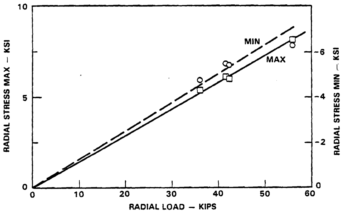
Figure 2-13. Tubewell Maximum and Minimum Stresses from Radial Loads with No Lateral Loads
