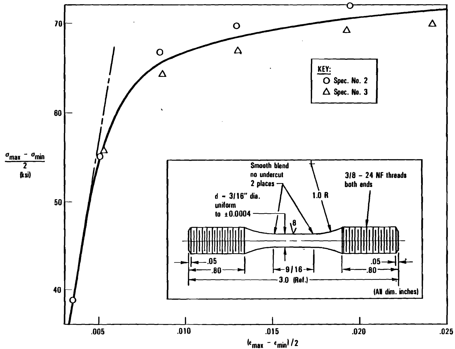
Figure 2-15. Results of Cyclic Stress-Strain Tests for 2014-T6 Wheel Forging
