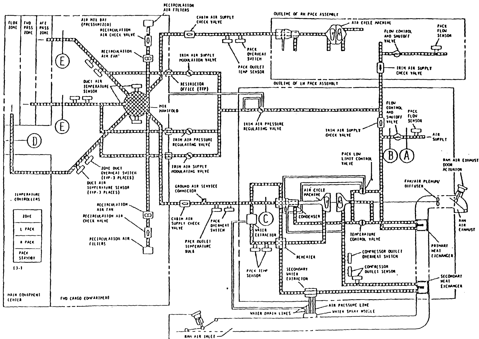
FIGURE 4.2.3.7-1. CONCEPT A, 767, HIGH FLOW MODE
