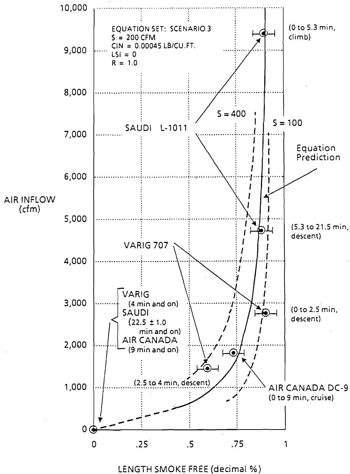
FIGURE 5-6. EQUATIONS COMPARED TO PAST FIRES
