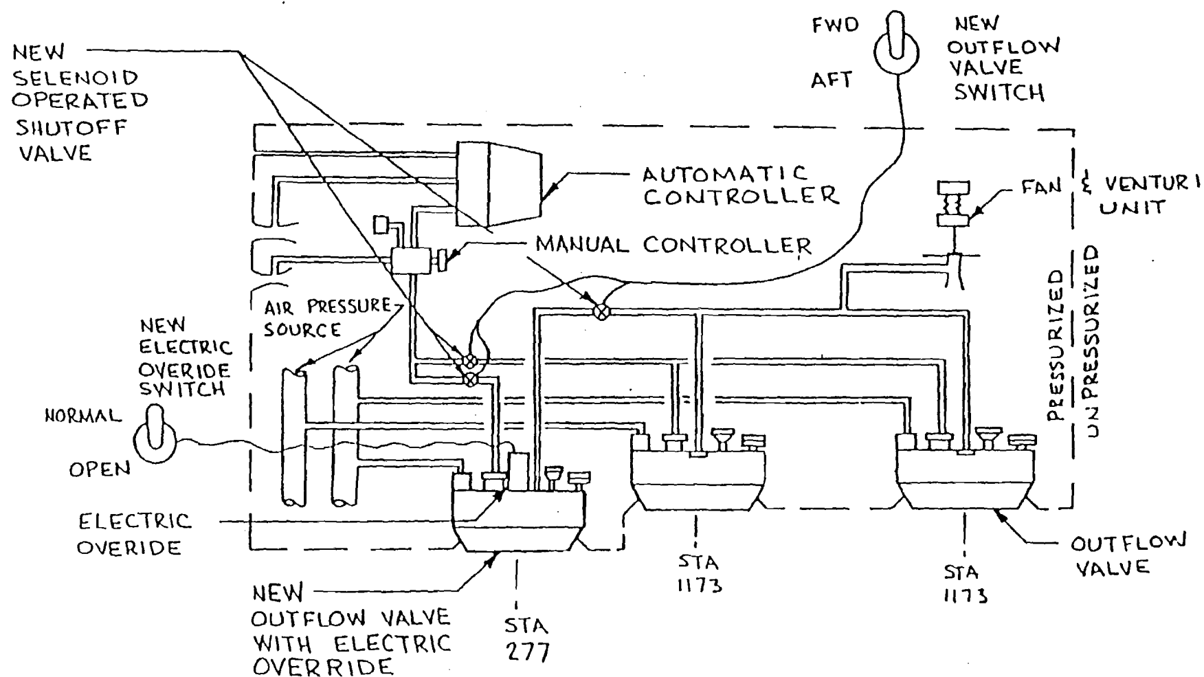
FIGURE 4.2.3.2-2 CONCEPT A, 727-100, DUAL OUTFLOW VALVE
