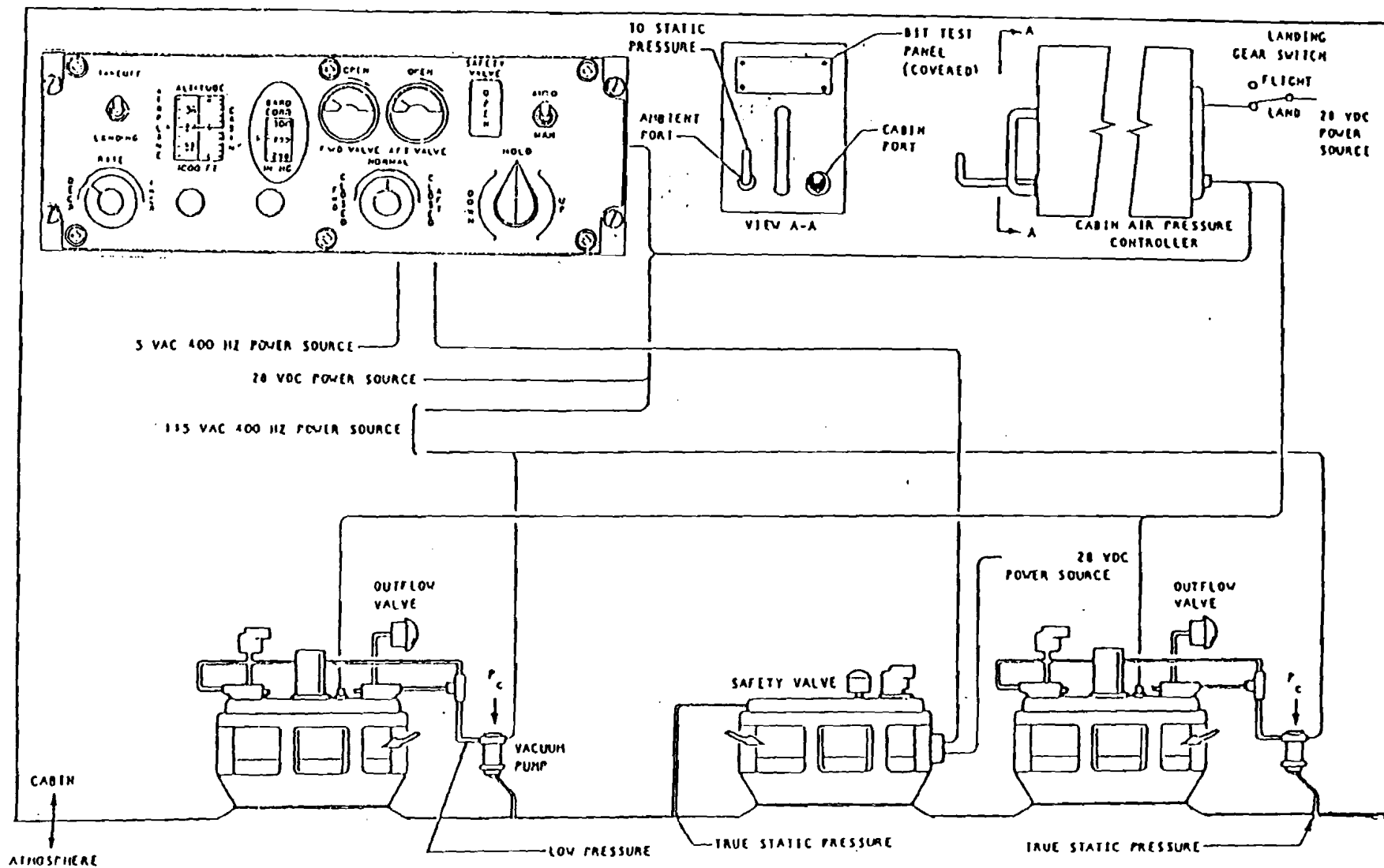
FIGURE 4.2.3.1-2. CONCEPT A, 707, DUAL OUTFLOW VALVE ELECTRO-PNEUMATIC
