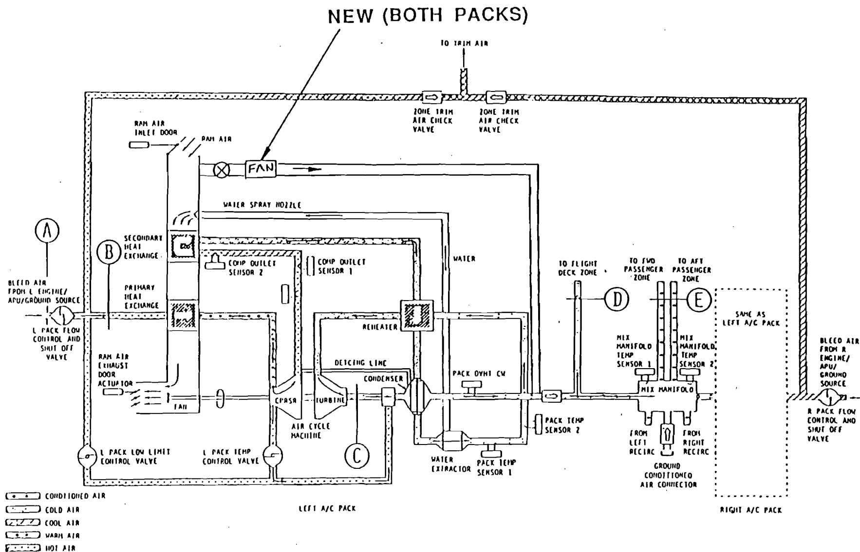
FIGURE 4.3.3.6-1. CONCEPT B, 757, RAM VENTILATION
