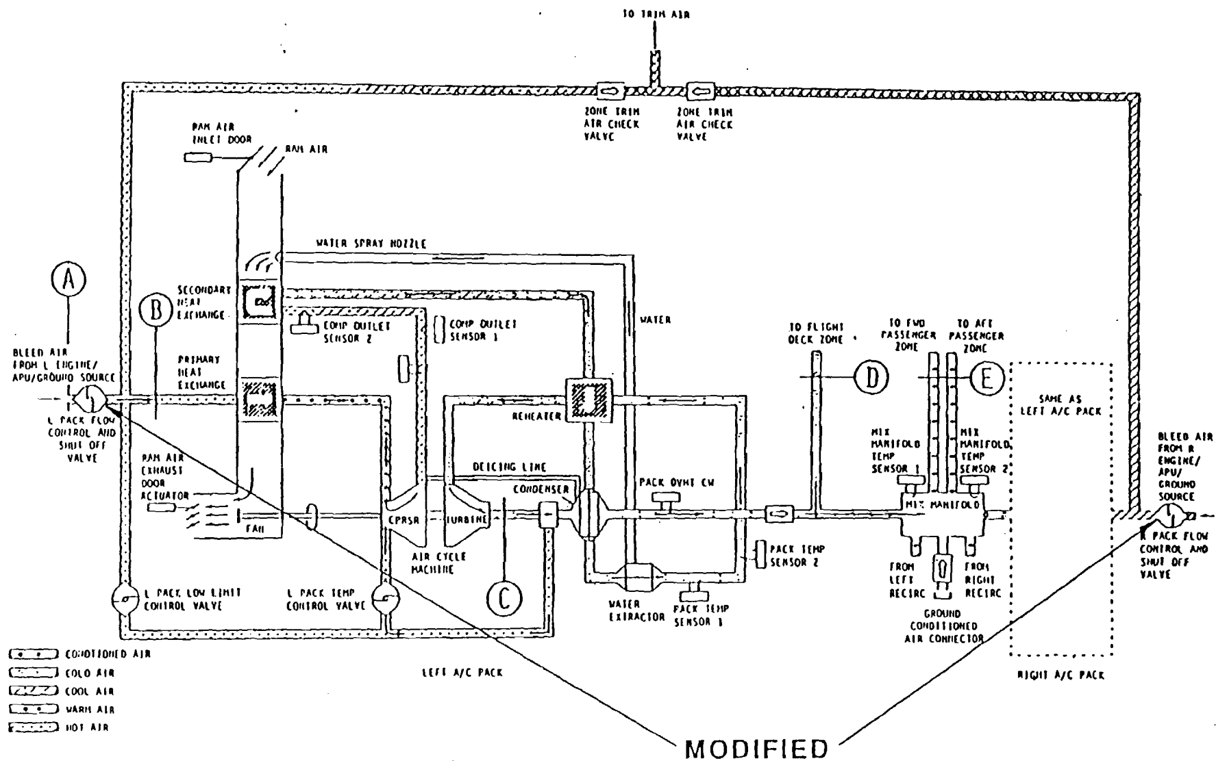
FIGURE 4.2, 3.6-1. CONCEPT A, 757, HIGH FLOW MODE
