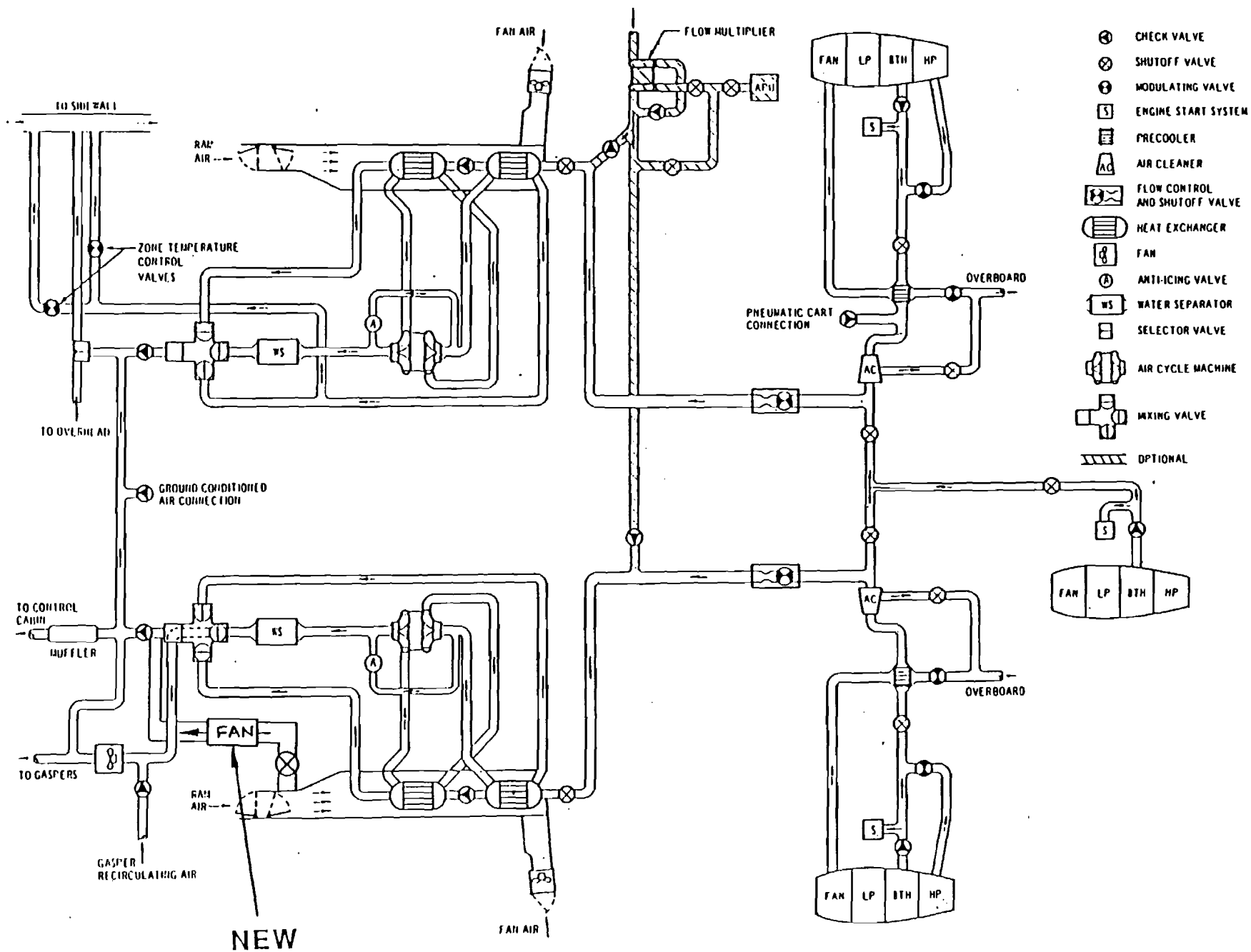
FIGURE 4.3.3.3-1. CONCEPT B, 727-200, RAM VENTILATION
