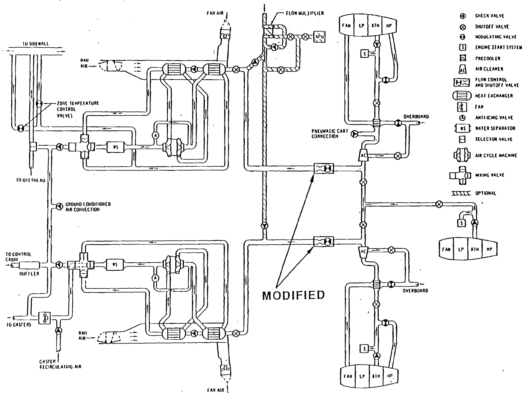
FIGURE 4.2.3.3-1 CONCEPT A 727-200 HIGH FLOW MODE
