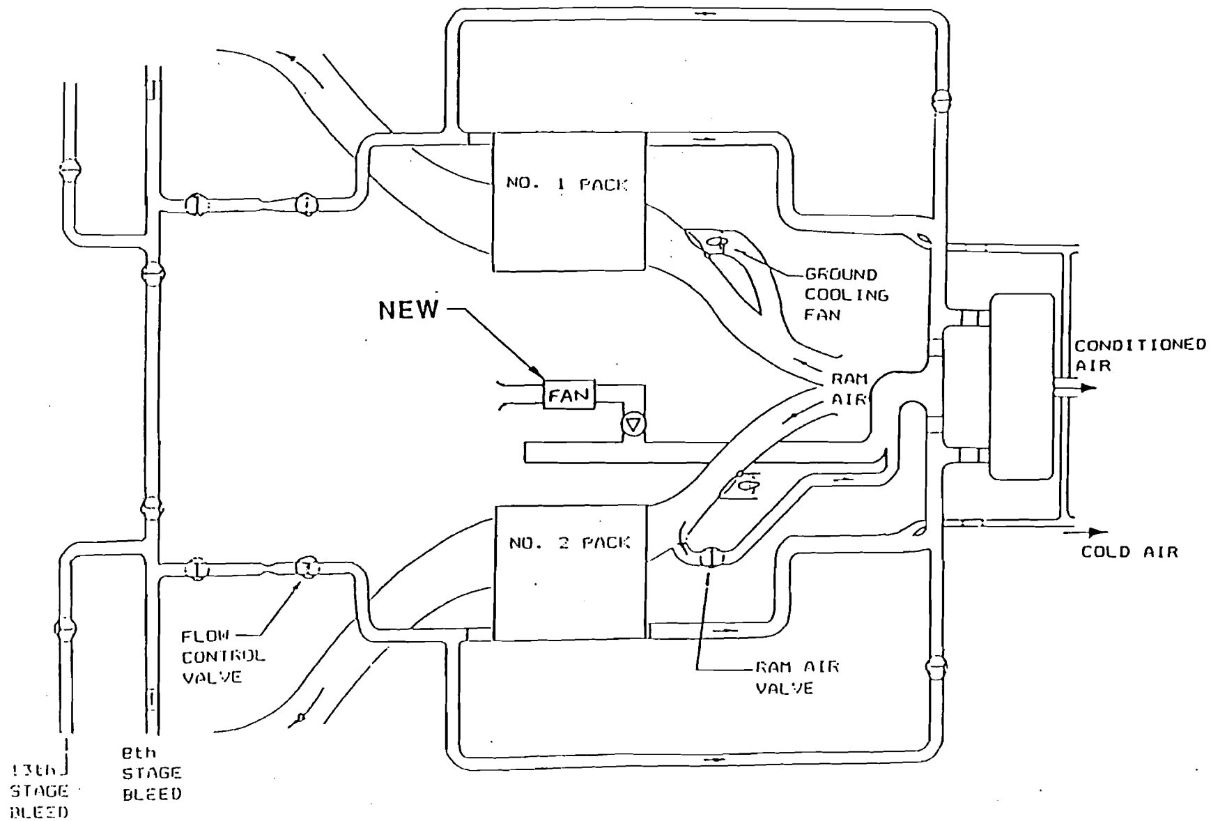
FIGURE 4.3.3.9-1. CONCEPT B, DC-9, RAM VENTILATION
