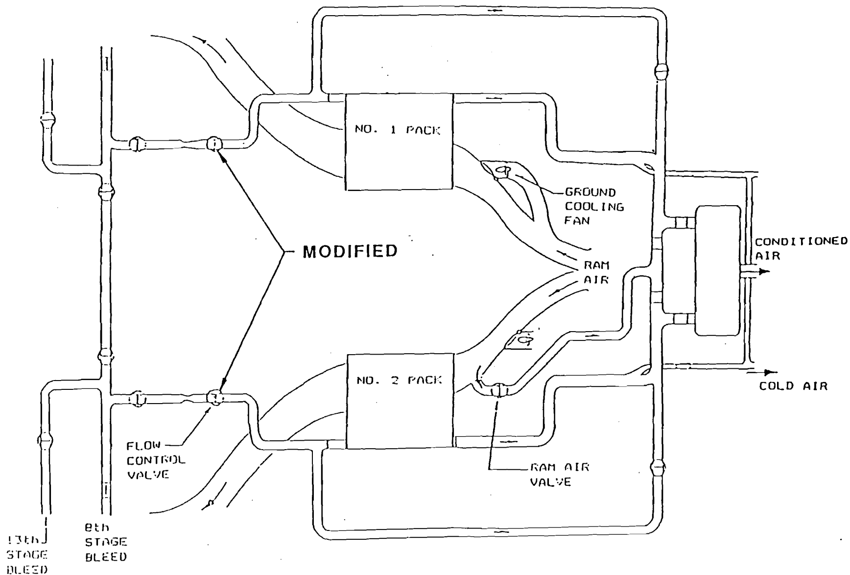
FIGURE 4.2.3.9-1. CONCEPT A, DC-9, HIGH FLOW MODE
