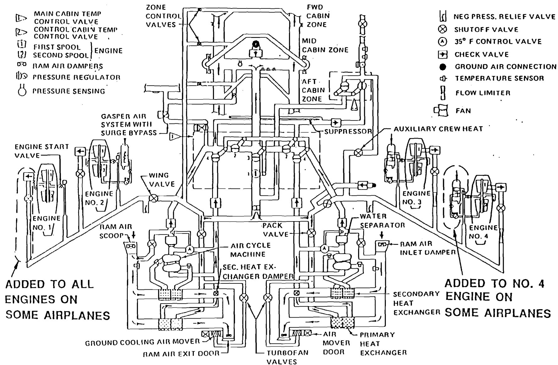
FIGURE 4.2.3.1-1. CONCEPT A, 707, HIGH FLOW MODE
