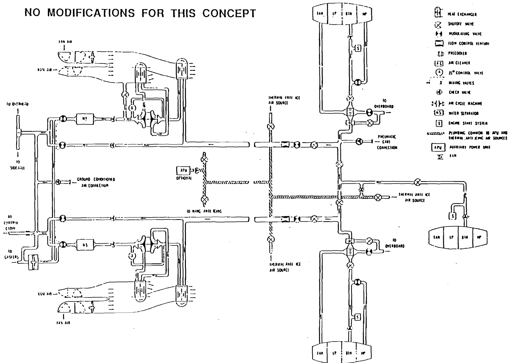
FIGURE 4.2.3.2-1. CONCEPT A, 727-100, HIGH FLOW MODE
