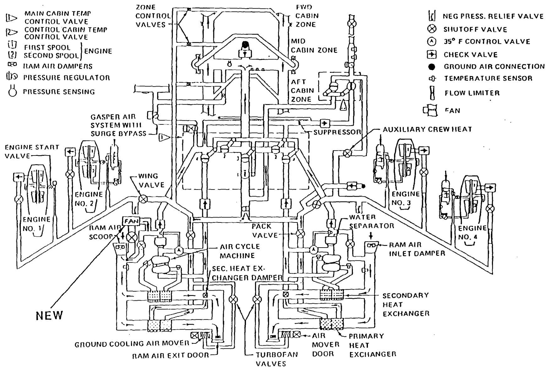
FIGURE 4.3.3.1-1. CONCEPT B, 707, RAM VENTILATION
