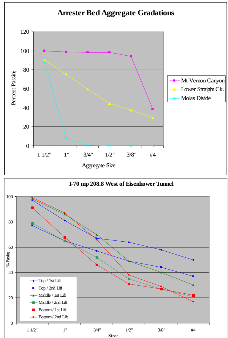
Figure 1. Top - Average gradations at Mt. Vernon Canyon, Lower Straight Creek and Molas Divide. Bottom -All samples Lower Straight Creek.
