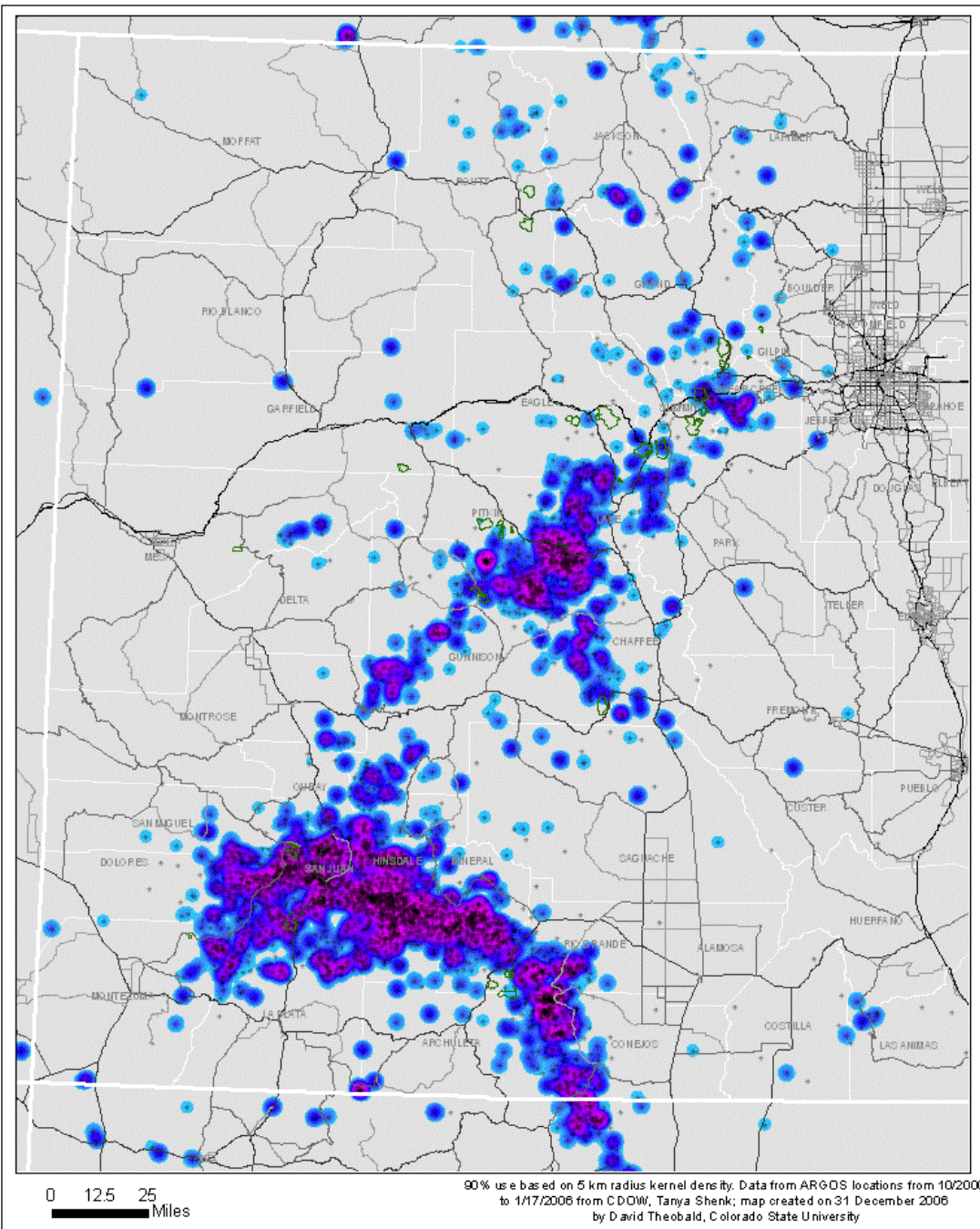
Figure 36. 90% kernel density function based on locations of 131 lynx from October 2000 to January 2006 derived from ARGOS satellites.
