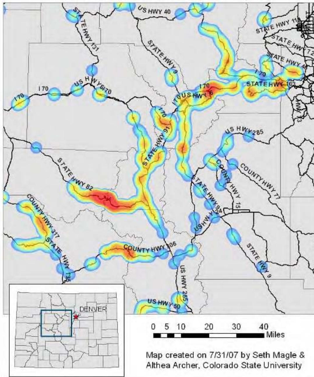
Figure 48. 95% kernel density map of potential areas of lynx highway crossings in west-central Colorado, based on straight-line connections between consecutive lynx spatial locations collected less than two weeks apart, as derived from ARGOS satellite telemetry.
