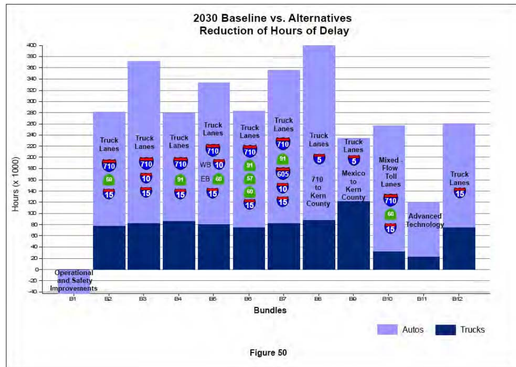
Figure 5.1 Delay Reduction from Truck Lane Alternatives
