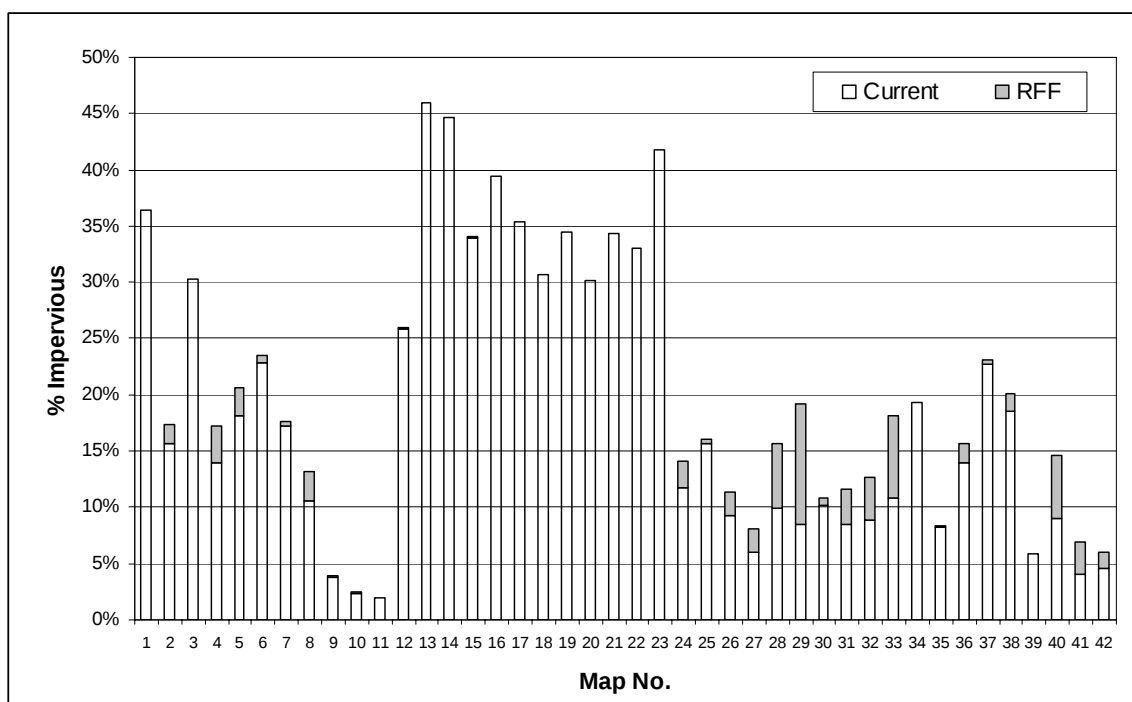
Figure 13. Percentage impervious areas of the project area watersheds
