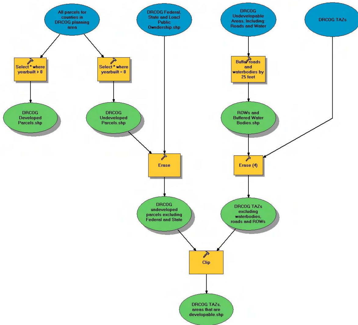
Figure 10. Model Builder diagram of regional projection method
