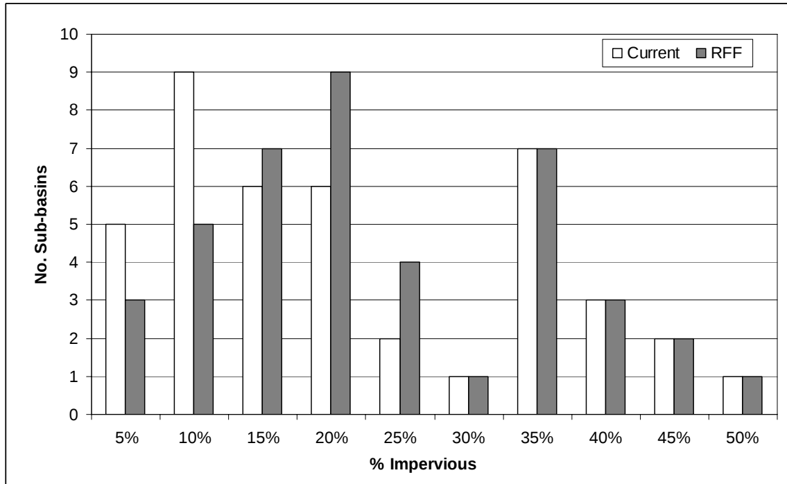
Figure 14. Number of sub-basins in interval category of % impervious
