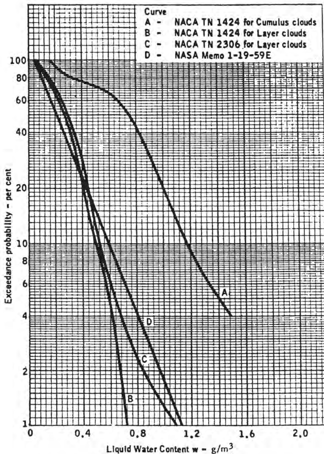
FIGURE 1-27. EXCEEDANCE PROBABILITY FOR MAXIMUM LWC (REFERENCES 1-6, 1-10 AND 1-16)
