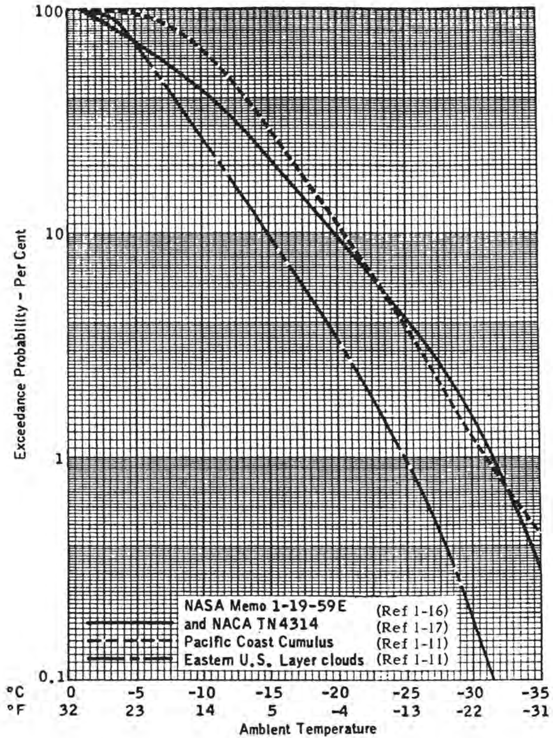
FIGURE 1-29. PROBABILITY OF CLOUD ICING TEMPERATURE
