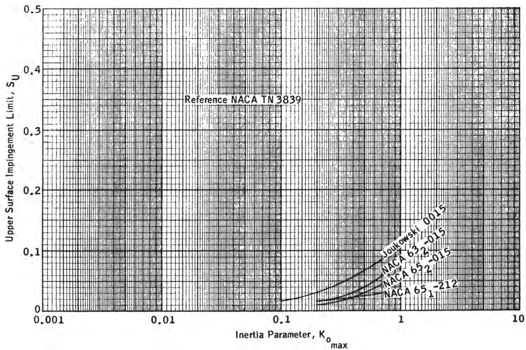
FIGURE 2-25. UPPER SURFACE IMPINGEMENT LIMITS FOR SEVERAL AIRFOILS AT 8° ANGLE OF ATTACK (EXPERIMENTAL DATA)
