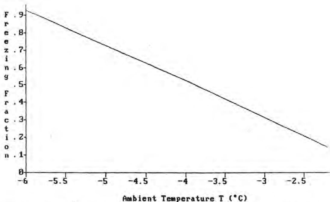
FIGURE 2-75. FREEZING FRACTION VS AMBIENT TEMPERATURE T_{\infty} FOR A CIRCULAR CYLINDER WITH DIAMETER 20 CM
