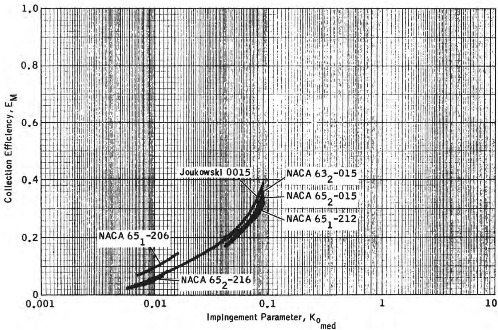
FIGURE 2-18. COLLECTION EFFICIENCY VERSUS K_{0_{MED}} FOR AIRFOILS -EXPERIMENTAL DATA FOR 4° ANGLE OF ATTACK
