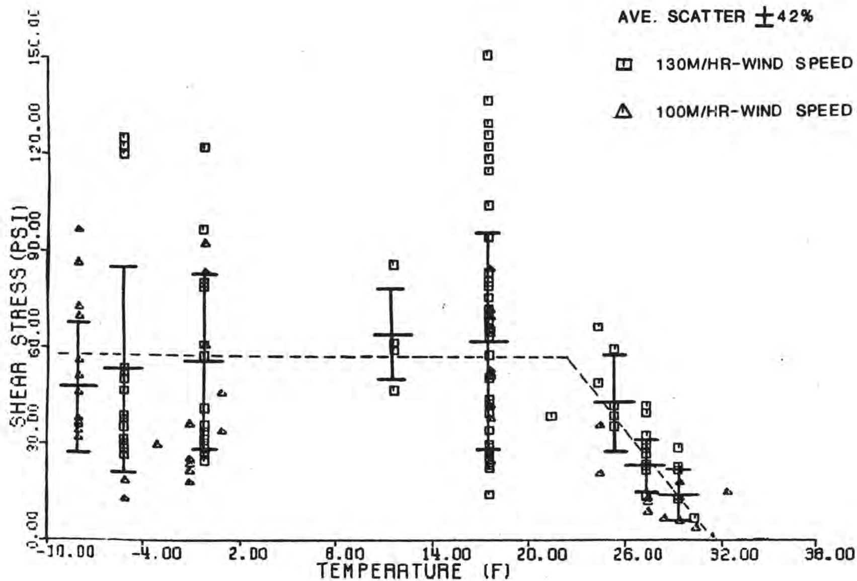
FIGURE 2-86. ADHESIVE SHEAR STRESS VS. INTERFACE TEMPERATURE (REFERENCE 2-64)
