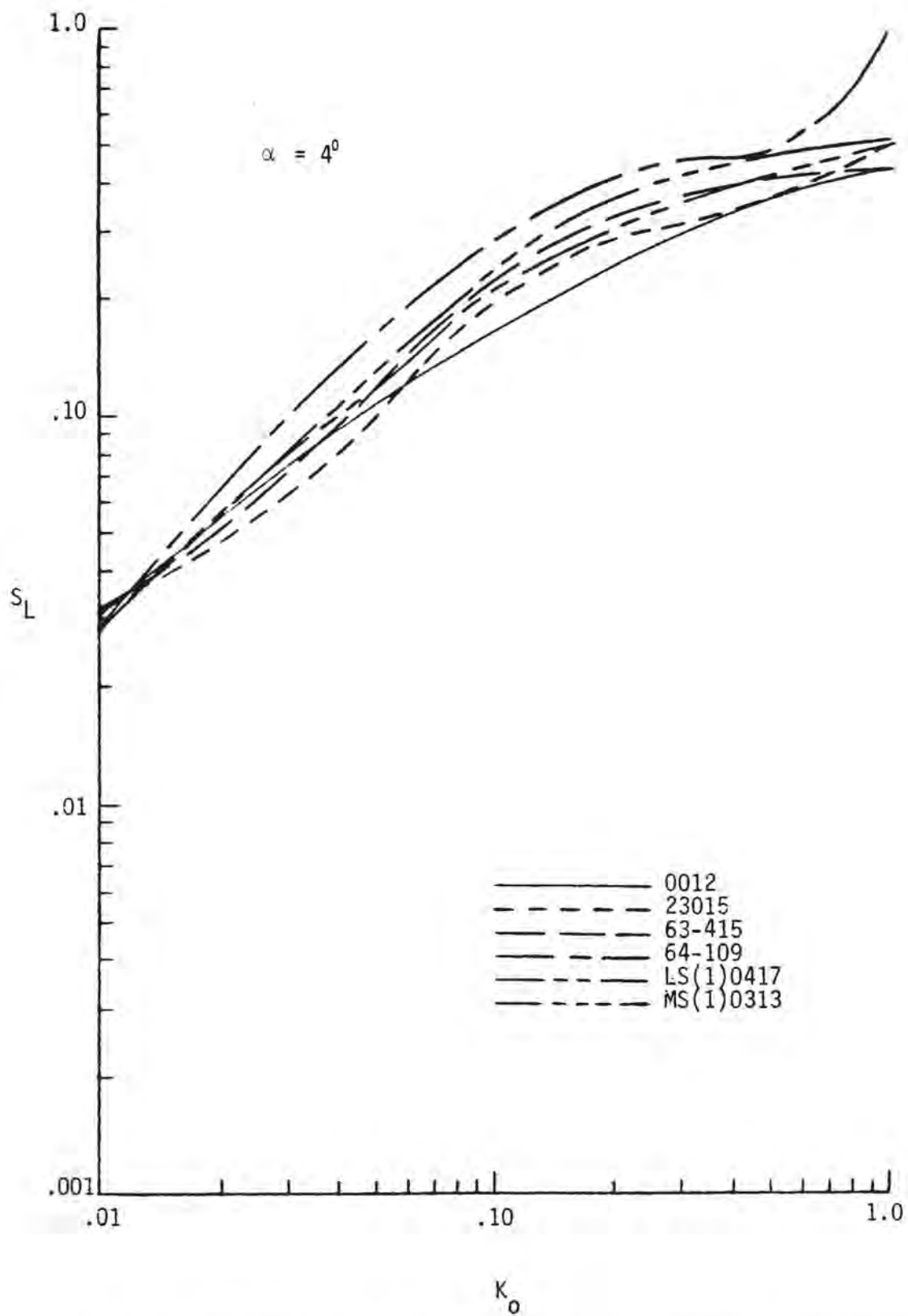
FIGURE 2-55. THEORETICAL DATA ON THE LOWER SURFACE IMPINGEMENT LIMIT OF SEVERAL AIRFOILS ( \alpha = 4^\circ )
