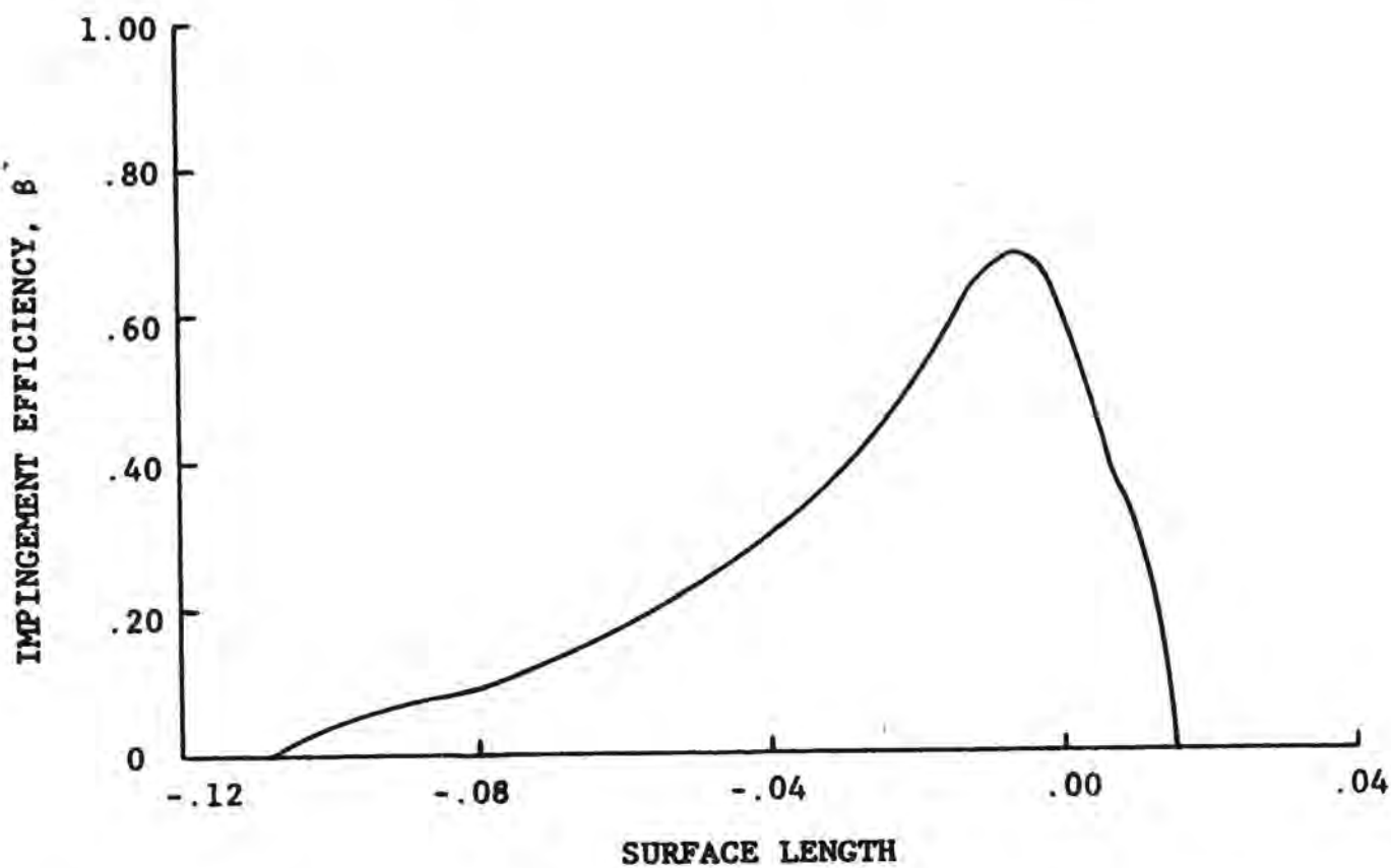
FIGURE 2-8. EXAMPLE OF IMPINGEMENT EFFICIENCY CURVE ( \beta -CURVE)
