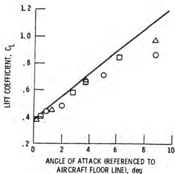
(a) Variation of aircraft C_L versus \alpha
