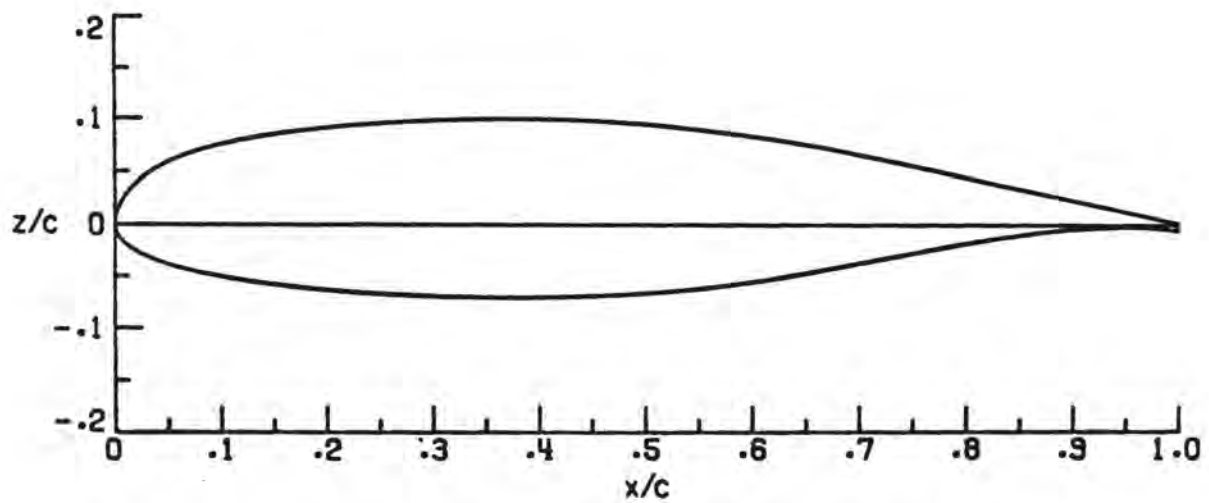
(C) MS(1)-0317 SUPERCRITICAL AIRFOIL
