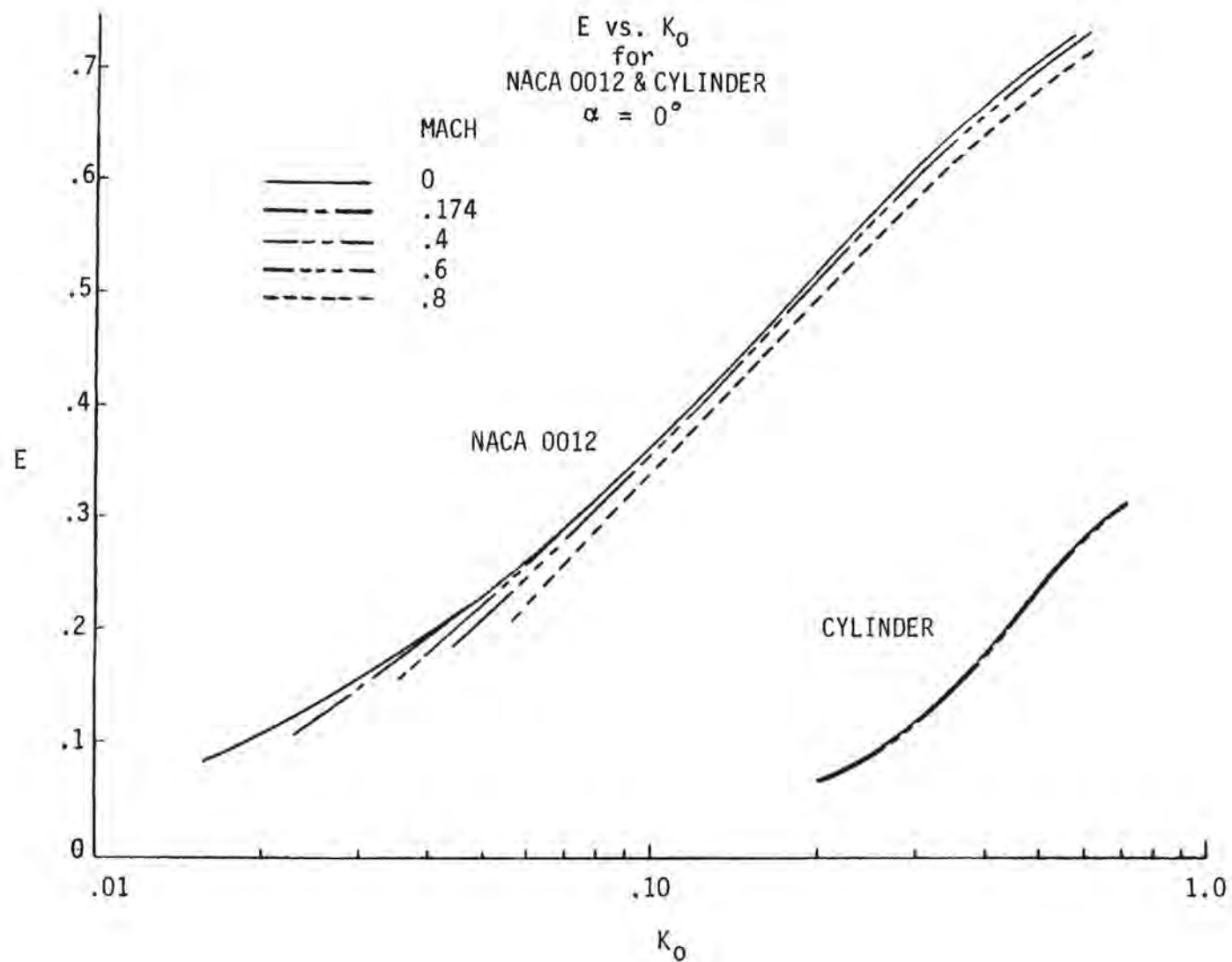
FIGURE 2-15. COMPRESSIBLE DROPLET IMPINGEMENT DATA ON A NACA 0012 AIRFOIL AND A CYLINDER
