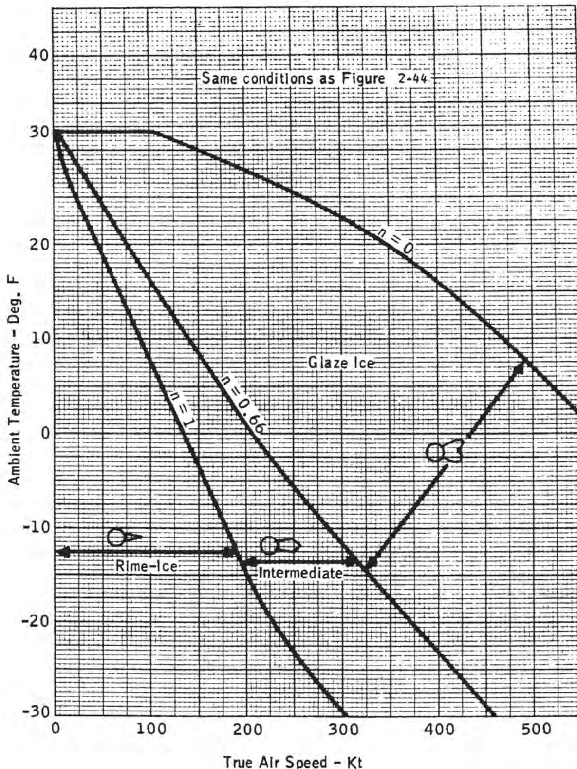
FIGURE 2-82. ICE SHAPE TYPES AS A FUNCTION OF SPEED AND AMBIENT TEMPERATURE FOR A LIQUID WATER CONTENT OF 0.5 \text{ G/M}^3 (REFERENCE 2-49)
