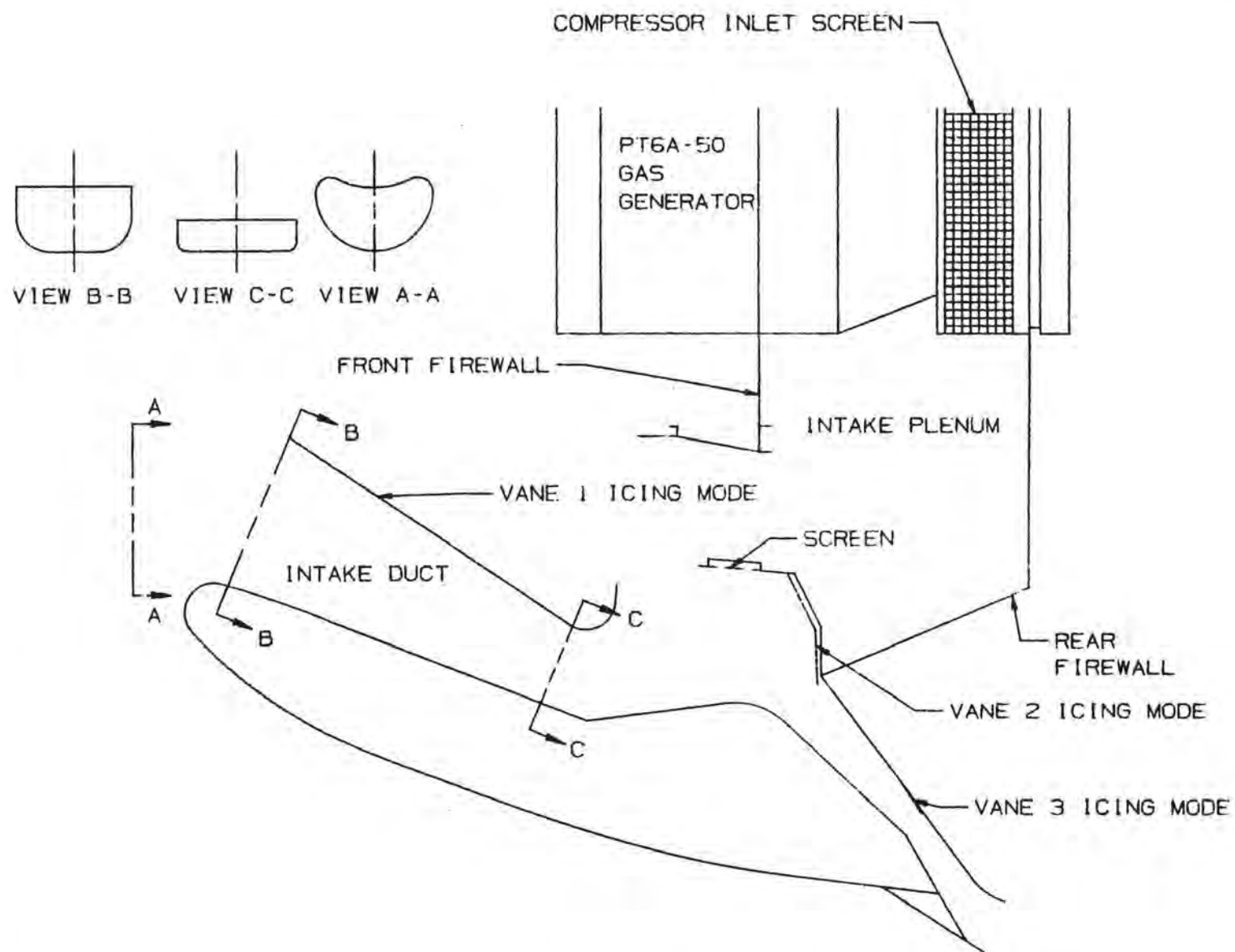
FIGURE 2-106b. PT6A-50 ANTI-ICING CONFIGURATION INERTIAL SEPARATION SYSTEM
