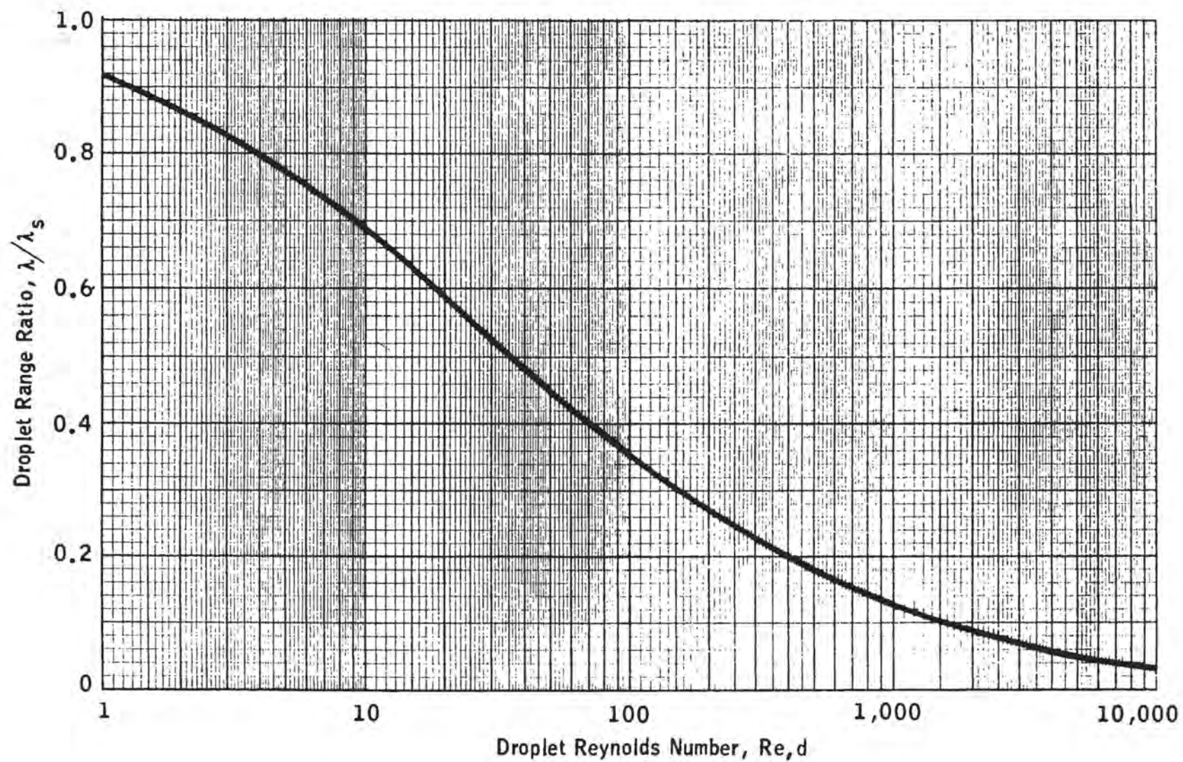
FIGURE 2-2. DROPLET RANGE RATIO AS A FUNCTION OF DROPLET REYNOLDS NUMBER (REFERENCE 2-22)
