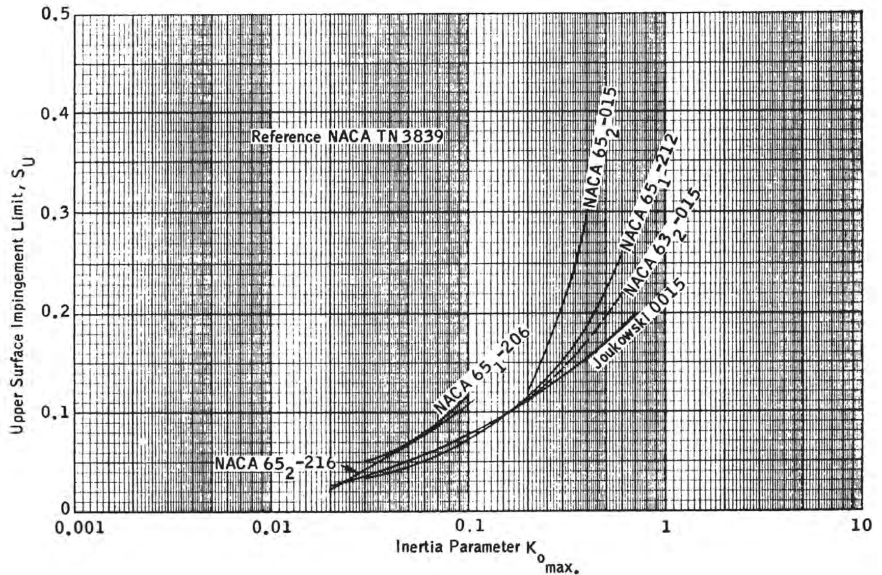
FIGURE 2-21. UPPER SURFACE IMPINGEMENT LIMITS FOR SEVERAL AIRFOILS AT 0° ANGLE OF ATTACK (EXPERIMENTAL DATA)
