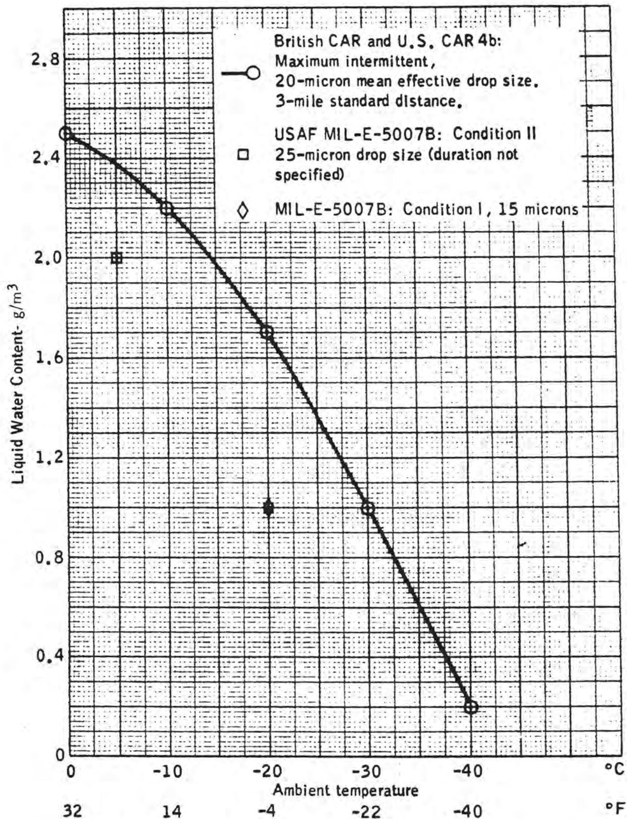
FIGURE 3-16. BRITISH AND US STANDARD FOR INTERMITTENT ICING (REFERENCE 3-2, 3-24, 3-31)
