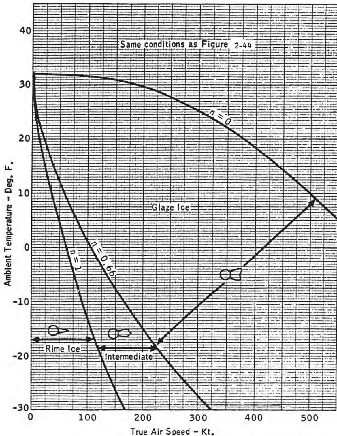
FIGURE 2-83. ICE SHAPE TYPES AS A FUNCTION OF SPEED AND AMBIENT TEMPERATURE FOR A LIQUID WATER CONTENT OF 1.0 \text{ G/M}^3 (REFERENCE 2-49)
