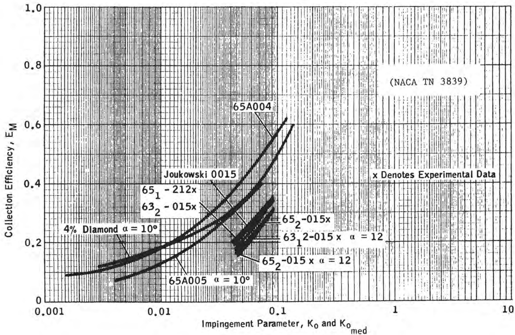
FIGURE 2-19. COLLECTION EFFICIENCY VERSUS K_0 FOR AIRFOILS - EXPERIMENTAL DATA FOR 8^\circ ANGLE OF ATTACK
