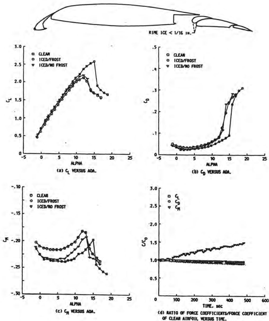
FIGURE 2-104. ICE SHAPE TRACING AND FORCE BALANCE MEASUREMENTS FOR EIGHT MINUTE ICING ENCOUNTER WITH T = 17^\circ\text{F} , \text{LWC} = .42 \text{ G/M}^3 , \text{MVD} = 13.4 \mu\text{m} , V = 158 \text{ FT/S} AND \alpha = 5^\circ FOR 5^\circ FLAP CONFIGURATION (REFERENCE 2-76)
