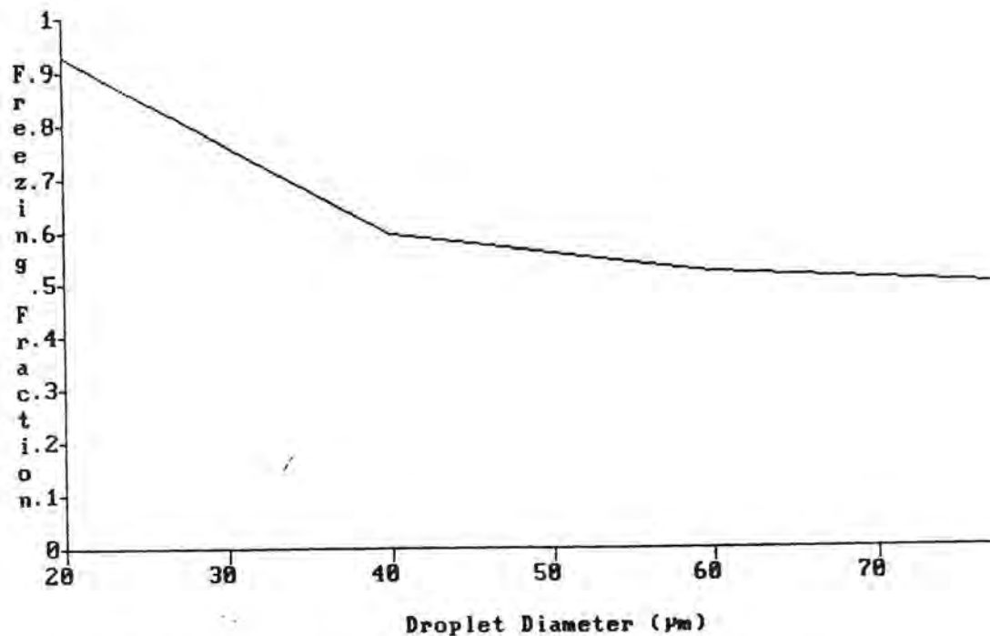
FIGURE 2-77. FREEZING FRACTION VS DROPLET DIAMETER \delta FOR A CIRCULAR CYLINDER WITH DIAMETER 20 CM
