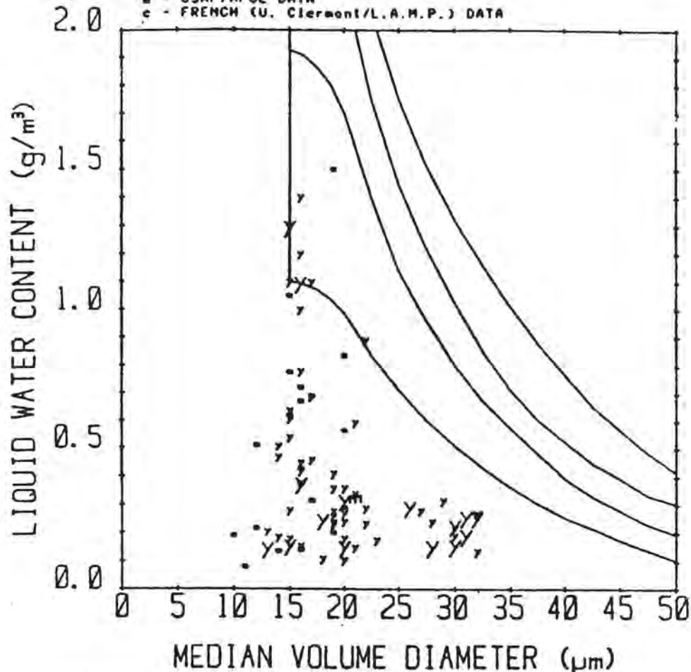
FIGURE 1-15. SCATTERPLOT OF OBSERVED LWC, MVD COMBINATIONS IN THE MODERN DATA FOR CONVECTIVE CLOUDS UP TO 10,000 FEET AGL AND FOR CLOUD TEMPERATURES FROM -4 TO 14 DEGREES FAHRENHEIT. The various plotting symbols represent various data sources as indicated in the key. The size of each plotted symbol is proportional to its weight (i.e., the observed horizontal extent of the associated icing event) as shown by the scale above the graph. The center of each plotted symbol corresponds to the average (and approximately constant) value of LWC and MVD observed during the icing event. Values of LWC for which no MVD measurements are available are plotted arbitrarily at 1 micron MVD. A total of 244 data miles is represented in this graph. The Intermittent Maximum envelope from Figure 4 of FAR-25, Appendix C, is superimposed for comparison. (Reference 1-20.)
