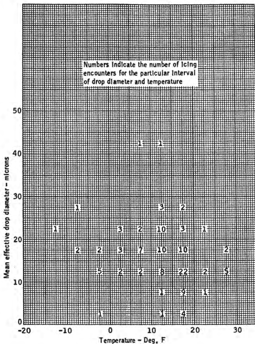
FIGURE 1-26. DROPLET DIAMETER VERSUS TEMPERATURE - CUMULUS CLOUDS (REFERENCE 1-5)
