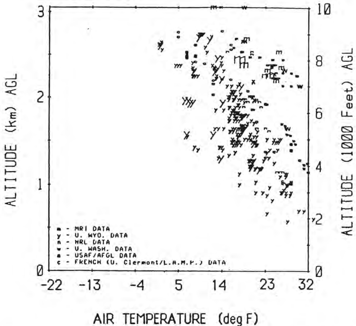
FIGURE 1-16. SCATTERPLOT OF ICING EVENT TEMPERATURES VS. ALTITUDE FOR MODERN DATA FROM SUPERCOOLED CONVECTIVE CLOUDS UP TO 10,000 FEET AGL. The various plotting symbols represent various data sources as indicated in the key. The size of each symbol is proportional to its statistical weight (i.e., the observed horizontal extent of the associated icing event) as shown by the scale above the graph. The center of each plotted symbol corresponds to the average (and approximately constant) value of altitude and OAT observed during the icing event. A total of 980 data miles is represented in this graph. (Reference 1-20.)
