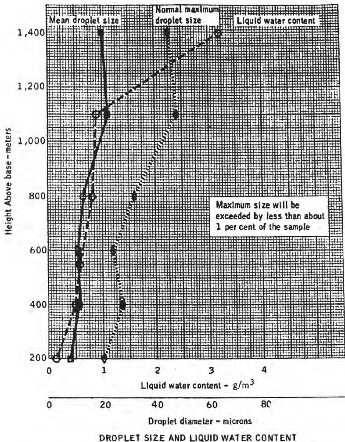
FIGURE 1-13. PROPERTIES OF TYPICAL CUMULUS CONGESTUS CLOUDS - LWC, DROP SIZE, TEMPERATURE, VERTICAL AND HORIZONTAL DIMENSIONS (REFERENCE 1-21)
