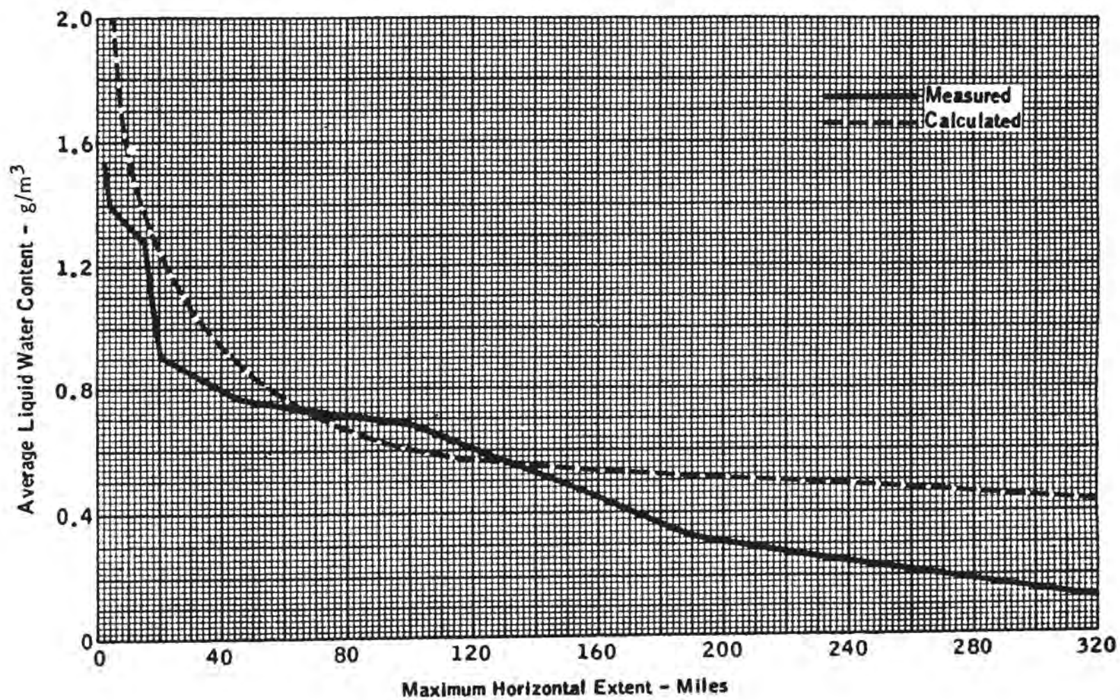
FIGURE 1-30. LWC VERSUS HORIZONTAL EXTENT (REFERENCE 1-9)
