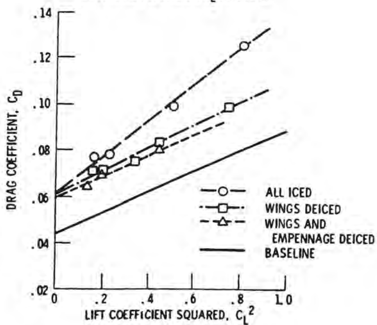
(b) Shift in aircraft drag polar,
