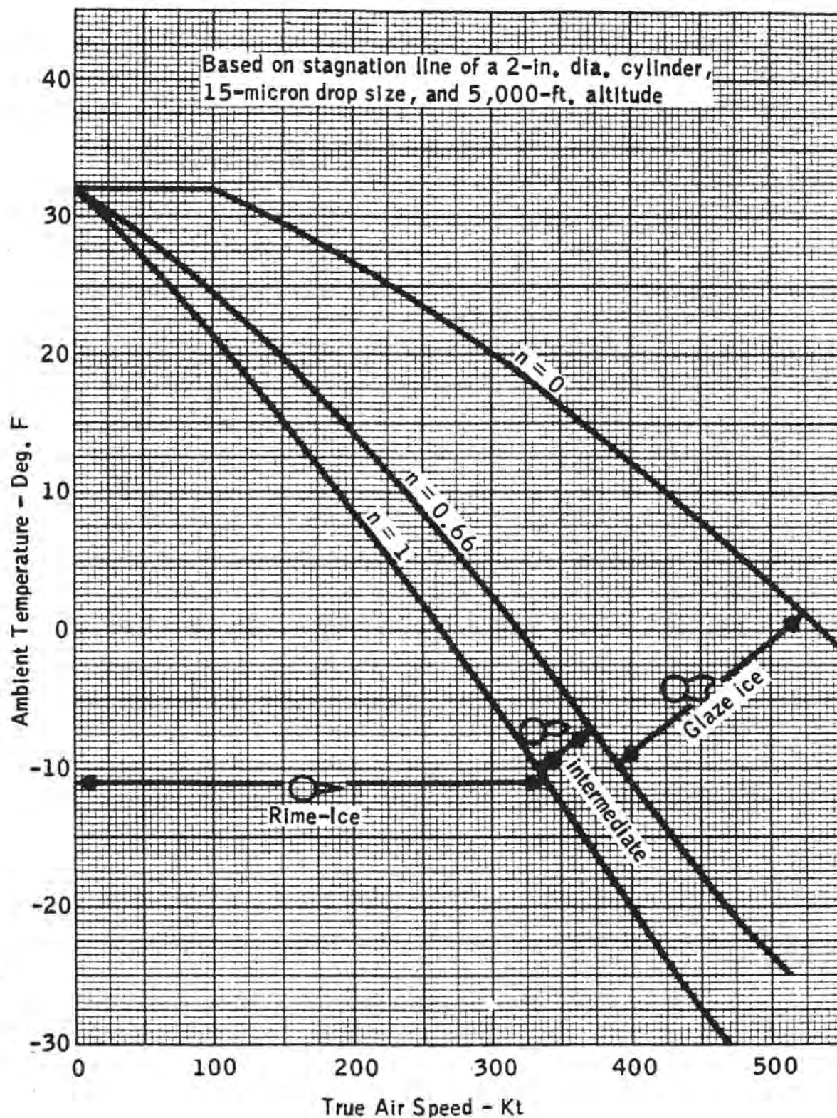
FIGURE 2-81. ICE SHAPE TYPES AS A FUNCTION OF SPEED AND AMBIENT TEMPERATURE FOR A LIQUID WATER CONTENT OF 0.2 \text{ G/M}^3 (REFERENCE 2-49)
