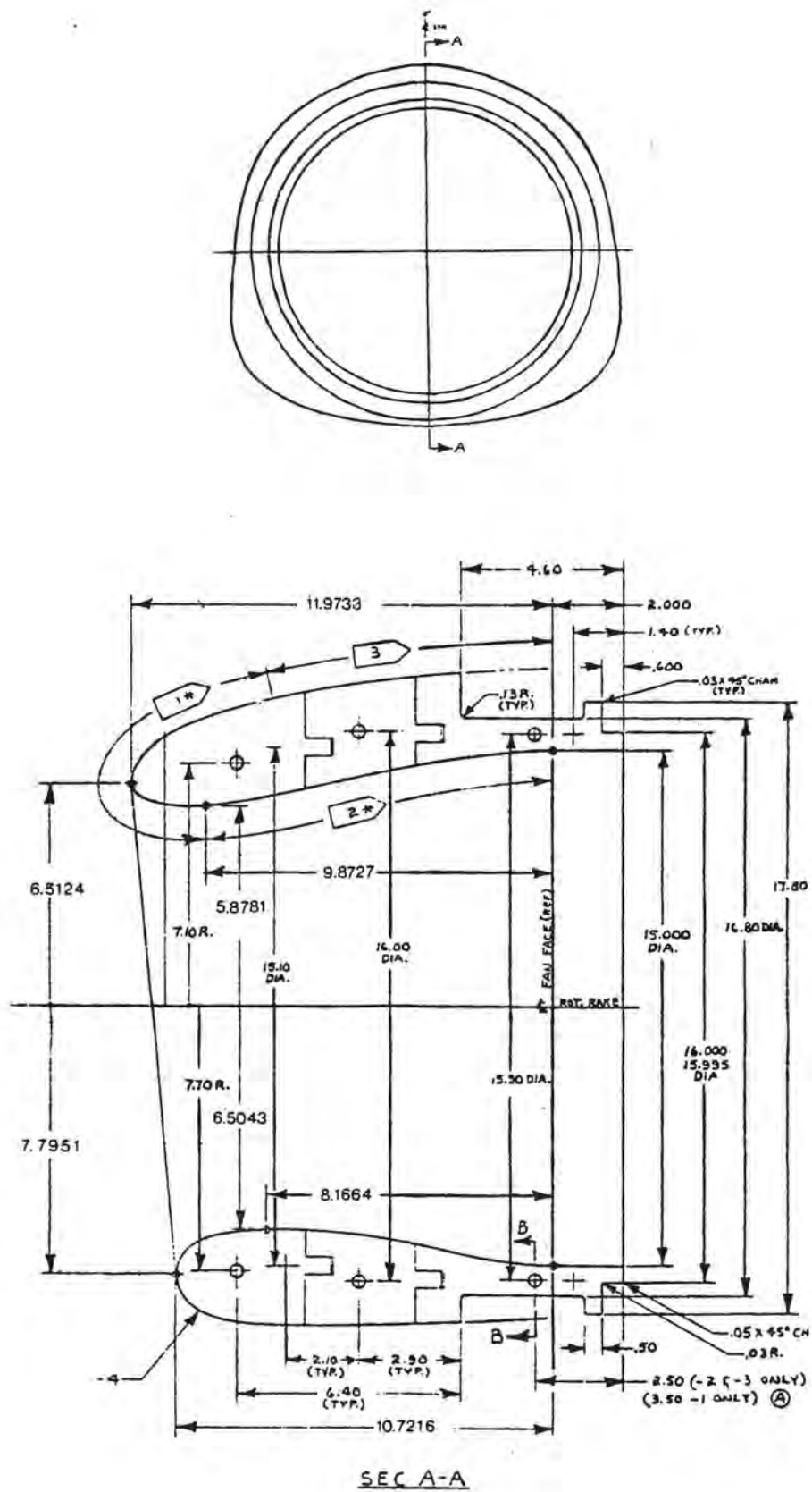
FIGURE 2-31. BOEING 737-300 INLET (REFERENCE 2-15)
