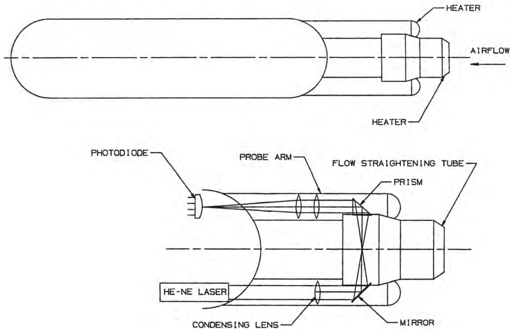
FIGURE 2-8. FORWARD SCATTERING SPECTROMETER PROBE (FSSP)
