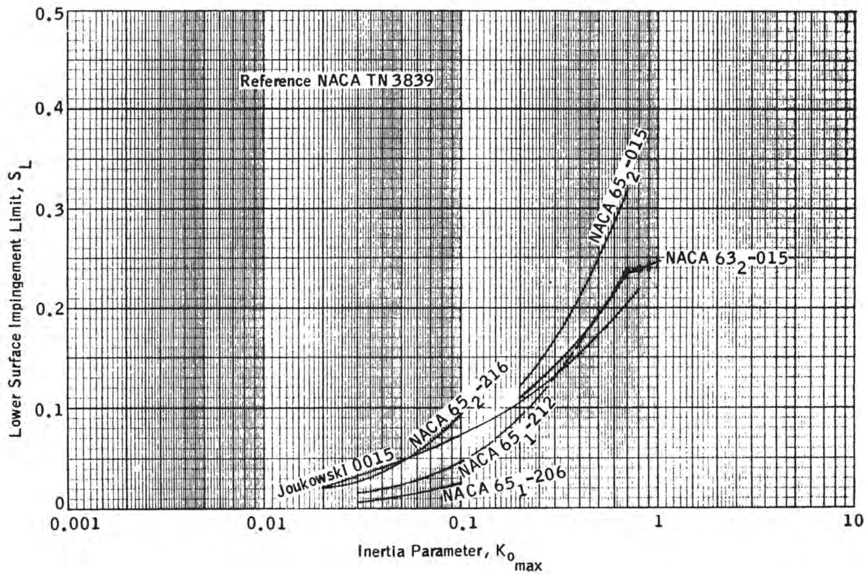
FIGURE 2-22. LOWER SURFACE IMPINGEMENT LIMITS FOR SEVERAL AIRFOILS AT 0^\circ ANGLE OF ATTACK (EXPERIMENTAL DATA)
