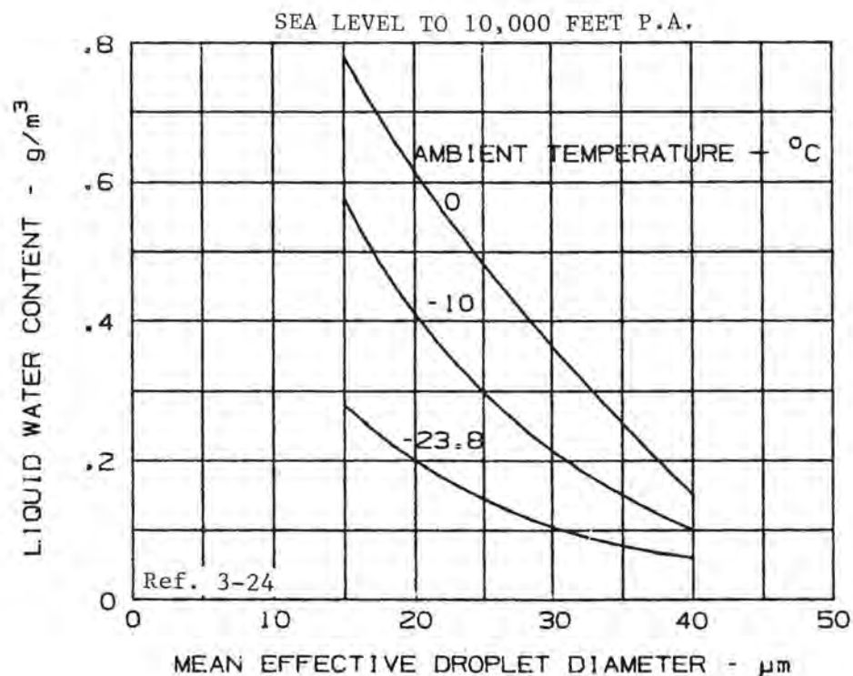
FIGURE 3-12. FAA ALTITUDE LIMITED ENVELOPE FOR CONTINUOUS ICING CONDITIONS
