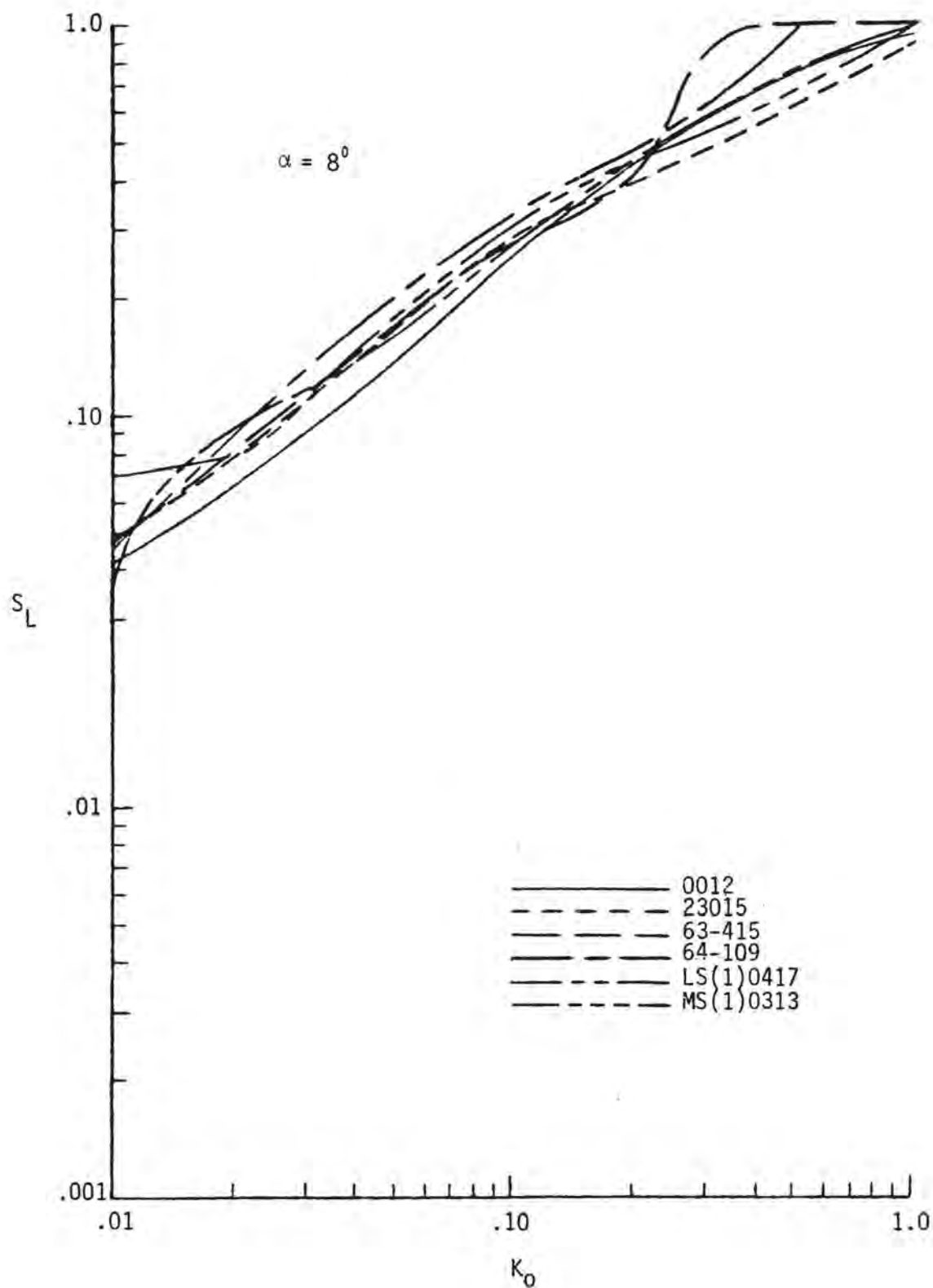
FIGURE 2-56. THEORETICAL DATA ON THE LOWER SURFACE IMPINGEMENT LIMIT OF SEVERAL AIRFOILS ( \alpha = 8^\circ )
