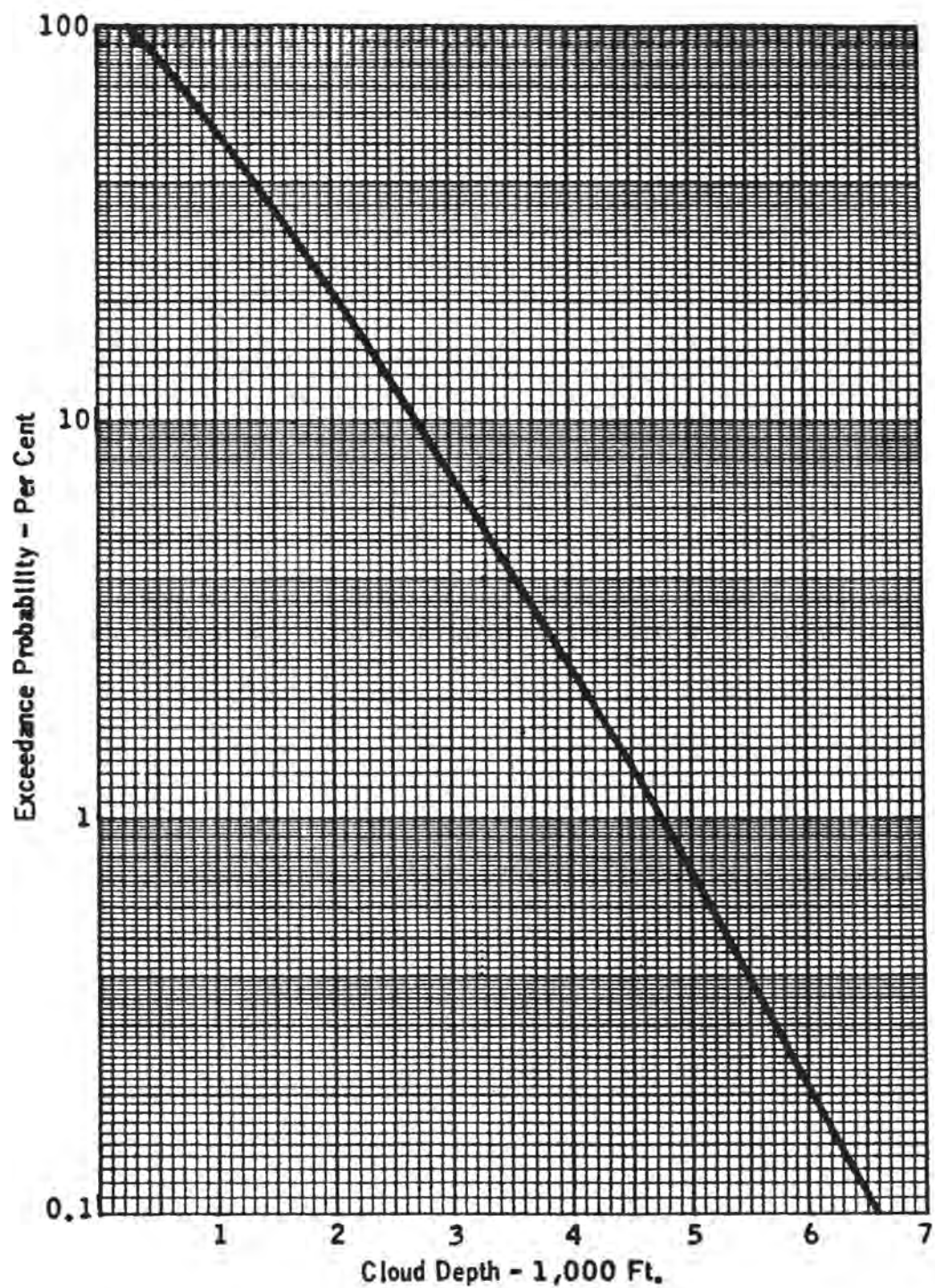
FIGURE 1-35. CLOUD DEPTH PROBABILITY FOR LAYER TYPE CLOUDS (REFERENCE 1-16)
