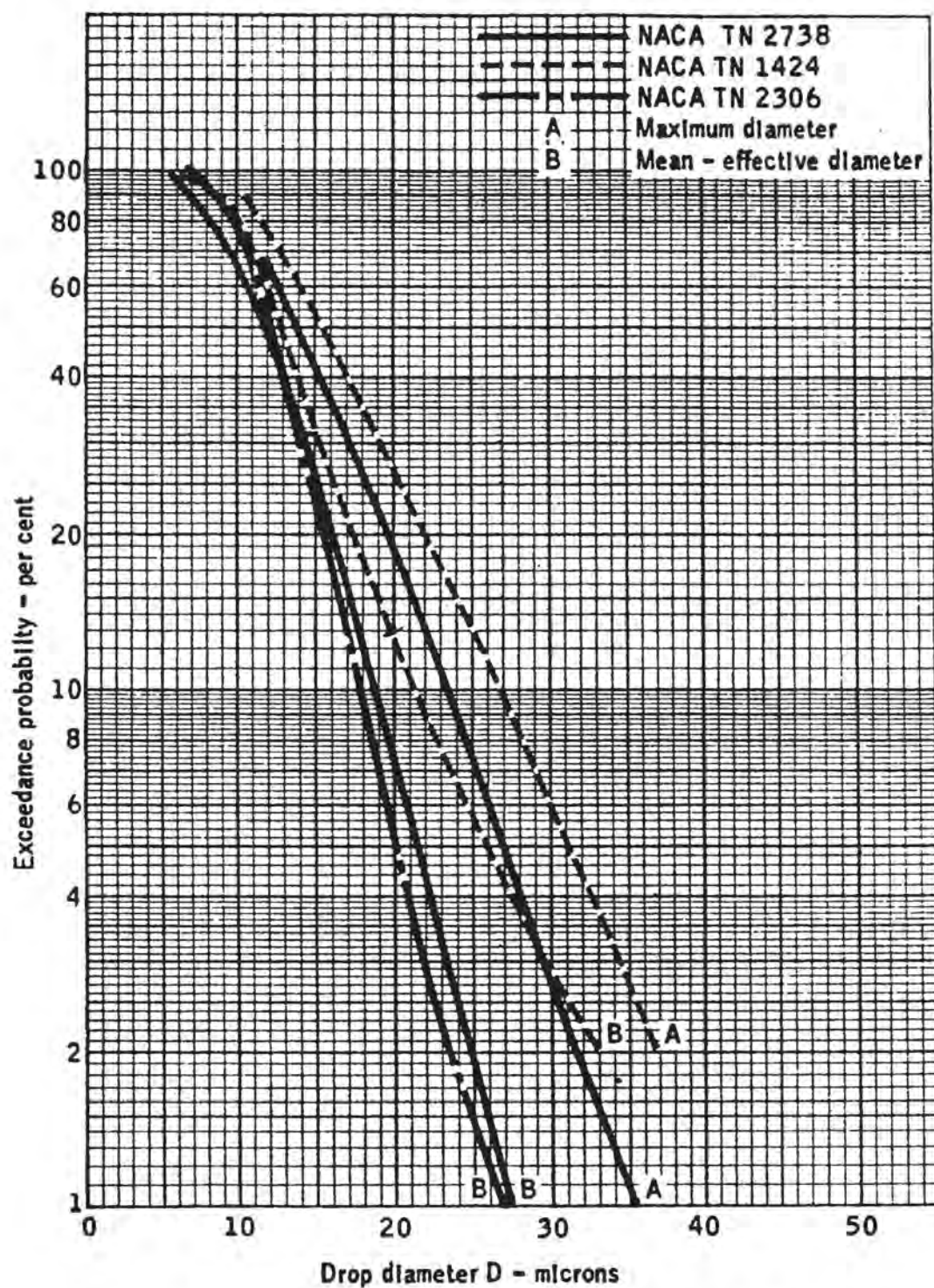
FIGURE 1-28. EXCEEDANCE PROBABILITY FOR DROP DIAMETER (REFERENCES 1-6, 1-10 AND 1-11)
