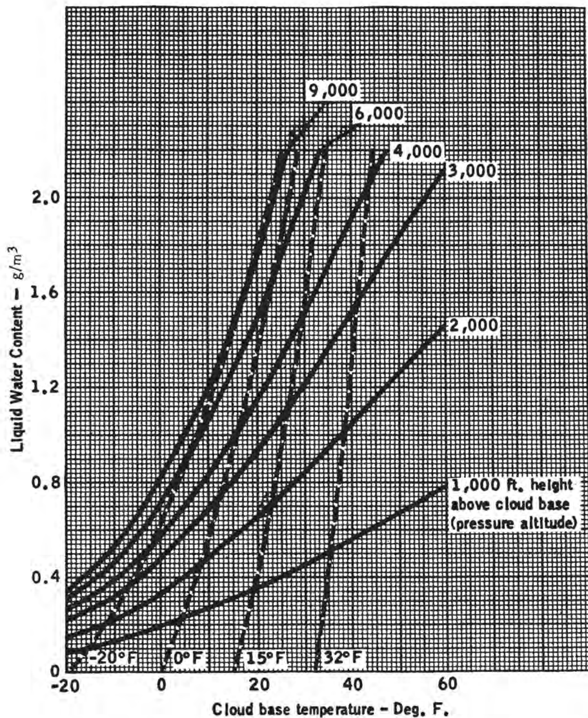
FIGURE 1-2. THEORETICAL LIQUID WATER CONCENTRATION IN CLOUDS FORMED BY ADIABATIC LIFTING (CLOUD BASE AT 948 FT. PRESSURE ALTITUDE).
