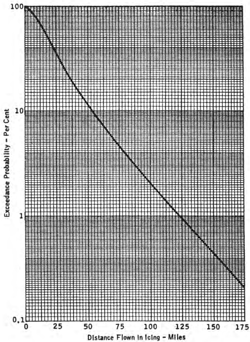
FIGURE 1-32. PROBABILITY CURVE OF DISTANCE FLOWN IN ICING (REFERENCE 1-16)
