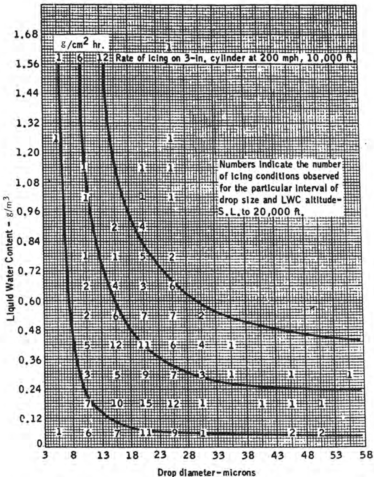
FIGURE 3-7. CUMULIFORM CLOUDS - LWC VERSUS DROP DIAMETER (REFERENCE 3-12)
