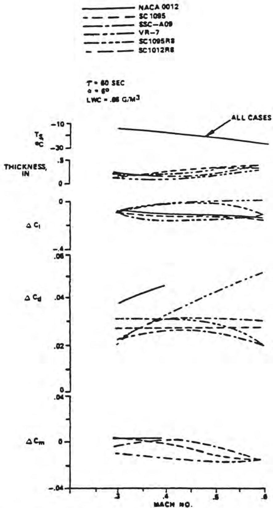
FIGURE 2-111. EFFECT OF MACH NUMBER ON ROTOR AIRFOIL PERFORMANCE
