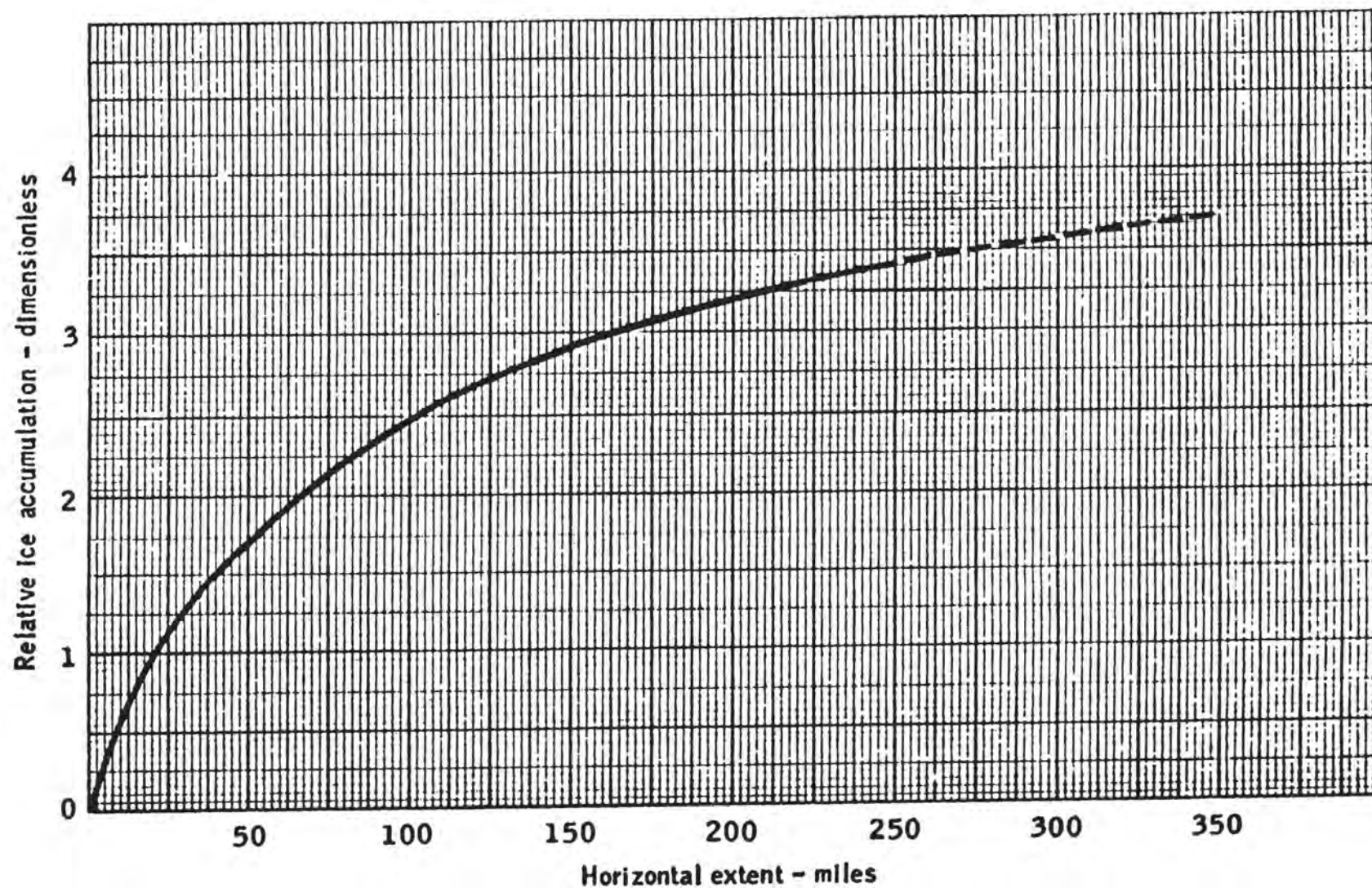
FIGURE 3-10. PLOT OF RELATIVE AMOUNT OF ICE ACCUMULATION FOR VARIOUS FLIGHT DISTANCES IN CONTINUOUS MAXIMUM ICING (BASED UPON A 20-MILE STANDARD DISTANCE AND THE DATA OF REFERENCE 3-36)
