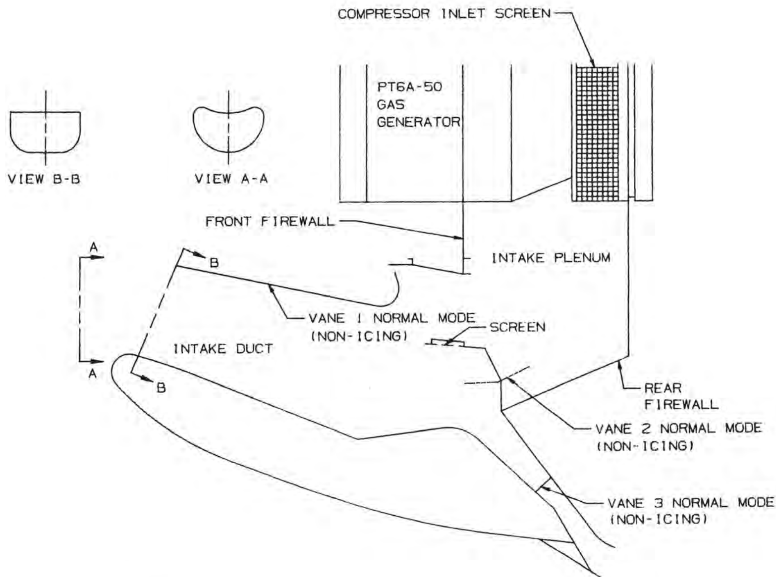
FIGURE 2-106a. PT6A-50 ANTI-ICING CONFIGURATION INERTIAL SEPARATION SYSTEM
