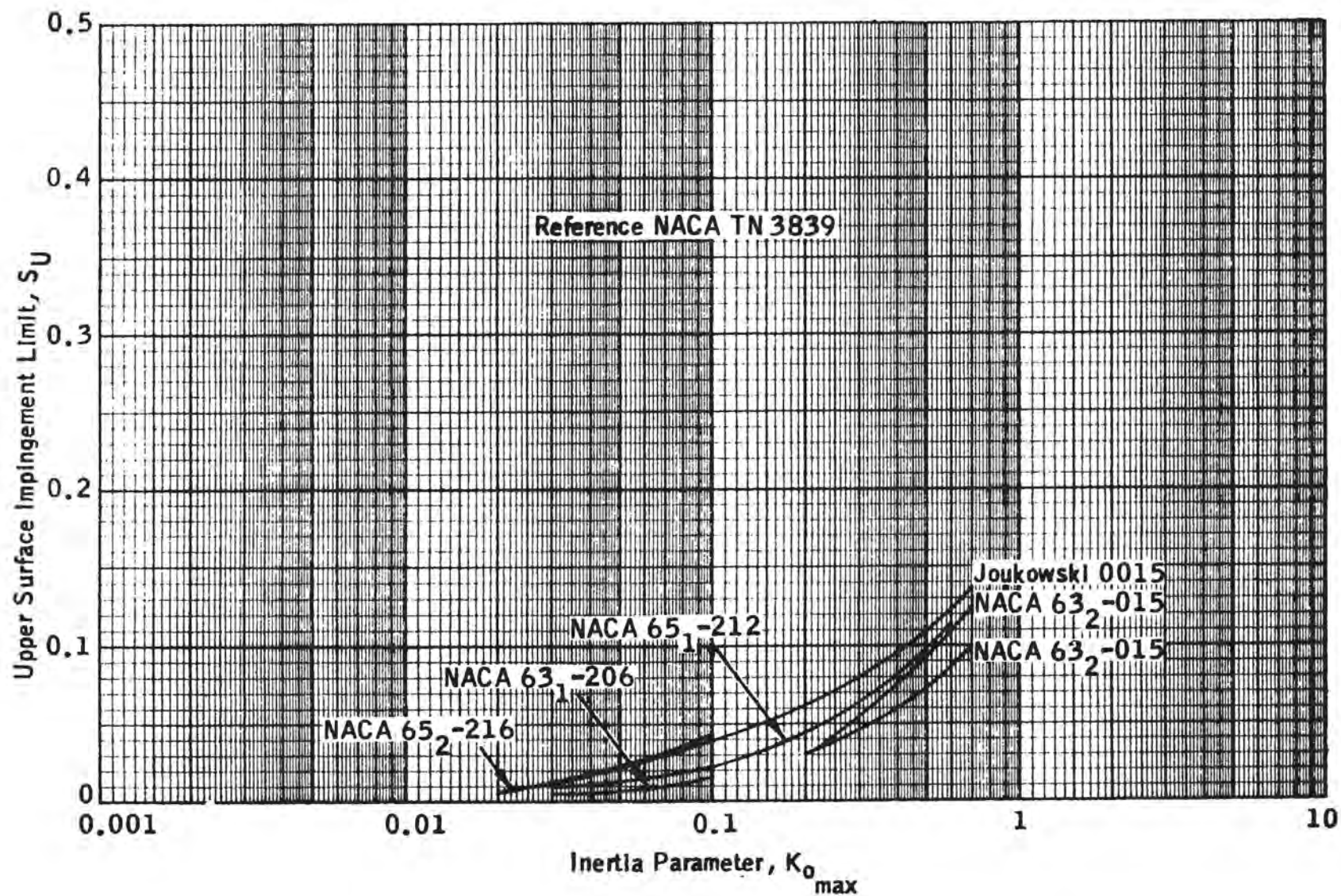
FIGURE 2-23. UPPER SURFACE IMPINGEMENT LIMITS FOR SEVERAL AIRFOILS AT 4° ANGLE OF ATTACK (EXPERIMENTAL DATA)
