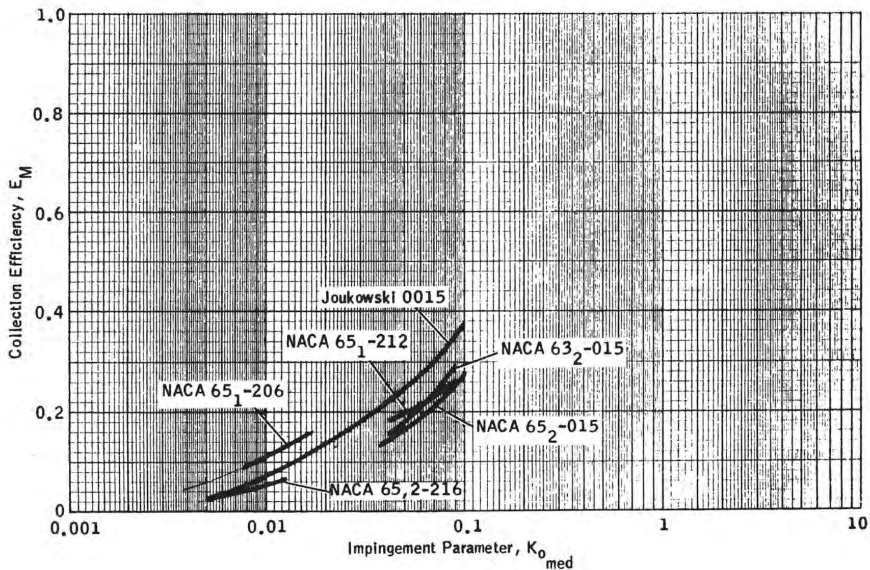
FIGURE 2-17. COLLECTION EFFICIENCY VERSUS K_{0_{med}} FOR AIRFOILS - EXPERIMENTAL DATA AT 0° ANGLE OF ATTACK
