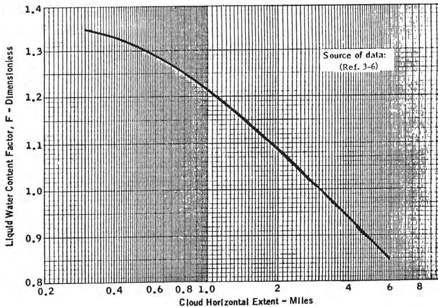
FIGURE 3-9. INTERMITTENT MAXIMUM ATMOSPHERIC ICING CONDITIONS - CUMULIFORM CLOUDS. VARIATION OF LWC FACTOR WITH CLOUD HORIZONTAL DISTANCE EXTENT (REFERENCE 3-2)
