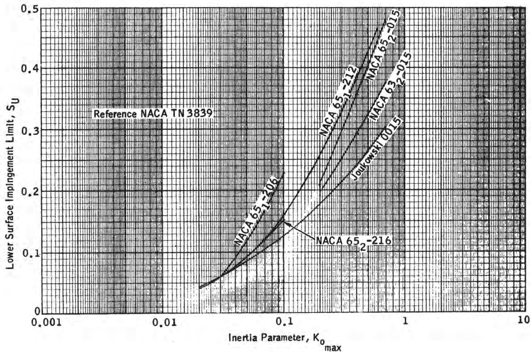
FIGURE 2-24. LOWER SURFACE IMPINGEMENT LIMITS FOR SEVERAL AIRFOILS AT 4° ANGLE OF ATTACK (EXPERIMENTAL DATA)
