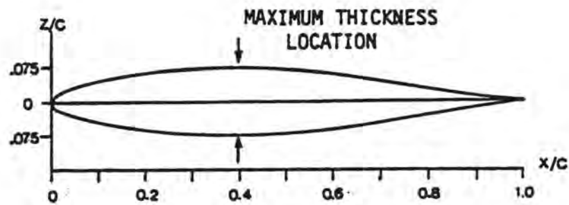
(B) 652015 AIRFOIL
