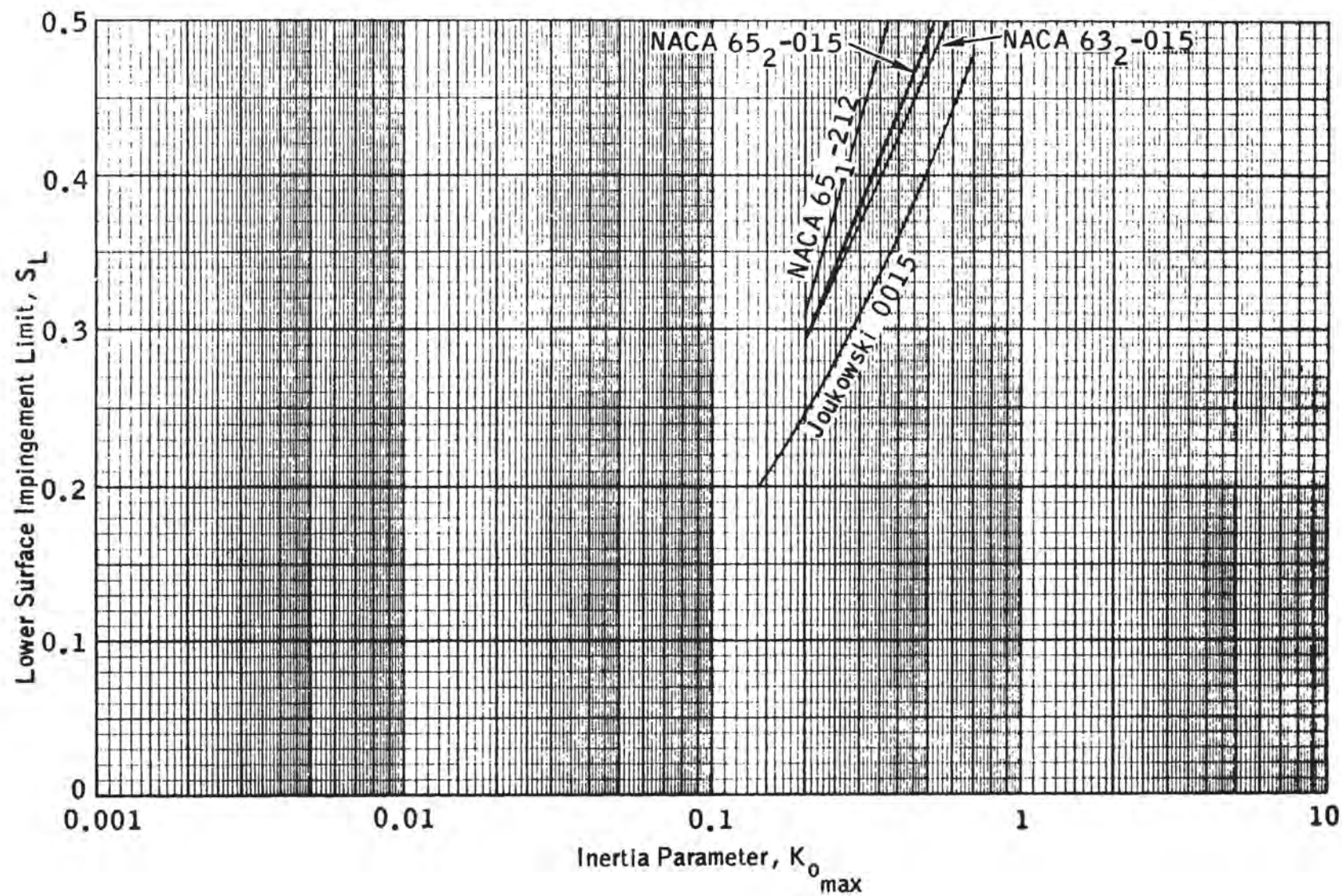
FIGURE 2-26. LOWER SURFACE IMPINGEMENT LIMITS FOR SEVERAL AIRFOILS AT 8° ANGLE OF ATTACK (EXPERIMENTAL DATA)
