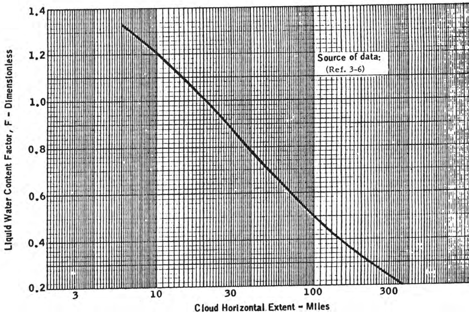
FIGURE 3-8. CONTINUOUS MAXIMUM ATMOSPHERIC ICING CONDITIONS - STRATIFORM CLOUDS. LWC FACTOR VERSUS CLOUD HORIZONTAL DISTANCE EXTENT (REFERENCE 3-2)
