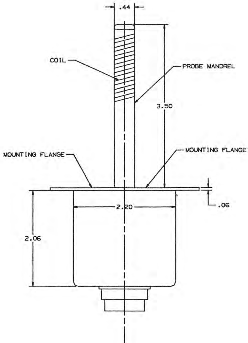
FIGURE 1-1. HOT WIRE ICE DETECTOR
