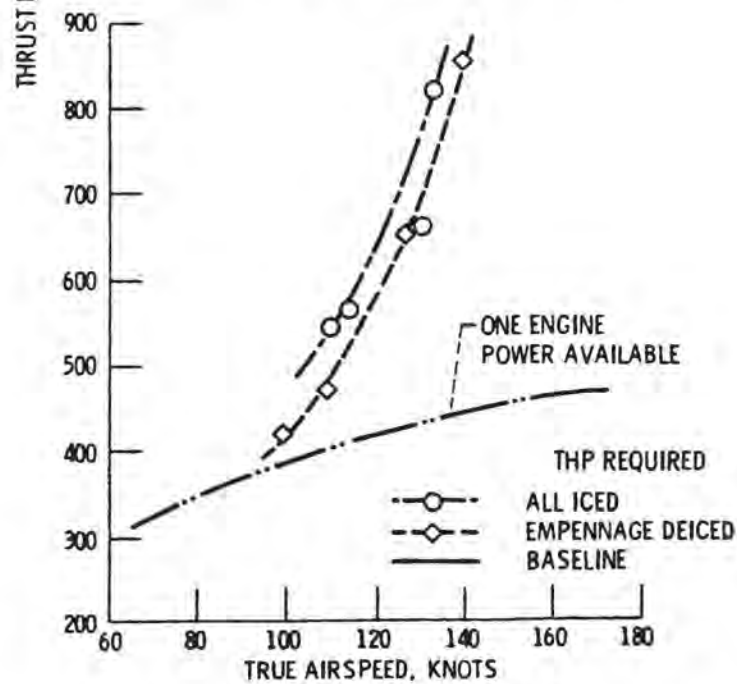
(b) Test conditions at 6000 ft. Flight test data corrected to standard weight only.
