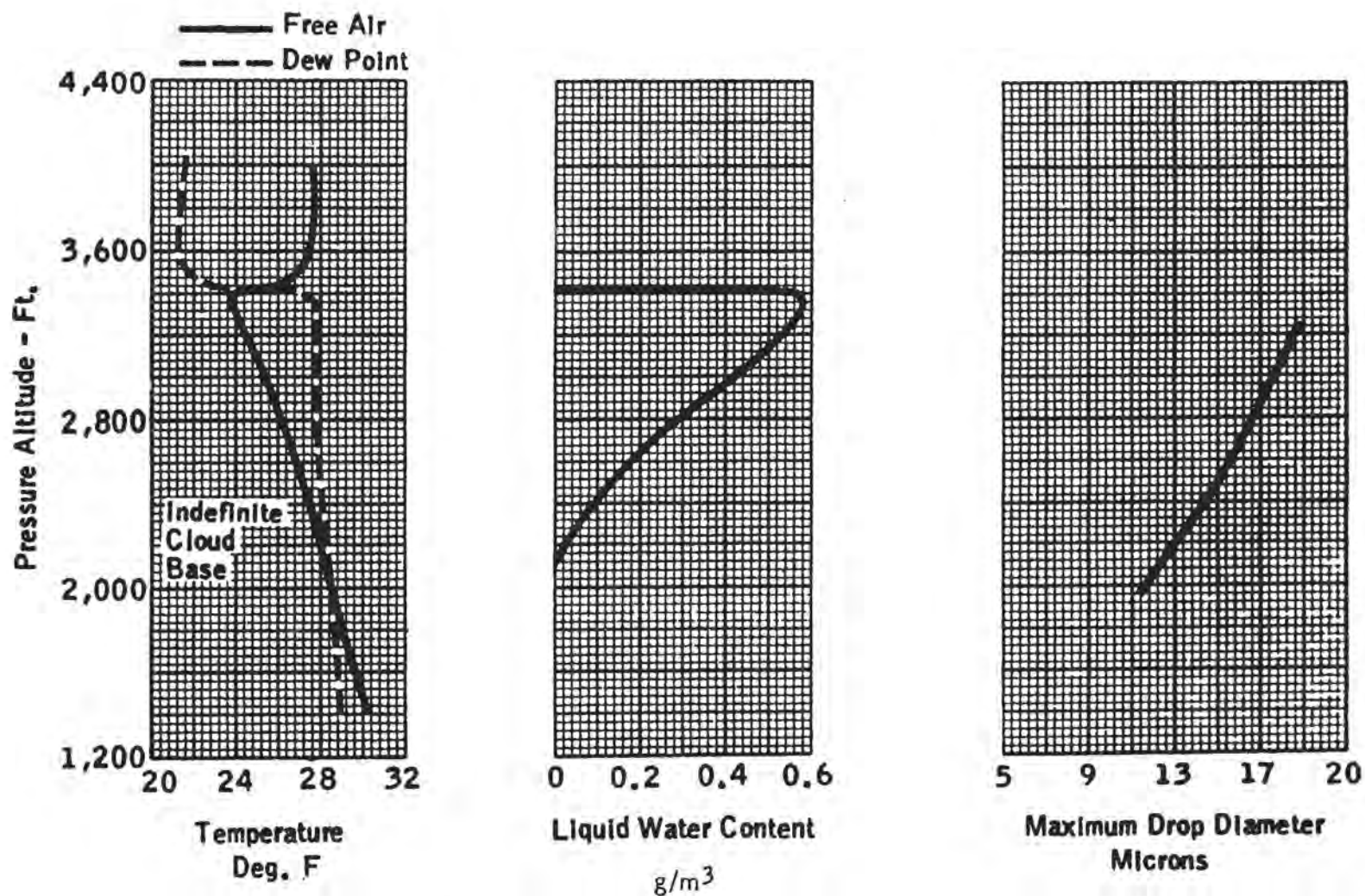
FIGURE 1-1. PROPERTIES OF A TYPICAL NON-CYCLONIC STRATUS CLOUD FROM FIGURE 3a. (REFERENCE 1-2)
