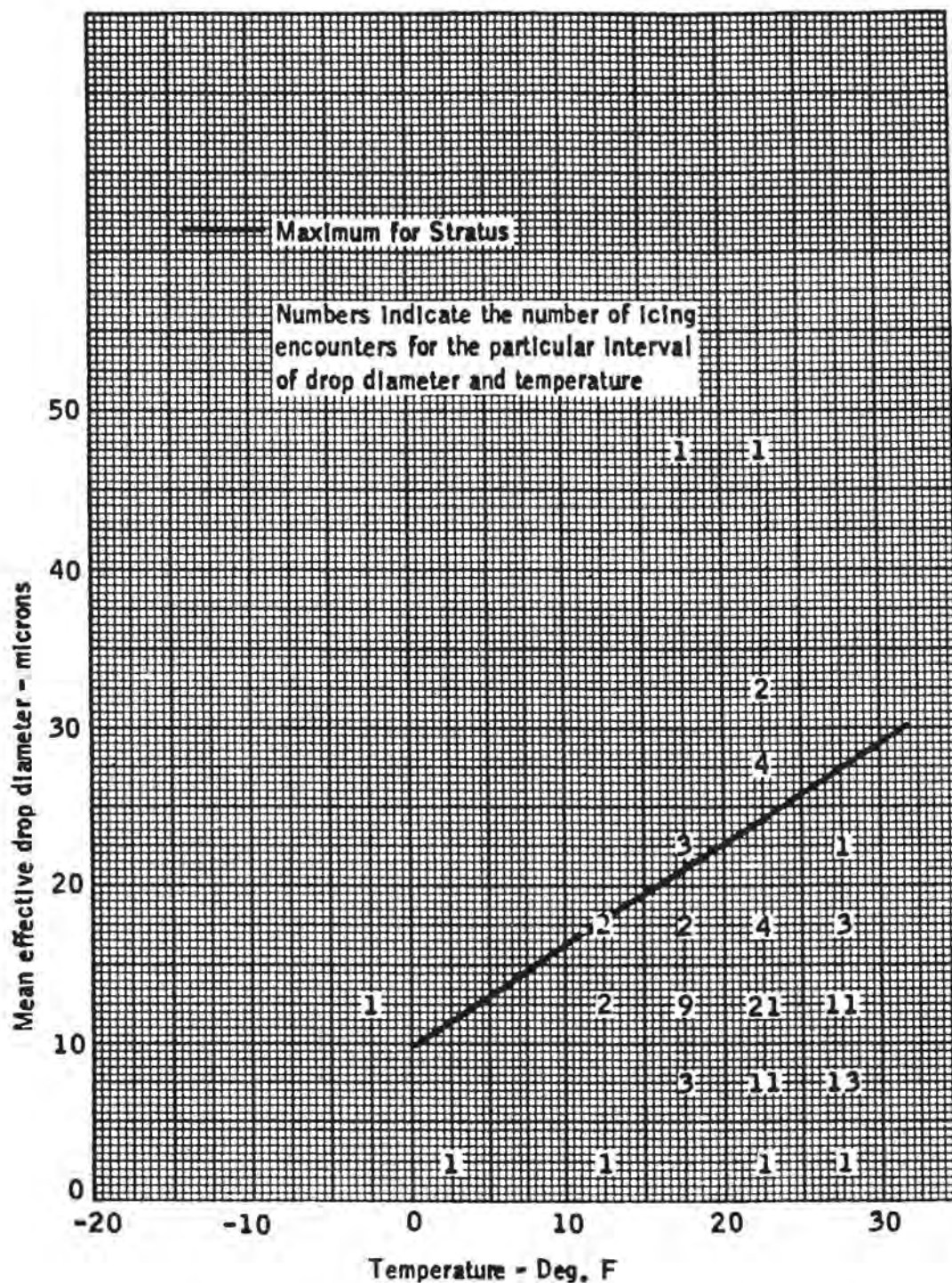
FIGURE 1-25. DROPLET DIAMETER VERSUS TEMPERATURE - STRATUS CLOUDS (REFERENCE 1-5)
