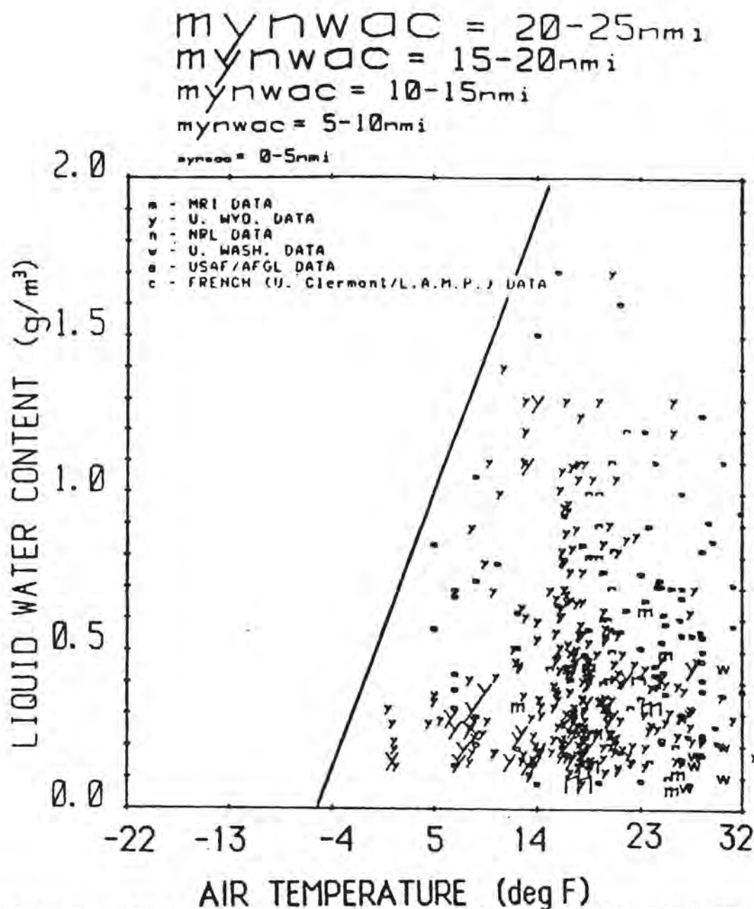
FIGURE 1-17. SCATTERPLOT OF LWC VS. OAT FOR MODERN DATA FROM SUPERCOOLED CONVECTIVE CLOUDS UP TO 10,000 FEET AGL. The various plotting symbols represent various data sources as indicated in the key. The size of each symbol is proportional to its statistical weight (i.e., the observed horizontal extent of the associated icing event) as shown by the scale above the graph. The center of each plotted symbol corresponds to the average (and approximately constant) value of LWC and OAT observed during the icing event. The solid line bounding the data points the apparent upper limit to LWC as a function of temperature for Continental U.S. supercooled convective clouds below 10,000 feet AGL. The position of the line is based on the maximum LWC values in the combined original data (presented in Reference 1-1) and modern data sets. A total of 980 data miles is represented in this graph. (Reference 1-20.)
