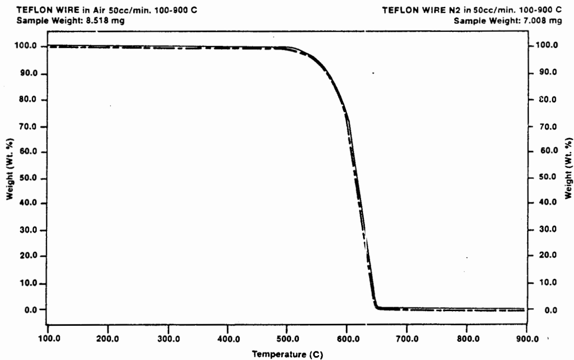
FIGURE 16. THERMOGRAVIMETRIC ANALYSIS--TEFLON
