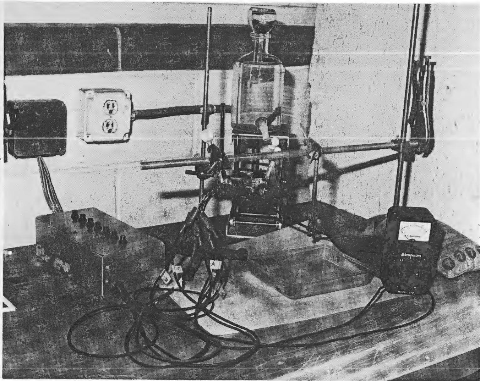
FIGURE 1. TEST DEVICE
