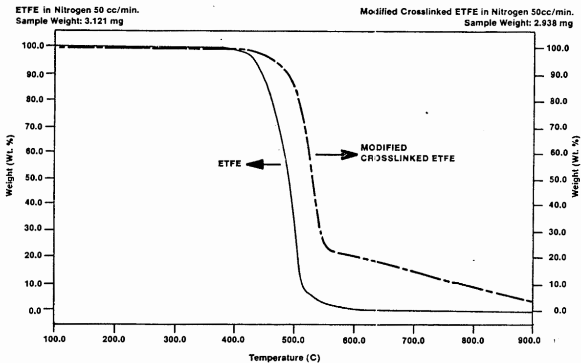
FIGURE 17. THERMOGRAVIMETRIC ANALYSIS--ETFE
