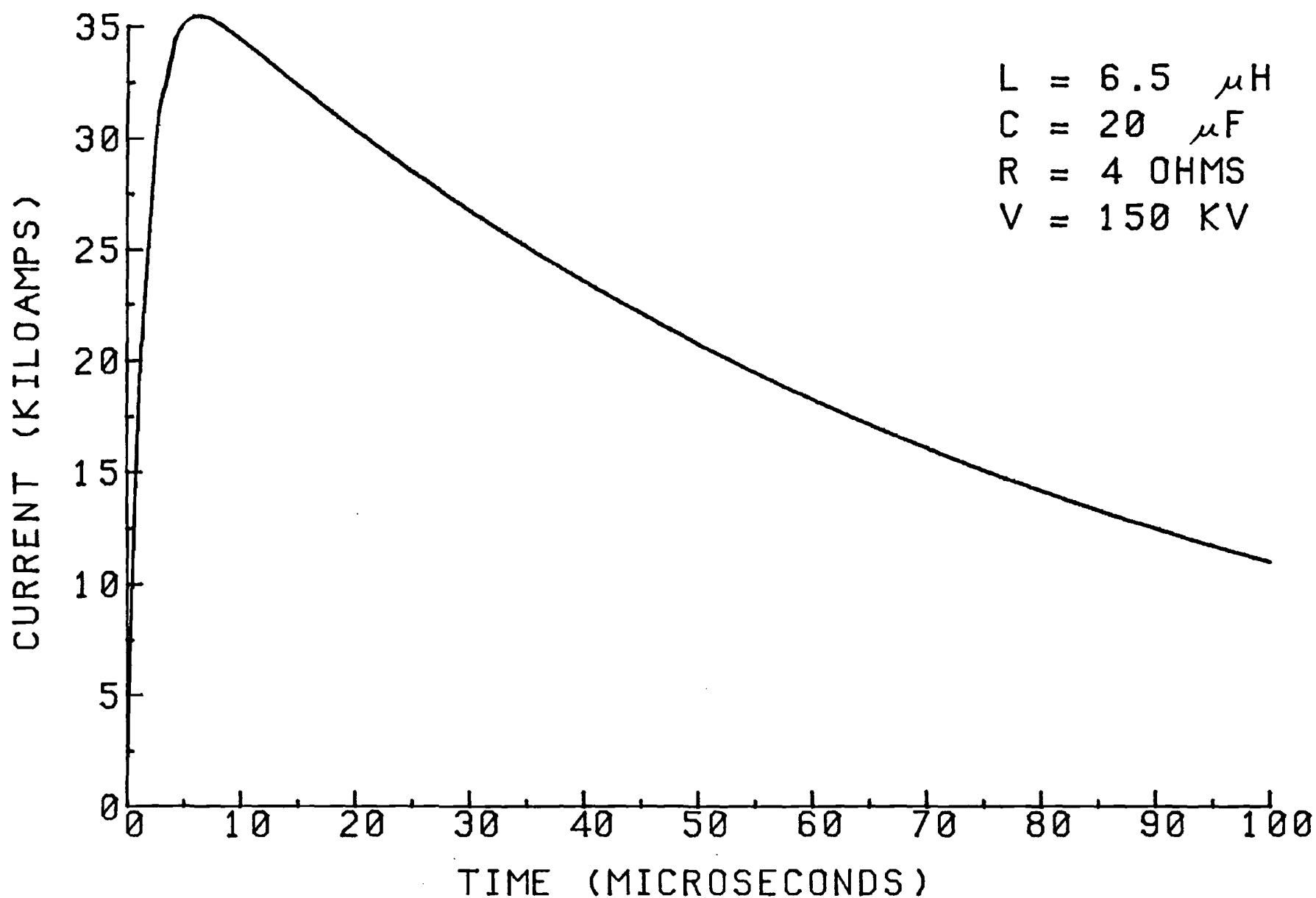
FIGURE 31 MODERATE-LEVEL PULSE CURRENT WAVEFORM WITH 20 MICROFARAD GENERATOR CAPACITY
