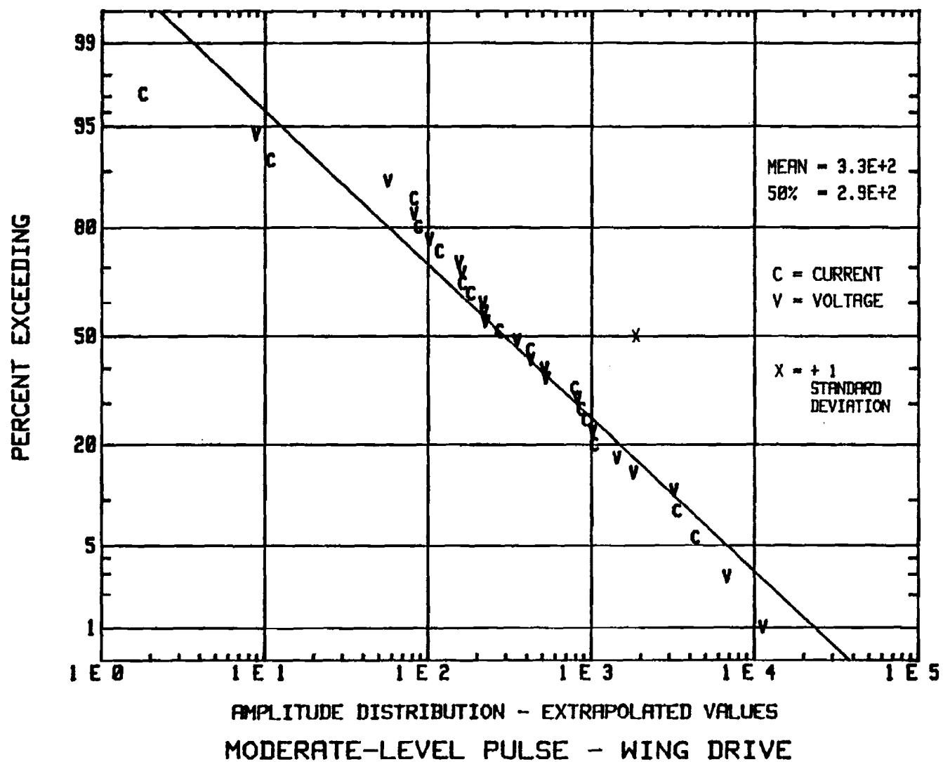
FIGURE 50 STATISTICAL DISTRIBUTION OF MODERATE-LEVEL PULSE EXTRAPOLATED VALUES WING DRIVE
