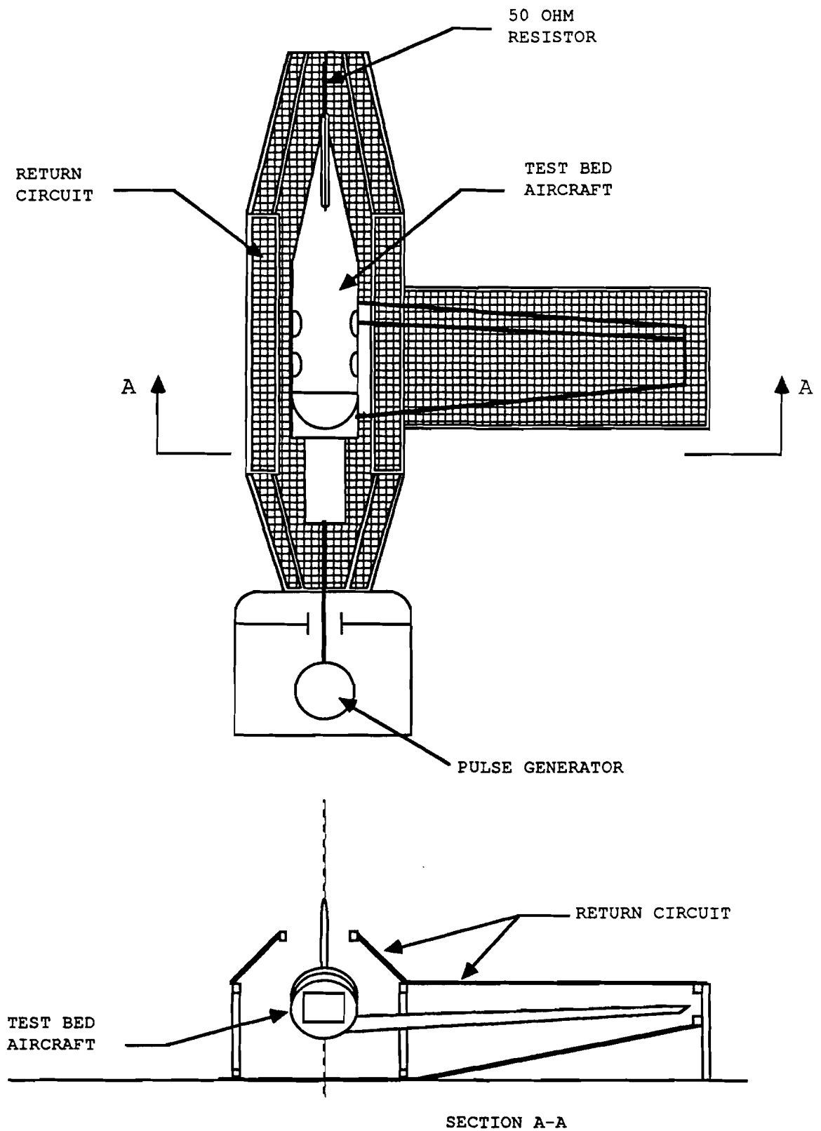
FIGURE 5 LOW-LEVEL FAST-RISE PULSE TEST SETUP
