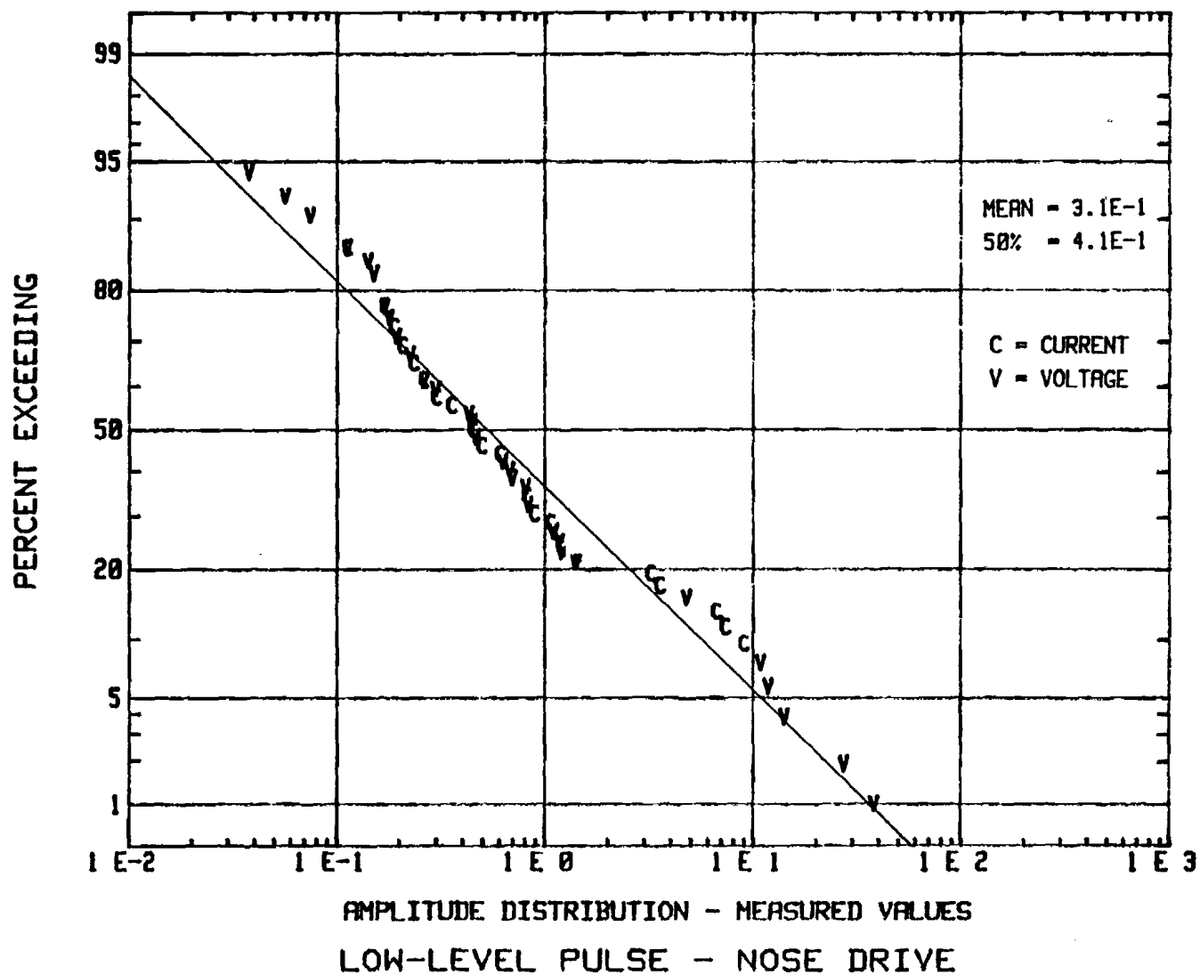
FIGURE 52 STATISTICAL DISTRIBUTION OF LOW-LEVEL PULSE MEASURED VALUES NOSE DRIVE
