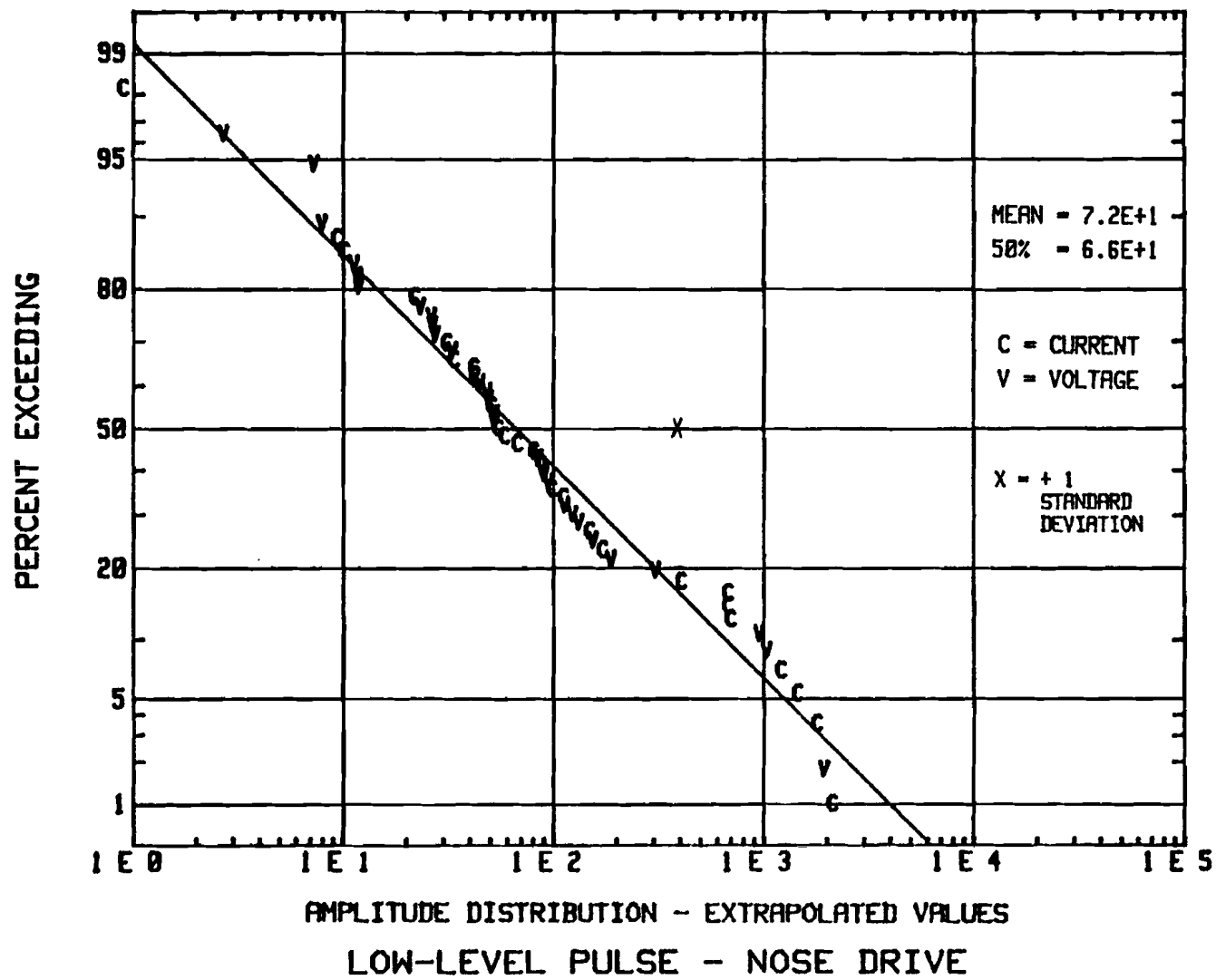
FIGURE 45 STATISTICAL DISTRIBUTION OF LOW-LEVEL PULSE EXTRAPOLATED VALUES NOSE DRIVE
