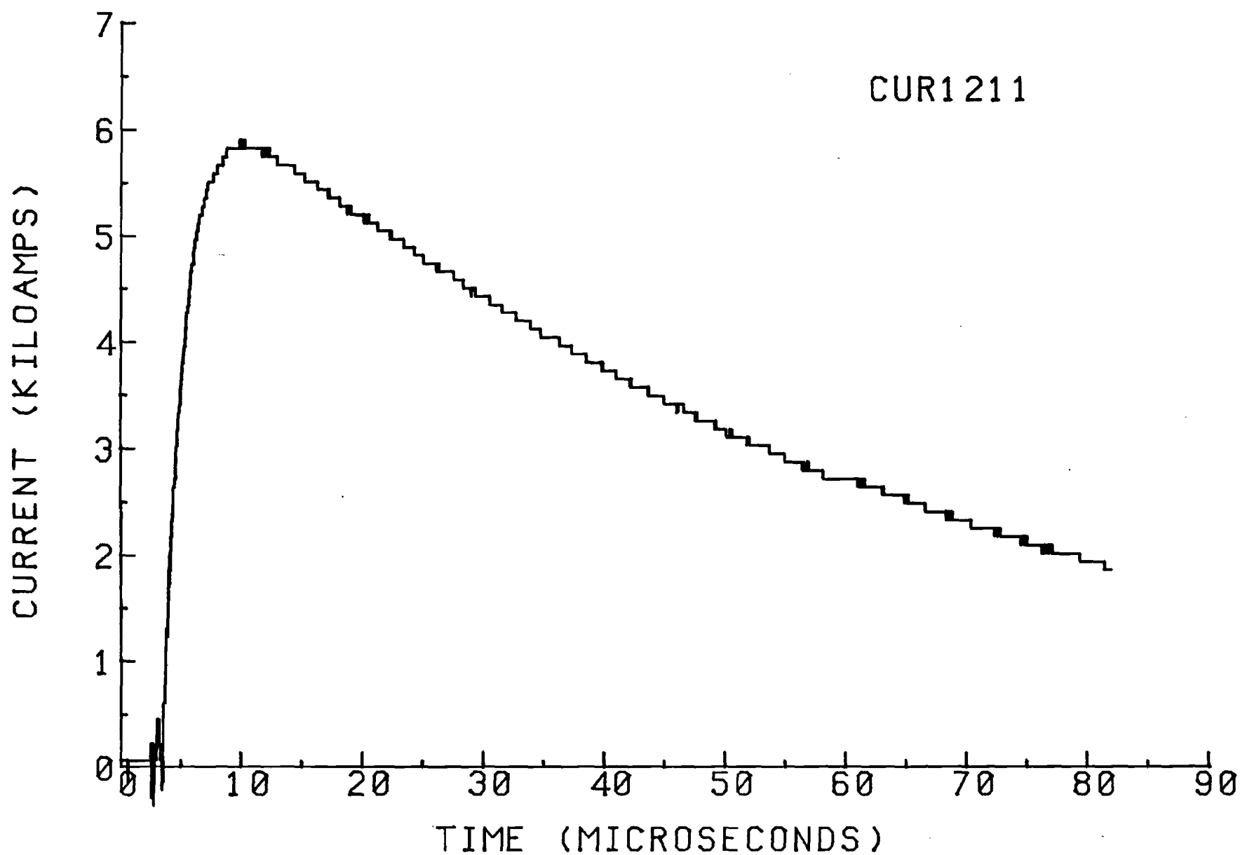
FIGURE 33 EXAMPLE SHOCK-EXCITATION CURRENT WAVEFORM
