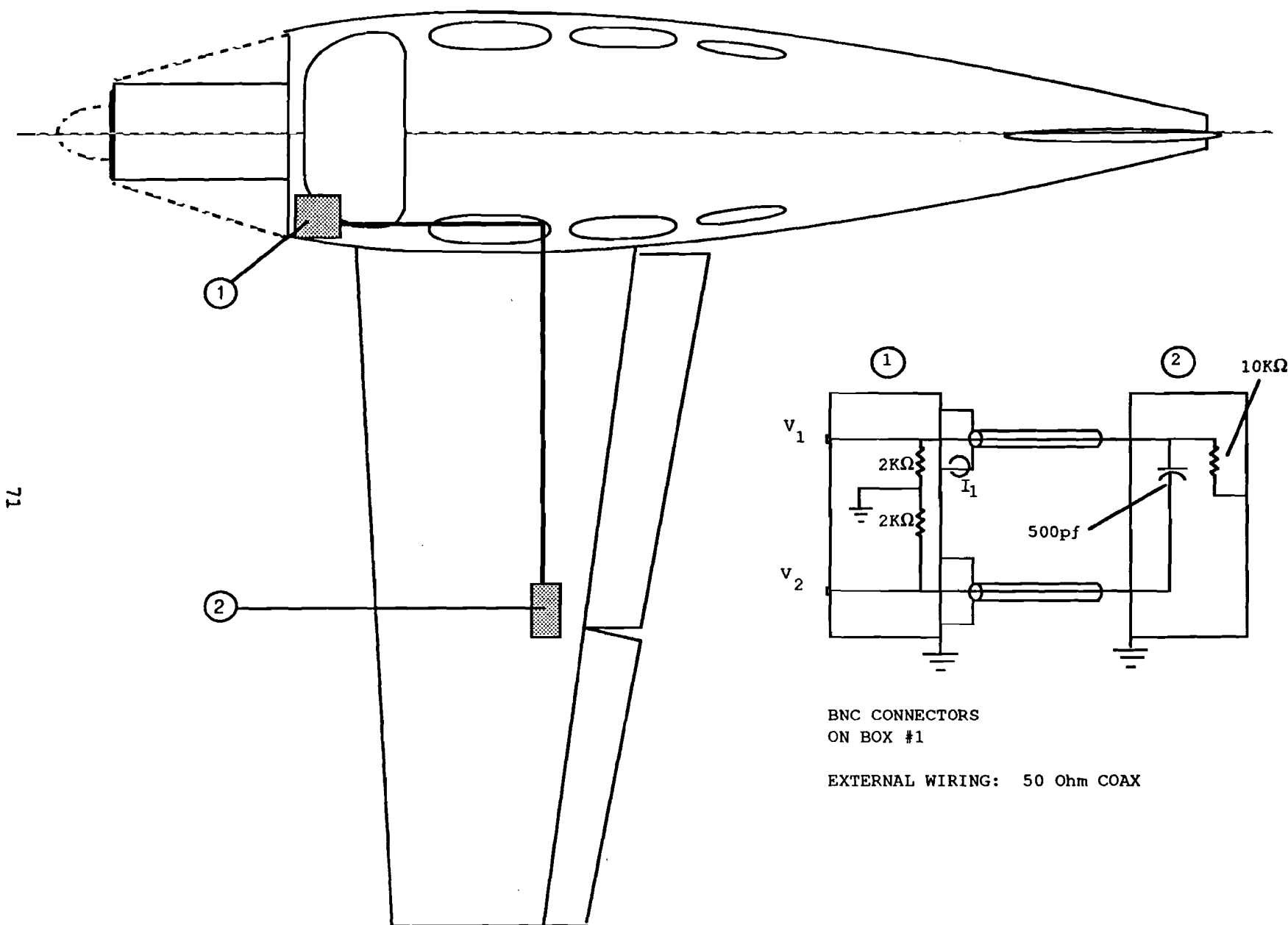
FIGURE 19 FUEL SYSTEM ELECTRICAL INSTALLATION AND CIRCUIT DETAIL
