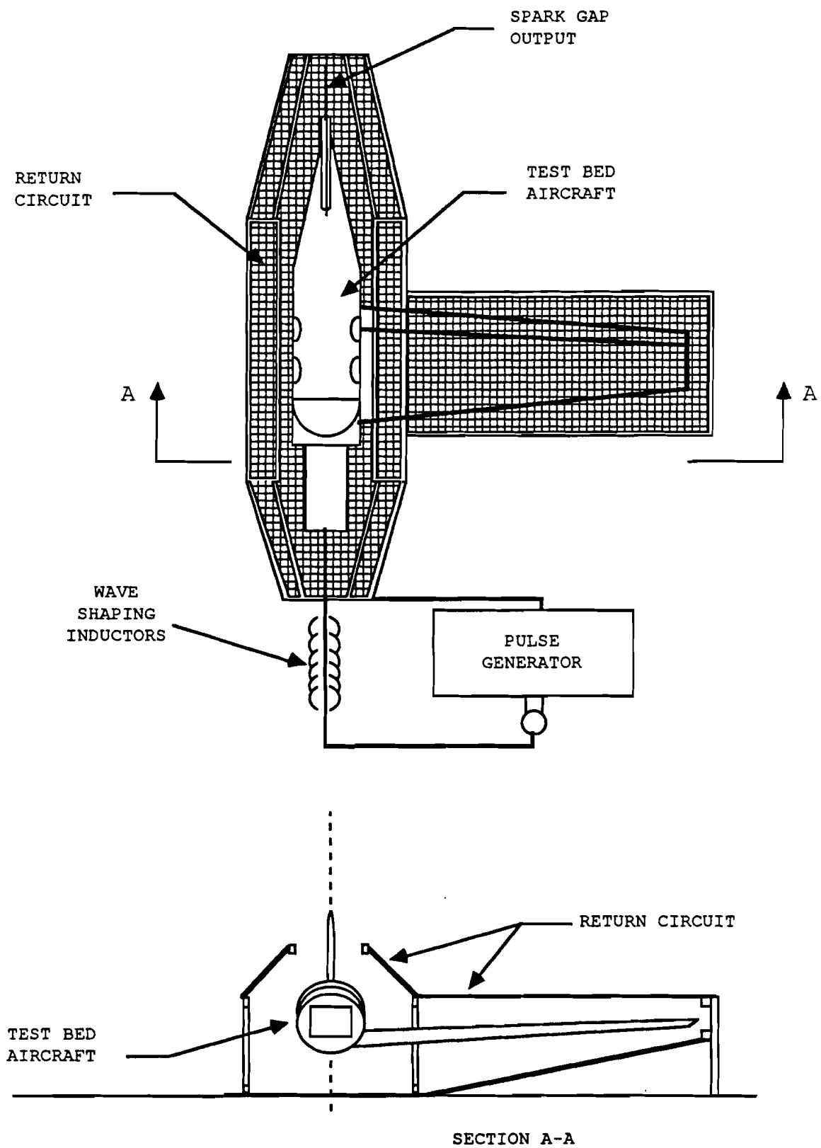
FIGURE 7 SHOCK-EXCITED TEST SETUP
