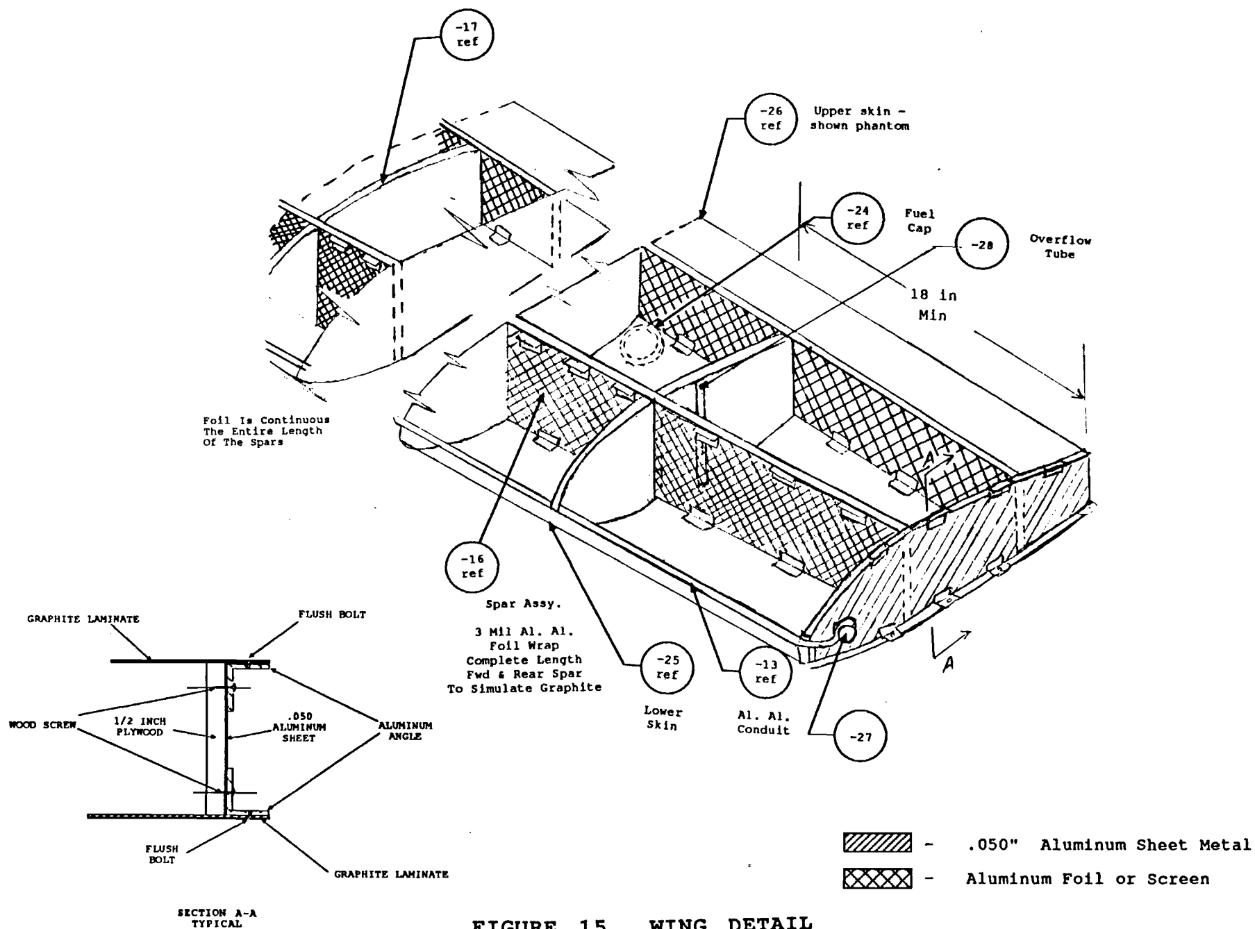
FIGURE 15 WING DETAIL
