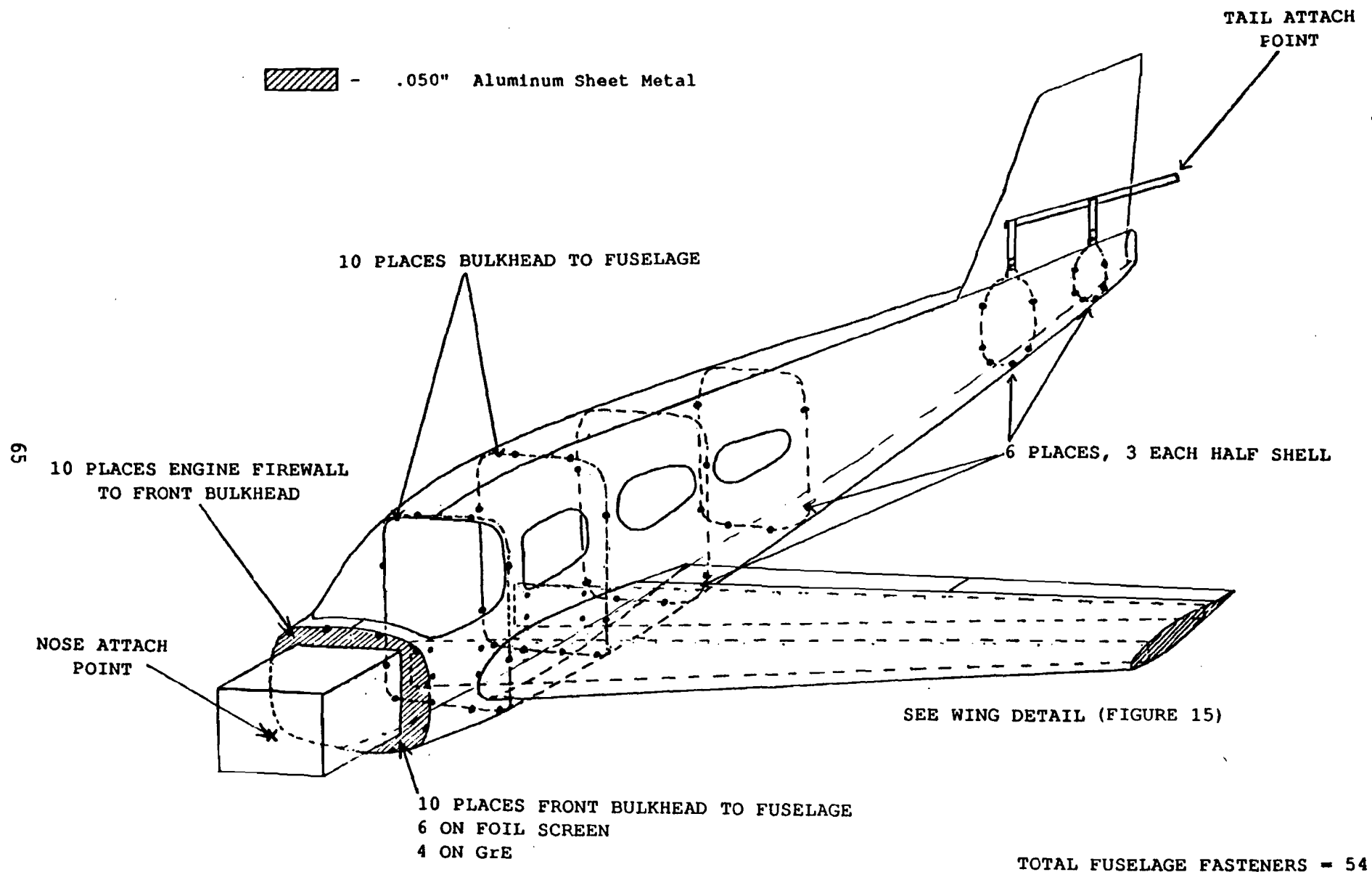
FIGURE 13 FUSELAGE FASTENER LOCATIONS
