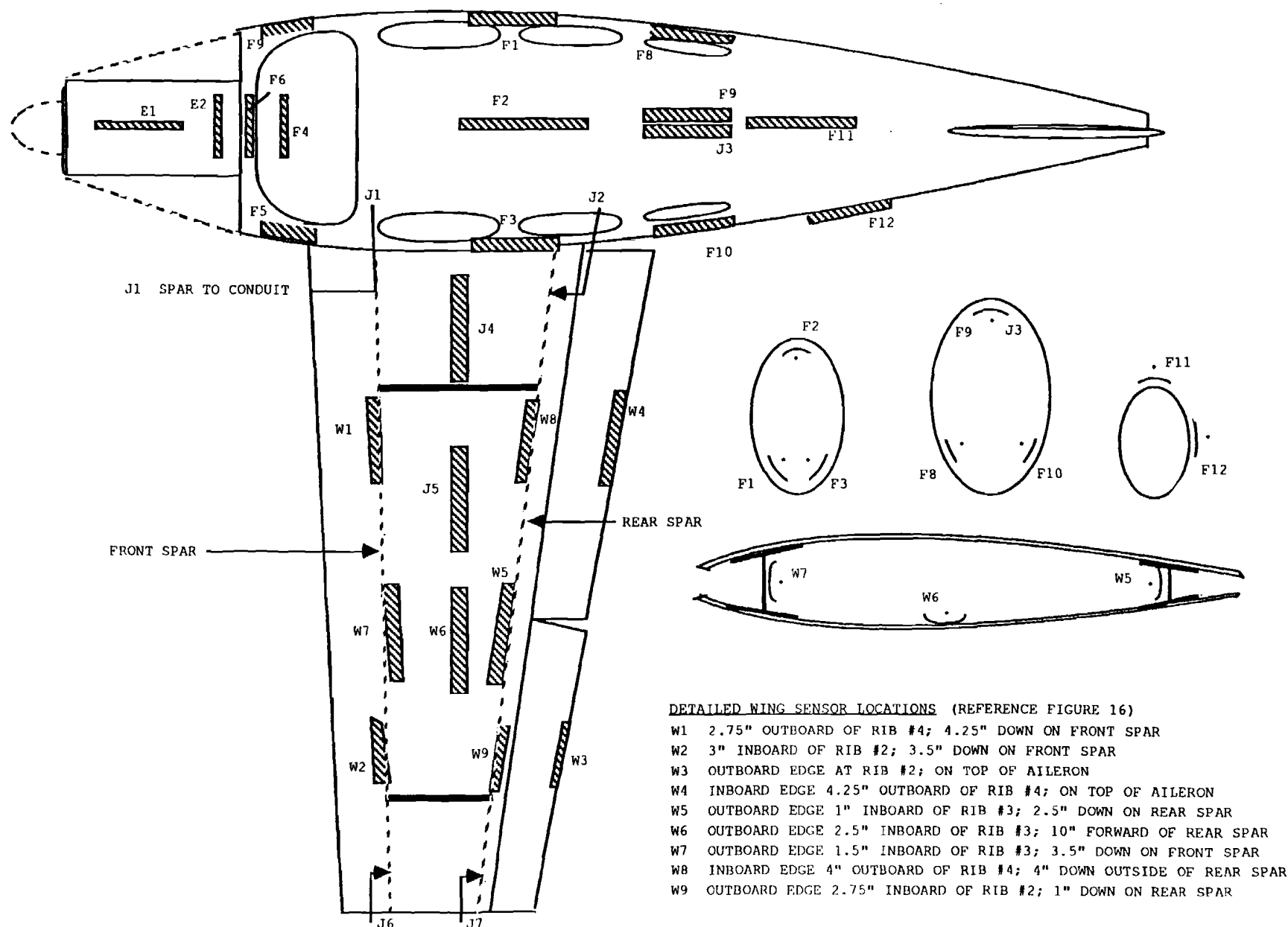
FIGURE 18 EM SOURCE CHARACTERIZATION SENSOR LOCATIONS (PLAN VIEW)
