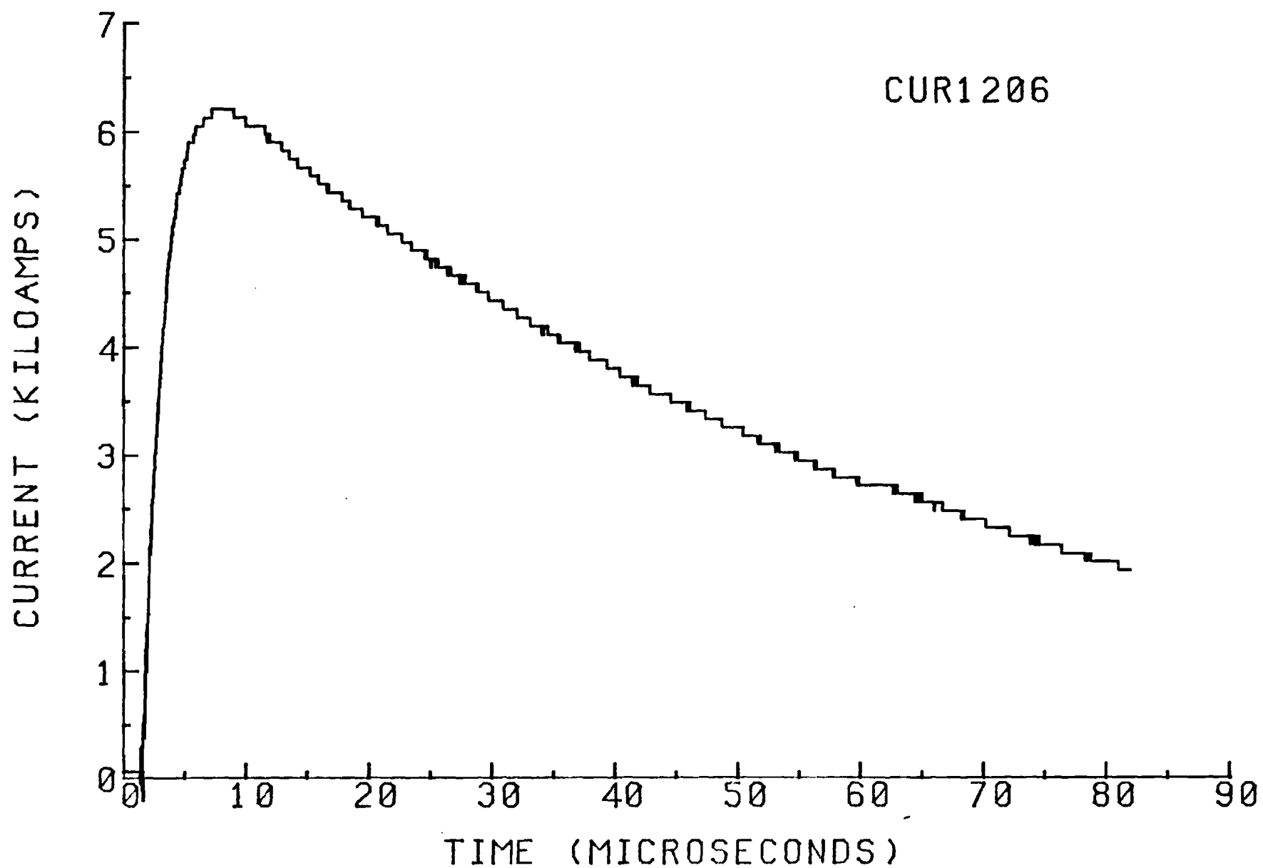
FIGURE 29 EXAMPLE 7 KA MODERATE-LEVEL PULSE CURRENT WAVEFORM
