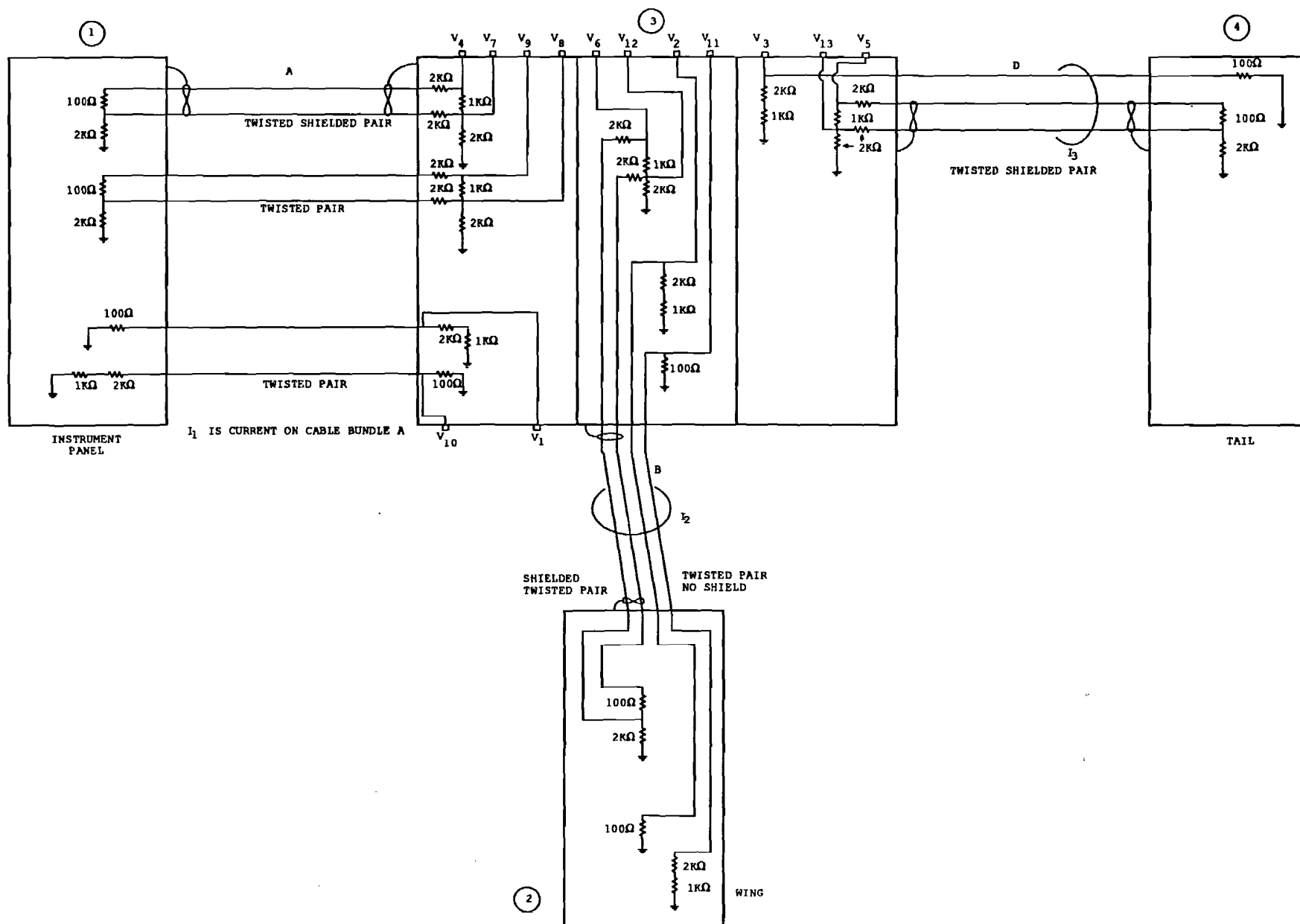
FIGURE 22 AUTO PILOT CIRCUIT DETAIL
