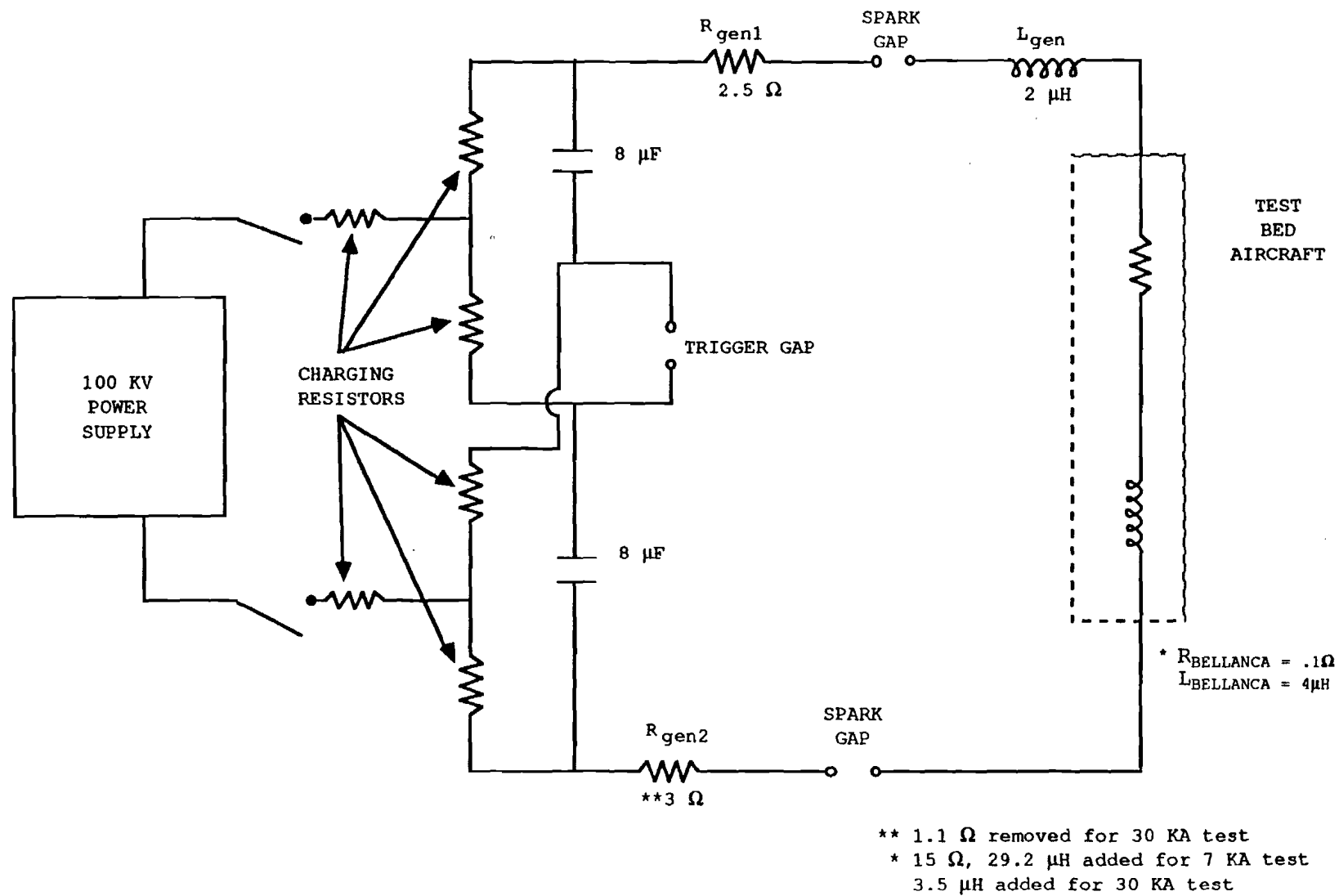
FIGURE 28 MODERATE-LEVEL PULSE GENERATOR CONFIGURATION
