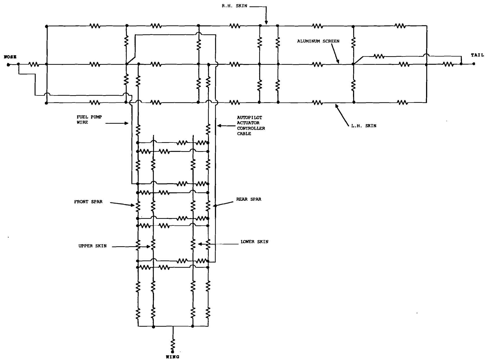
FIGURE 61 TEST BED RESISTOR MODEL
