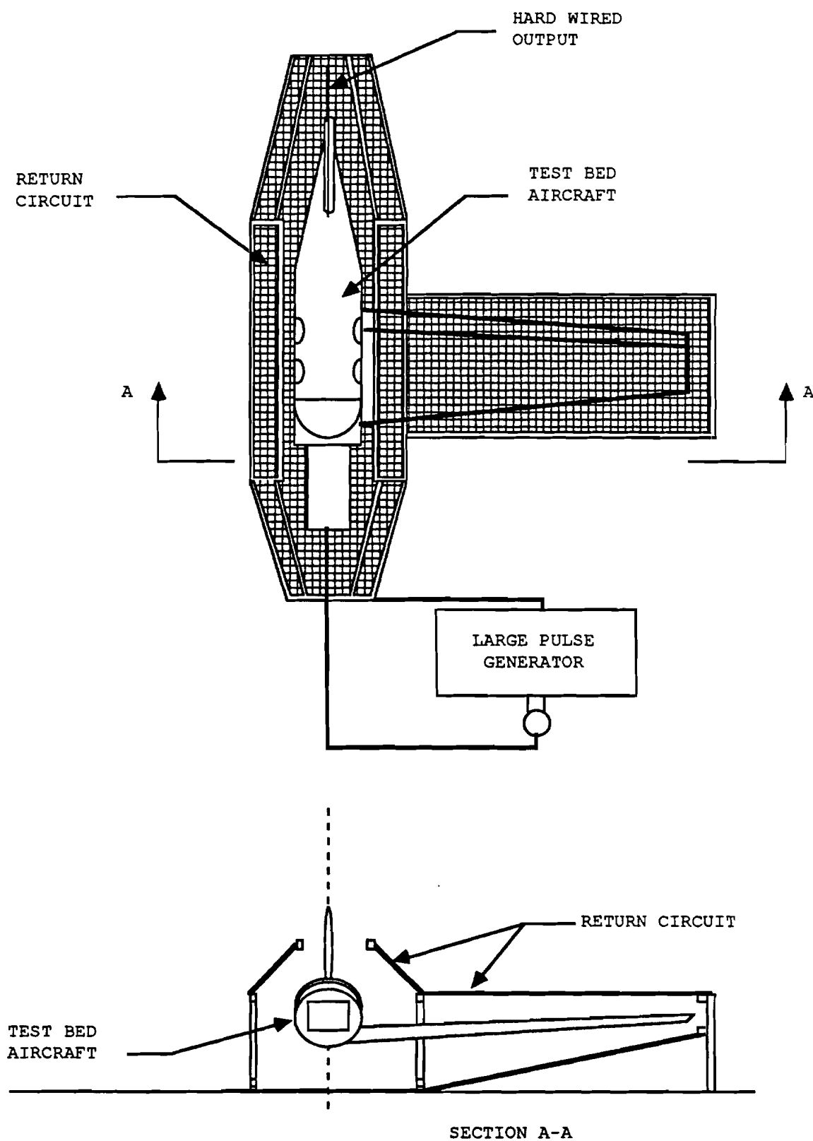
FIGURE 6 MODERATE LEVEL PULSE TEST SETUP
