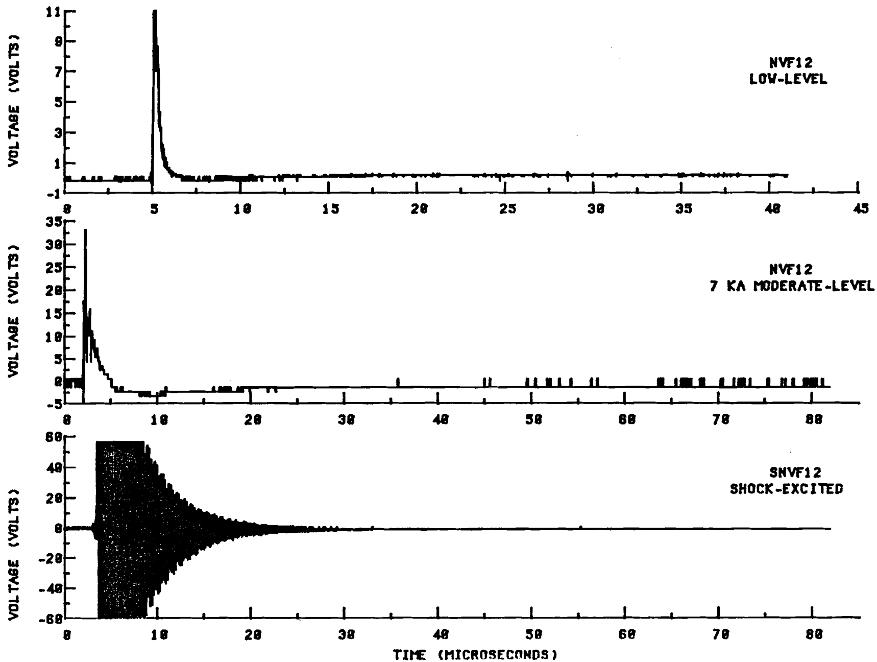
FIGURE 43 EXAMPLE I-DOT RESPONSE MEASUREMENT
