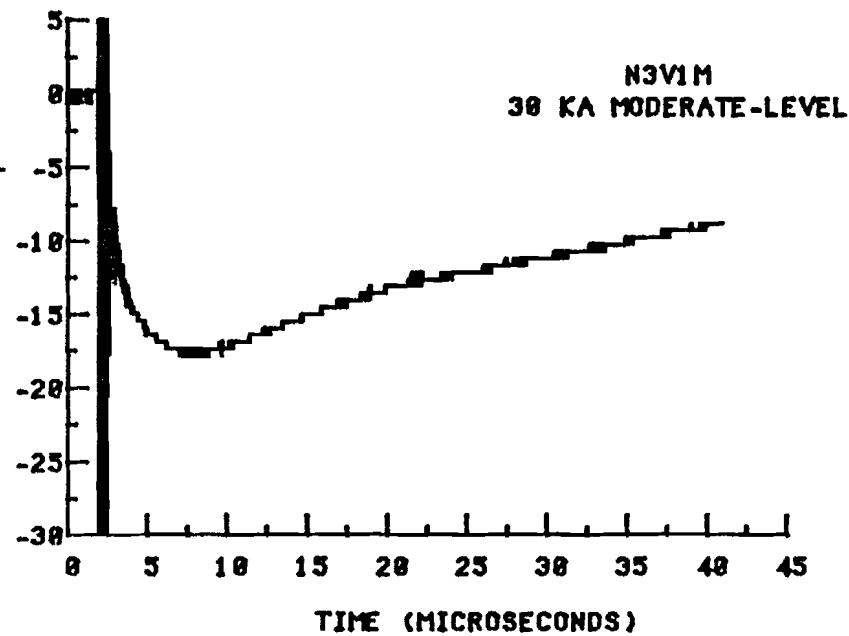
FIGURE 42 EXAMPLE RESISTIVE RESPONSE MEASUREMENT
