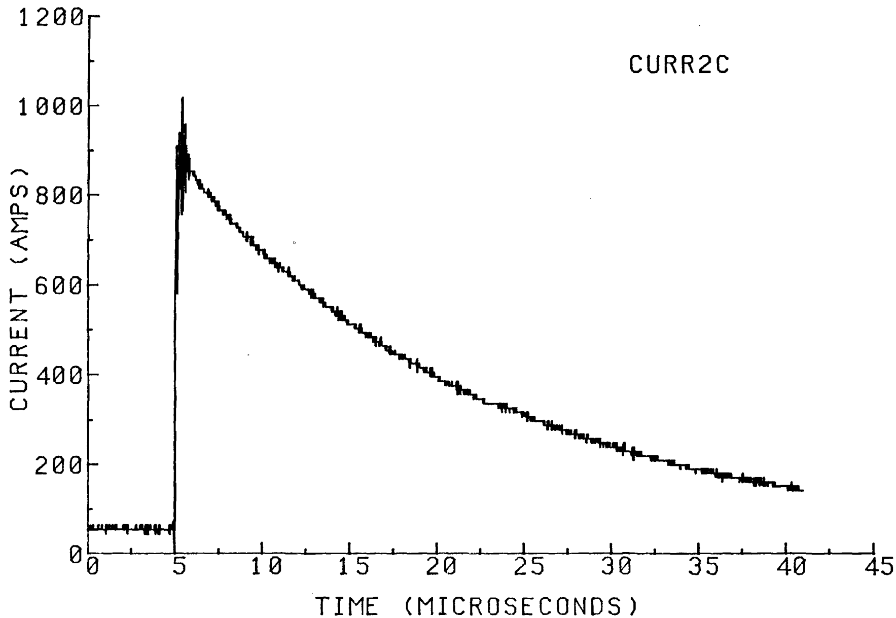
FIGURE 27 EXAMPLE LOW-LEVEL PULSE CURRENT WAVEFORM
