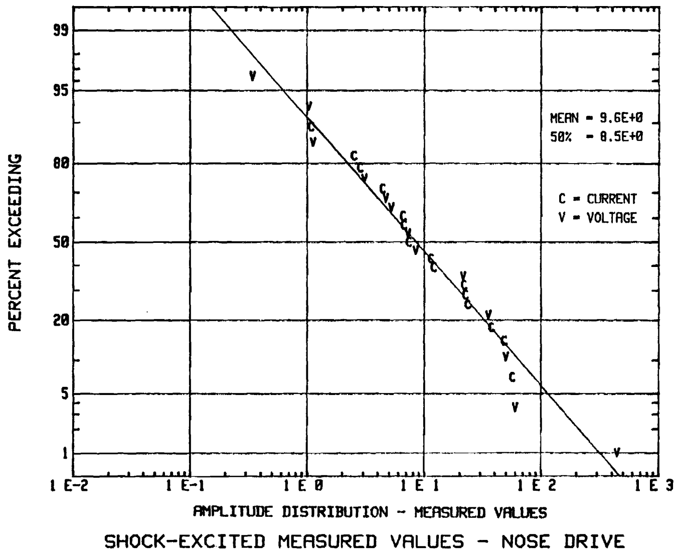
FIGURE 54 STATISTICAL DISTRIBUTION OF SHOCK-EXCITATION MEASURED VALUES NOSE DRIVE
