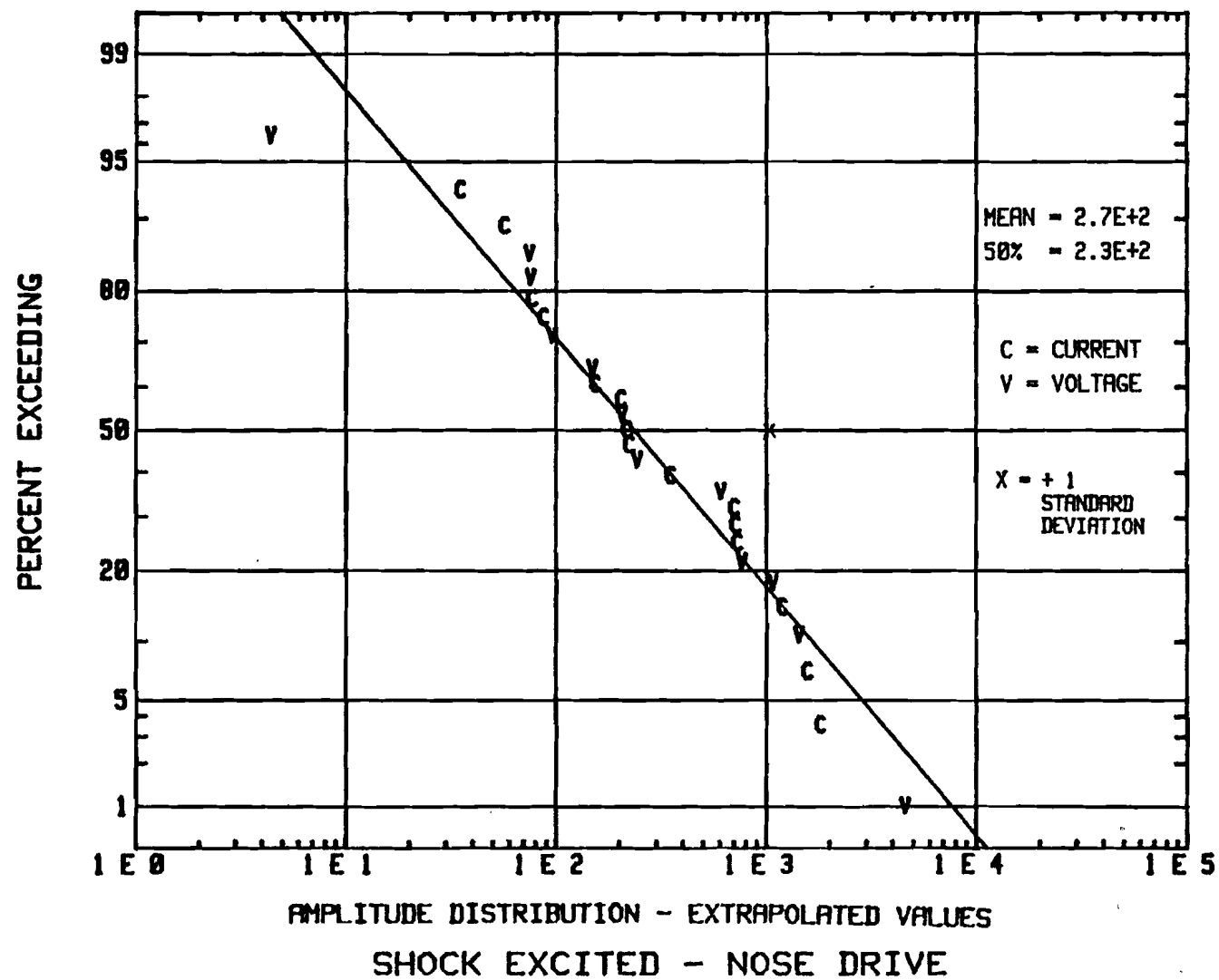
FIGURE 47 STATISTICAL DISTRIBUTION OF SHOCK-EXCITATION EXTRAPOLATED VALUES NOSE DRIVE
