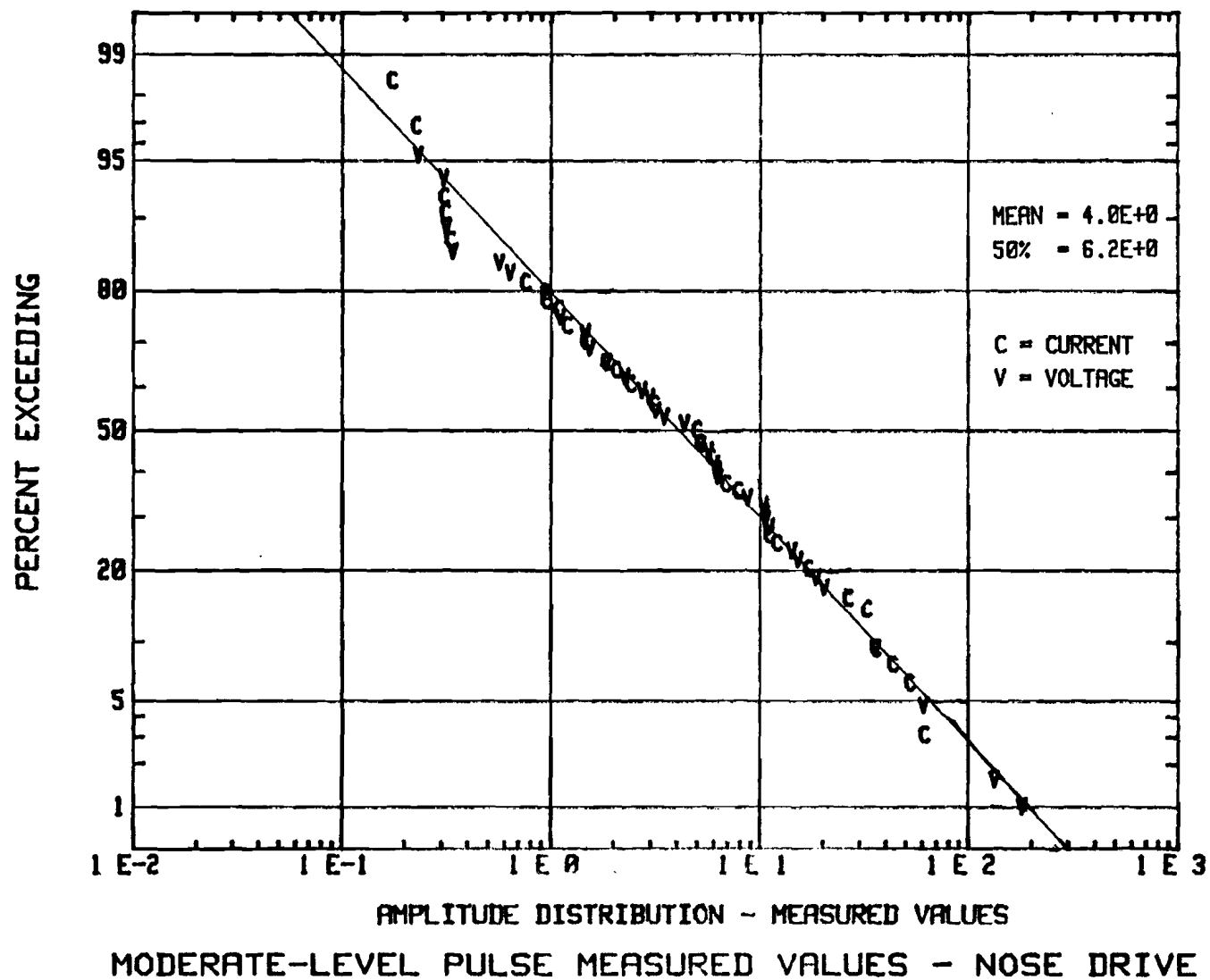
FIGURE 53 STATISTICAL DISTRIBUTION OF MODERATE-LEVEL PULSE MEASURED VALUES NOSE DRIVE
