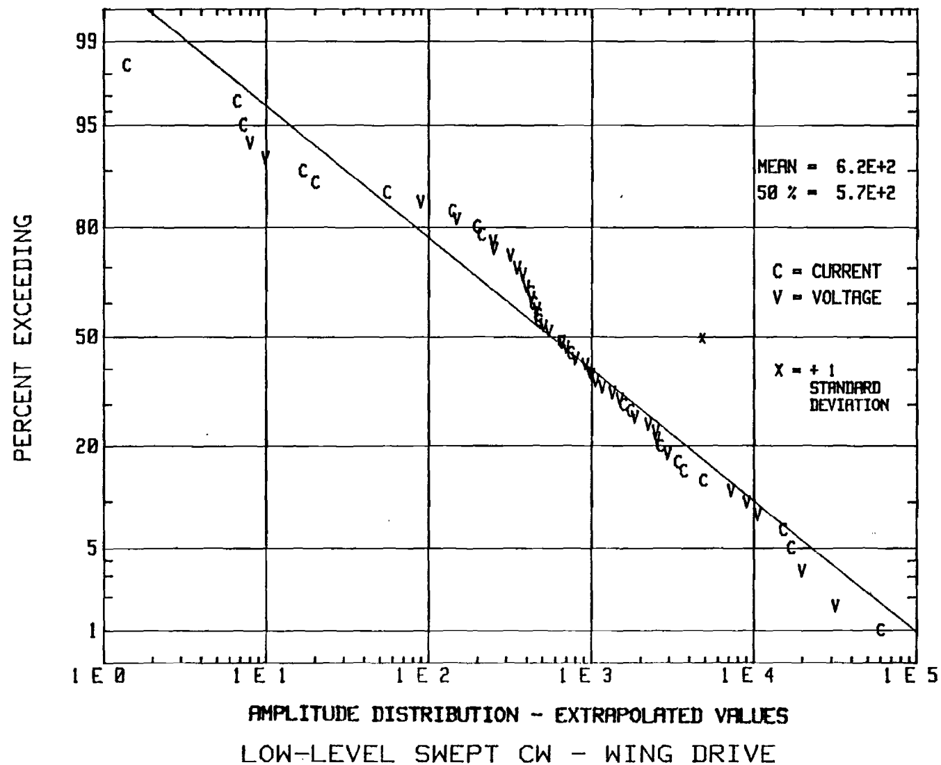
FIGURE 48 STATISTICAL DISTRIBUTION OF SWEEP CW EXTRAPOLATED VALUES - WING DRIVE
