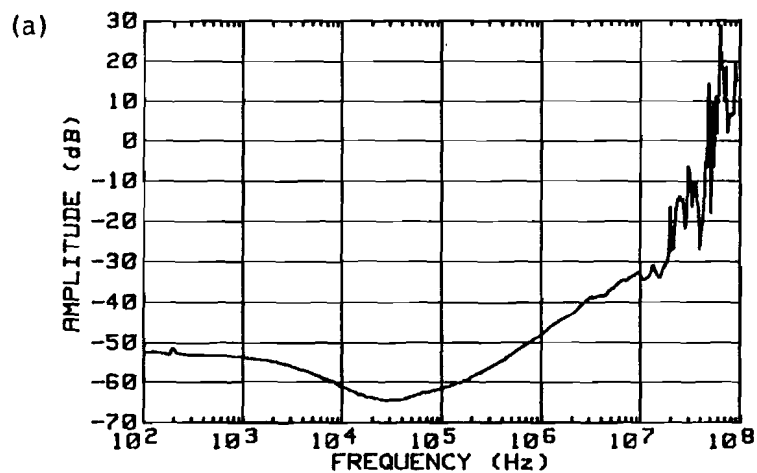
TEST POINT N3V1 - MEASURED DATA
