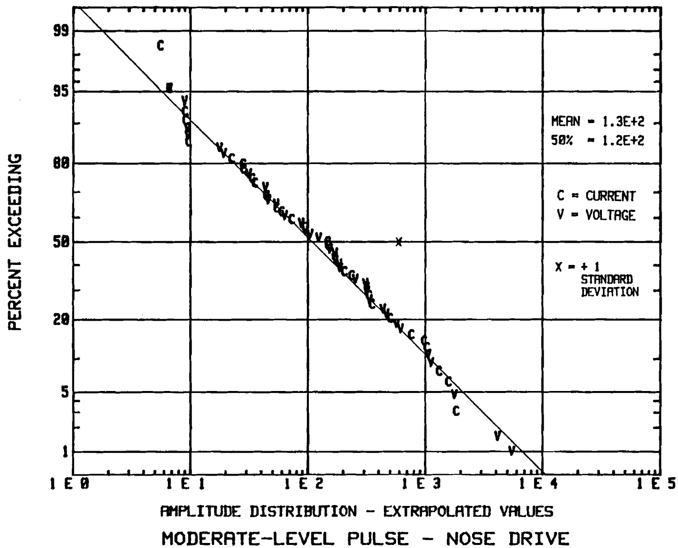
FIGURE 46 STATISTICAL DISTRIBUTION OF MODERATE-LEVEL PULSE EXTRAPOLATED VALUES NOSE DRIVE
