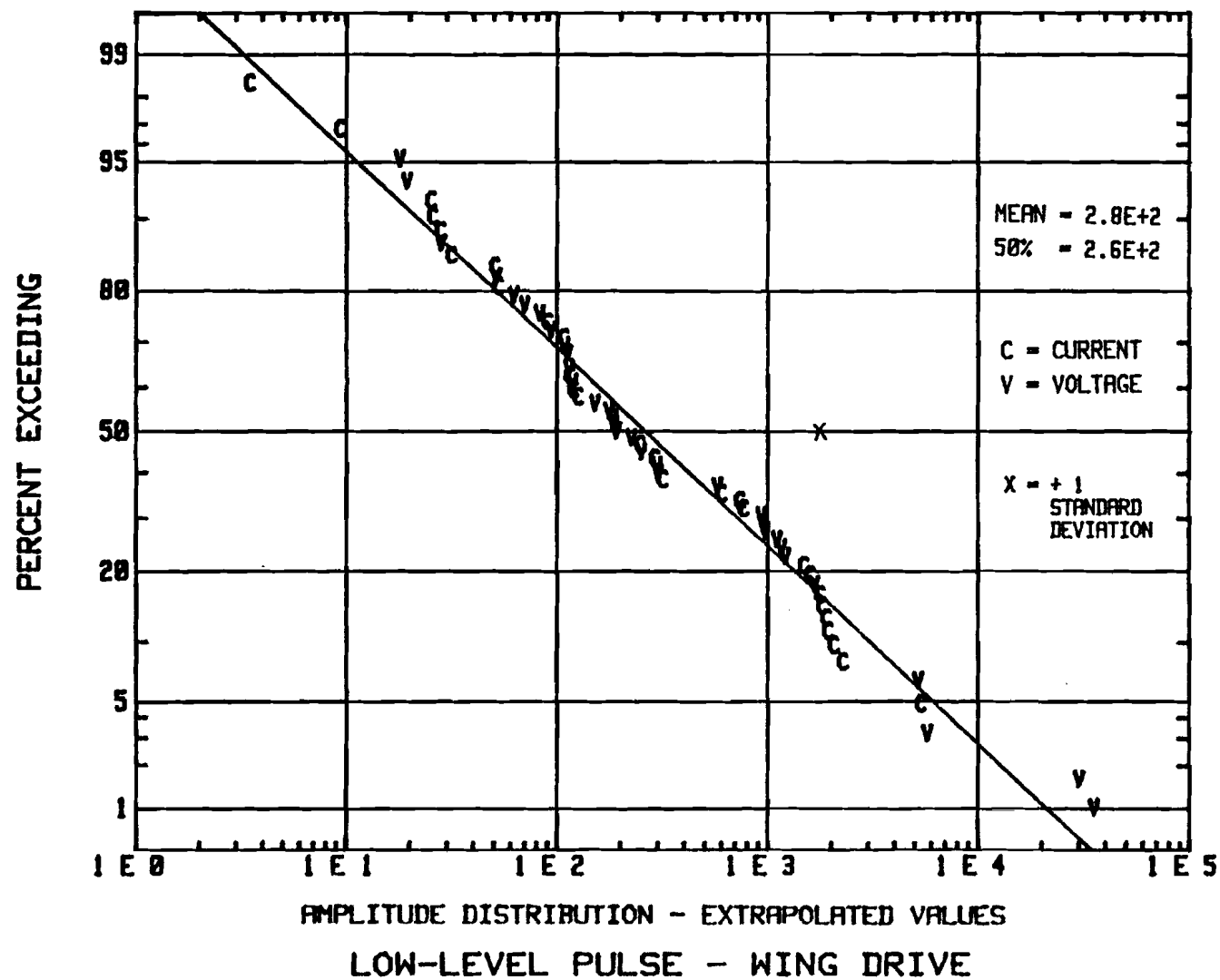
FIGURE 49 STATISTICAL DISTRIBUTION OF LOW-LEVEL PULSE EXTRAPOLATED VALUES WING DRIVE
