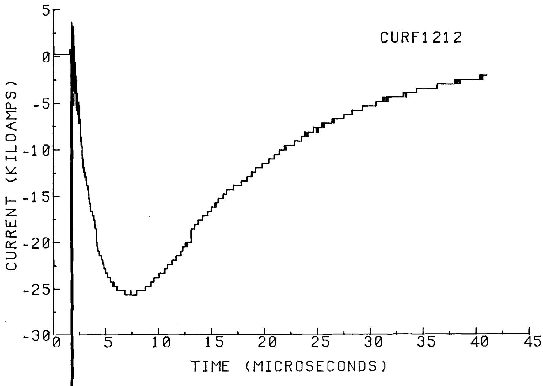
FIGURE 32 EXAMPLE 30 KA MODERATE-LEVEL PULSE CURRENT WAVEFORM
