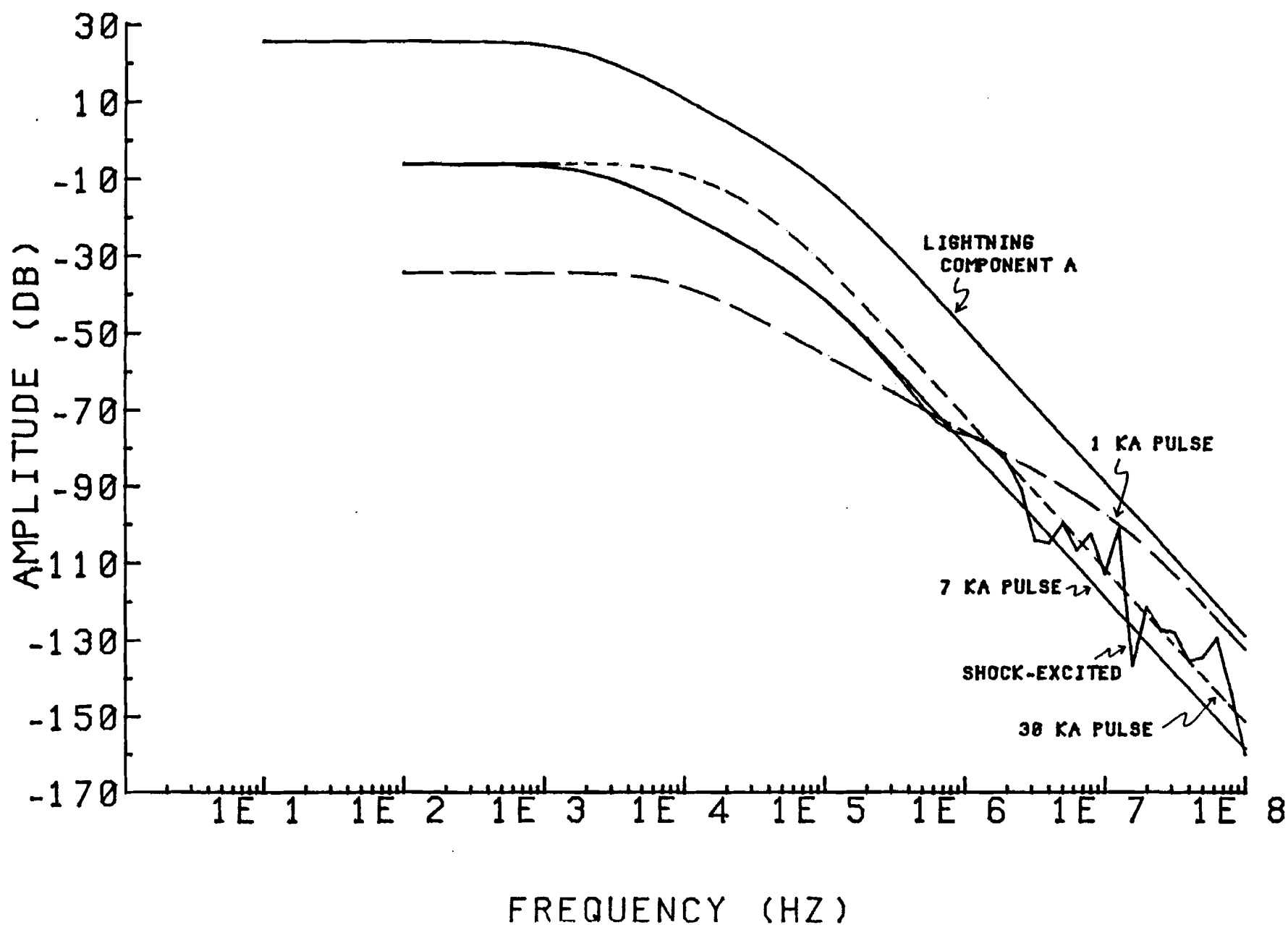
FIGURE 40 COMPARISON OF PULSE CURRENT SPECTRA WITH SEVERE LIGHTNING SPECTRUM
