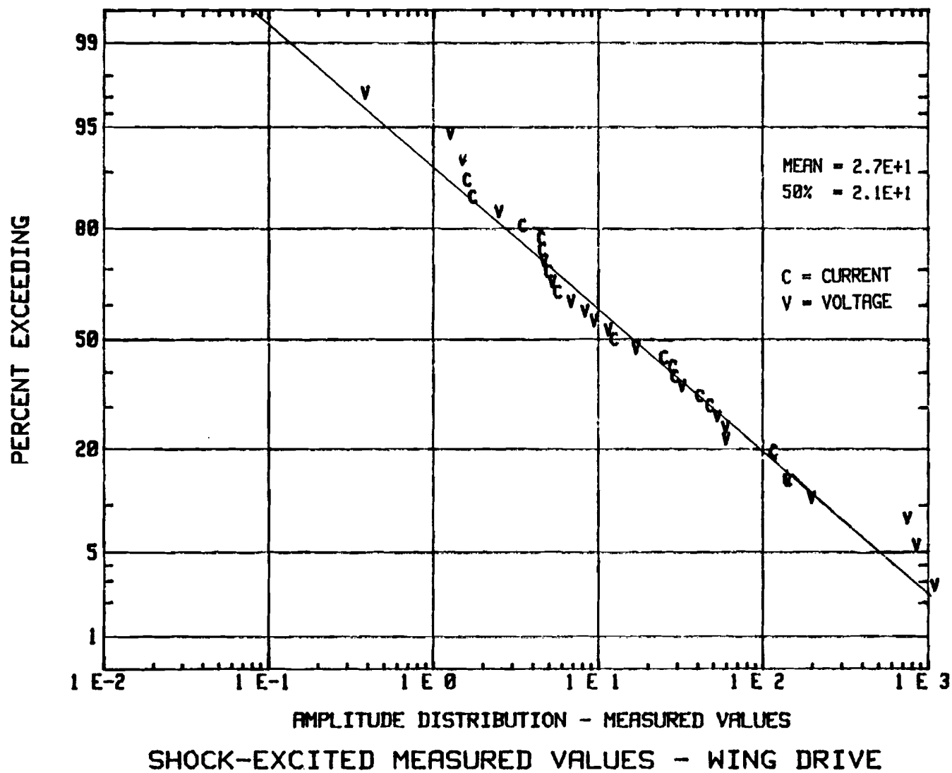
FIGURE 57 STATISTICAL DISTRIBUTION OF SHOCK-EXCITATION MEASURED VALUES WING DRIVE
