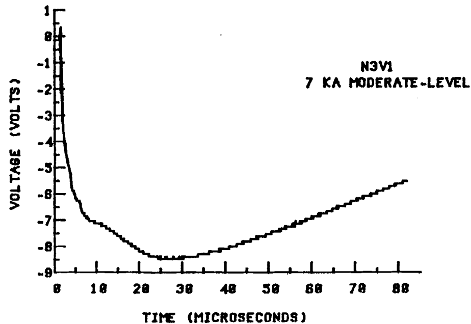
FIGURE 42 EXAMPLE RESISTIVE RESPONSE MEASUREMENT
