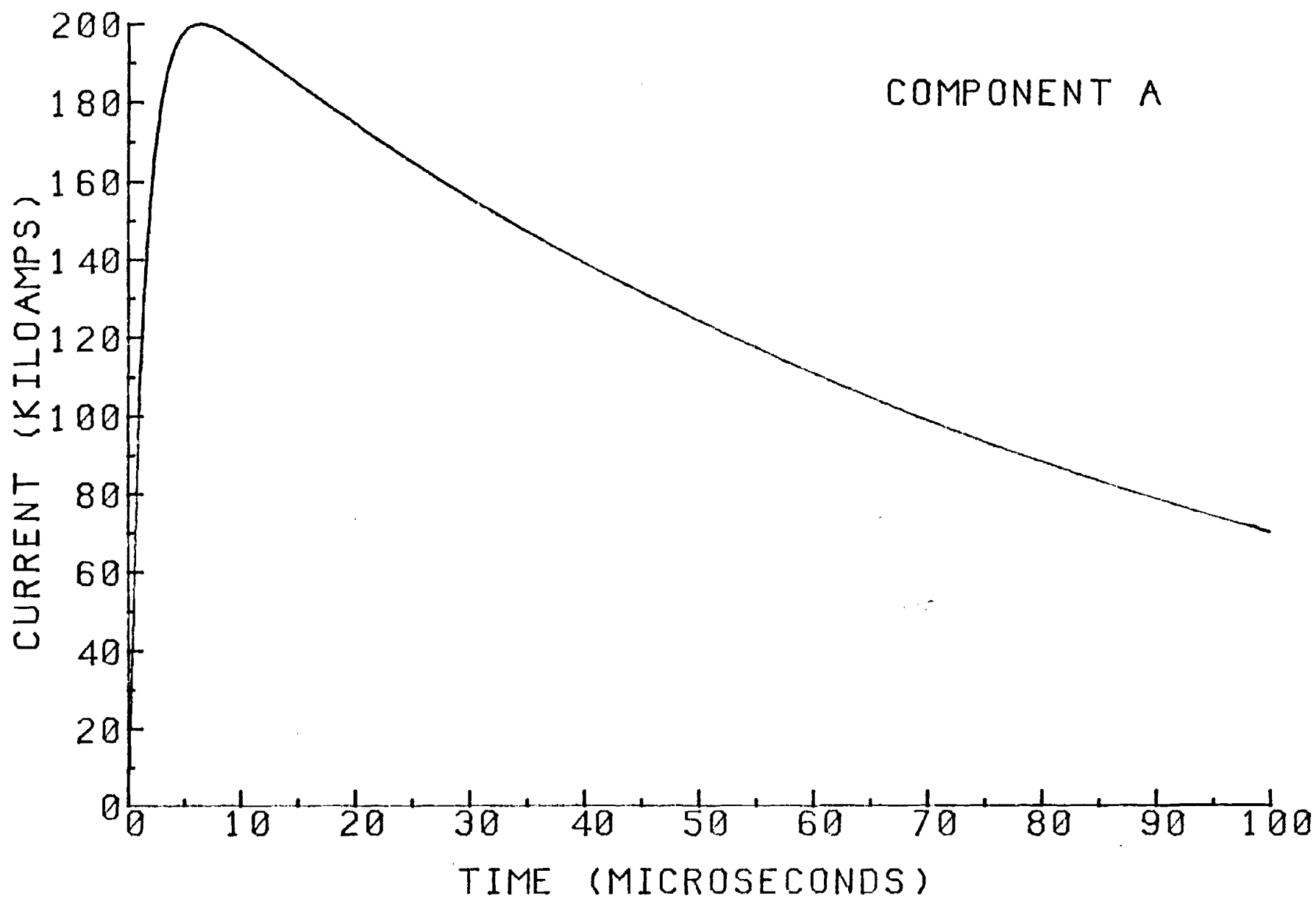
FIGURE 30 COMPONENT A SEVERE LIGHTNING THREAT CURRENT WAVEFORM
