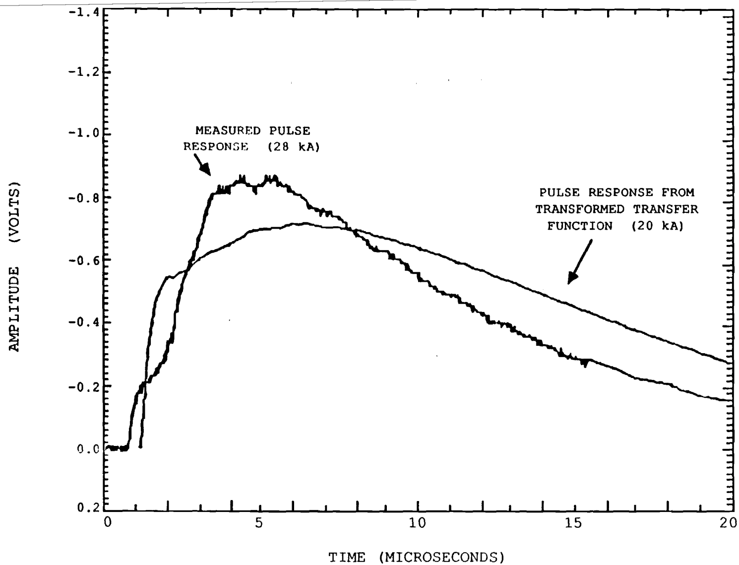
FIGURE 4 MEASURED VS. FOURIER TRANSFORMED DATA
