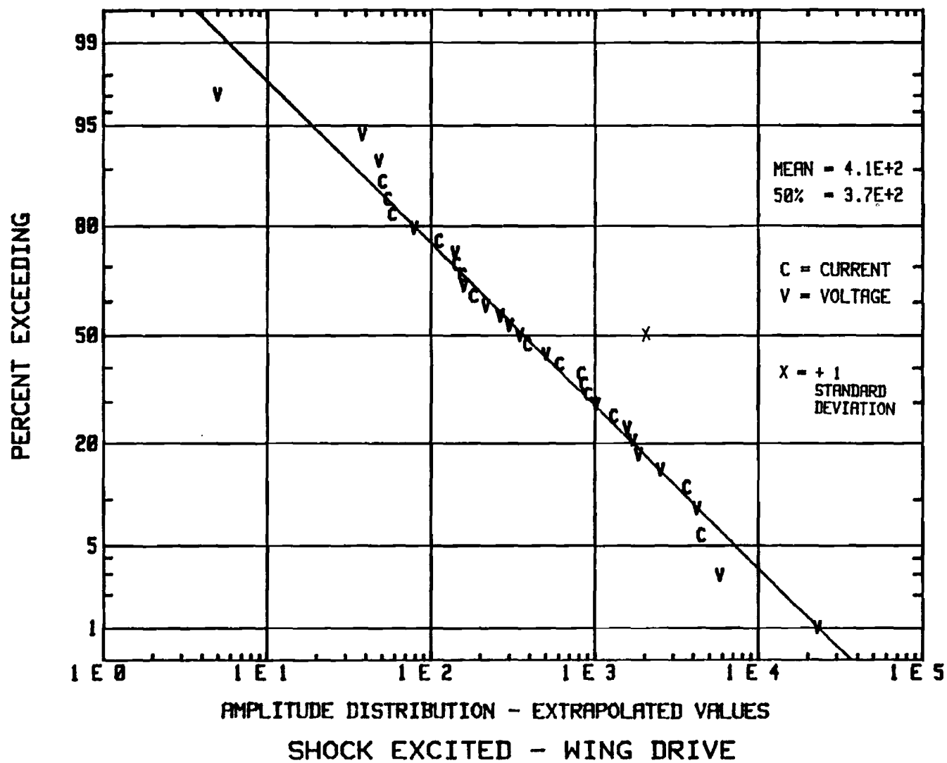
FIGURE 51 STATISTICAL DISTRIBUTION OF SHOCK-EXCITATION EXTRAPOLATED VALUES WING DRIVE
