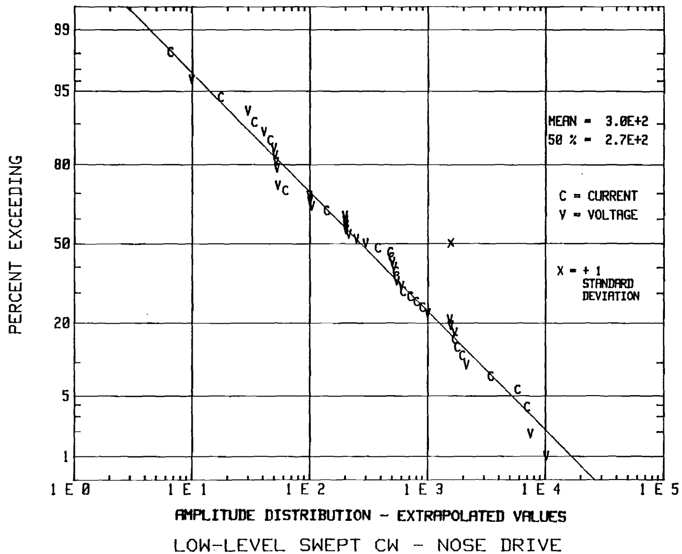
FIGURE 44 STATISTICAL DISTRIBUTION OF SWEEP CW EXTRAPOLATED VALUES - NOSE DRIVE
