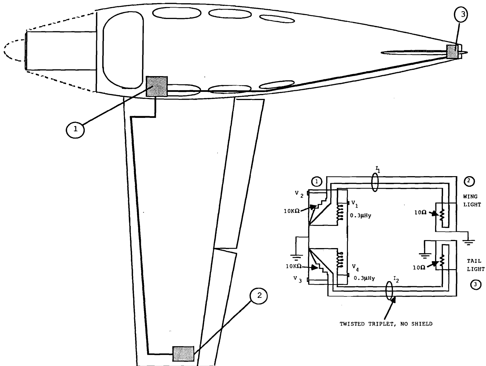
FIGURE 23 ELECTRIC POWER TO LIGHTS - INSTALLATION AND CIRCUIT DETAIL
