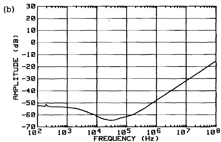
TEST POINT N3V1 - SMOOTHED DATA
