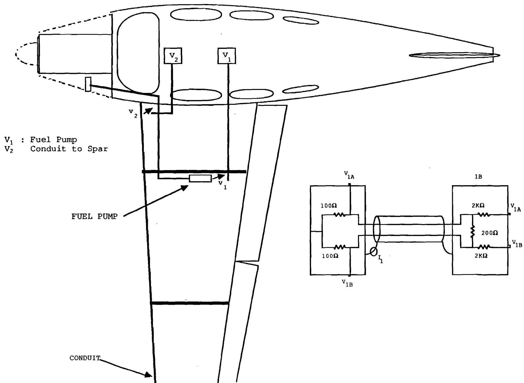
FIGURE 24 FUEL SYSTEM MECHANICAL INSTALLATION AND CIRCUIT DETAIL
