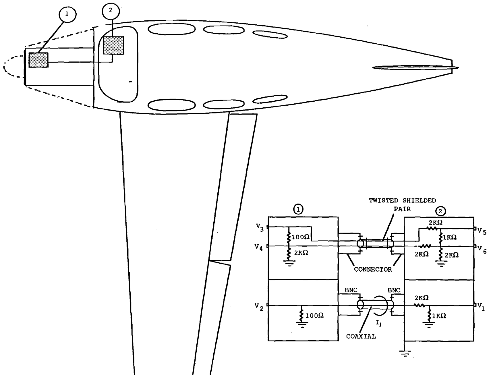
FIGURE 20 ENGINE CONTROL INSTALLATION AND CIRCUIT DETAIL
