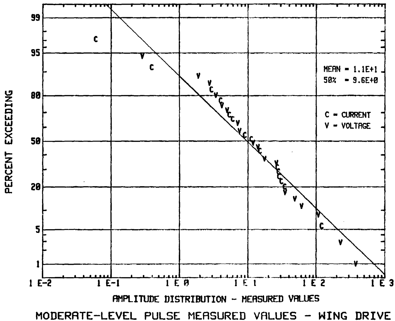
FIGURE 56 STATISTICAL DISTRIBUTION OF MODERATE-LEVEL PULSE MEASURED VALUES WING DRIVE
