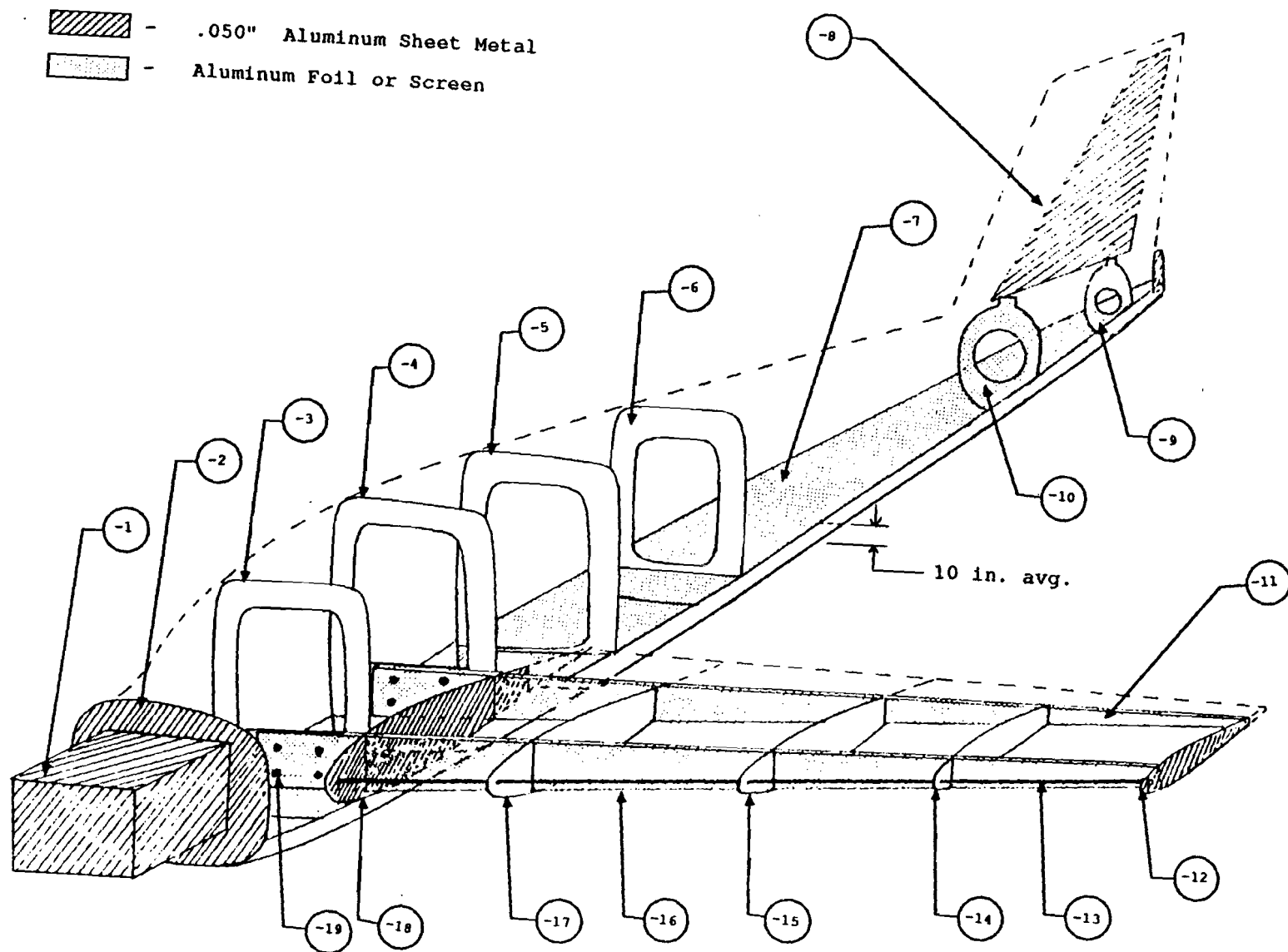
FIGURE 11 TEST BED INTERNAL DETAIL
