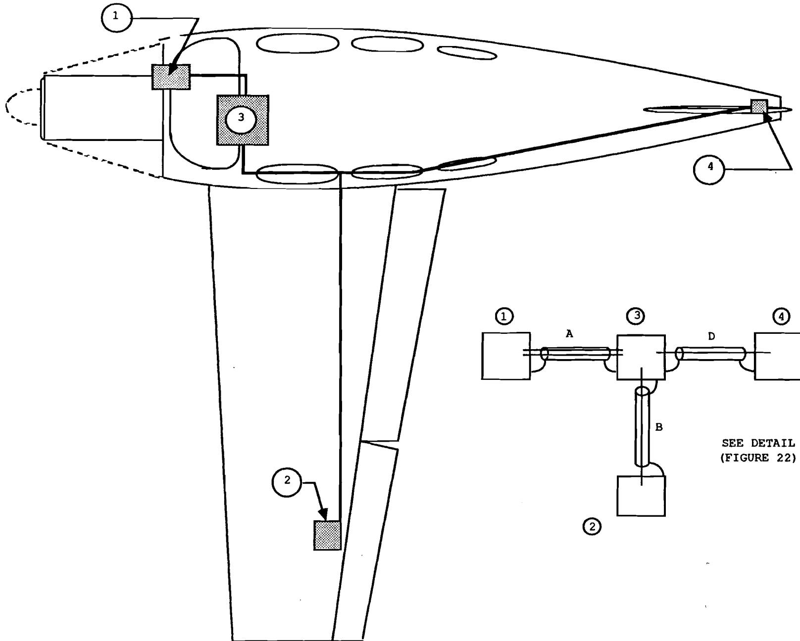
FIGURE 21 AUTOPILOT INSTALLATION
