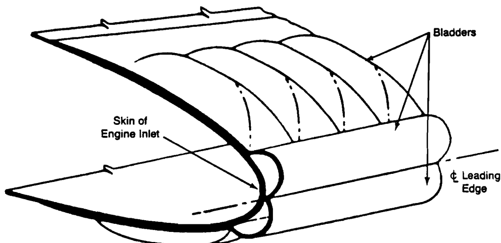
Figure 2-5. Schematic Cross-Section of a Pneumatic Boot De-Icer (Inflated) as Installed on an Engine Inlet
