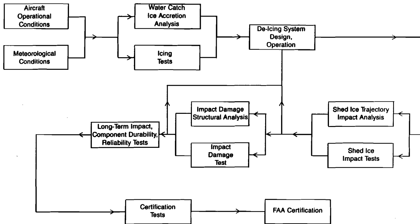
Figure 5-1. Inlet De-Ice System Certification Process
