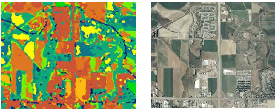
Fig. 26 A 3*3 majority analysis was applied to the ISODATA classification product of ETM+ 06/16/2002, reducing some salt-and-pepper effects from the classification results. A more generalized wetland distribution pattern can be found
