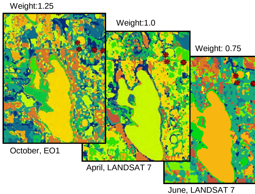
Fig. 27 Weighted overlay of ISODATA classifications from the three different season images
