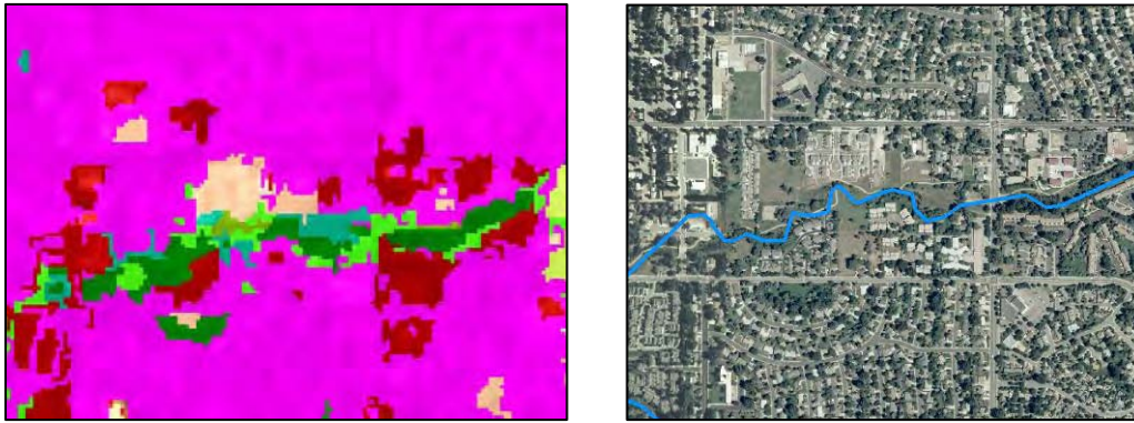
Fig.22 Involvement of stream layer in delineating wetlands in the neighborhood (shown on the left) is aided by inclusion of the stream network layer into the DEFINIENS® software as an analysis feature
