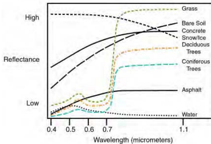
Fig. 15 Reflectance of different vegetation category and materials
