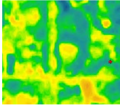
Fig.12 The greenness layer has been found highly corresponding to the existence of wetland locations. The dark blue color on the right is correspondent to the vegetation on the left
