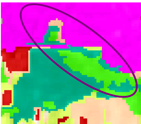
Fig. 31 Comparison of individual marsh identification and its location in the real world shows the success of this wetland mapping method
