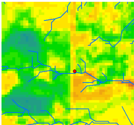
Fig.17 NDVI of August from ASTER 08132003 imagery
