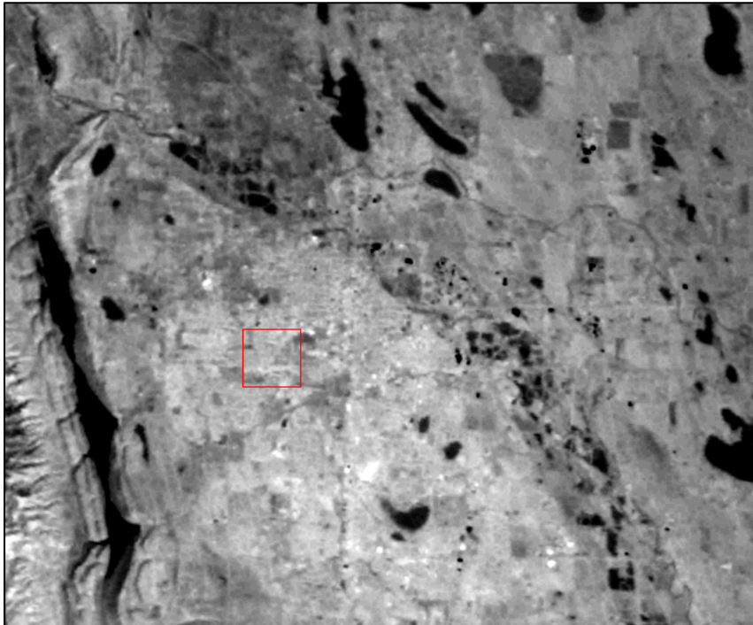
Fig.11 At-satellite surface temperature generated from ETM+ of 04/16/2003 data for Fort Collins and adjacent area
