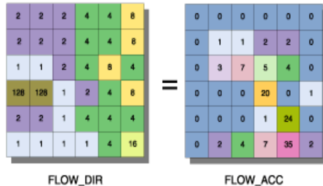
Fig. 20 Flow accumulation operation concept
