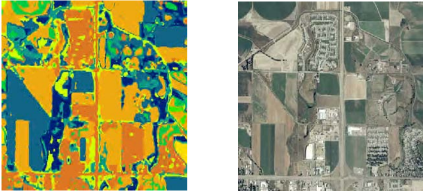
Fig. 24 From the ISODATA classification of EO1 ALI 10/26/2001 imagery, the wetland delineation is promising. The blue color in this thematic layer represents the high potential as a wetland
