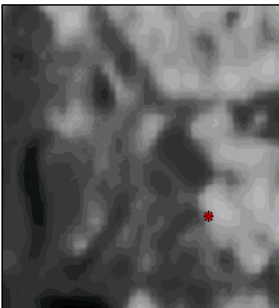
Fig. 14 The brightness layer of the same sample site shows that the grey and medium dark areas are likely to be wetlands
