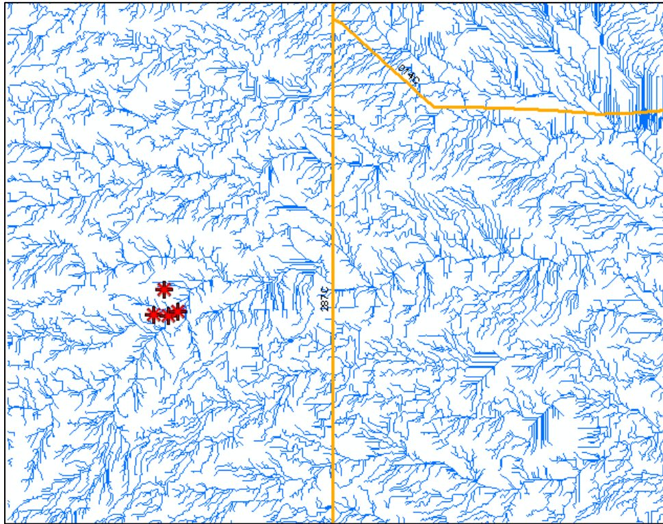
Fig. 21 Generated stream network from 10-meter DEM
