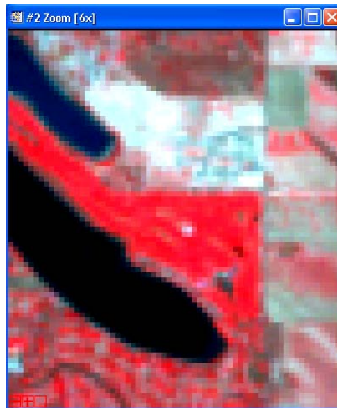
Fig. 9 Raw ETM+ imagery (30m)
