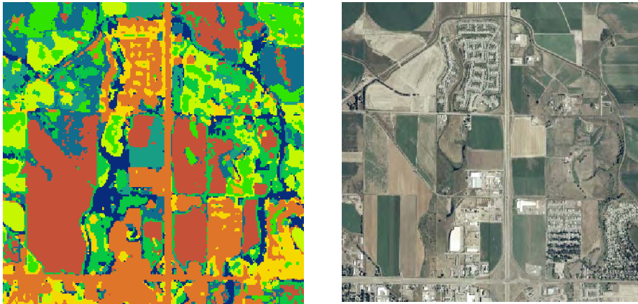
Fig. 25 ISODATA classification of April LANDSAT 7 data provides valuable supplement information of different season for wetland delineation
