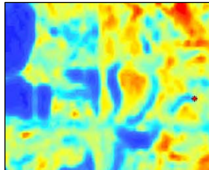
Fig. 13 Wetness, the bluer the color is the wetter the place is. These wet locations correspond to the wetlands and ponds on the left NAIP image
