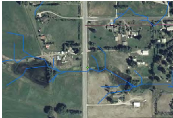
Fig. 16 NAIP photo with the generated stream network in blue lines
