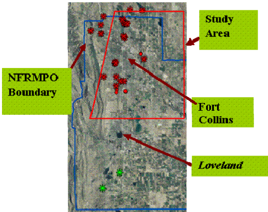
Fig. 6 Study area in vicinity of Fort Collins, CO
