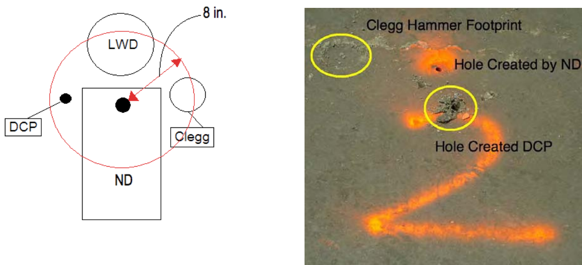
Figure 3-5. Typical Layout Adopted for Single Location Testing
