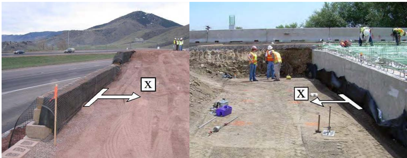
Figure 4-1. Offset X for MSE Wall and Bridge Approach Testing
