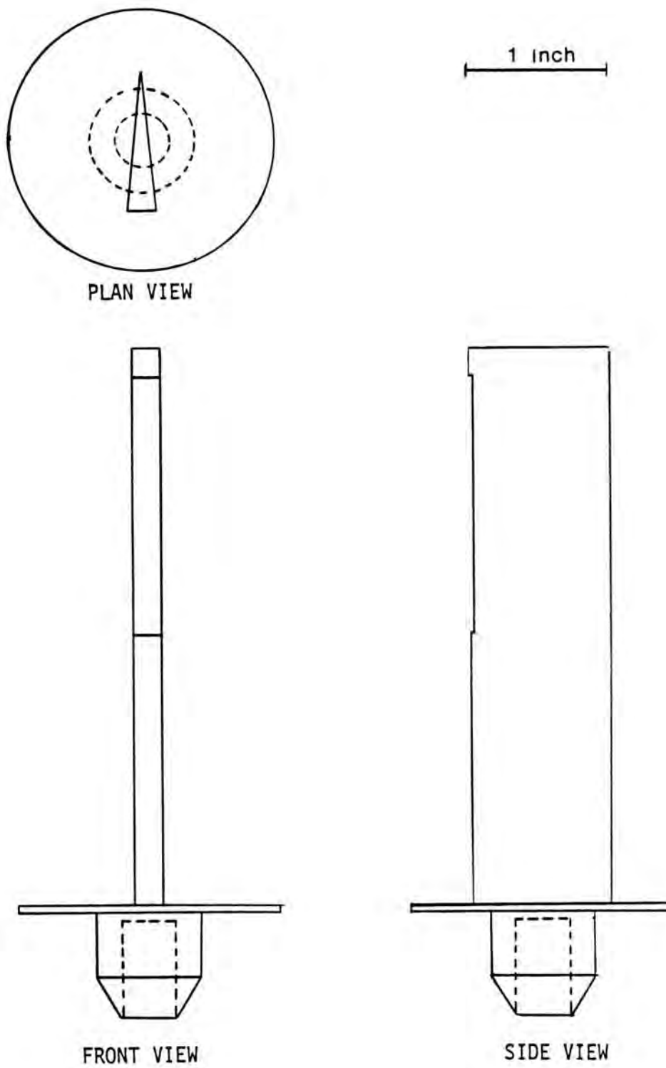
FIGURE 3.12 REFERENCE COLLECTOR BLADE.
