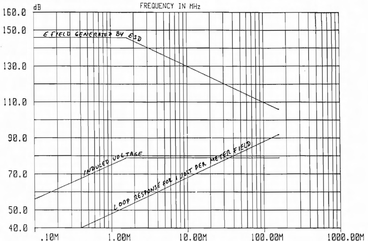
FIGURE 61. INDUCED VOLTAGE ON A LOOP FROM ESD
