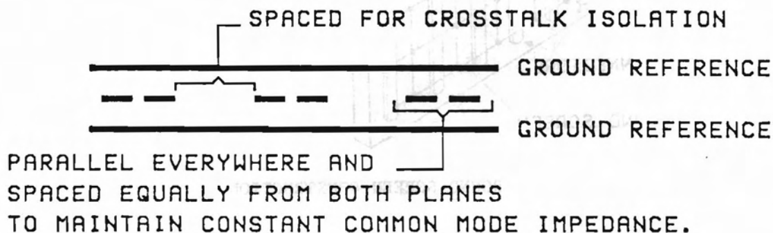
FIGURE 30. VIDEO SIGNAL DISTRIBUTION
