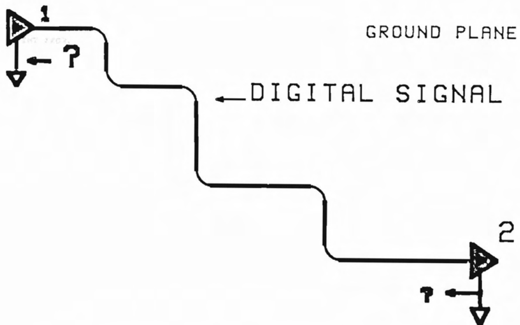
FIGURE 7. HOW DOES THE CURRENT RETURN?
