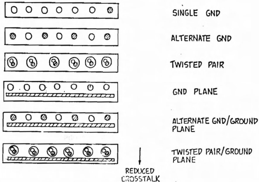
FIGURE 39. RIBBON CABLE
