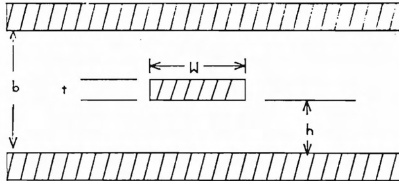
FIGURE 16. STRIPLINE
