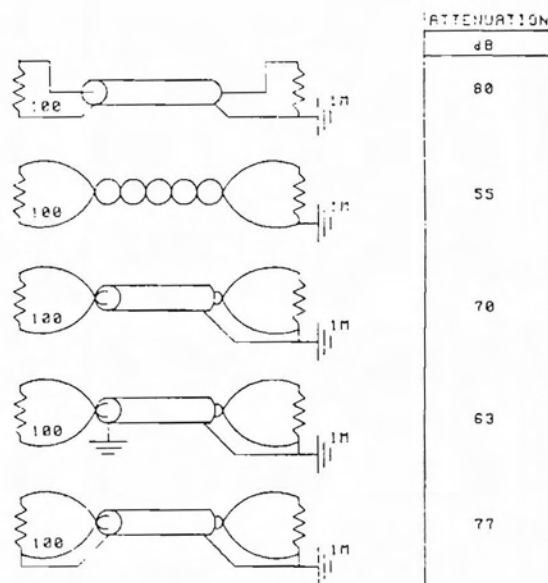
FIGURE 40. CABLE TERMINATION METHODS - ONE END GROUNDED
