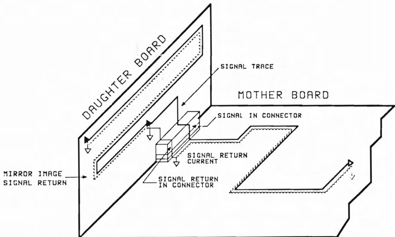
FIGURE 11. DAUGHTER BOARD TO MOTHERBOARD GROUNDING
