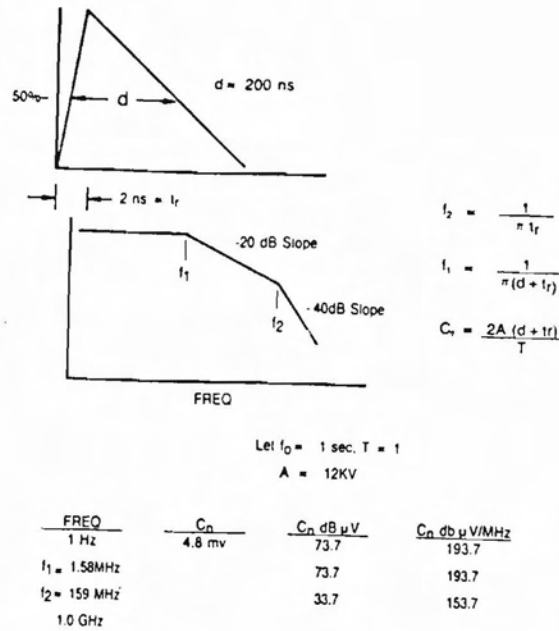
FIGURE 50. ESD VOLTAGE PREDICTION
