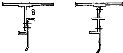
SECTION OF RIB
