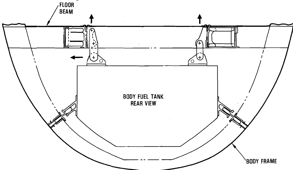
Figure 5-13. Tank Attachment Layout
