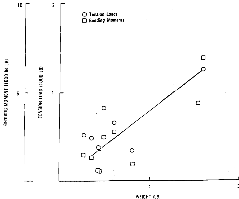
Figure 6-4. Example Breakaway Valve Weights and Separation Tension Loads and Bending Moments were Obtained from Test Data
