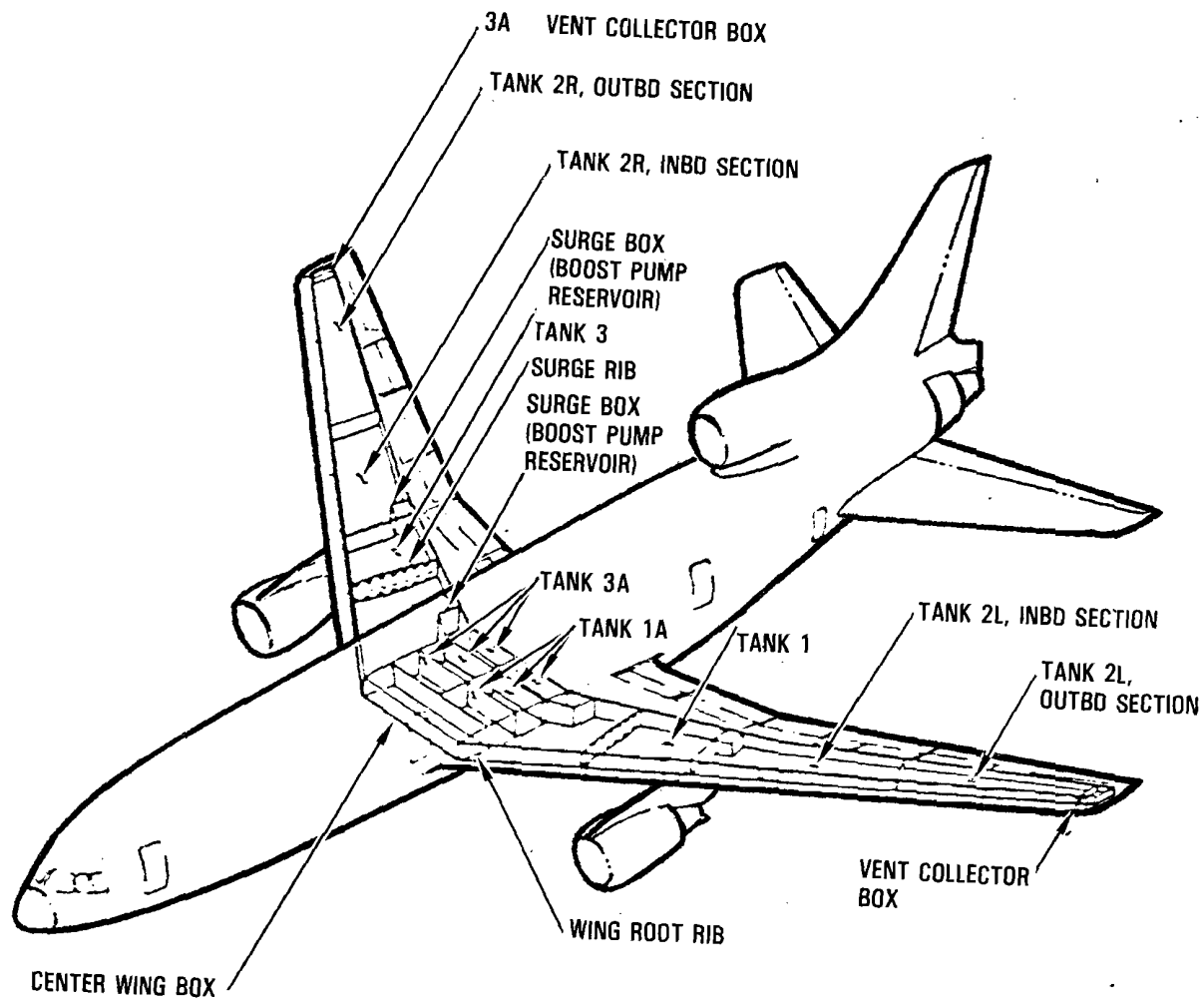
Figure 6-8. Spanwise Wing Fuel Tank Compartmentation
