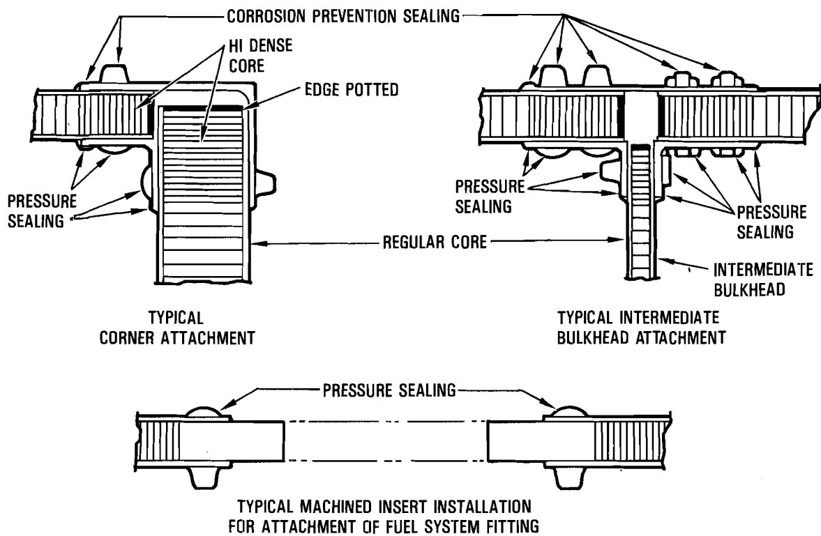
Figure 5-12. Fuel Tank Shell Construction
