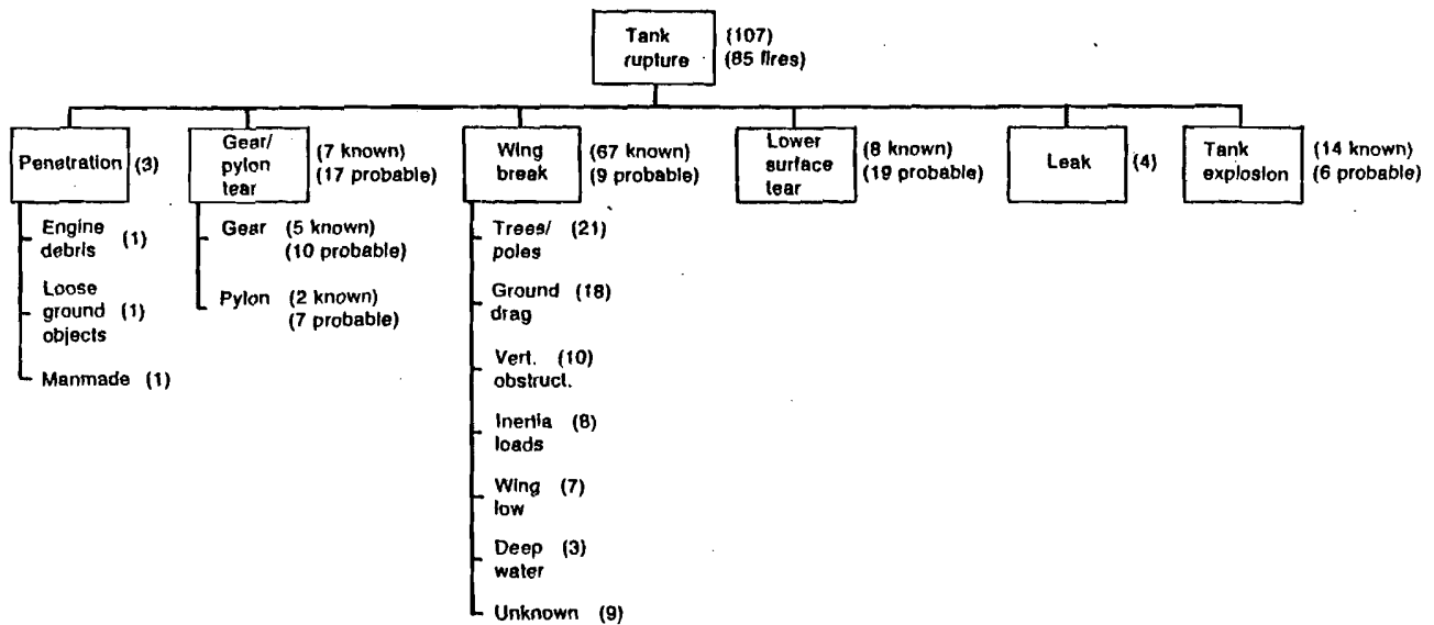
Figure 7-1. Types of Tank Rupture
