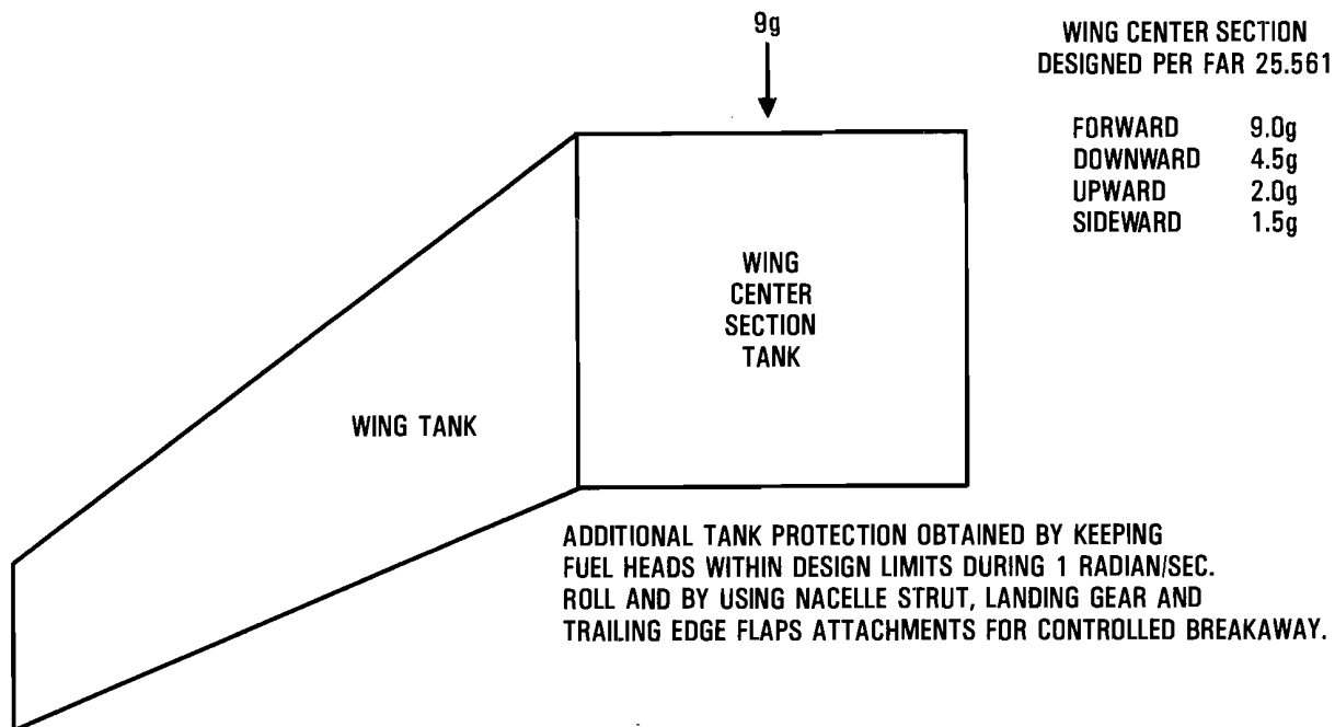
Figure B-4. Fuel Tank Load Factors
