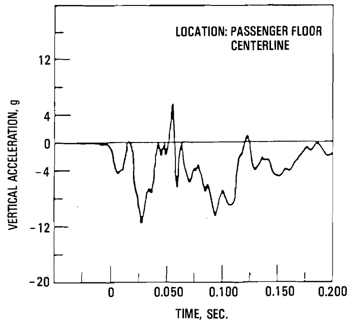
Figure 3-13. Results of Narrow-Body Airplane Forward Fuselage Section (With Cargo) Test (Reference 16)
