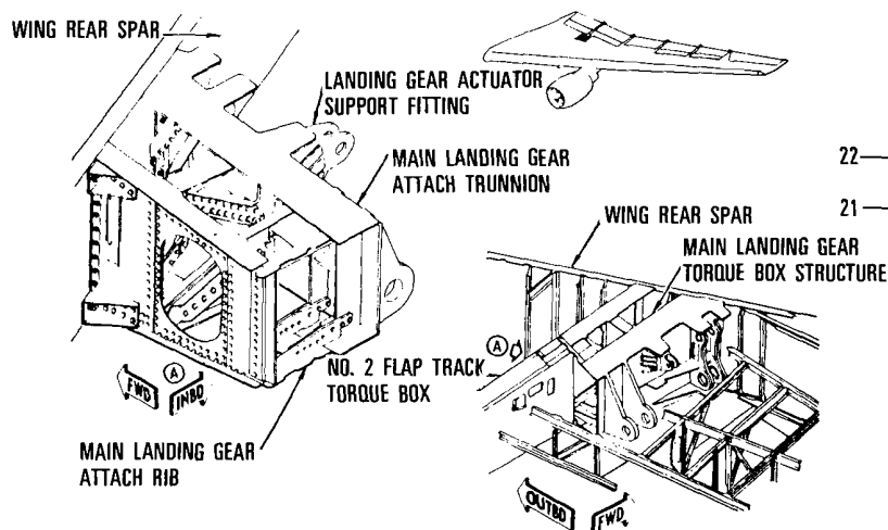
Figure 6-2. Main Landing Gear Components
