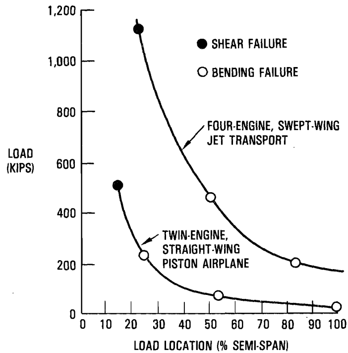
Figure 4-1. Examples of Local Concentrated Loads Required to Fail Wings in Chordwise Shear or Bending
