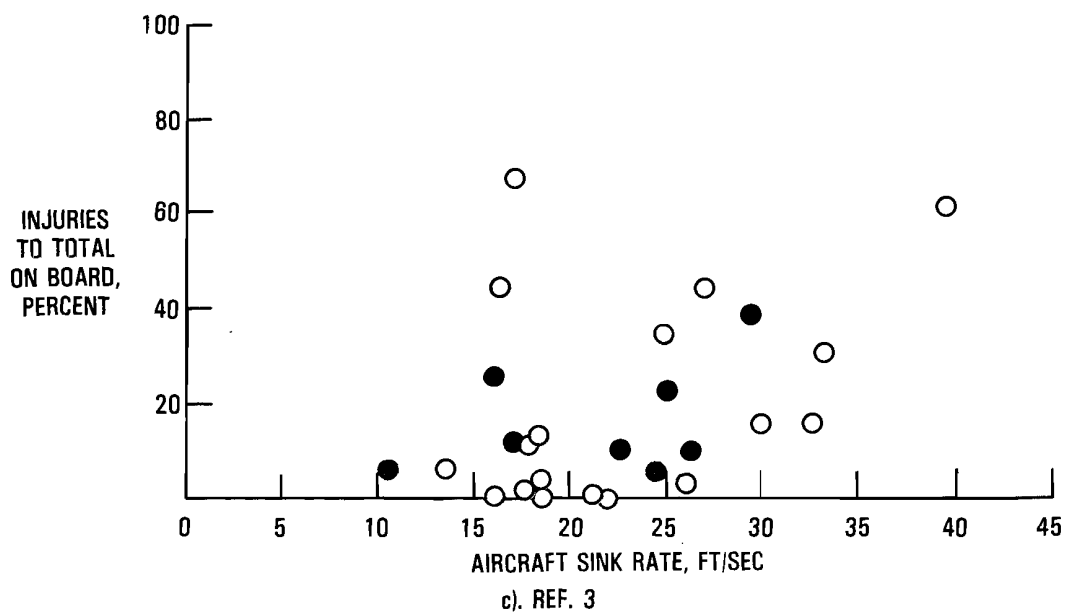
Figures 3-4. Injuries as a Function of Sink Rate
