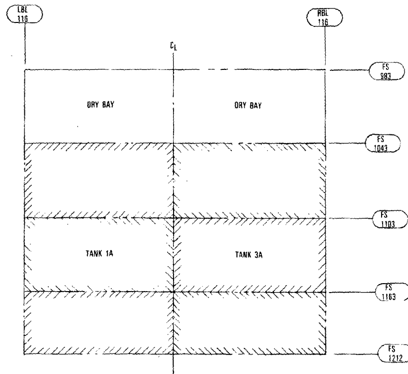
Figure 7-14. Center Section Tanks for Current Wide-body Airplane
