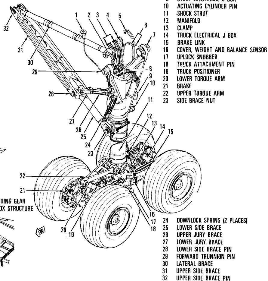
Figure 6-2. Main Landing Gear Components
