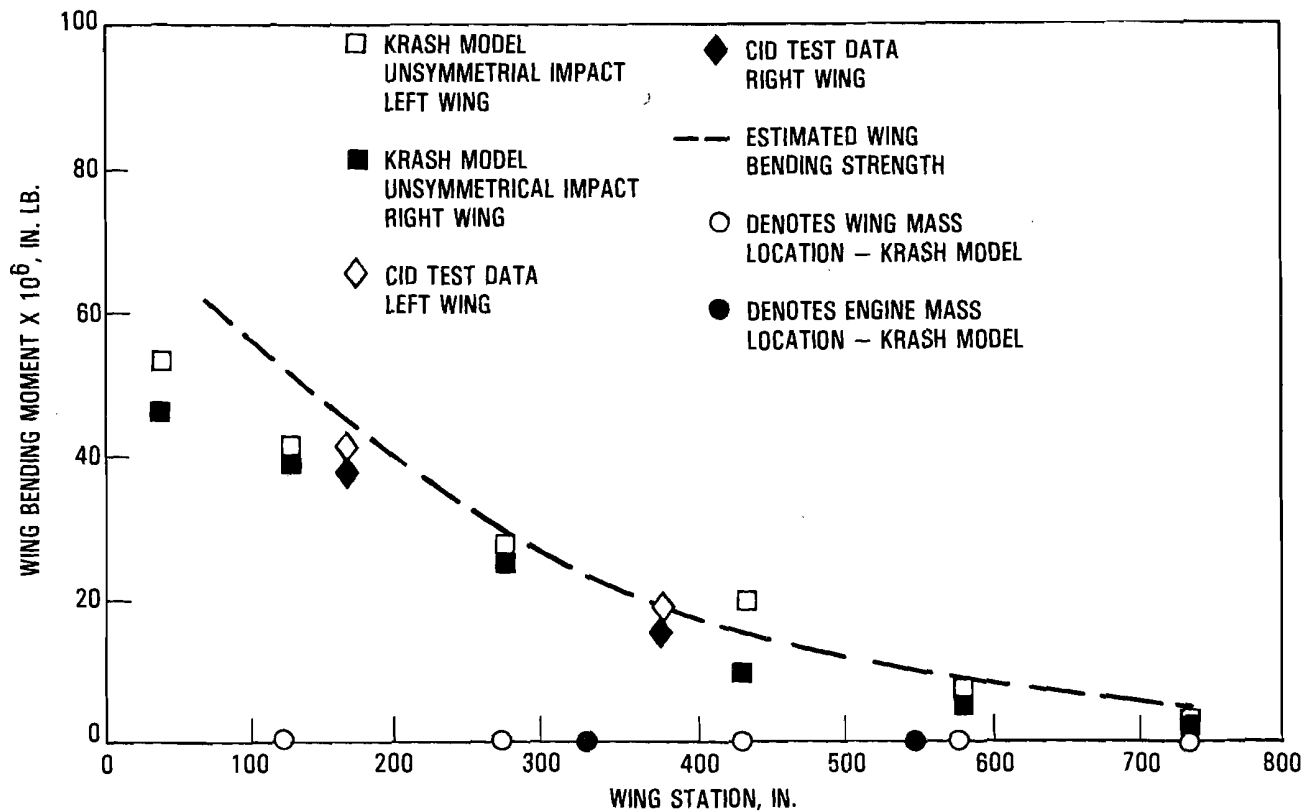
Figure 3-19. Comparison of KRASH Analysis and CID Airplane Test Wing Bending
