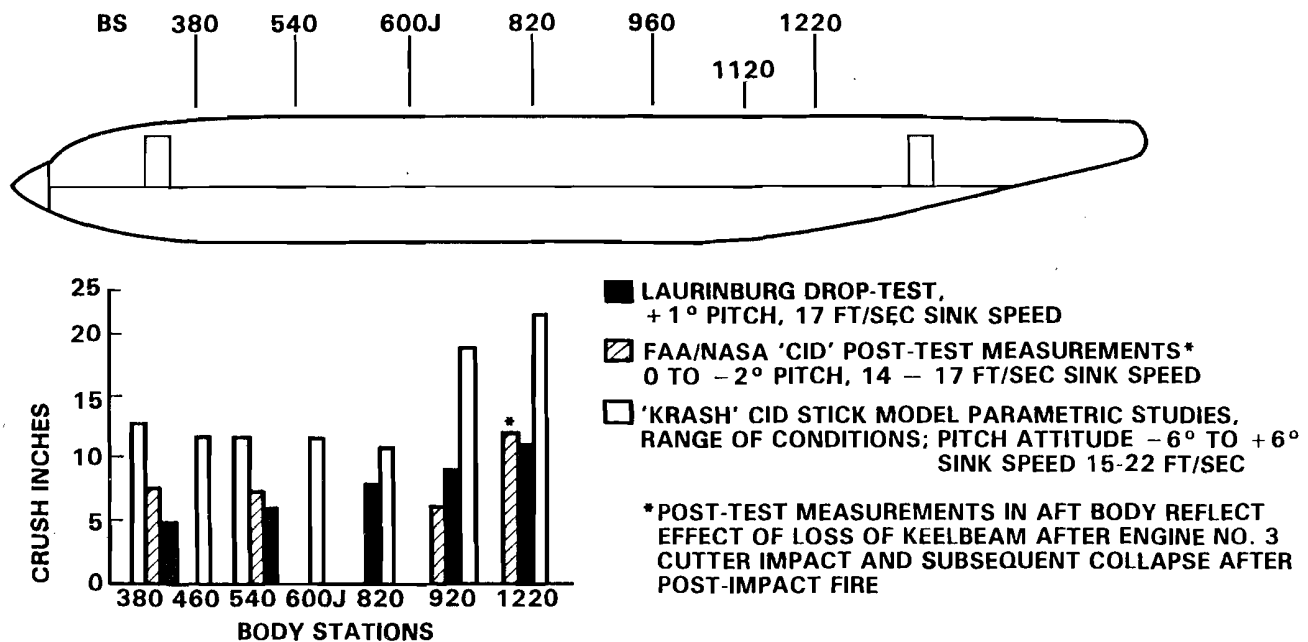
Figure 3-11. Lower Fuselage Underside Crush
