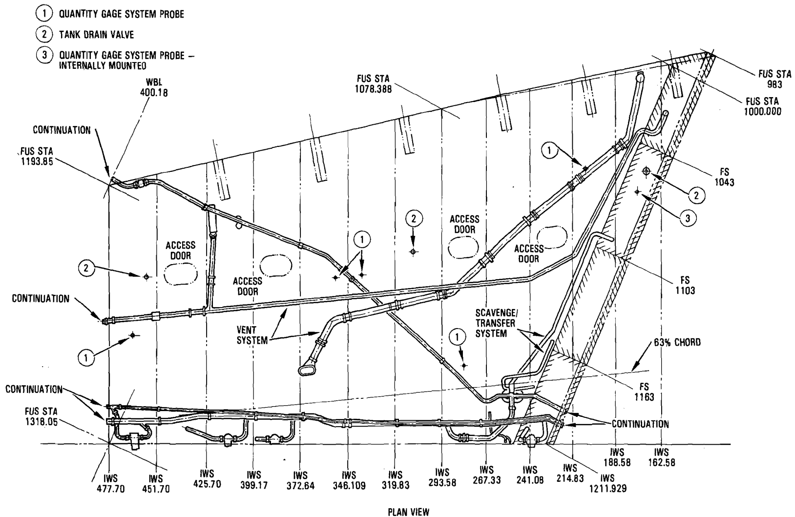
Figure 7-13. Redesign of Wing Inboard Section for CRFS
