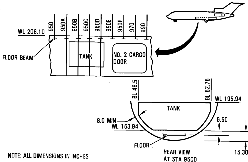
Figure B-5. Cargo Compartment Tank Installation
