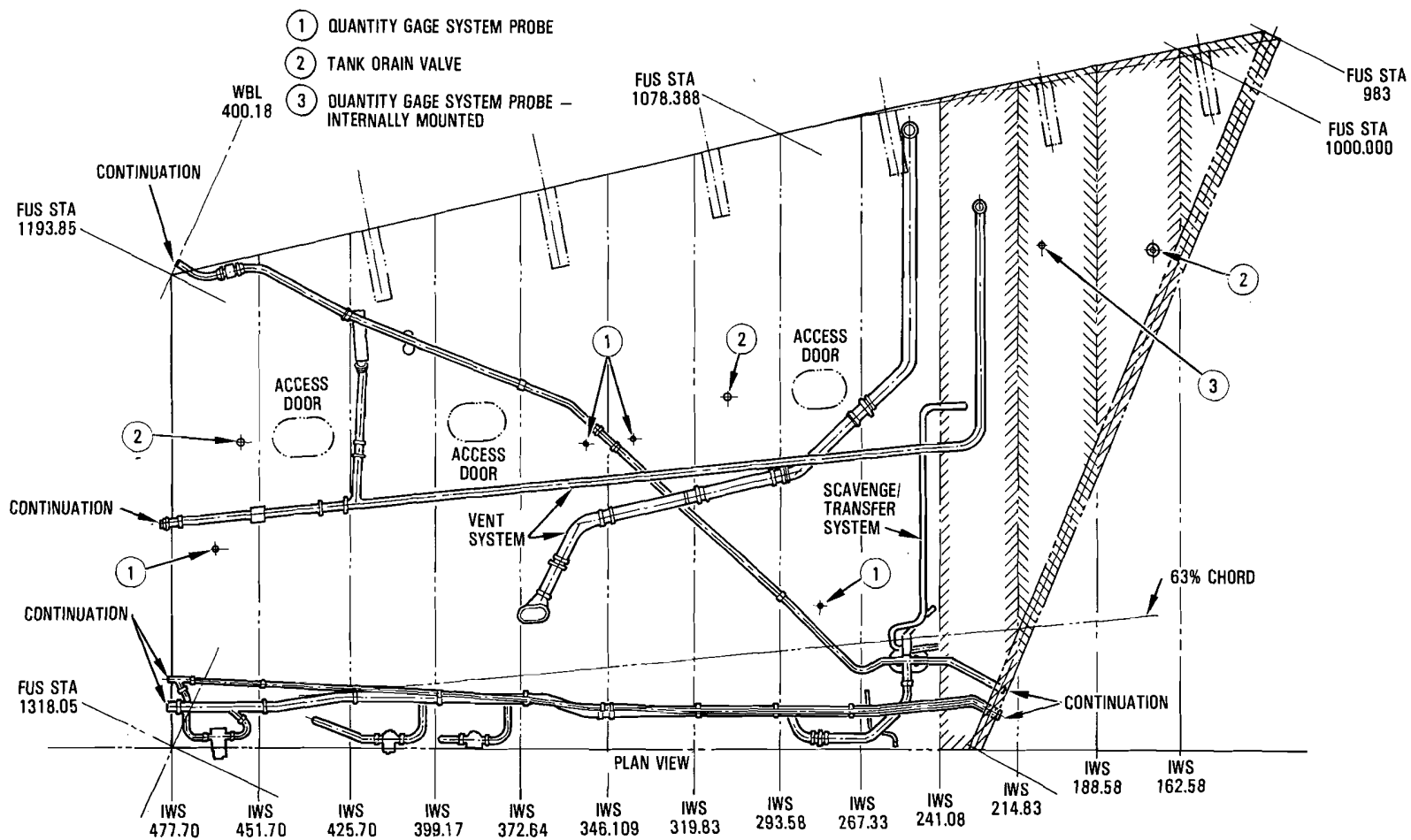
Figure 7-12. Modification of Existing Wing Inboard Section for CRFS
