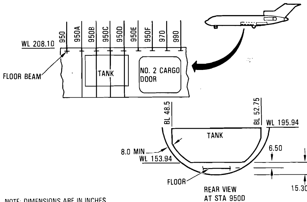
Figure 5-11. Fuel Tank General Arrangement, Narrow-Body Transport Airplane
