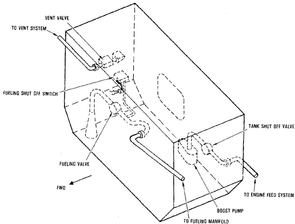
Figure 7-15. Typical Fuselage Auxiliary Tank Arrangement
