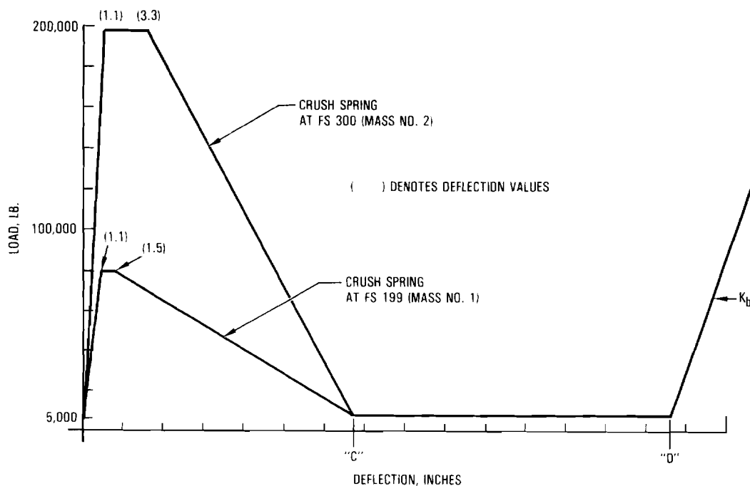
Figure 3-39. Nose Gear Bulkhead Crush Spring Characteristics
