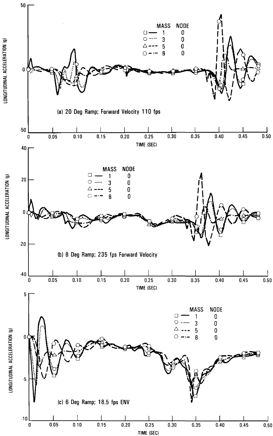
Figure 3-59. Baseline Stick Model Longitudinal Acceleration Histories
