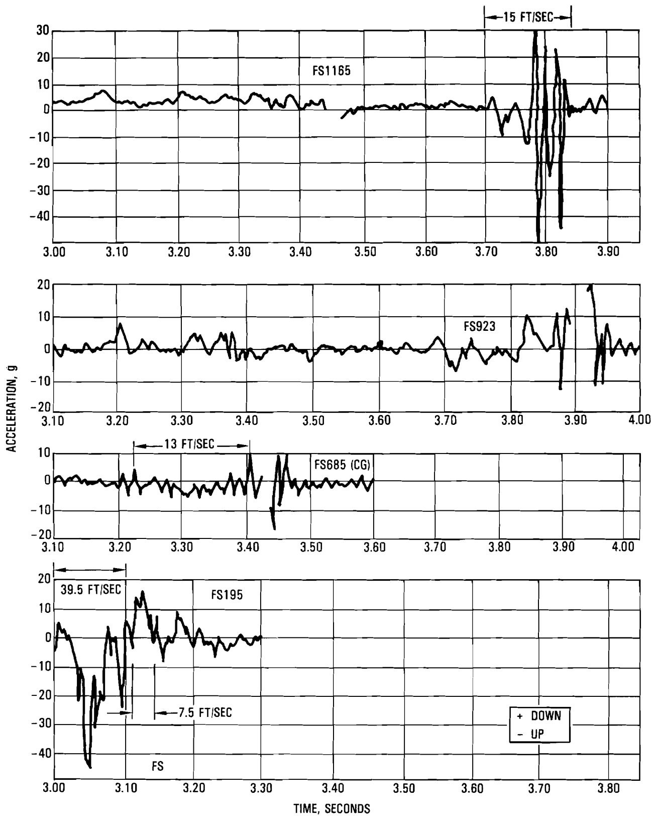
Figure 3-64b. Floor Deceleration, L1649 Test, 20 Degree Slope Impact
