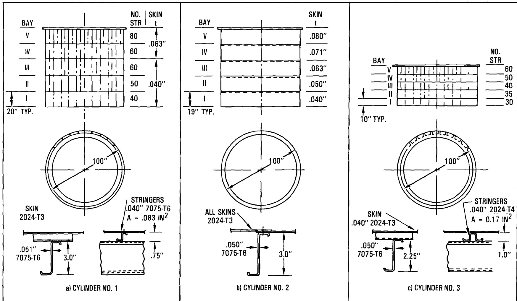
Figure 3-68. Structural Configurations, Axial Test Cylinders (Reference 4)
