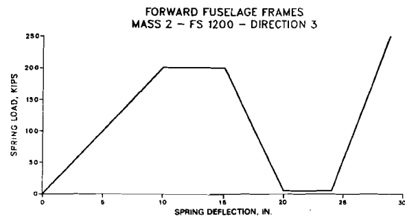
Figure 3-55. Load- Deflection Curves - Set K4
