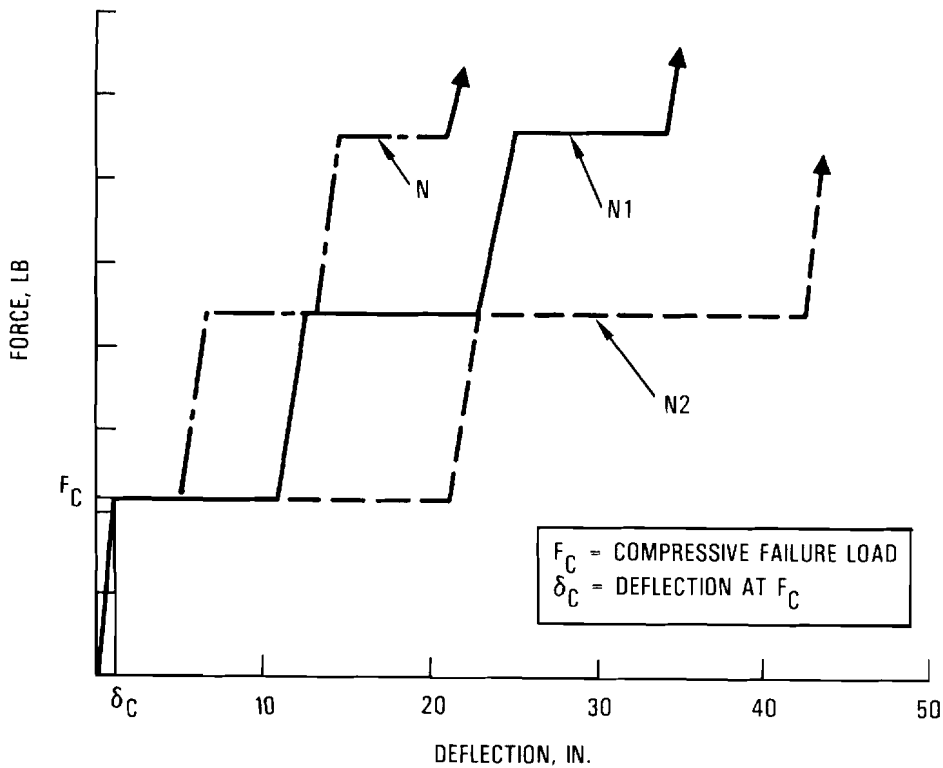
Figure 3-72. Beam Axial Non-Linear Load-Deflection Behavior
