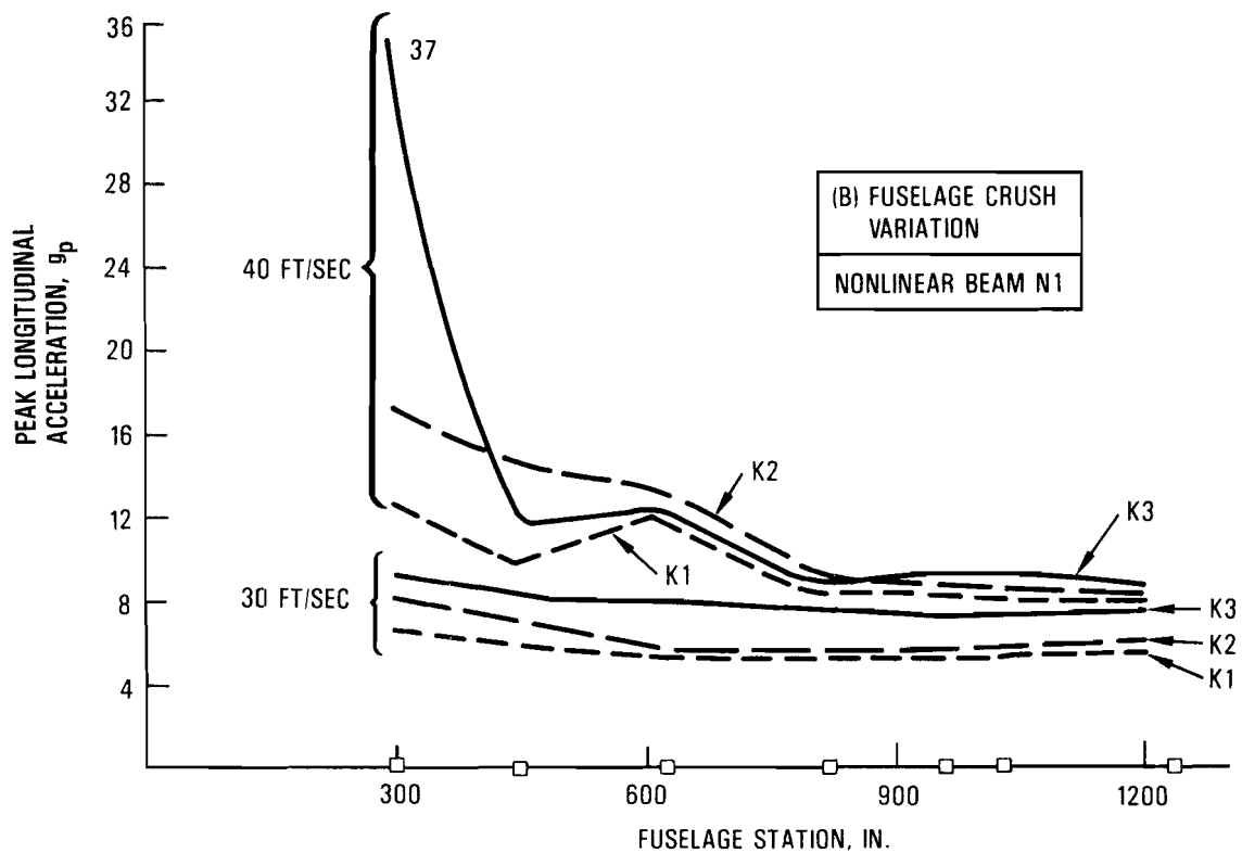
Figure 3-74. Peak Acceleration Distribution
