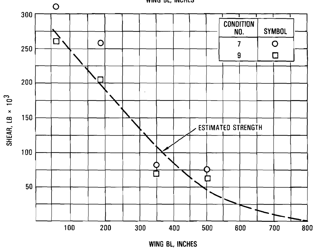
Figure 3-26. Comparison of Wing Shear and Bending, Conditions 7, 9
