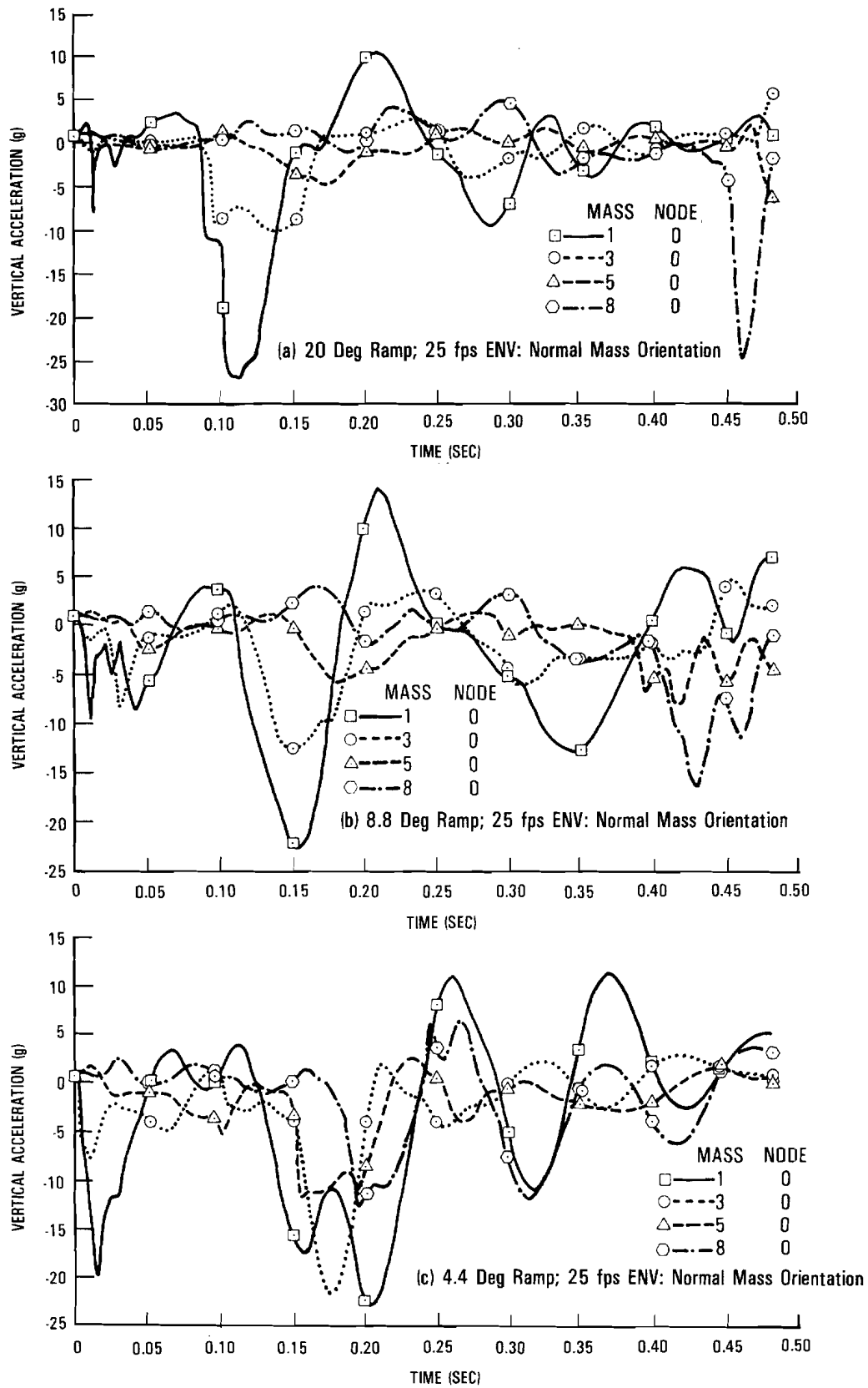
Figure 3-47. Stick Model Vertical Acceleration Histories
