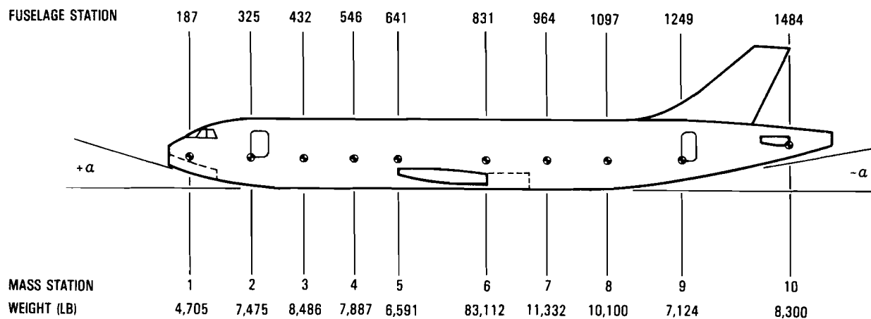
(a) REFERENCE 4 AIRPLANE CONFIGURATION
