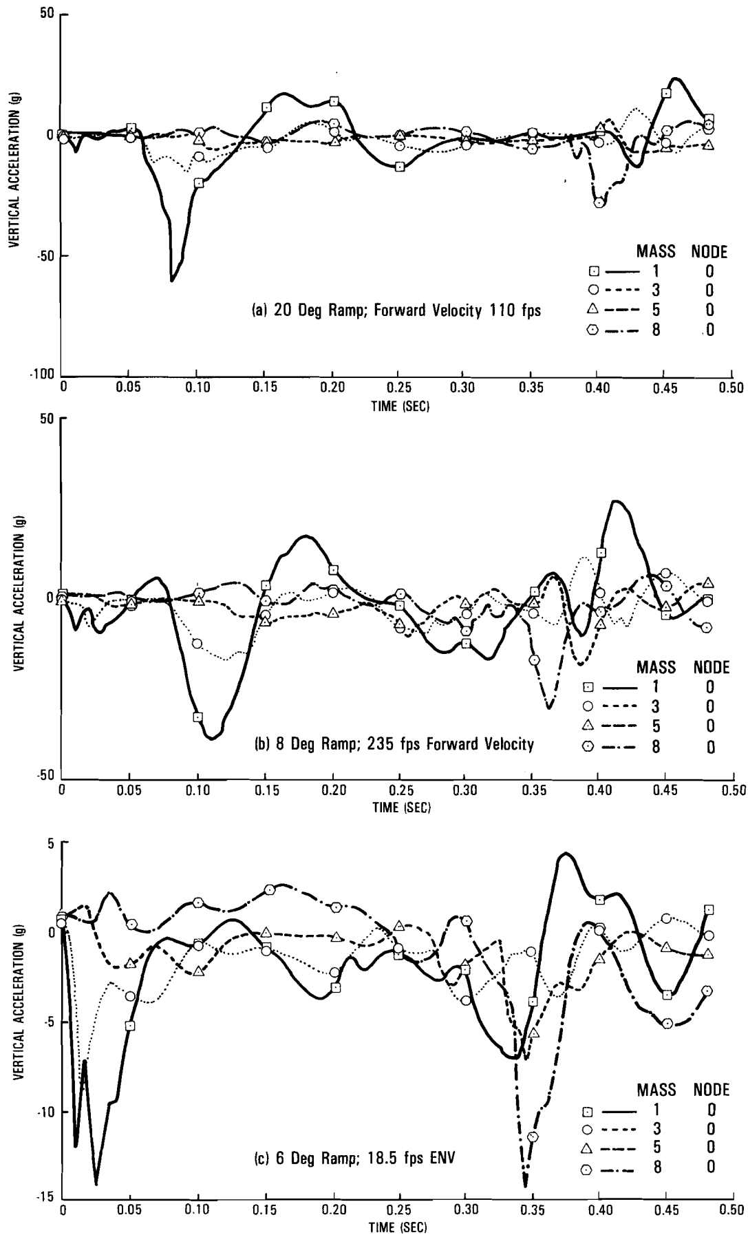
Figure 3-58. Baseline Stick Model Vertical Acceleration Histories
