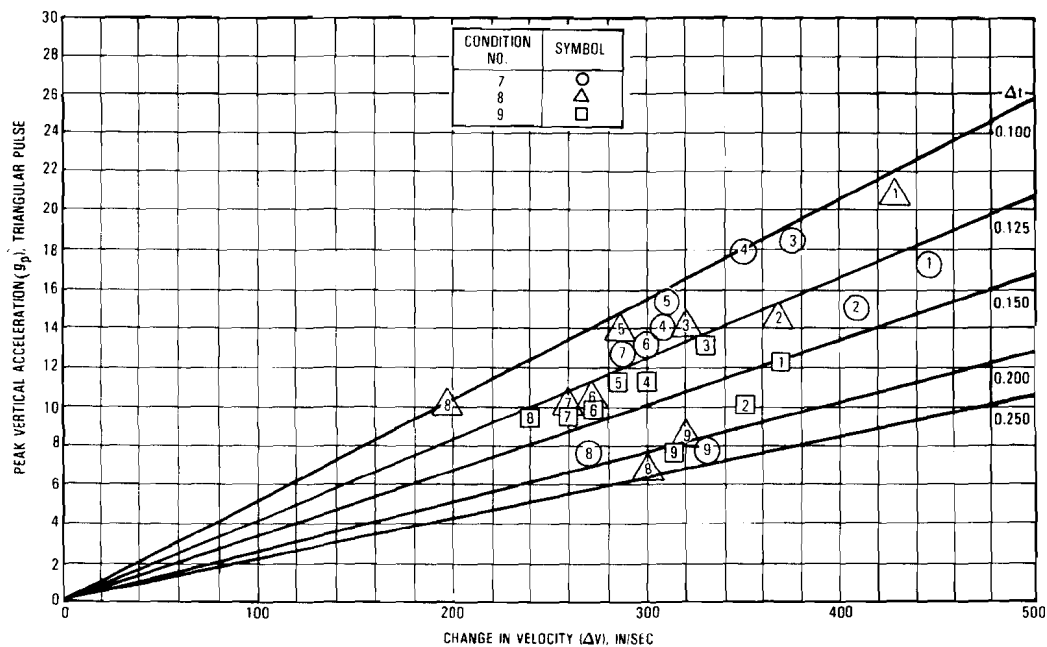
Figure 3-18. Comparison of Pulse Data for Conditions 7, 8, 9
