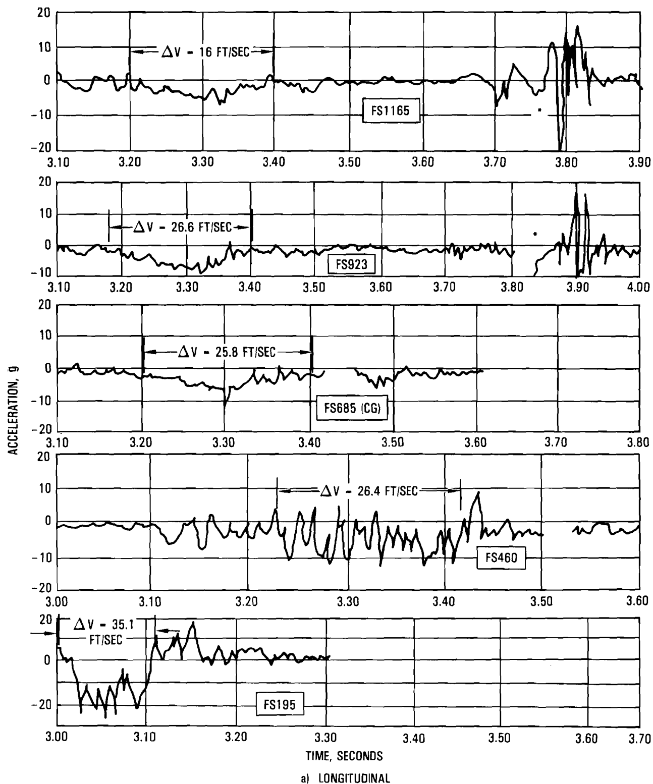
Figure 3-64a. Floor Acceleration, L-1649 Test, 20 Degree Slope Impact
