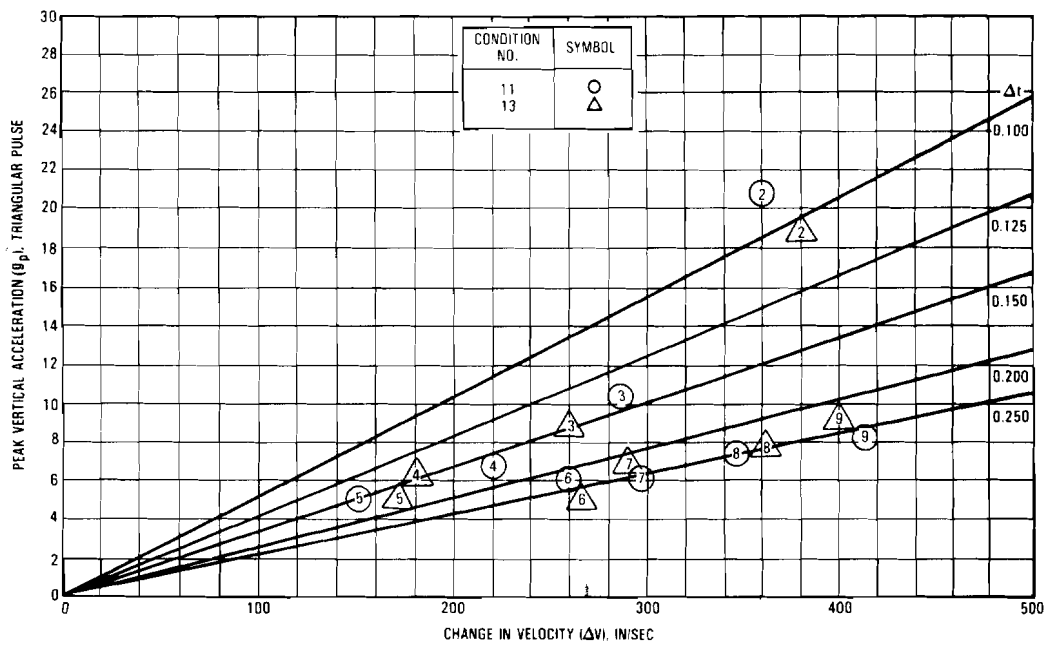
Figure 3-20. Comparisons of Pulse Data For Conditions 11, 13
