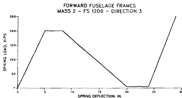
Figure 3-54. Load- Deflection Curves - Set K3
