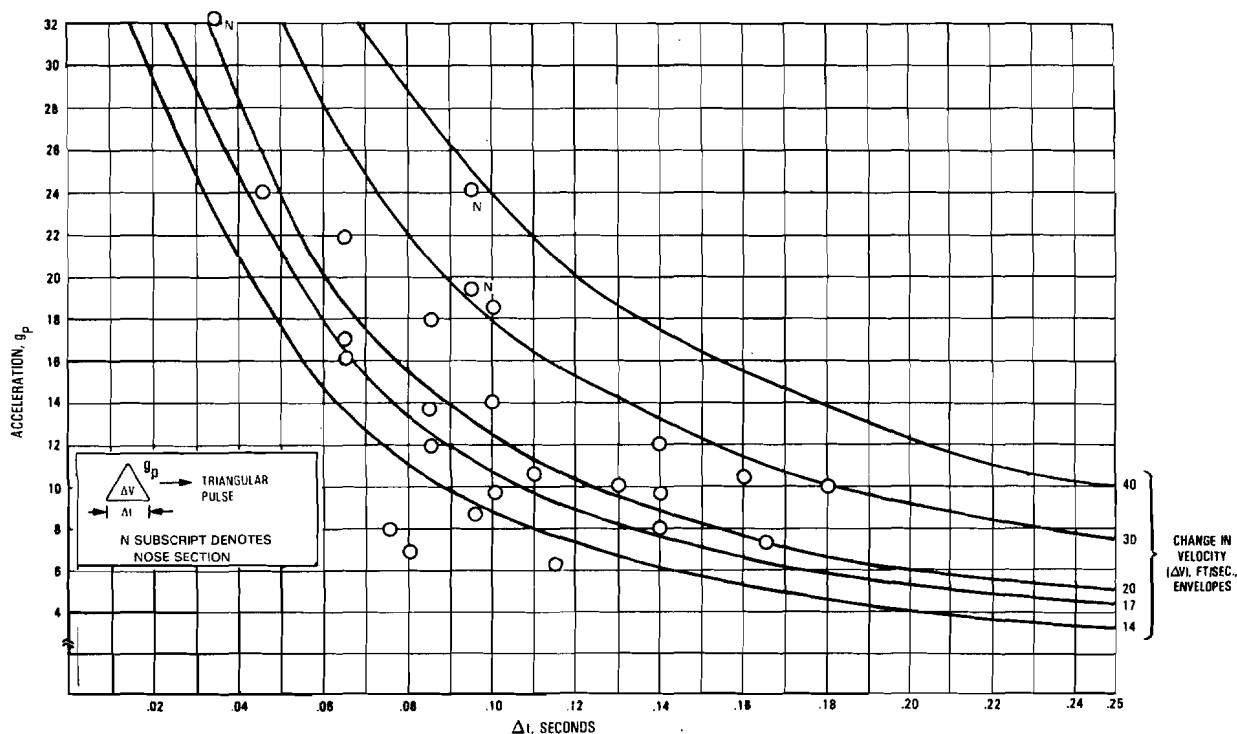
Figure 3-28. Analytically Obtained Vertical Pulses - Gears Extended Condition
