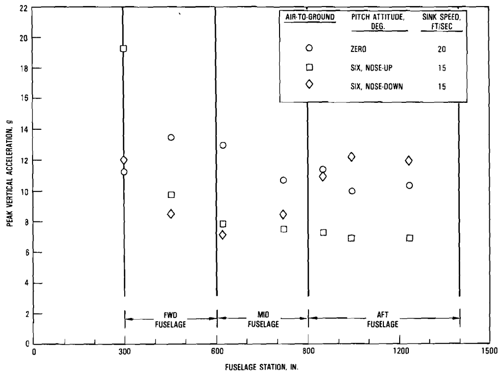
Figure 3-13. Peak Vertical Acceleration Versus Fuselage Station
