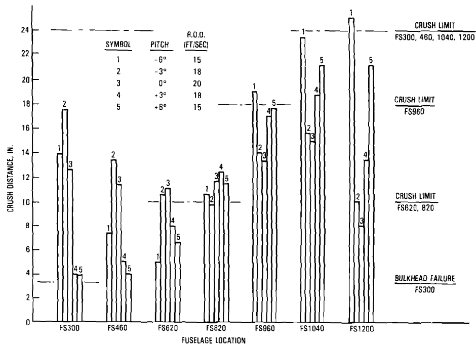
Figure 3-8. Fuselage Crush Distribution
