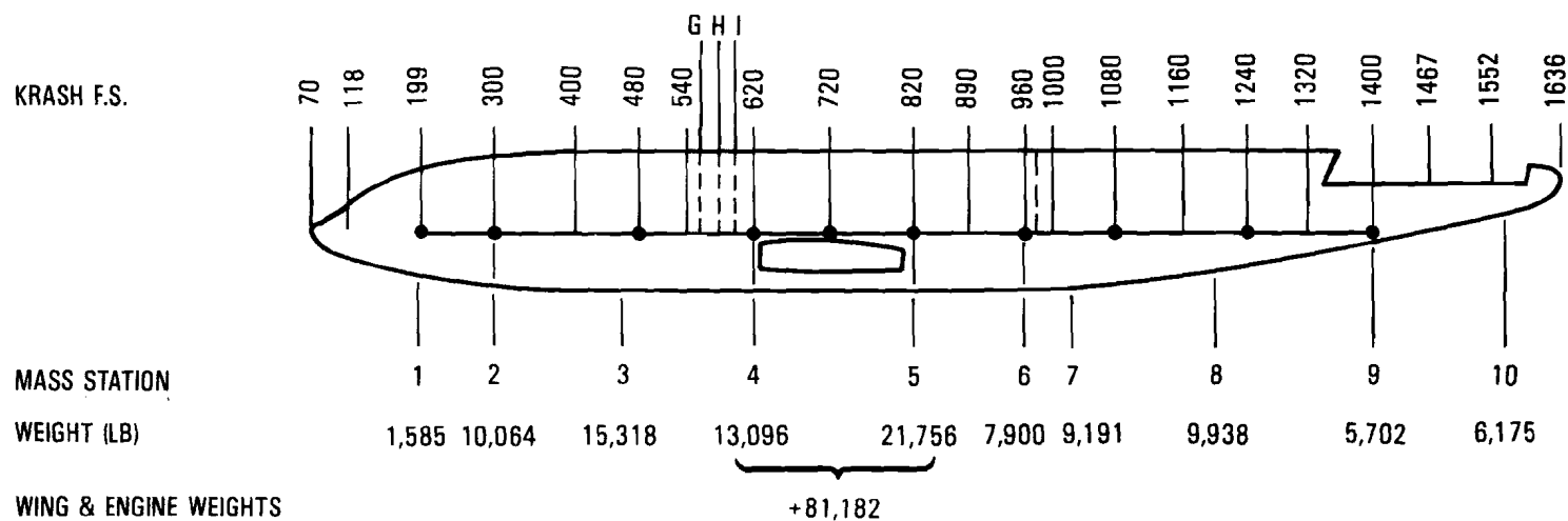
(b) CID AIRPLANE CONFIGURATION
