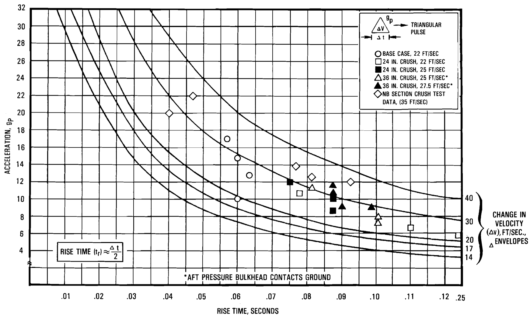
Figure 4-4. Analytically Obtained Vertical Pulses, Air-to-Ground Impact-Crush Variation
