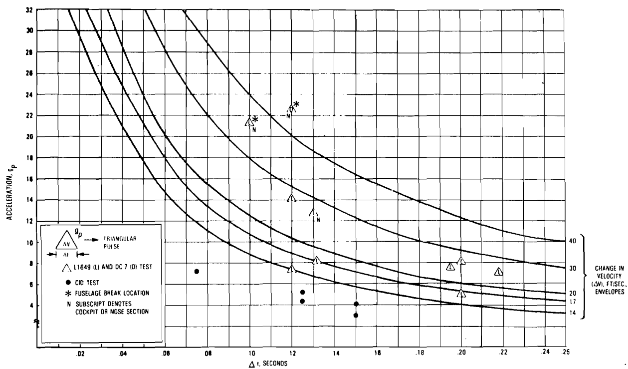
Figure 3-67. Measured Longitudinal Pulses
