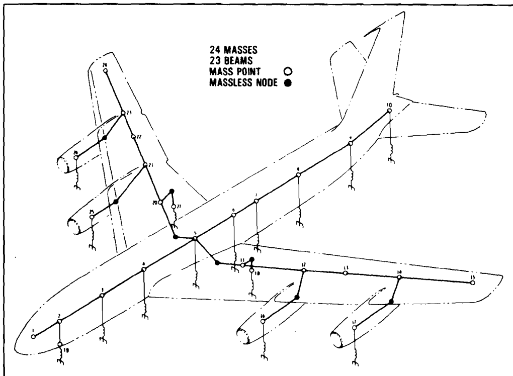
Figure 1-2. CID KRASH Stick Model
