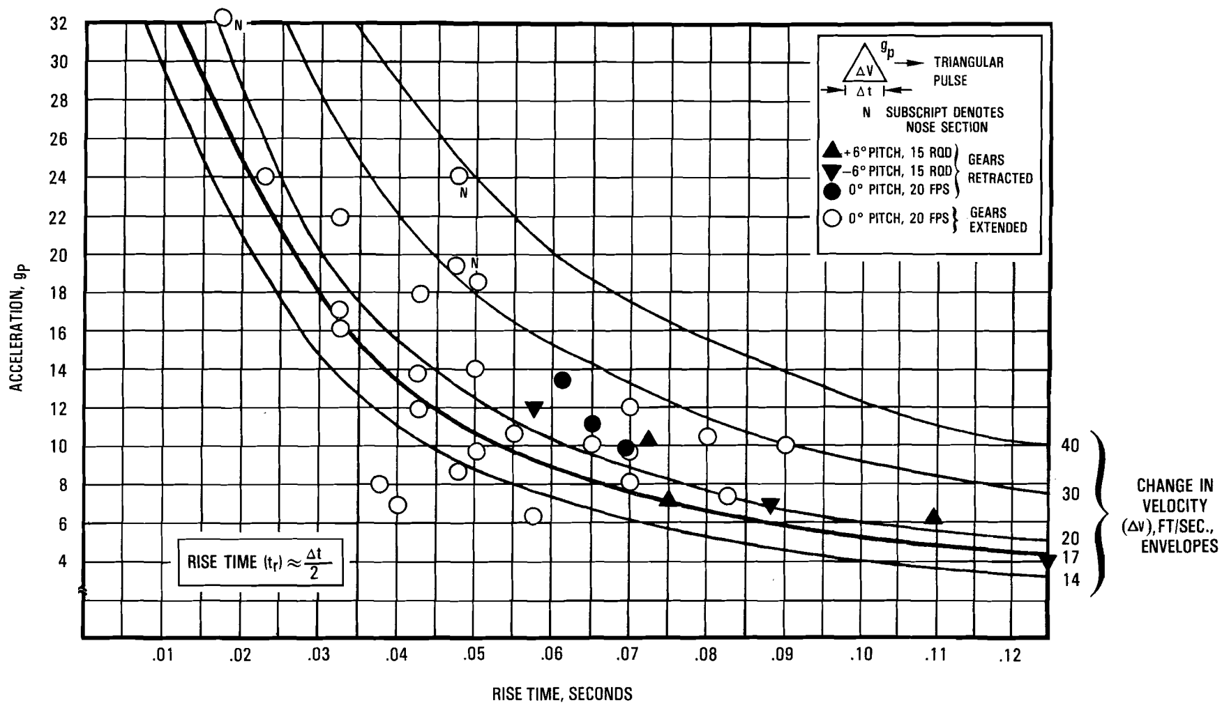
Figure 4-3. Analytically Obtained Vertical Pulses - Air-to-Ground, Gears Extended and Retracted
