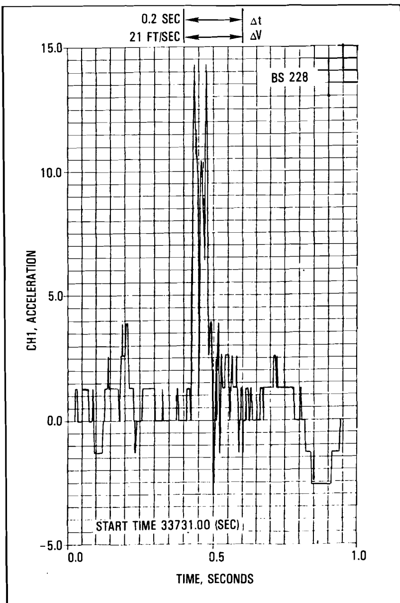
Figure 3-62. CID Test Normal (Vertical) Direction Floor Accelerations - BS228 - BS540
