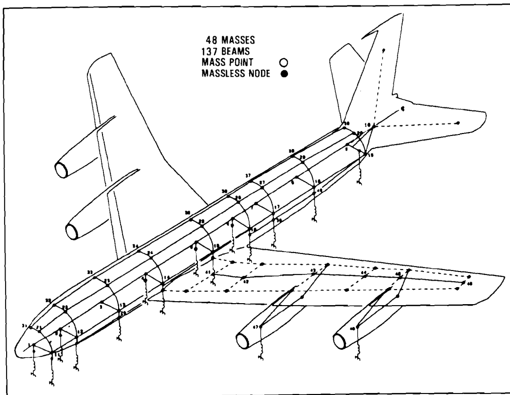
Figure 1-3. Expanded CID KRASH Model
