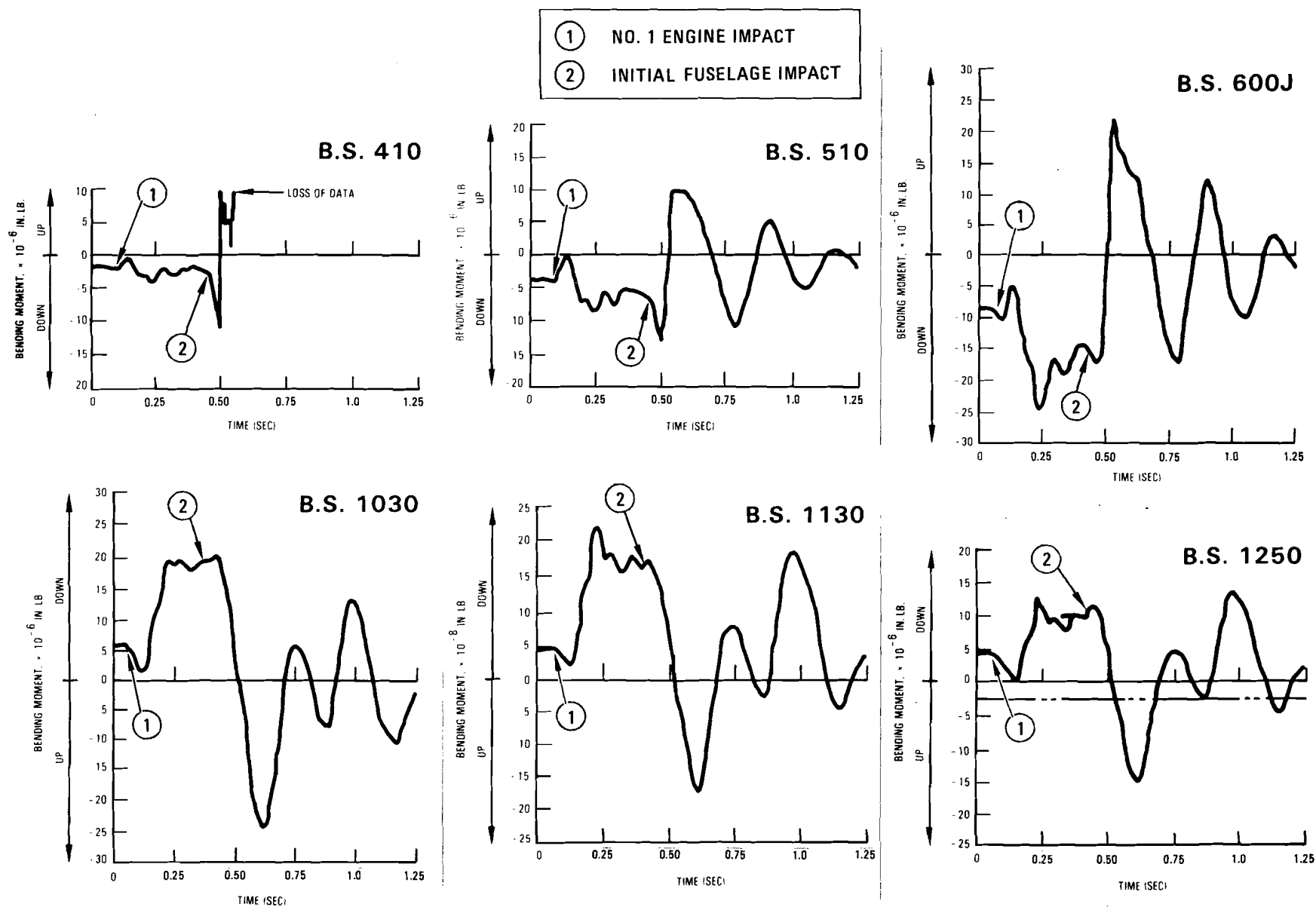
Figure 2-5. CID Test Results, Engine and Fuselage Impacts
