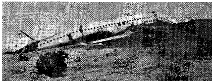
Figure 3-37. L-1649 Wreckage Shows Two Fuselage Breaks
