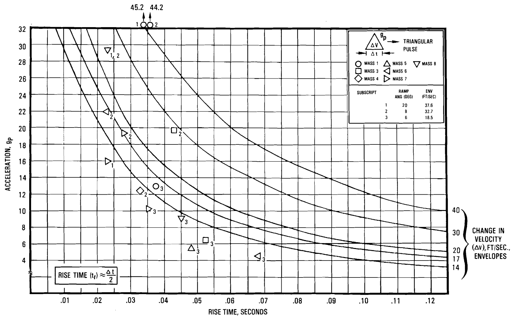
Figure 4-6. Vertical Pulses Obtained from Ramp Impacts
