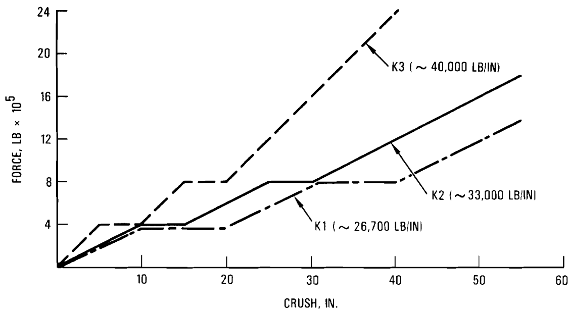
Figure 3-71. Axial Crush Spring Load-Deflection Characteristics
