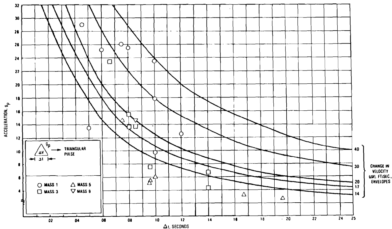
Figure 3-57. Vertical Pulses Obtained from Ramp Impacts
