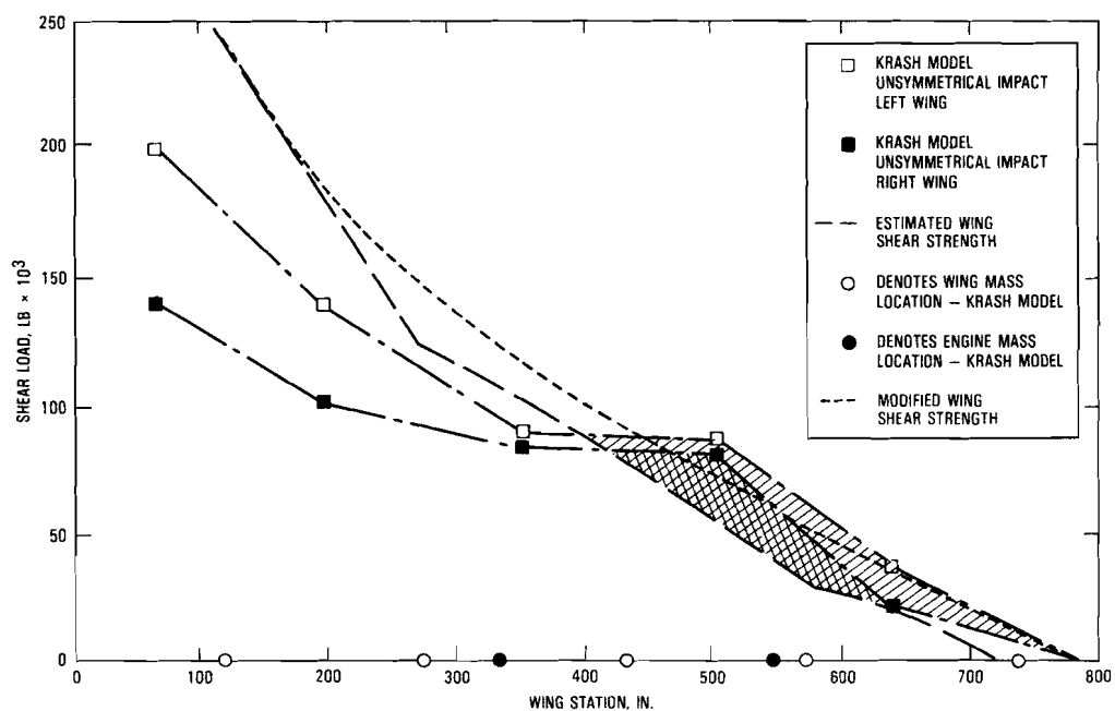
Figure 2-7. KRASH Analysis Wing Shear Distribution
