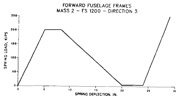
Figure 3-53. Load- Deflection Curves - Set K2
