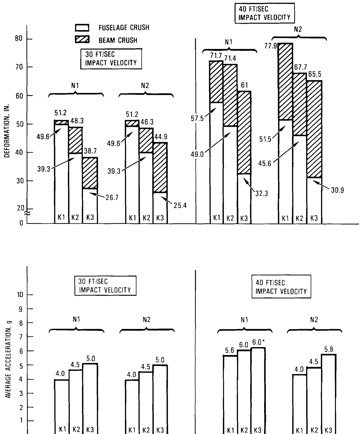
Figure 3-73. Ddeformed Distance and Average Acceleration Results
