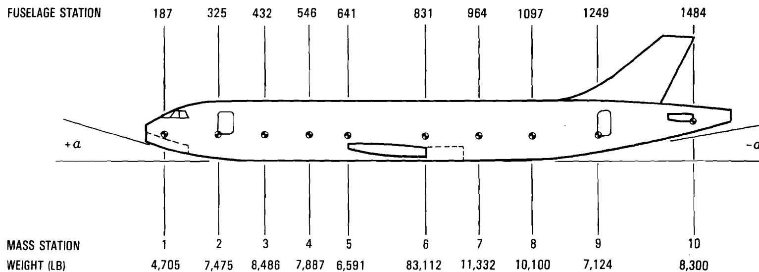
(a) REFERENCE 4 AIRPLANE CONFIGURATION
