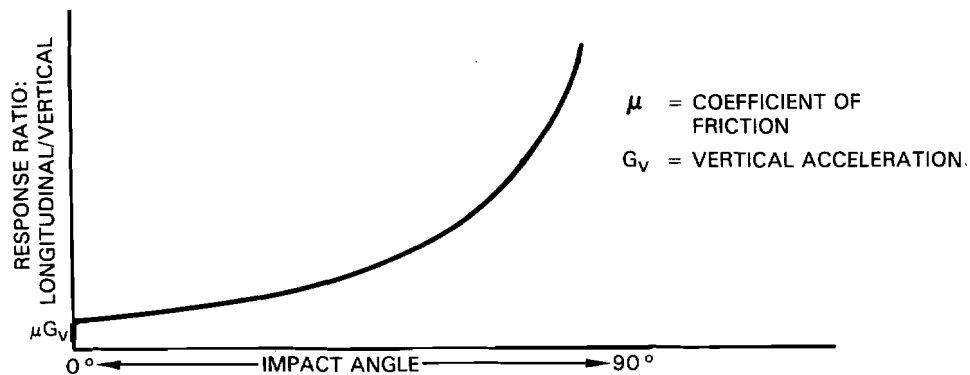
Figure 3-35. Trend of Relative Responses Versus Impact Angle
