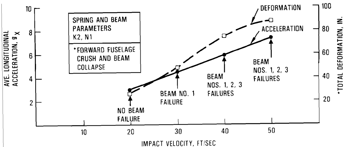
Figure 3-75. Acceleration Versus Impact Velocity
