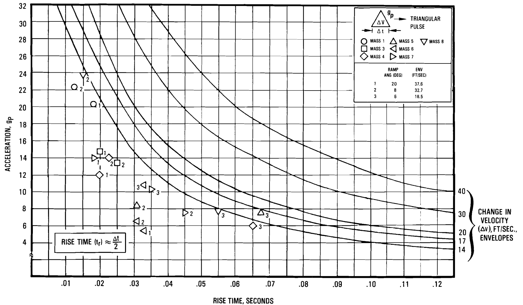
Figure 4-5. Longitudinal Pulses Obtained from Ramp Impacts
