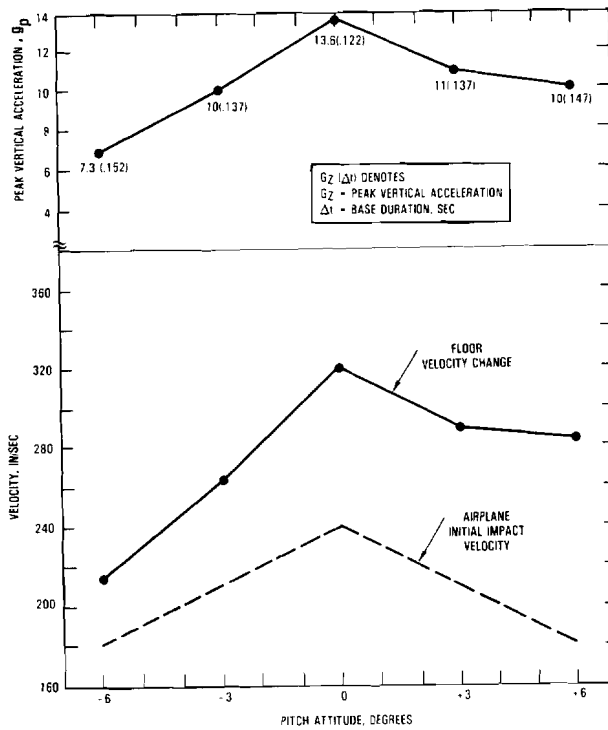
Figure 3-9. Forward Fuselage Floor Dynamic Triangular Pulse Parameters as a Function of Airplane Pitch Attitudes at Impact
