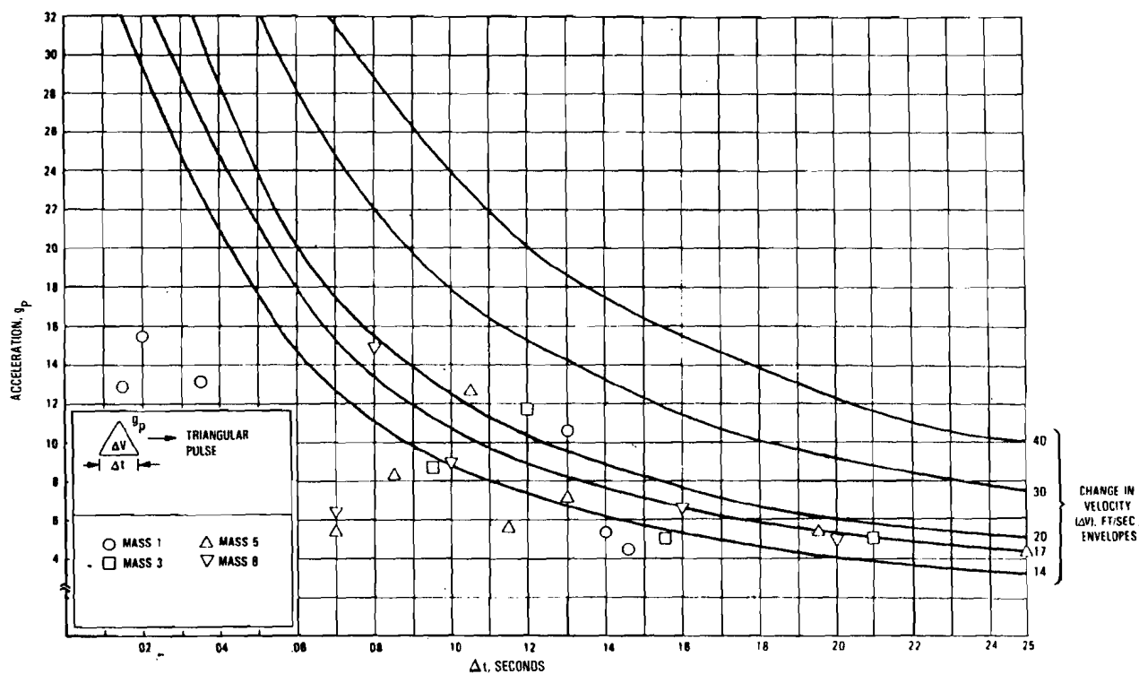
Figure 3-56. Longitudinal Pulses Obtained from Ramp Impacts
