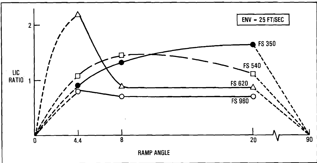
Figure 3-49. LIC Ratio Versus Ramp Angle, ENV = 25 ft/sec
