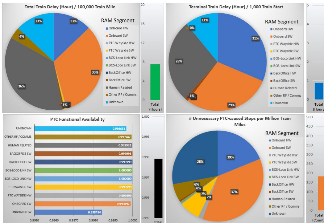
Figure 61. Aggregate RAM KPI Distribution per RAM Segment with Reduction in the Time to Swap a Lead Locomotive to 30 Minutes
