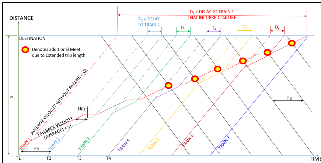
Figure D1. Illustration of Train Delay Impact due to Onboard HW Failure for Scenario 1 Where Passing Trains are Affected
