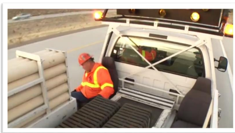
Figure 19. ADOT cone truck (44).
