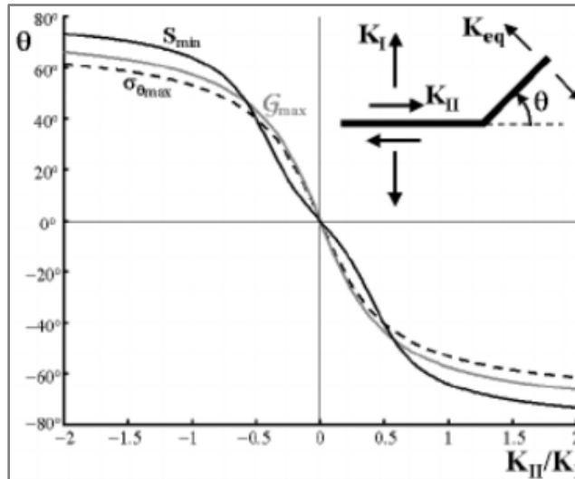
Figure 50. Crack Propagation Angle \theta Prediction
