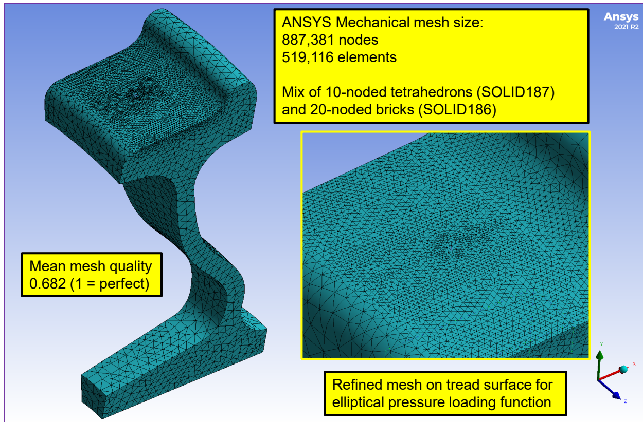
Figure 72. Baseline Computational Mesh
