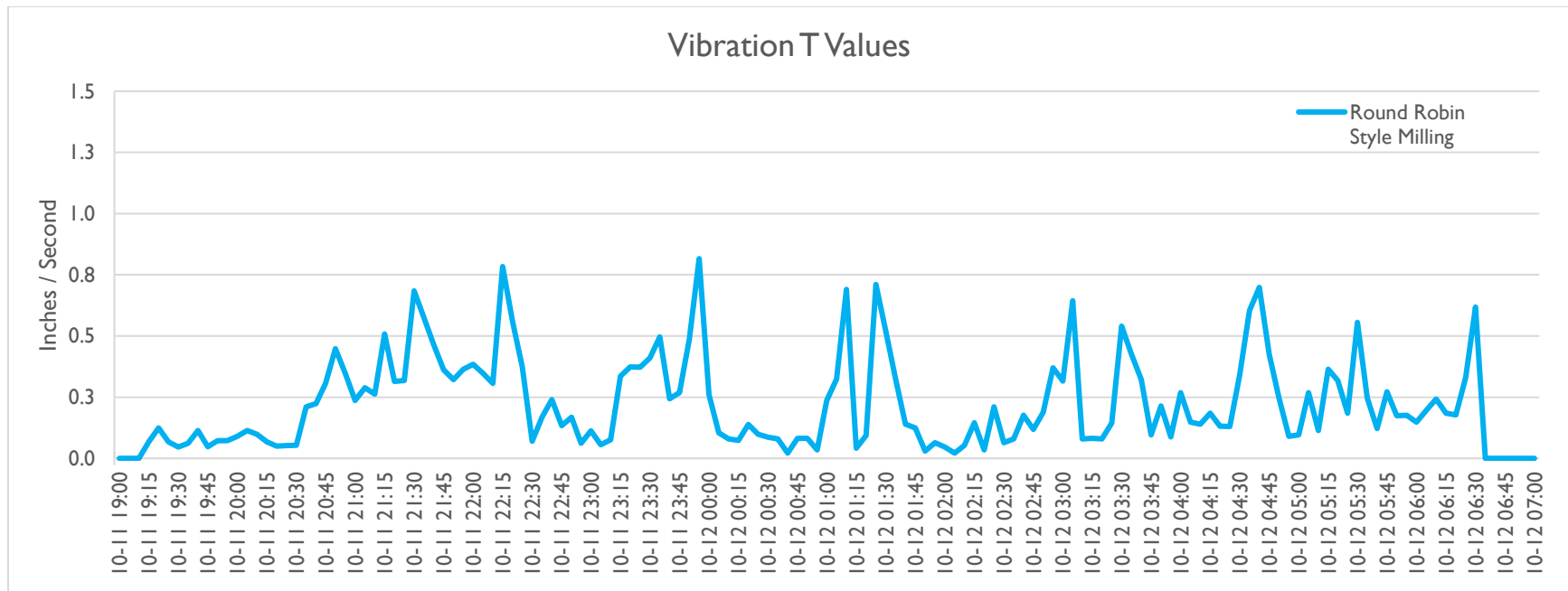
Figure 7. Round Robin Style Milling Transverse Vibration Example
