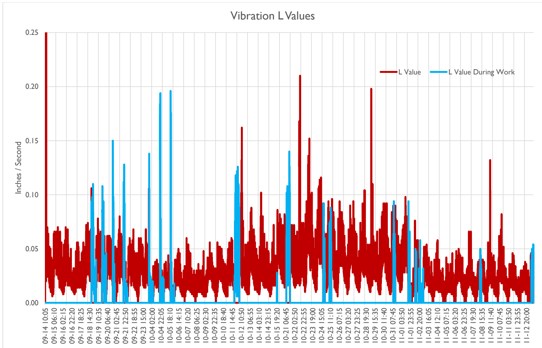
Figure 4. Lateral Vibration Values
