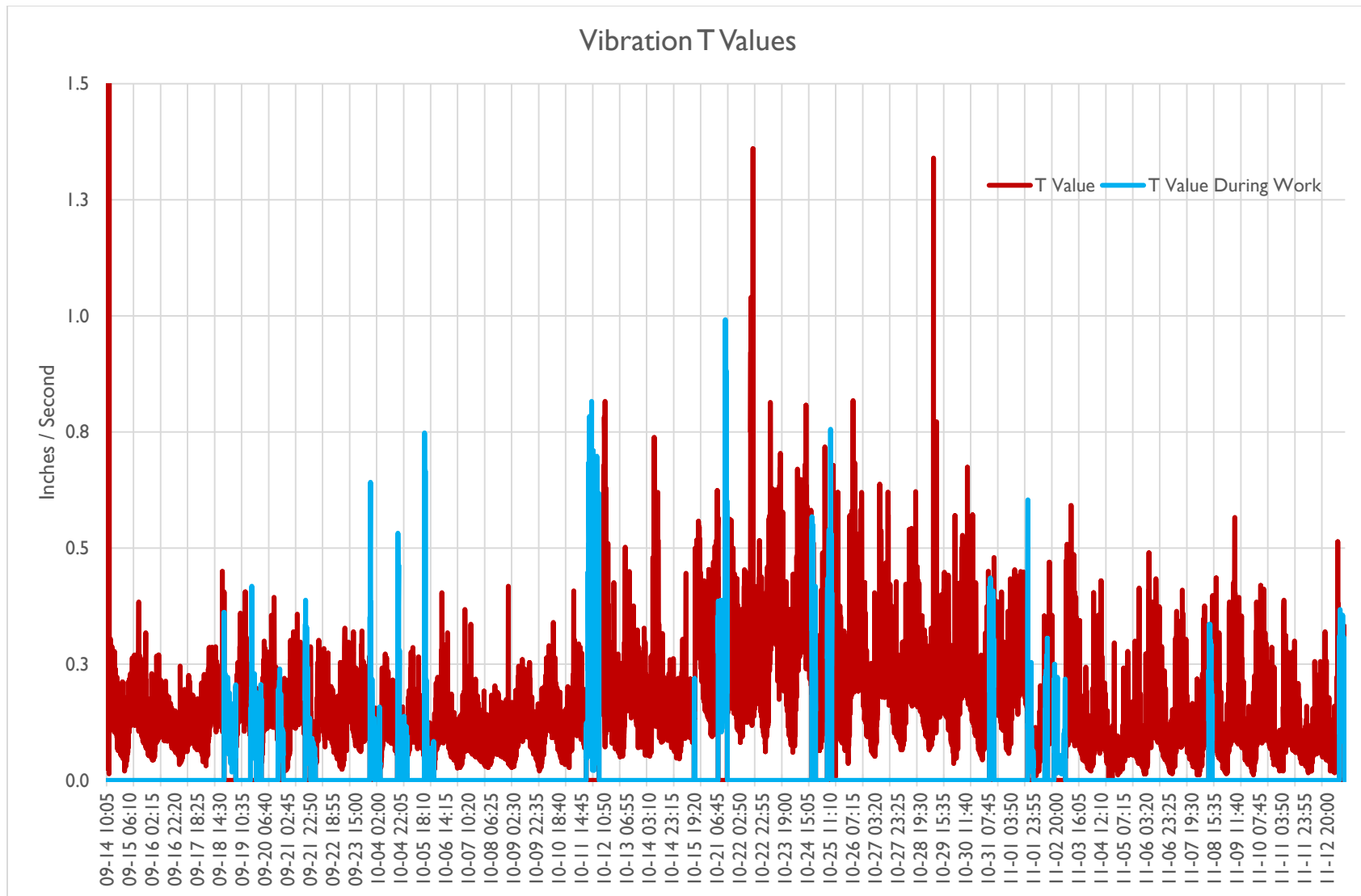
Figure 5. Transverse Vibration Values
