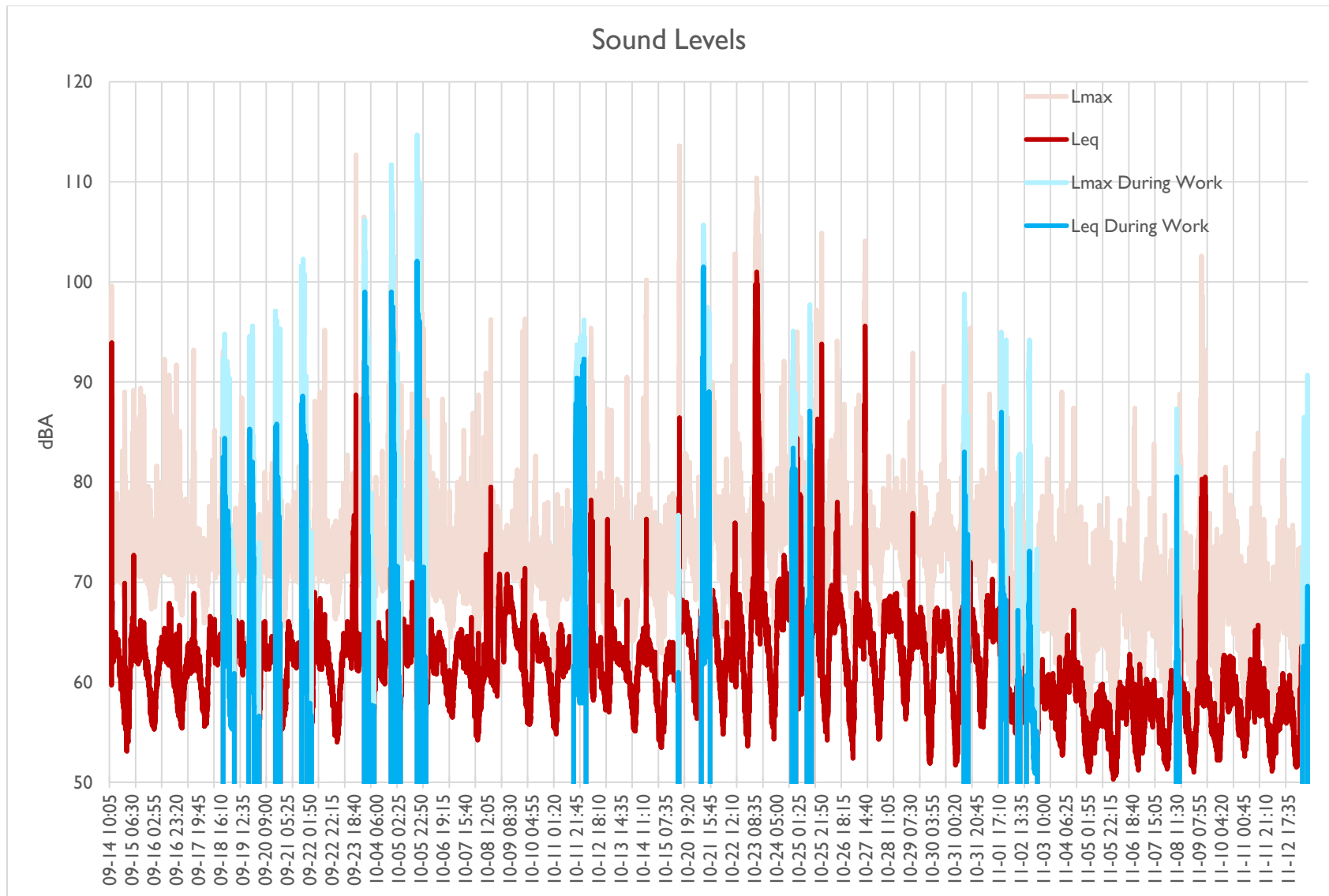
Figure 6. Sound Level Values
