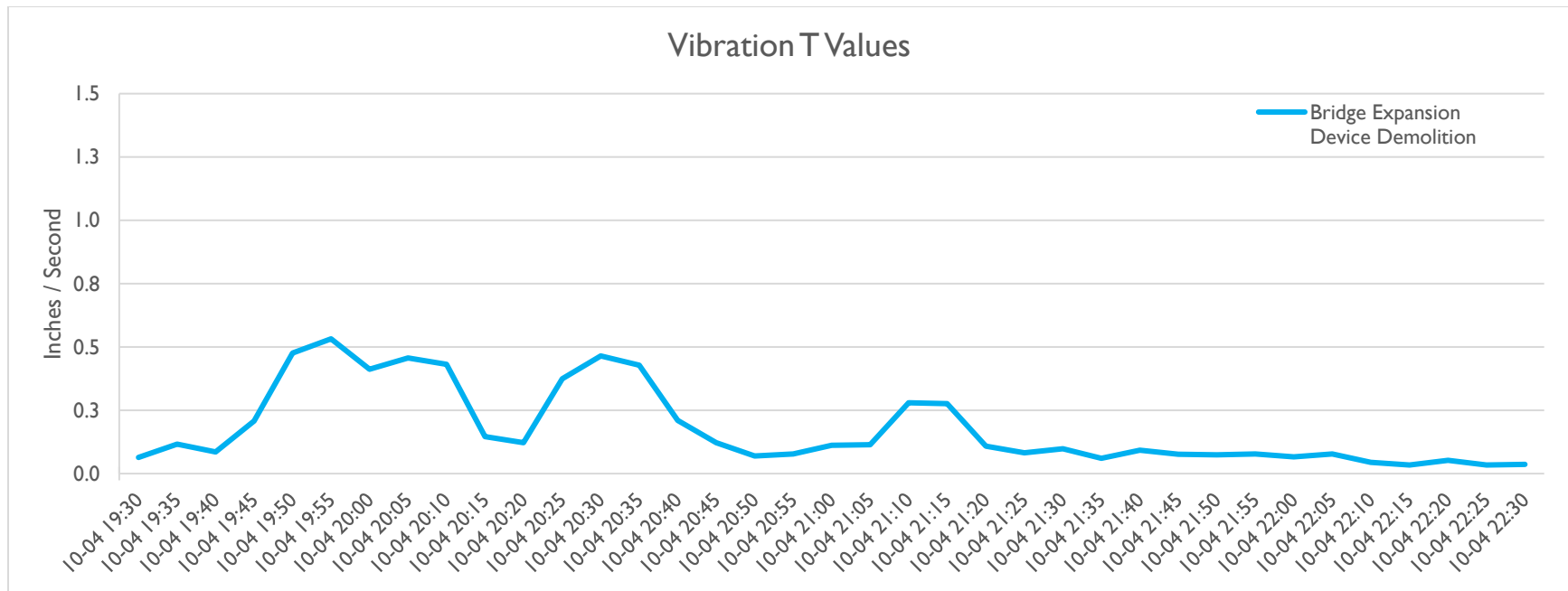
Figure 8. Bridge Expansion Device Demolition Transverse Vibration Example
