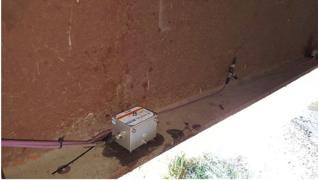
Figure 3. Photo of mounted vibration sensor
