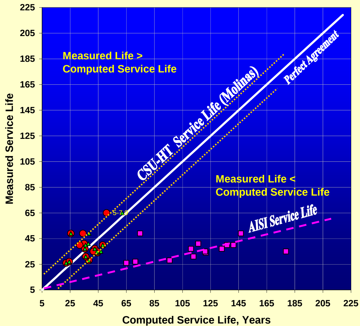
Figure 14. Measured and computed service lives using: i) AISI eq. ; ii) CALTRANS eq.; iii) Modified CALTRANS equation (CSU-HT)
