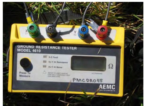
Figure 8. Soil resistivity measuring equipment
